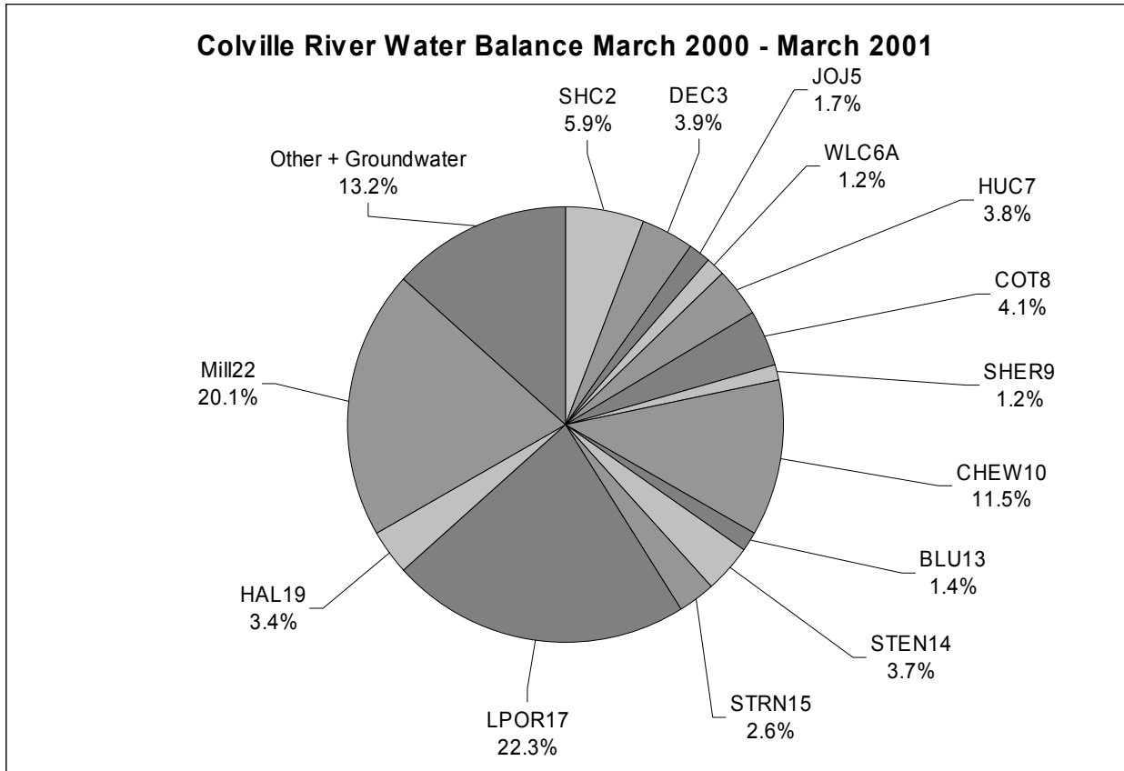
Figure 4. Estimated tributary contribution to the Colville River for the March 2000 through March 2001 study period.
