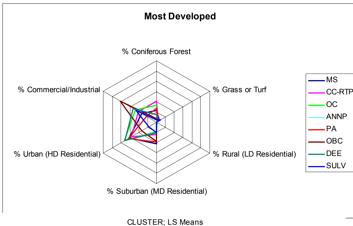
Figure 8-39. Web Plot and Membership of the Most Developed Cluster (Cluster 4)
