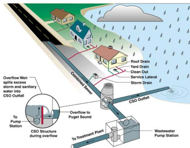
Figure 5-16. 1992. Combined Sewer Overflow Includes Flows from Stormwater from Streets, Roofs, and Foundation Drains as well as Infiltration Flow (COB 2003)
