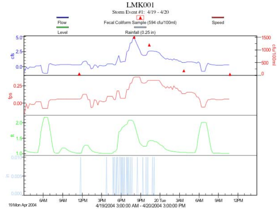
Figure 7-48. Storm-Event Response for Selected Stormwater Outfalls in the Sinclair-Dyes Inlet Watershed During the 2003-2004 Storm Season (TEC 2004)
