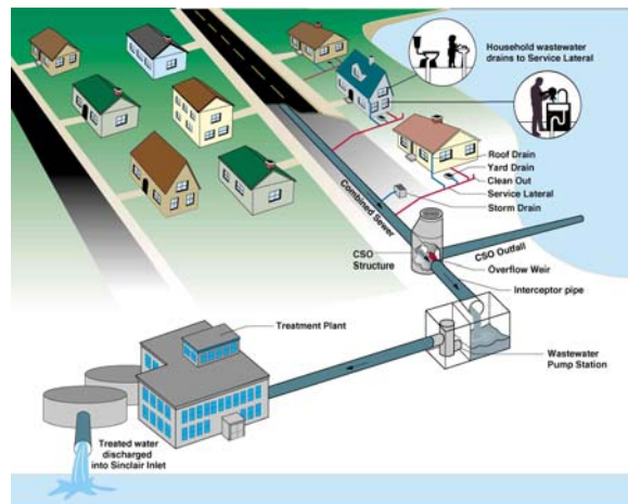
Figure 5-15. 1974: System Upgrade Reroutes Flows to Wastewater Treatment Plant
