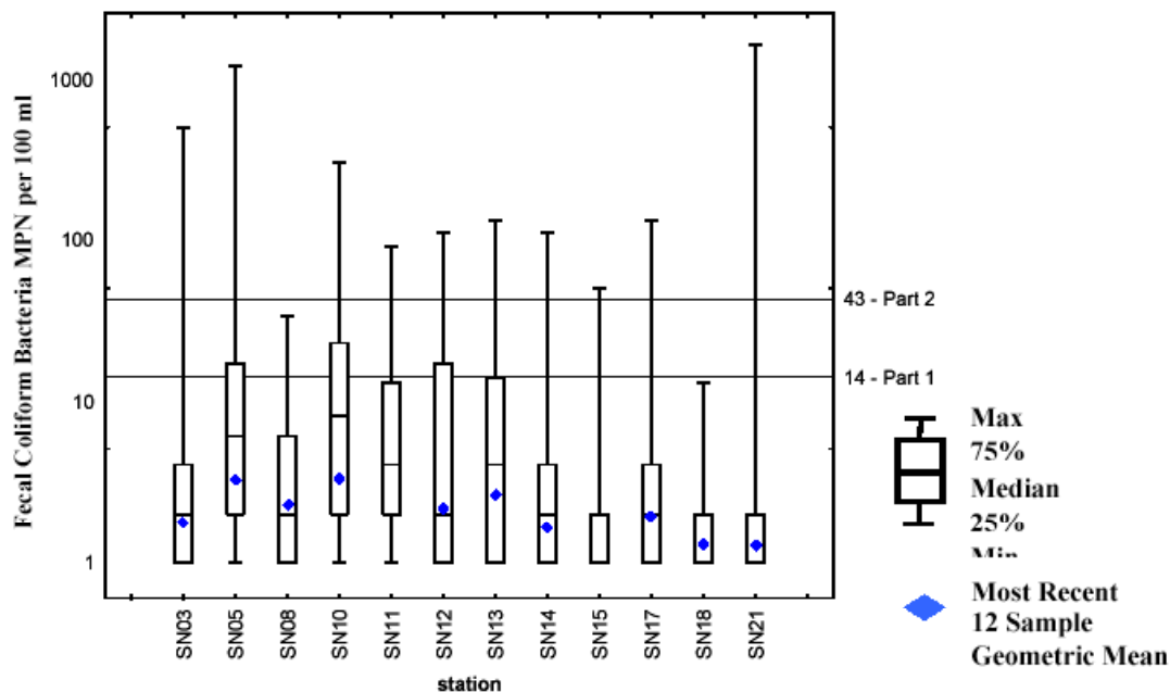
Figure 5-7. Sinclair Inlet Marine Water-Quality Data Summary for 1996-2003 (KCHD 2004)
