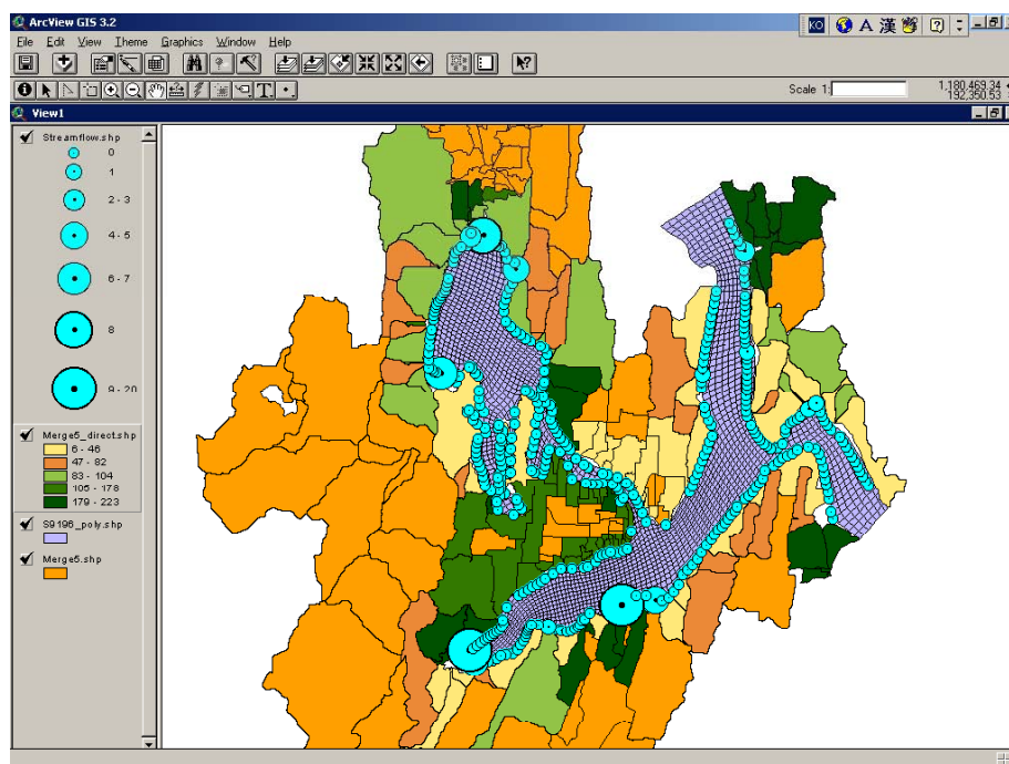
Figure 8-69. The CH3D Model Input for Sinclair-Dyes Inlet Showing Relative Pour-Point Flow Magnitudes Calculated from the HSPF Watershed Model
