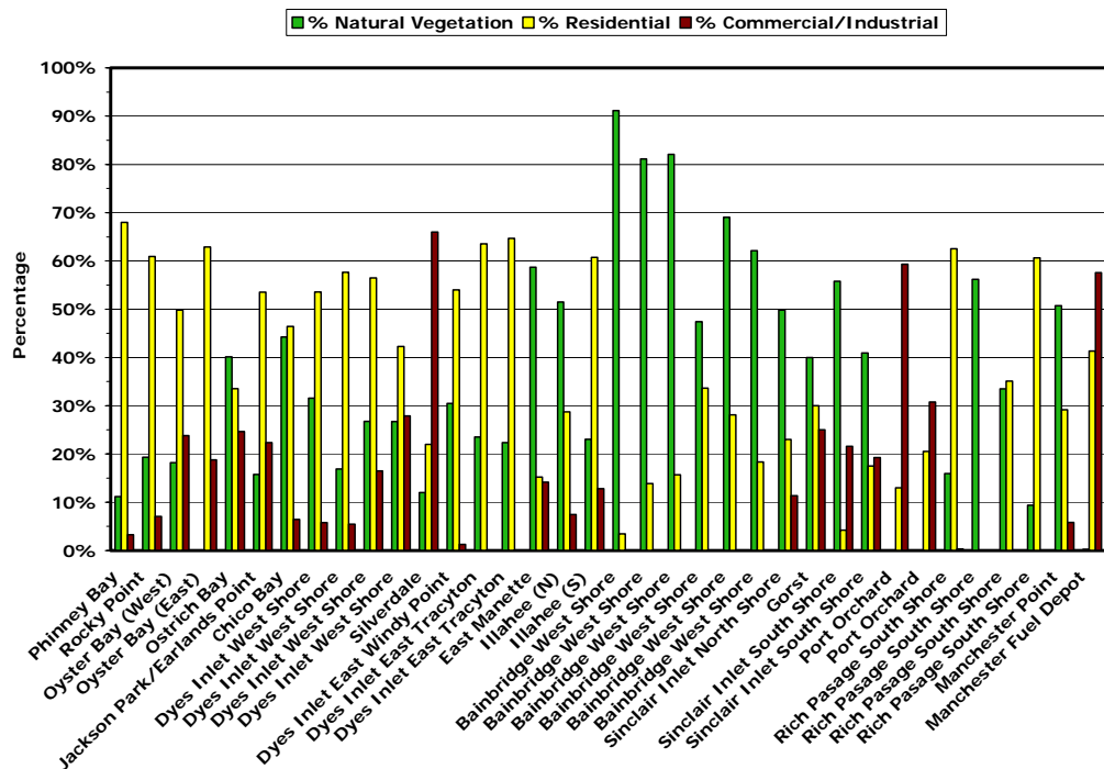
Figure 7-1. Shoreline Drainage Basin Land-Use and Land-Cover Summary for the Sinclair-Dyes Inlet Watershed
