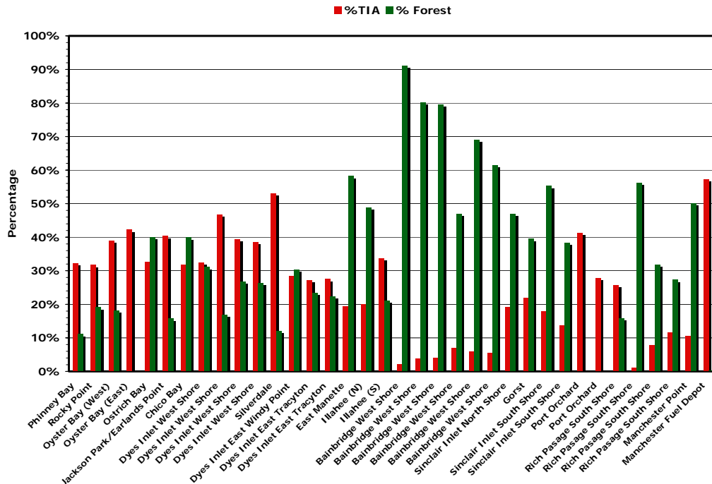
Figure 7-2. Shoreline Drainage Basin Total Impervious Area and Native Forest Cover Summary for the Sinclair-Dyes Inlet Watershed
