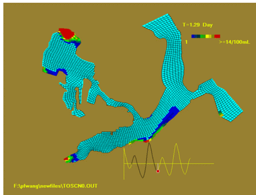
Figure 8-71. The CH3D Model Results For Sinclair-Dyes Inlet Showing the Output from a Simulated Storm Event that Results in Polluted Stream Outflow at Several Locations
