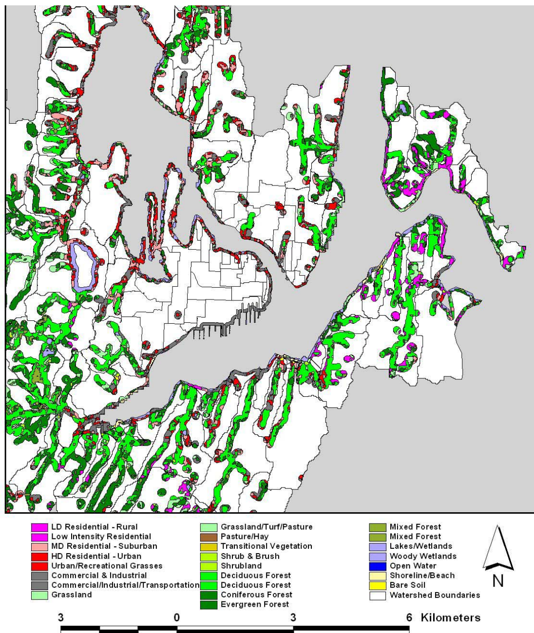
Figure 3-17. Sinclair-Dyes Inlet Watershed Riparian Assessment Results
