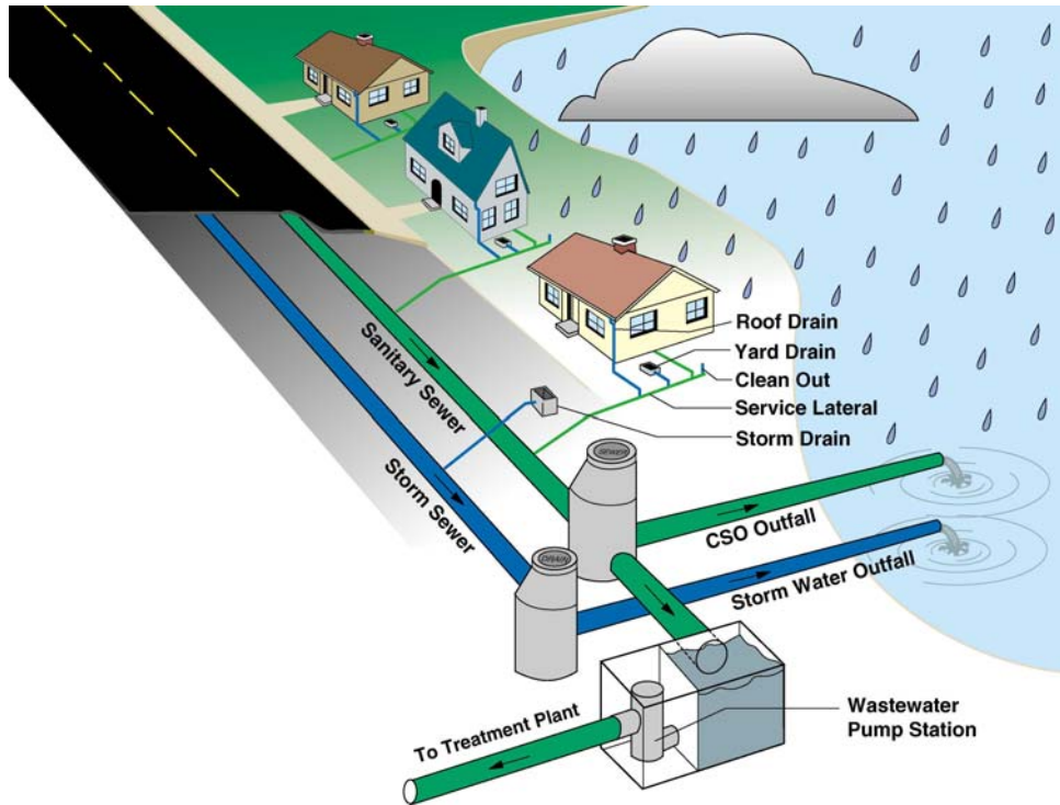
Figure 5-17. 2000-Current: Combined Sewer Overflow Reduced Through Separated Stormwater System; Street Runoff Removed from System; Private Property Runoff Still Enters Sanitary Sewer System Contributing to Combined Sewer Overflows (COB 2003)
