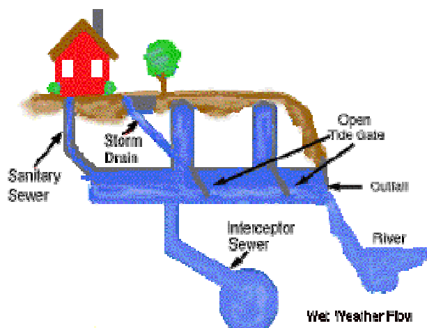
Figure 2-6. Generalized Combined Sewer System during Wet Weather (EPA 2002)
