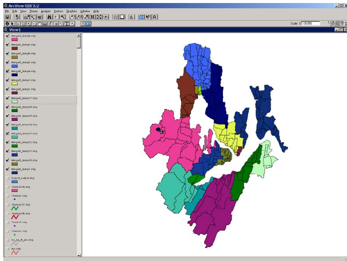
Figure 8-63. Representation of the HSPF model developed for the watershed, showing subbasin delineations.
