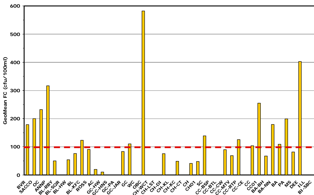
Figure 6-14. Geometric Mean (Part I WQS shown as a dashed red line) Fecal Coliform Data for Dry Seasons during the 2000-2003 Study Period for Stream Sample Sites
