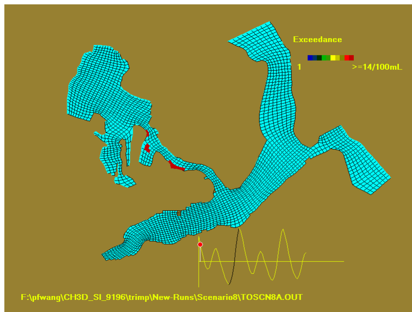
Figure 8-73. The CH3D Model Results for Sinclair-Dyes Inlet Showing the Maximum Extent of Violation of Water-Quality Standards from a Simulated Combined Sewer Overflow Event After 100% Completion of Sewer System Improvements by City of Bremerton
