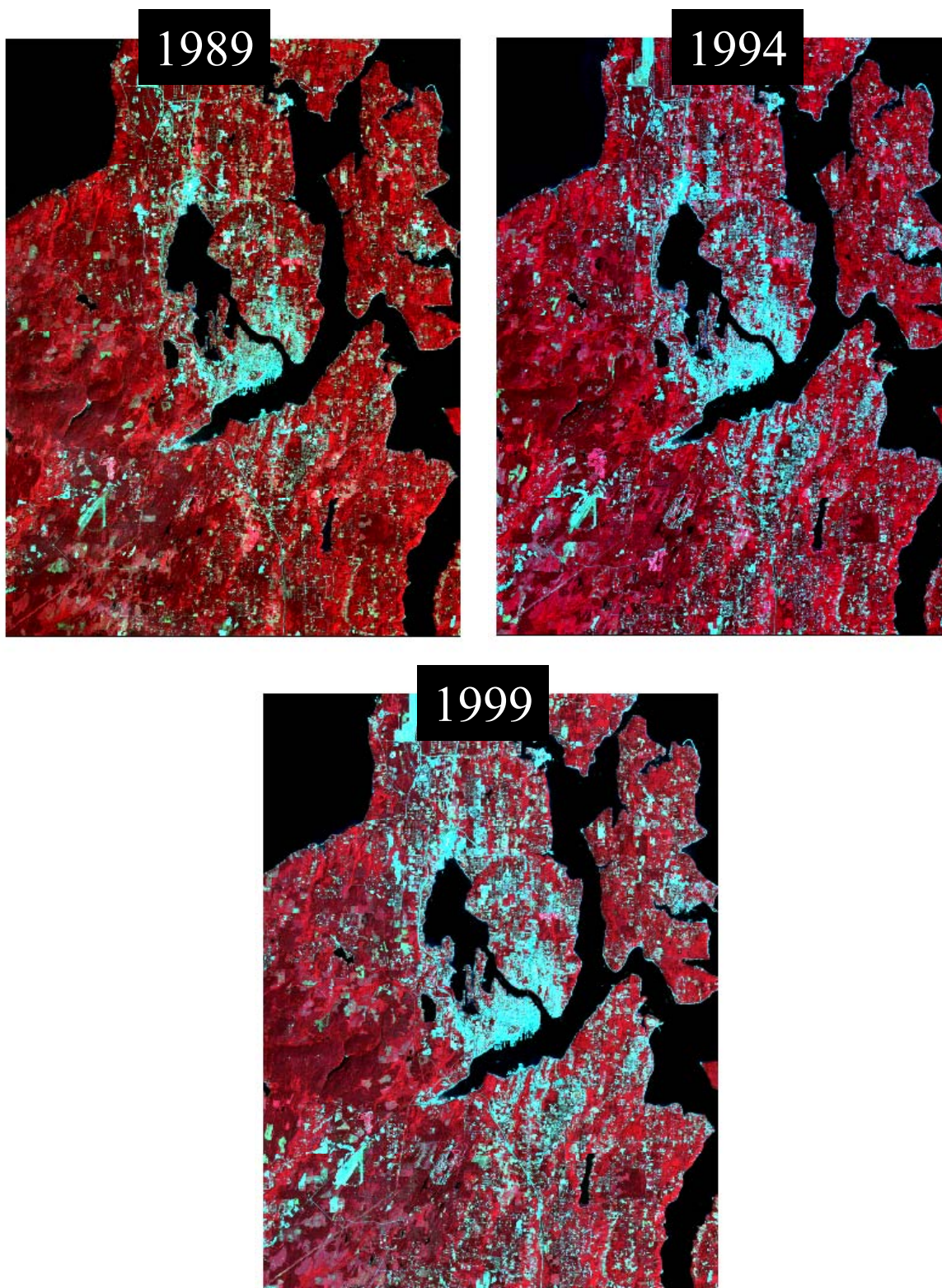
Figure 9-1. Land-Use and Land-Cover Changes Illustrated by Multi-Spectral Satellite Imagery of the Study Area from 1989 to 1999 (from Vandervoort, 2001)
