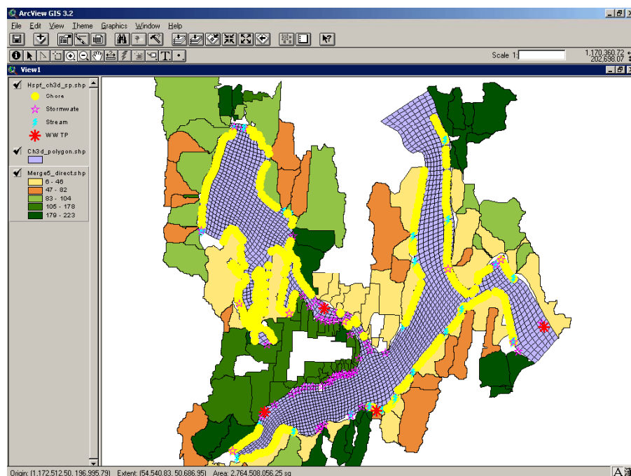
Figure 8-68. The CH3D Model Input for Sinclair-Dyes Inlet Showing Pour-Point Designations
