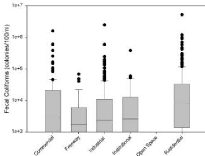
Figure 2-9. Data from the National Stormwater Quality Database for Fecal Coliform (Pitt et al., 2004)
