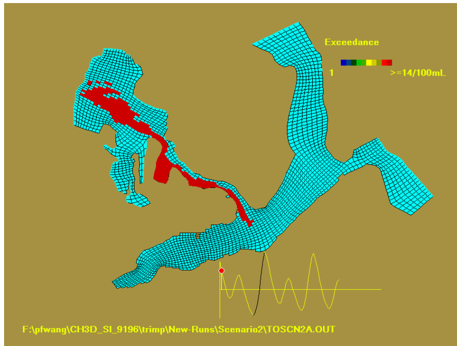
Figure 8-72. The CH3D Model Results for Sinclair-Dyes Inlet Showing the Maximum Extent of Violation of Water-Quality Standards from a Simulated Combined Sewer Overflow Event After 80% Completion of Sewer System Improvements by City of Bremerton
