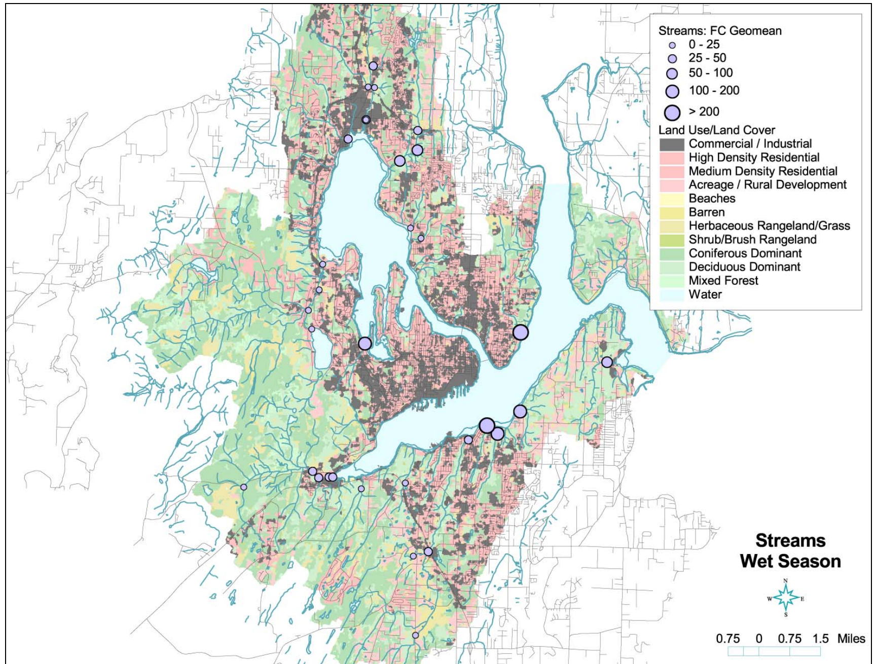
Figure 9-20. Bacterial Pollution Levels and Water-Quality Violations for Streams in the Sinclair-Dyes Inlet Watershed: Wet-Season (April-October) Fecal Coliform Sample Data Available for the 2000-2003 Study Period, Including KCHD and WA-DOH Data
