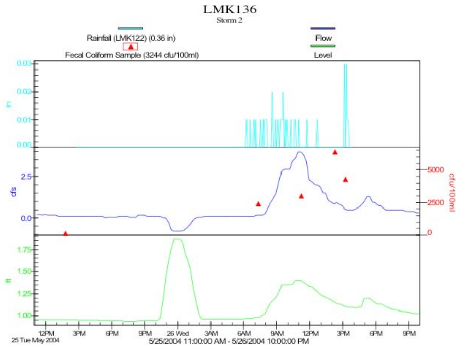
Figure 7-52. Storm-Event Response for Selected Stormwater Outfalls in the Sinclair-Dyes Inlet Watershed During the 2003-2004 Storm Season (TEC 2004)
