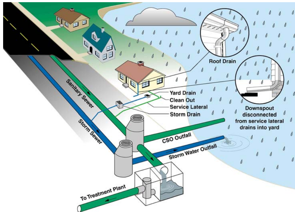
Figure 5-18. Program Goal: Route Stormwater to Ground Surface or to Stormwater Where it is Cost Effective (COB 2005)
