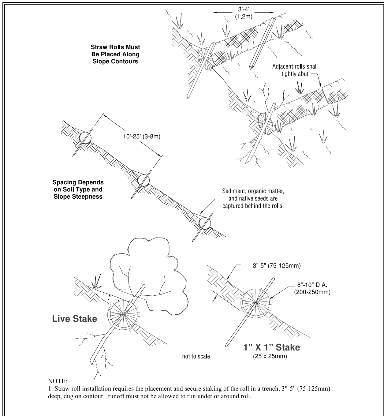
Figure 4.21 – Straw Wattles
