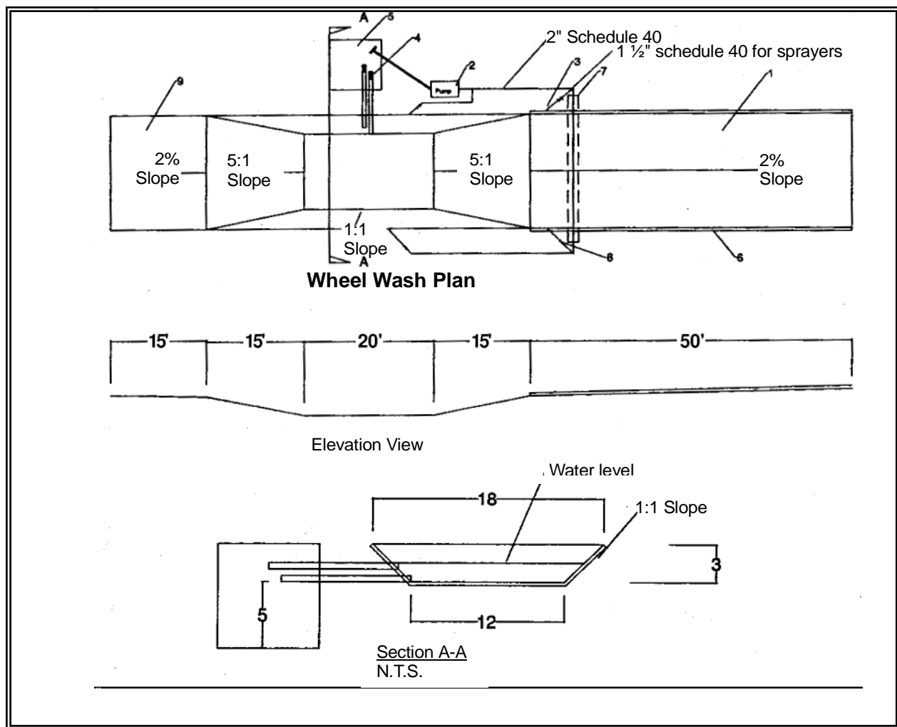
Figure 4.3 Wheel Wash
