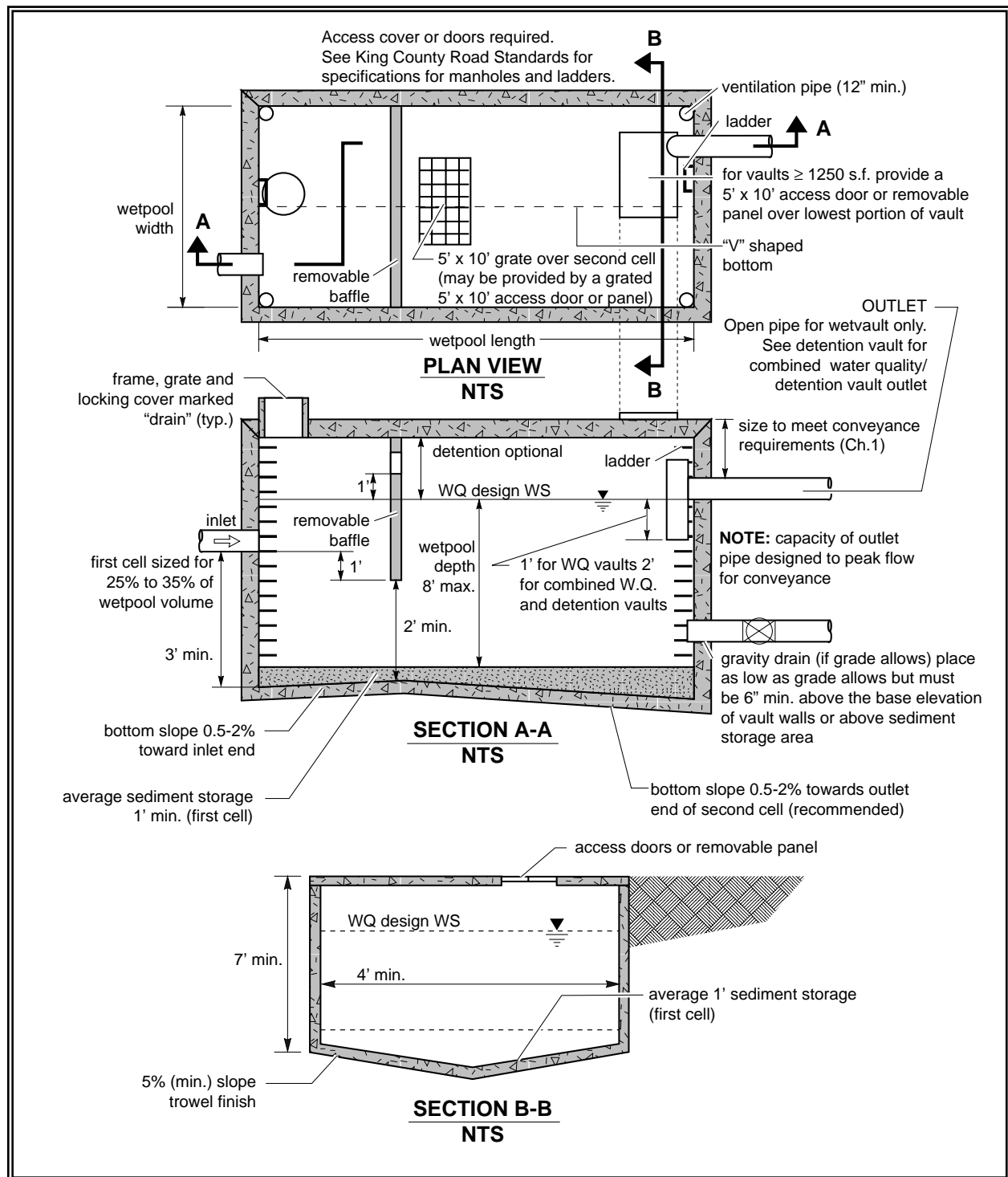
Figure 10.6 – Wetvault
