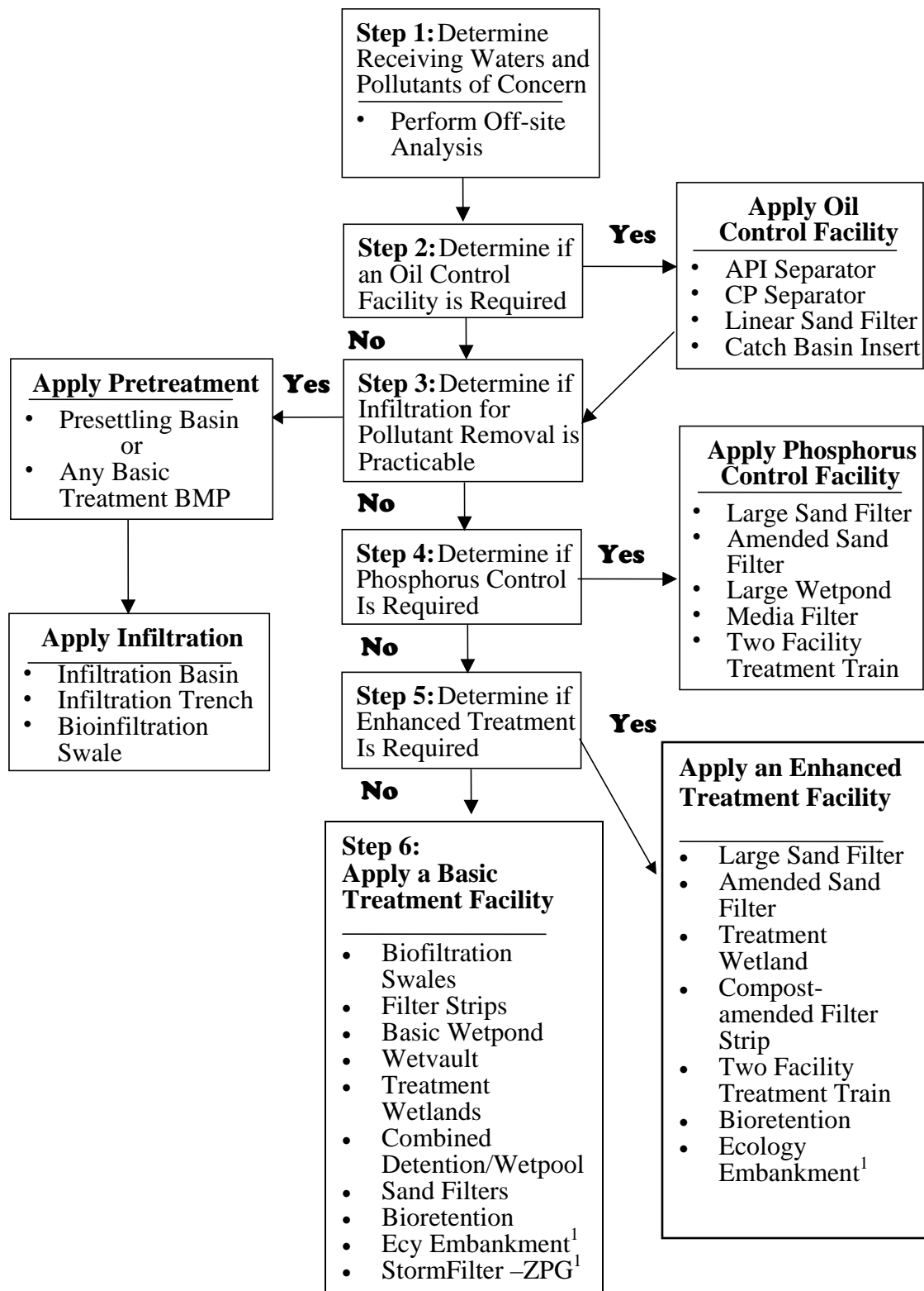
Figure 2.1 – Treatment Facility Selection Flow Chart
