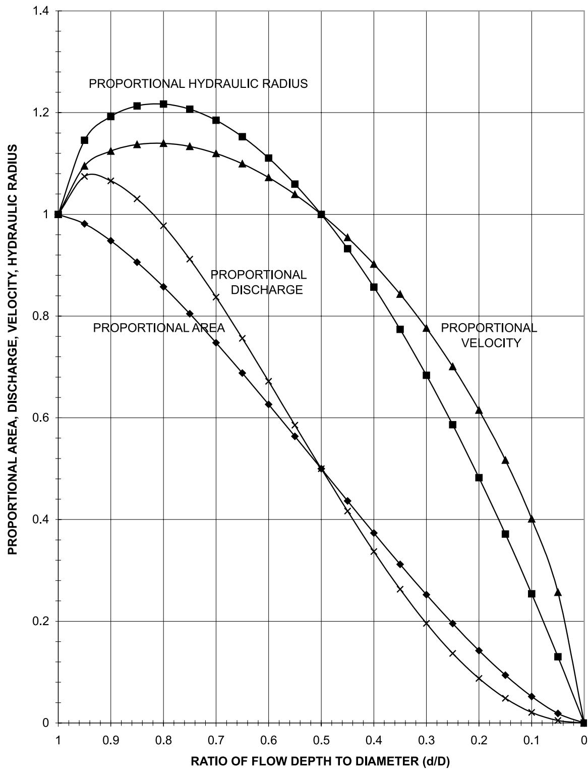
Figure 10.5 – Circular Channel Ratios
