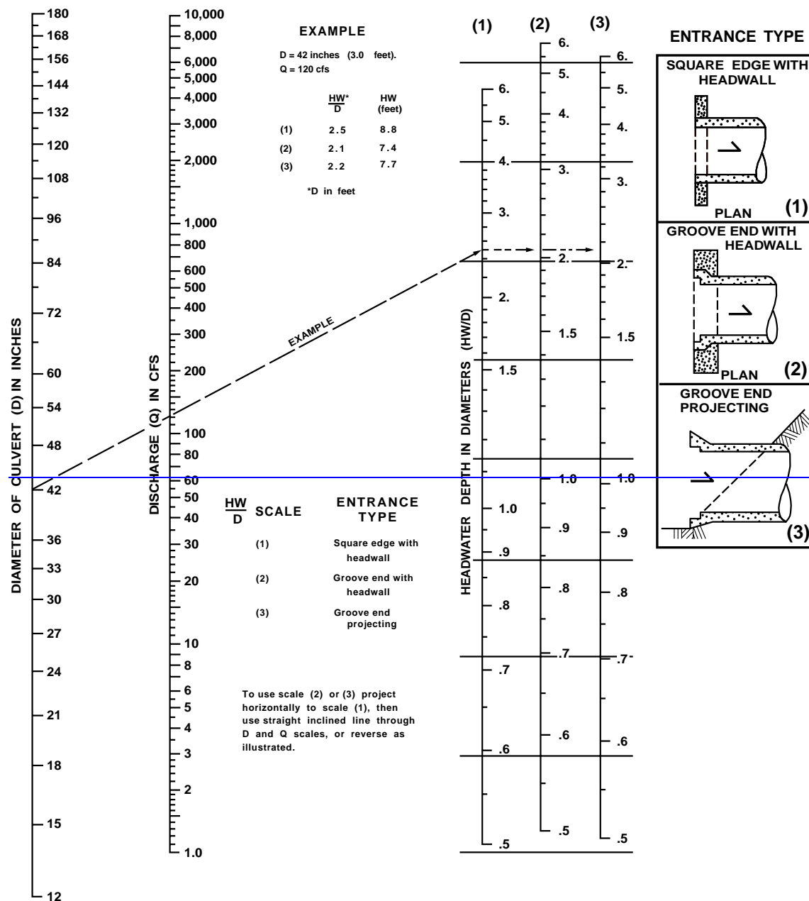
Figure 10.2 – Headwater Depth for Smooth Interior Pipe Culverts with Inlet Control
