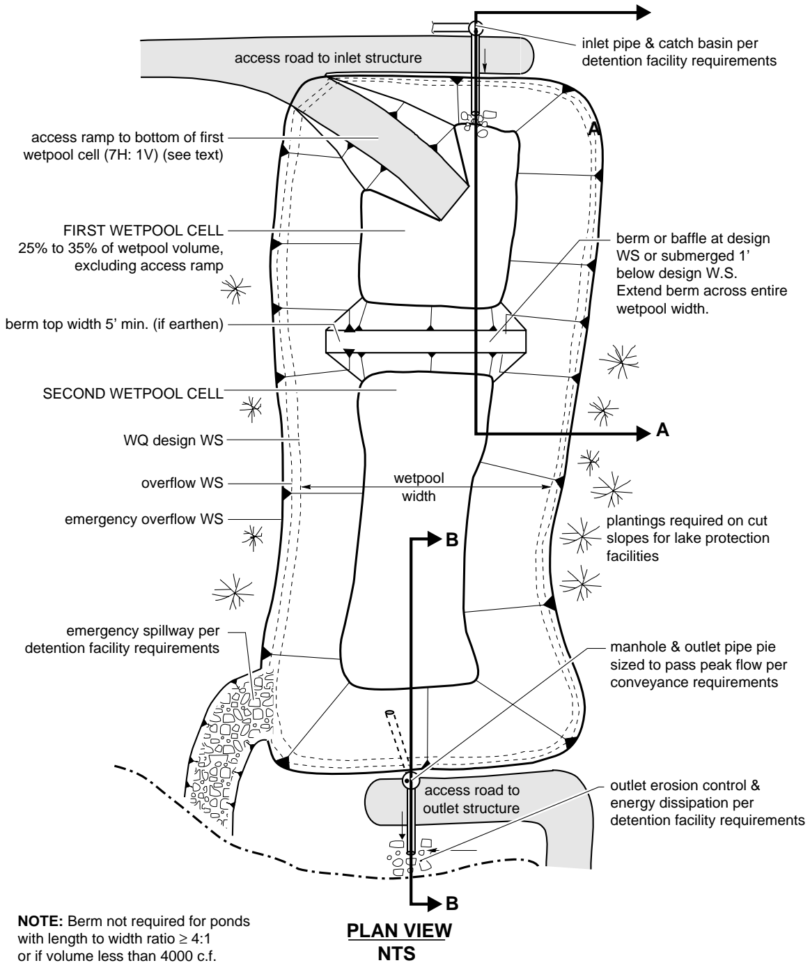
Figure 10.1a – Wetpond
