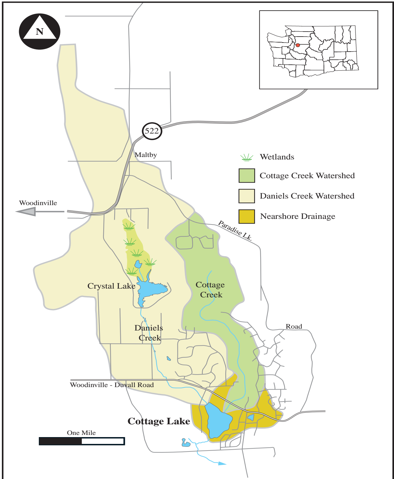
Figure 1. Cottage Lake Watershed. Cottage Lake has two main inlet tributaries, Daniels Creek and Cottage Lake Creek. The Daniels Creek drainage encompasses approximately 70 percent (3,100 acres) of the total watershed, while the Cottage Lake Creek drainage encompasses approximately 23 percent (1,000 acres) of the watershed.
