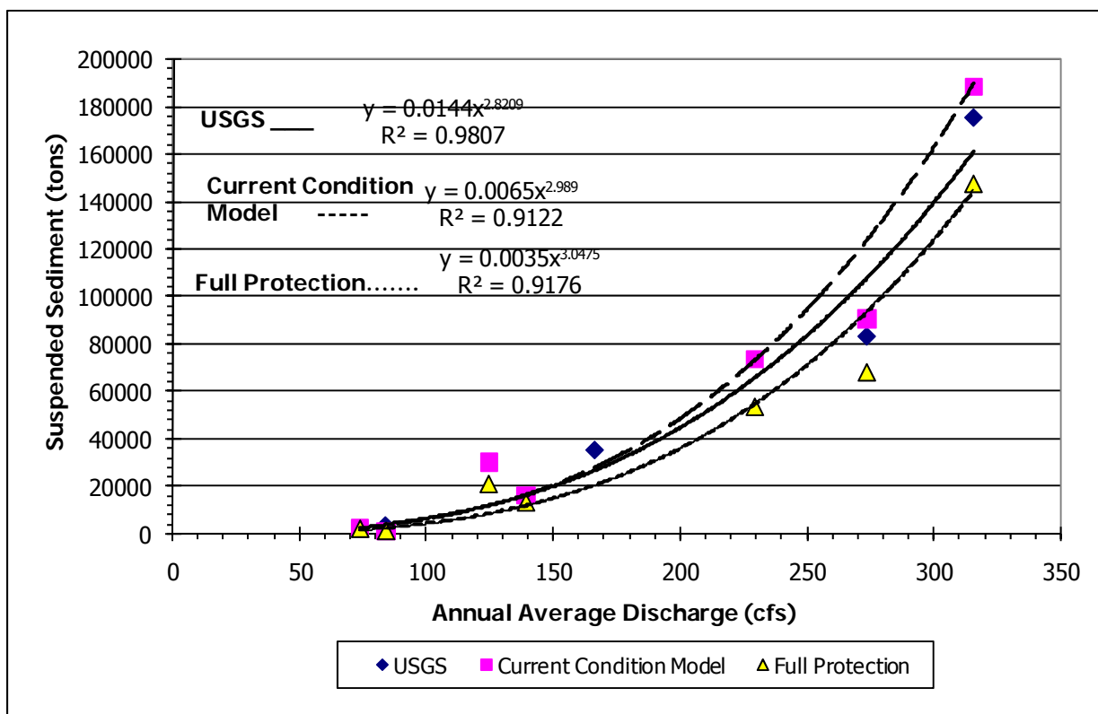
Figure 38. The estimated change in the sediment rating curve. At the mouth of Hangman Creek after estimated full protection scenario improvements are implemented in the watershed. The current condition model estimate and USGS study data (SCCD, 2002) are also shown.
