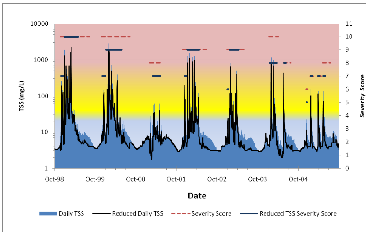
Figure 39. A comparison of estimated current and estimated full protection ( reduced ) scenario. Suspended sediment conditions for trout species at the mouth of Hangman Creek including lethal and sub-lethal severity scores calculated from the formula by Newcombe and Jensen (1996).
