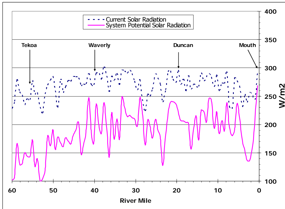
Figure 22. System-potential thermal loads along Hangman Creek. Compared to loads under current conditions based on shade and aspect inputs to the Shade model. Thermal loads are in terms of watts per square meter ( W/m^2 ).
