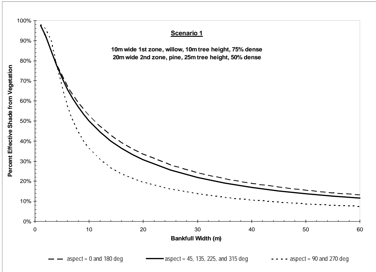
Figure 23. Shade curve constructed for sites in the Hangman Creek watershed. Based on system-potential vegetation maximum heights and stream orientation (aspect) to sunlight in August. (A stream that runs north and south has an aspect of 0 and 180 degrees).
