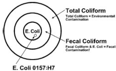
Figure 2. Relationship between total coliform, fecal coliform, and E. coli. (Washington State Department of Health, 2005).
