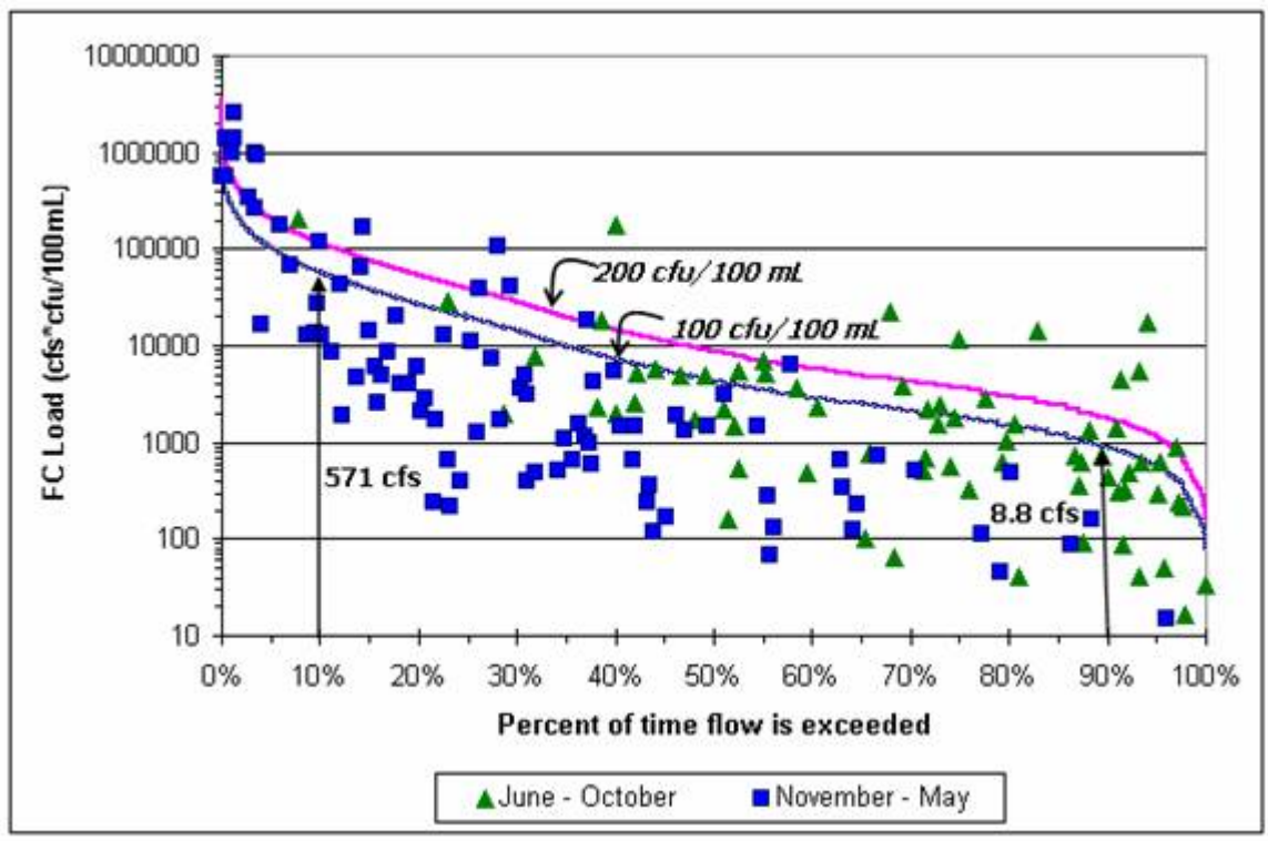
Figure 14. Seasonally-stratified fecal coliform loads. Calculated from data collected from 1989 to 2004 at the mouth of Hangman Creek (Ecology site 56A070). Loads are compared to criteria-compliant fecal coliform loads (solid lines) along a frequency curve for daily average flows from 1948 to 2004.
