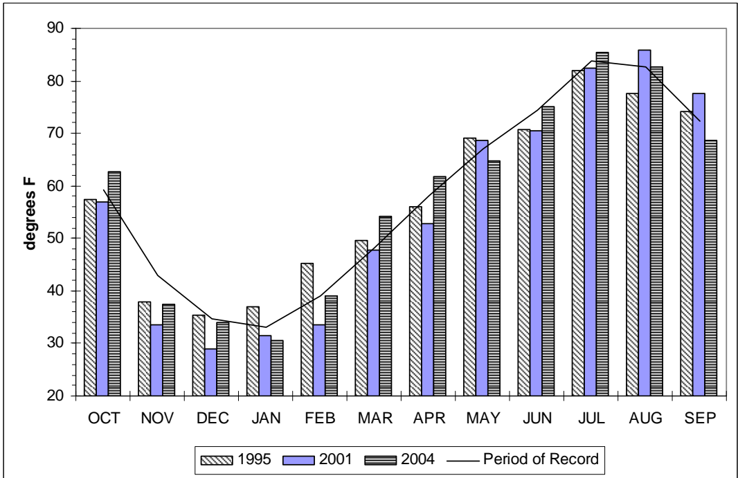
Figure 9. A comparison of long-term average monthly maximum temperatures. (Period of Record) Compared to those in water years 1995, 2001, and 2004 at the Spokane Airport (Western Regional Climate Center, 2006).
