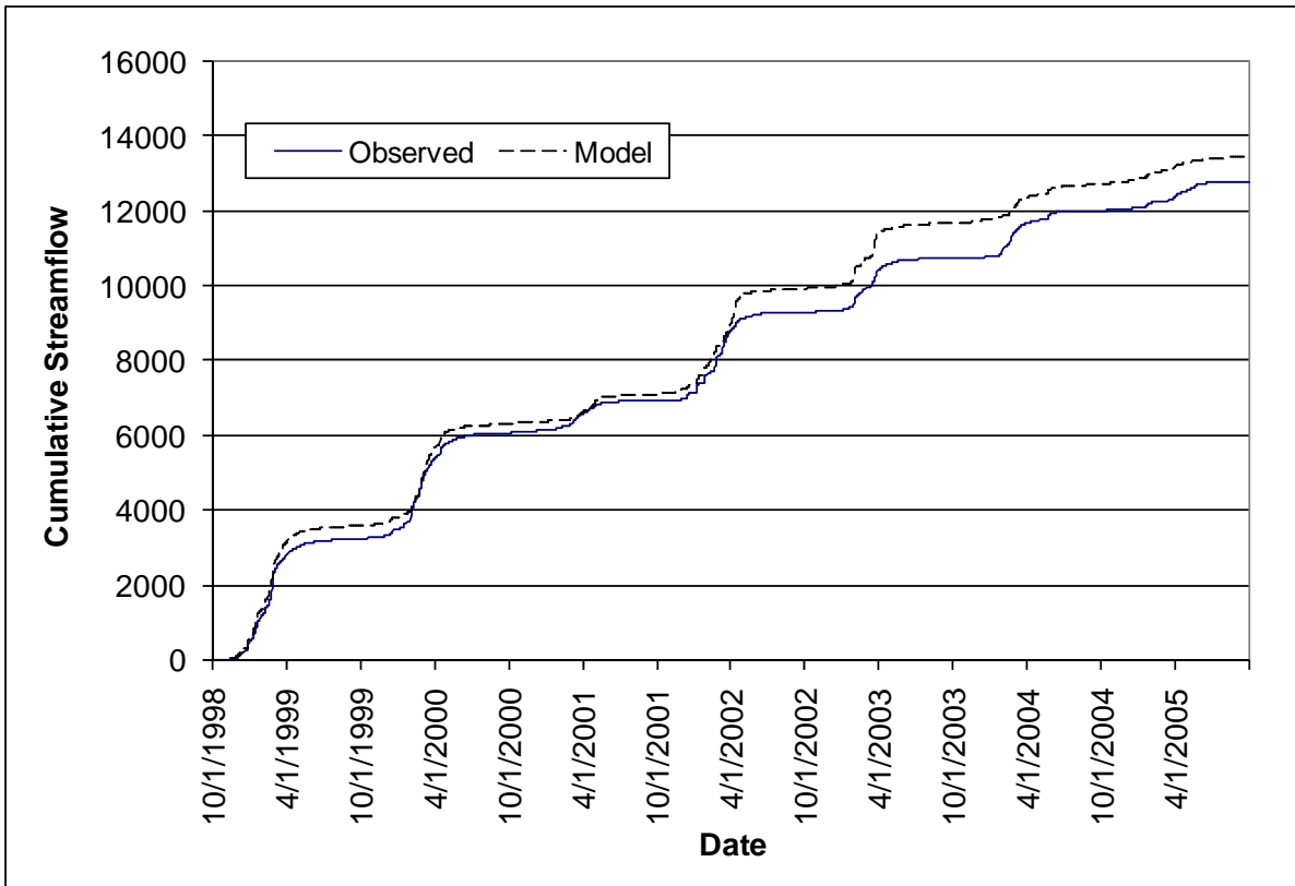
Figure 34. WARMF model of Hangman Creek (Cadmus and CDM, 2007) hydrological calibration output compared to observed streamflow data for 1998-2005: cumulative flow volume.
