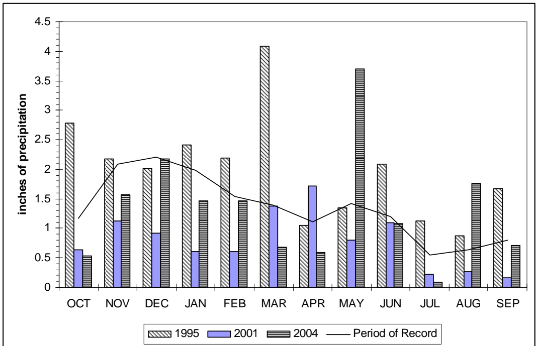
Figure 10. A comparison of long-term average monthly rainfall volumes. (Period of Record) Compare to volumes in water years 1995, 2001, and 2004 at the Spokane Airport (Western Regional Climate Center, 2006).
