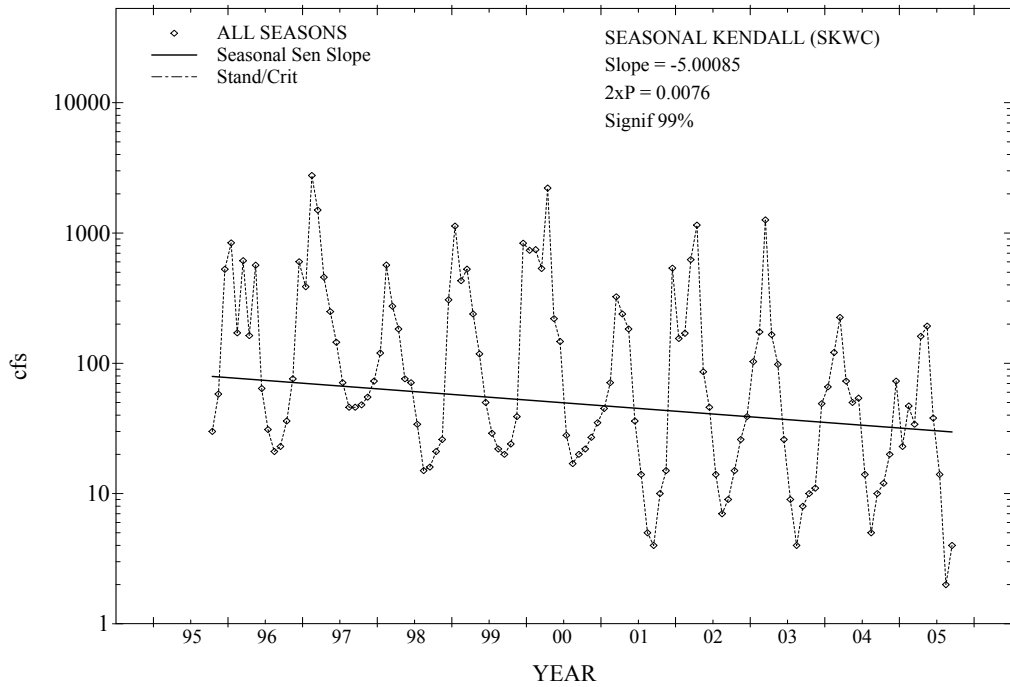
Figure 12. USGS discharge trend on Hangman Creek at mouth. (12424000), 1995–2005.
