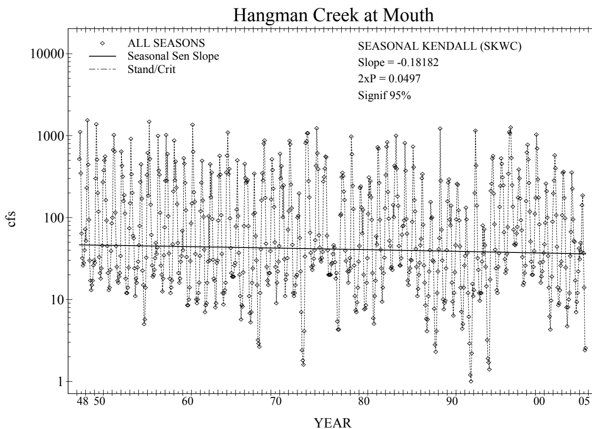
Figure 7. A Seasonal Kendall trend analysis. Monthly median flows for Hangman Creek at the USGS station (12424000).
