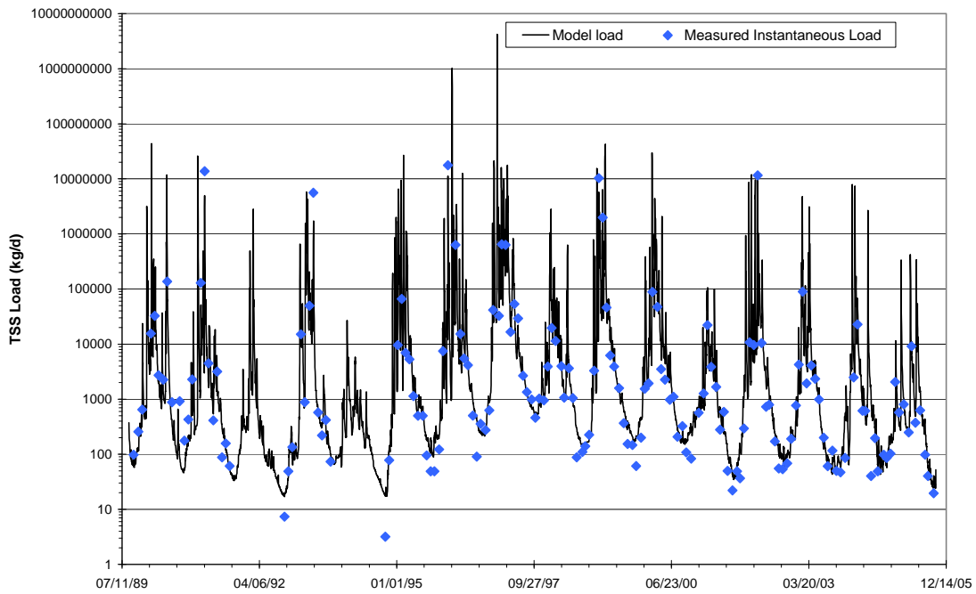
Figure 31. Total suspended solids (TSS) estimated loads. In kilograms per day (kg/d) from the multiple regression model compared to TSS estimated loads based on monthly TSS samples and instantaneous discharge measurements collected at the mouth of Hangman Creek (Ecology station 56A070).
