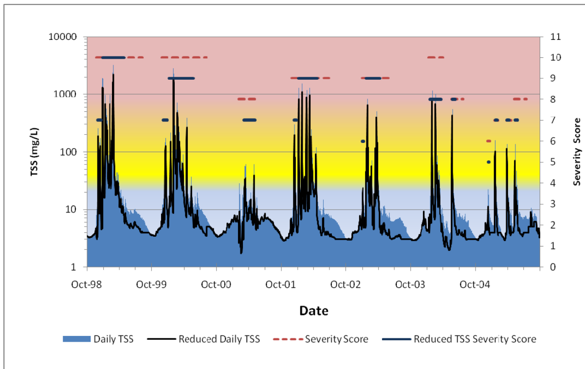
Figure ES5. A comparison of estimated current and estimated full protection. (Reduced) Scenario suspended sediment conditions for trout species at the mouth of Hangman Creek including lethal and sub-lethal severity scores calculated from the formula by Newcombe and Jensen (1996).
