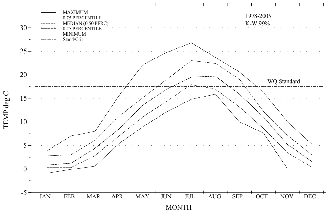
Figure 17. Monthly statistics for instantaneous temperature measurements. Taken at the mouth of Hangman Creek from 1978 to 2005 (Ecology Station 56A070).
