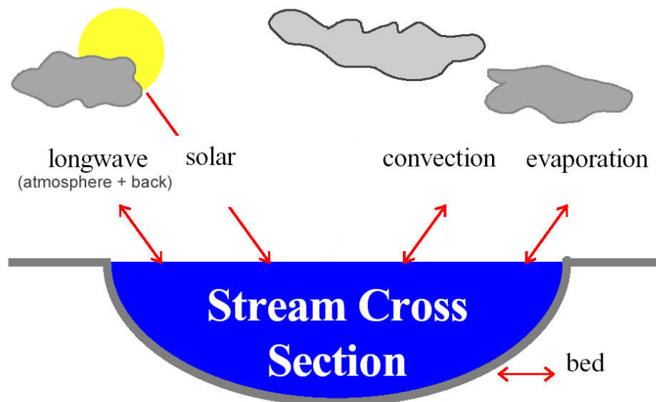
Figure B-2. Surface heat exchange processes. Those that affect water temperature net\ heat\ flux = solar + longwave\ atmosphere + longwave\ back + convection + evaporation + bed ). Heat flux between the water and streambed occurs through conduction and hyporheic exchange.
