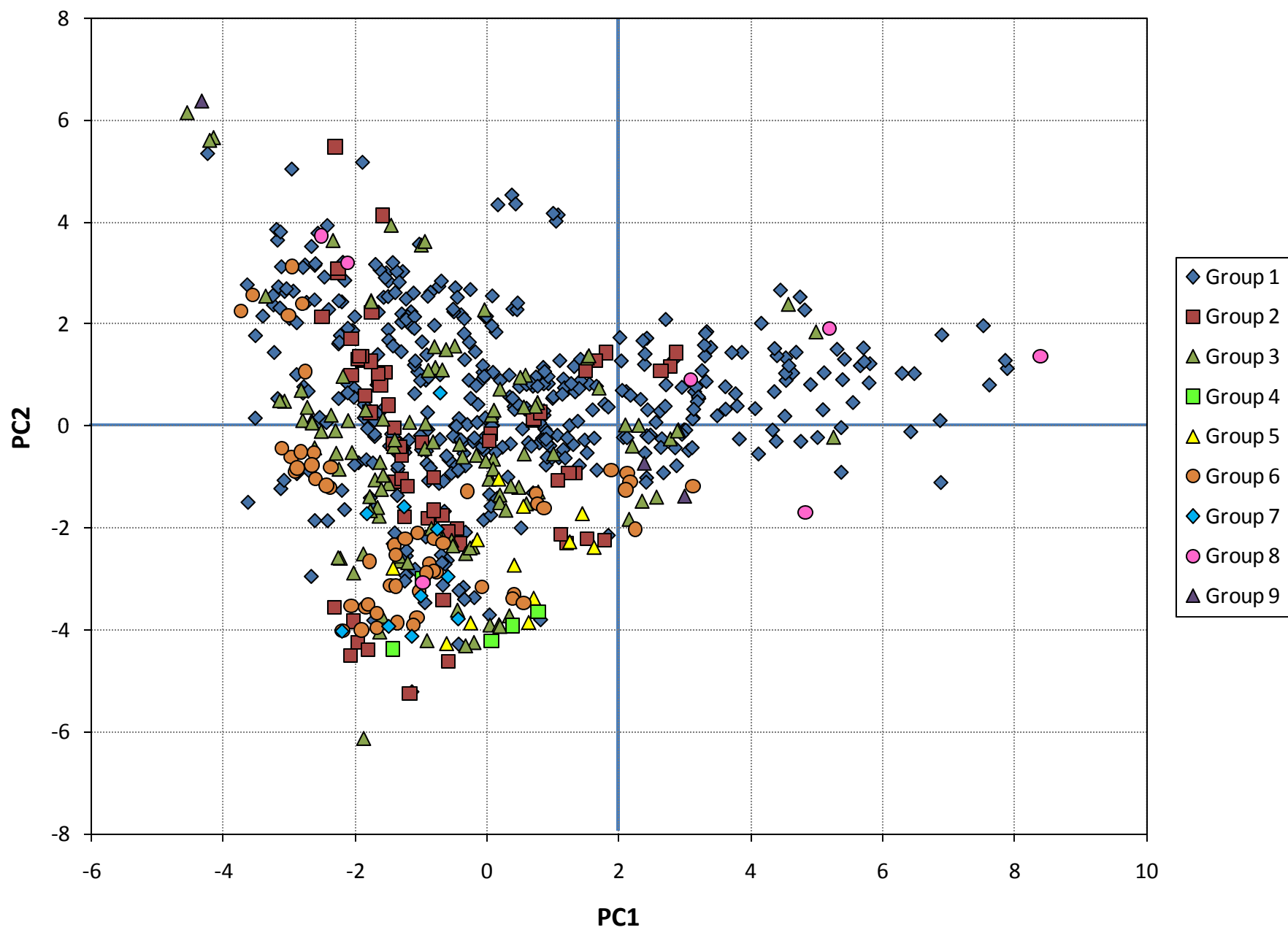
Figure 23. Biplot of PC1 against PC2 with samples coded according to HCA groupings (phenon 212).
