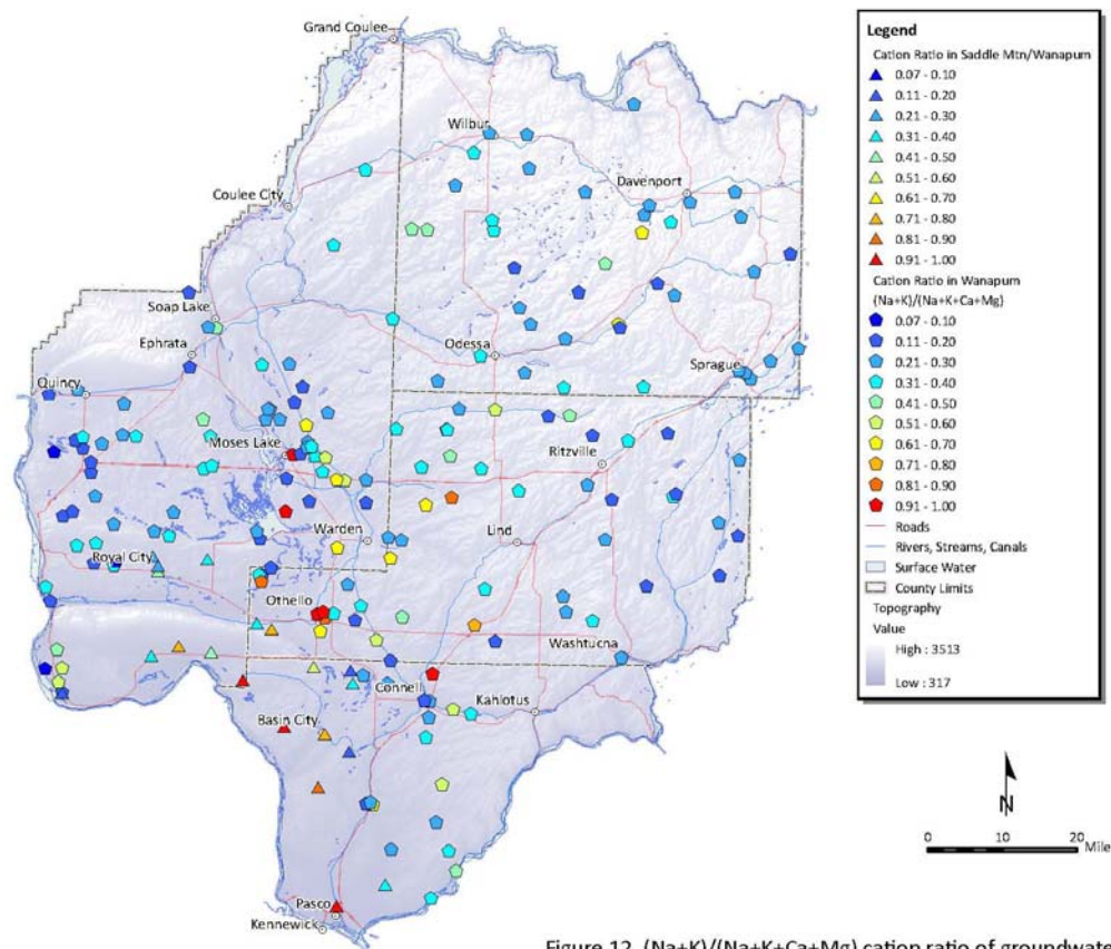
Figure 12. (Na+K)/(Na+K+Ca+Mg) cation ratio of groundwater samples from wells producing from the Wanapum Basalt.
