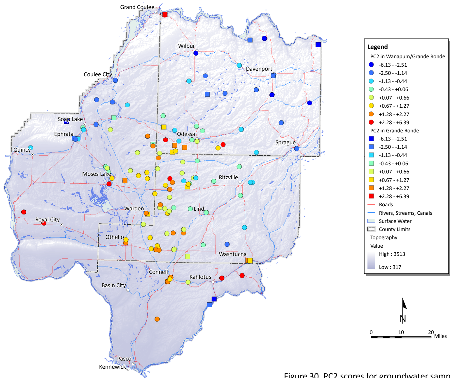
Figure 30. PC2 scores for groundwater samples from wells producing from the Grande Ronde Basalt.
