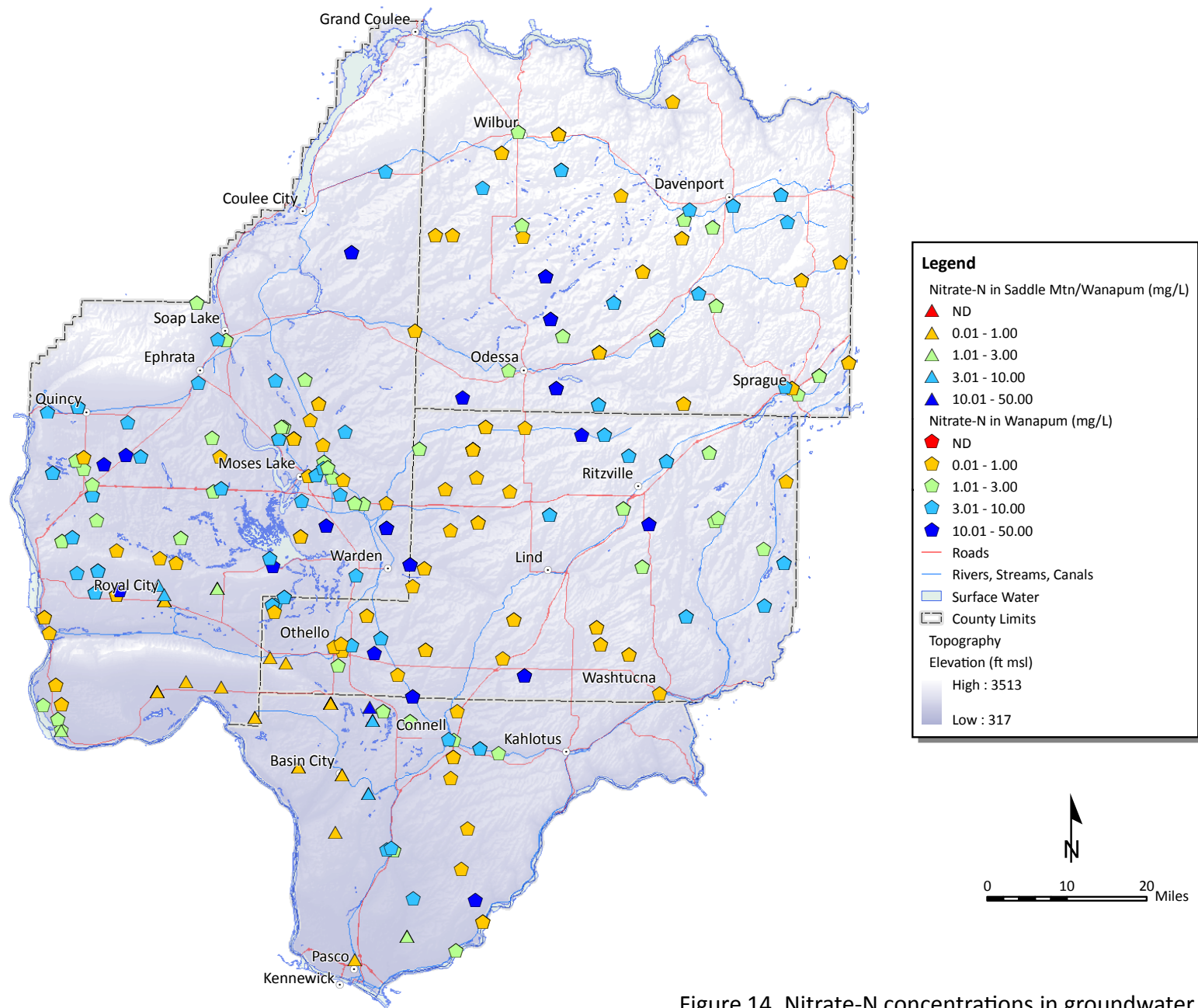
Figure 14. Nitrate-N concentrations in groundwater samples from wells producing from the Wanapum Basalt.
