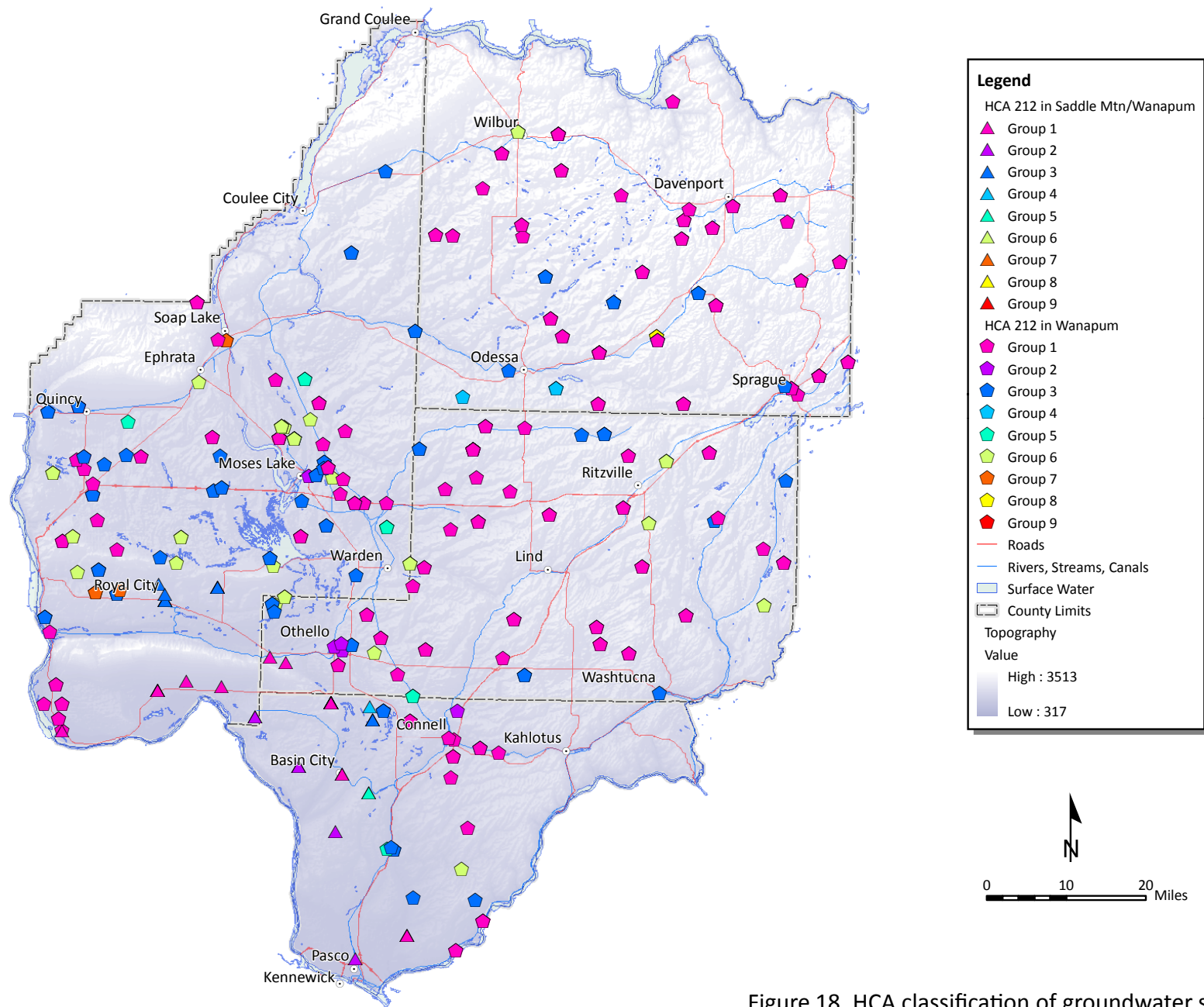
Figure 18. HCA classification of groundwater samples from wells producing from the Wanapum Basalt.
