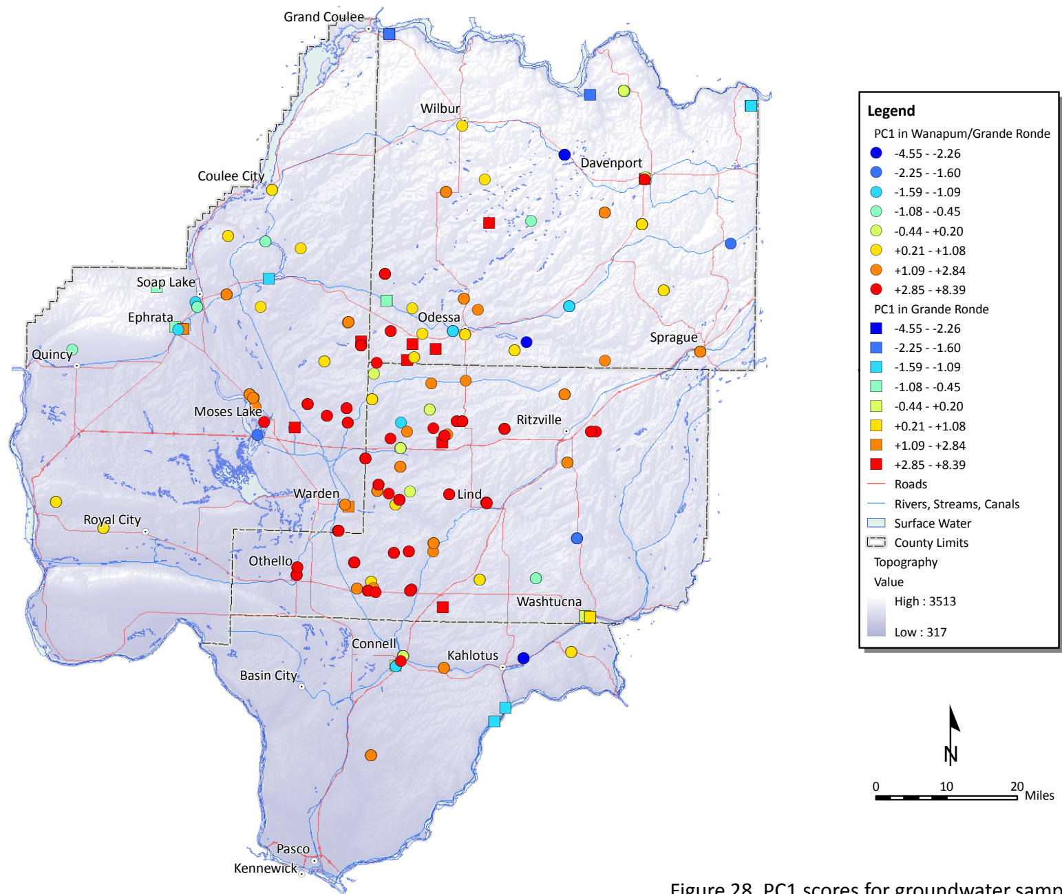
Figure 28. PC1 scores for groundwater samples from wells producing from the Grande Ronde Basalt.
