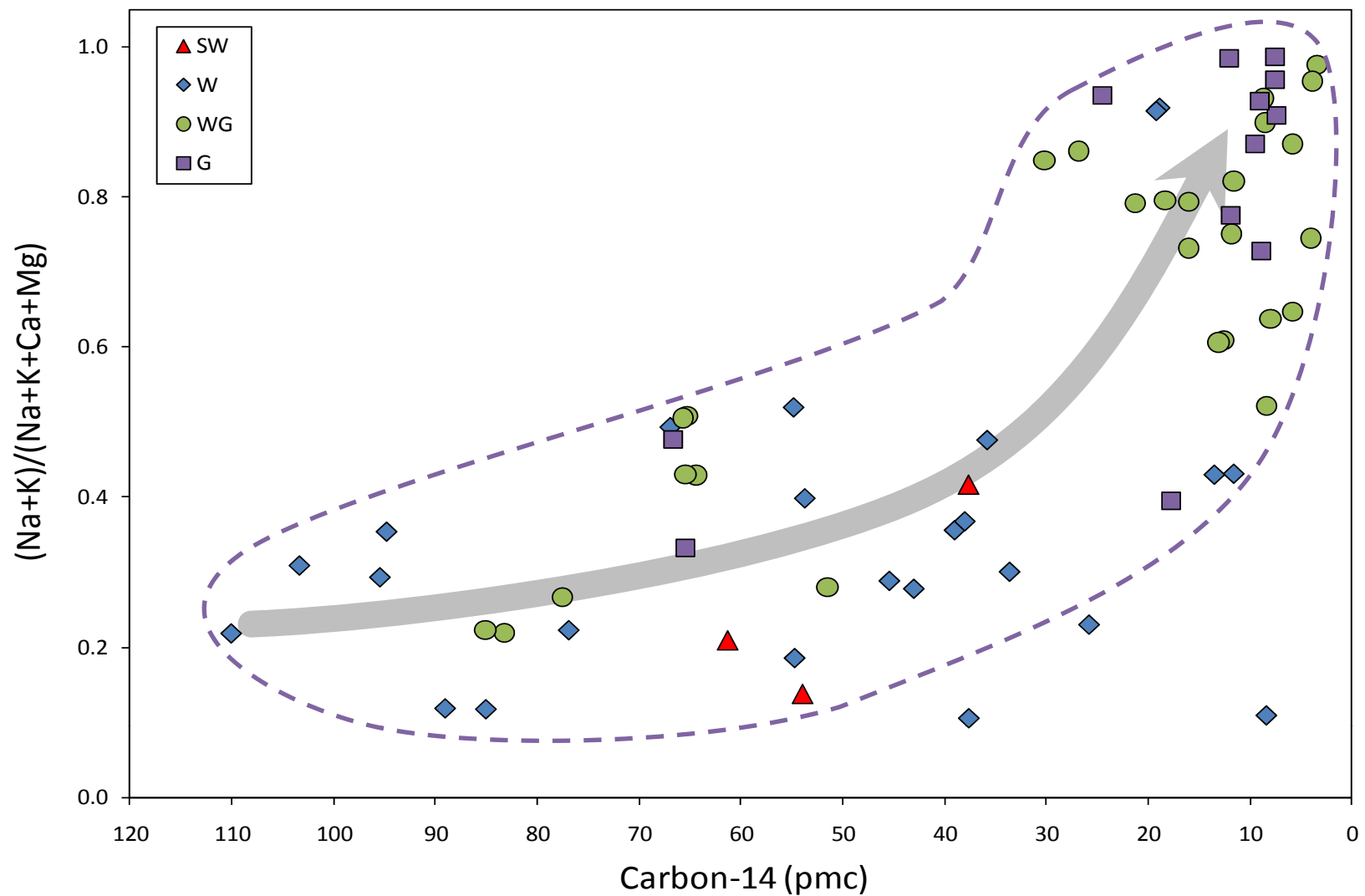
Figure 6. Variation of cation ratio (Na+K)/(Na+K+Ca+Mg) as a function of Carbon-14 activity (percent modern) of CRBG groundwater. Arrow indicates trend with increasing groundwater residence time. SW - wells producing from Saddle Mountains and Wanapum Basalts, W - wells producing from the Wanapum Basalts, WG - wells producing from the Wanapum and Grande Ronde Basalt, G - wells producing from the Grande Ronde Basalt.
