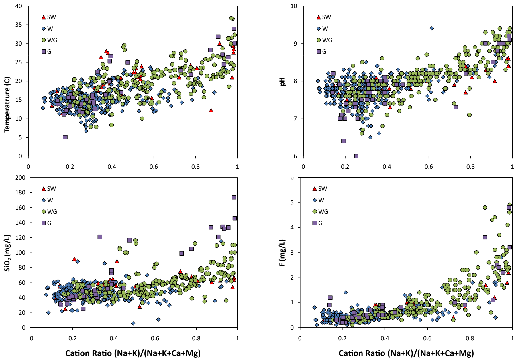
Figure 9. Variation of groundwater temperature, pH, silica and fluoride concentrations with cation ratio (Na+K)/(Na+K+Ca+Mg) . SW - wells producing from Saddle Mountains and Wanapum Basalts, W - wells producing from the Wanapum Basalt, WG - wells producing from the Wanapum and Grande Ronde Basalts, G - wells producing from the Grande Ronde Basalt.
