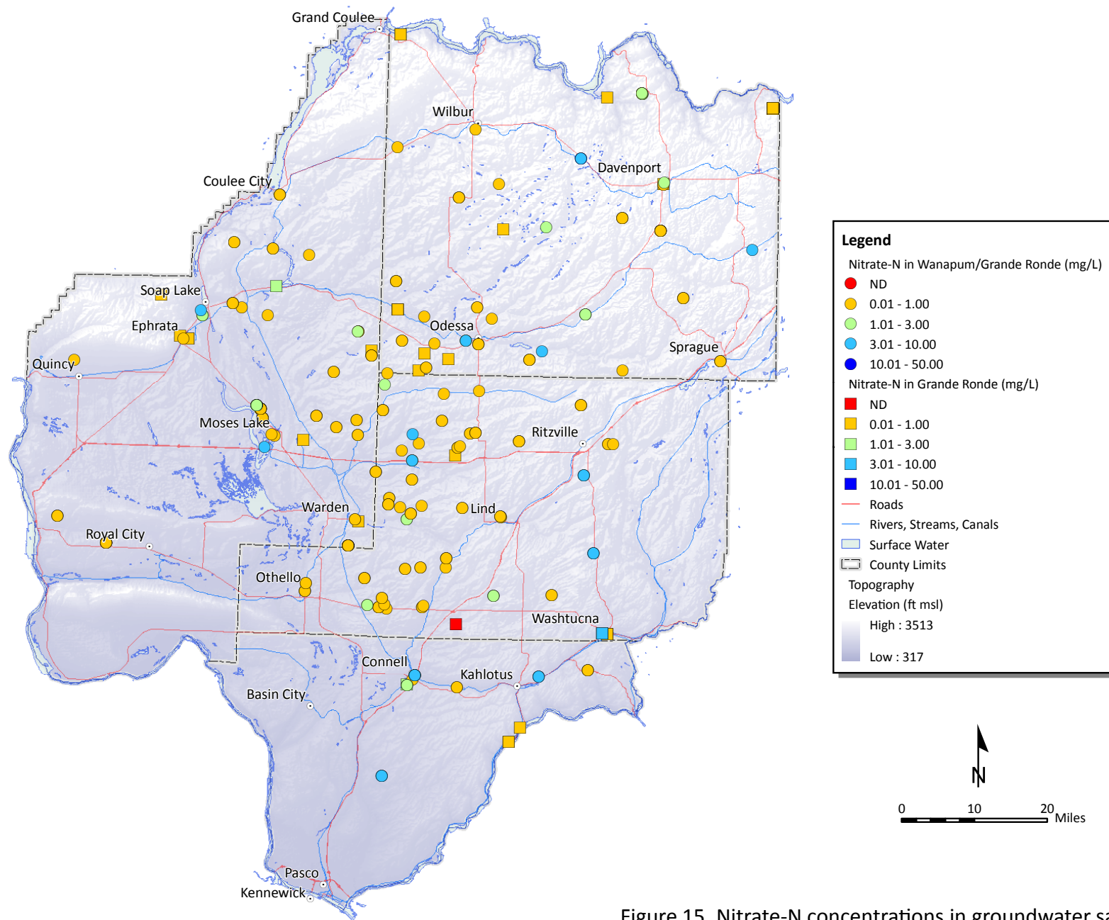
Figure 15. Nitrate-N concentrations in groundwater samples from wells producing from the Grande Ronde Basalt.
