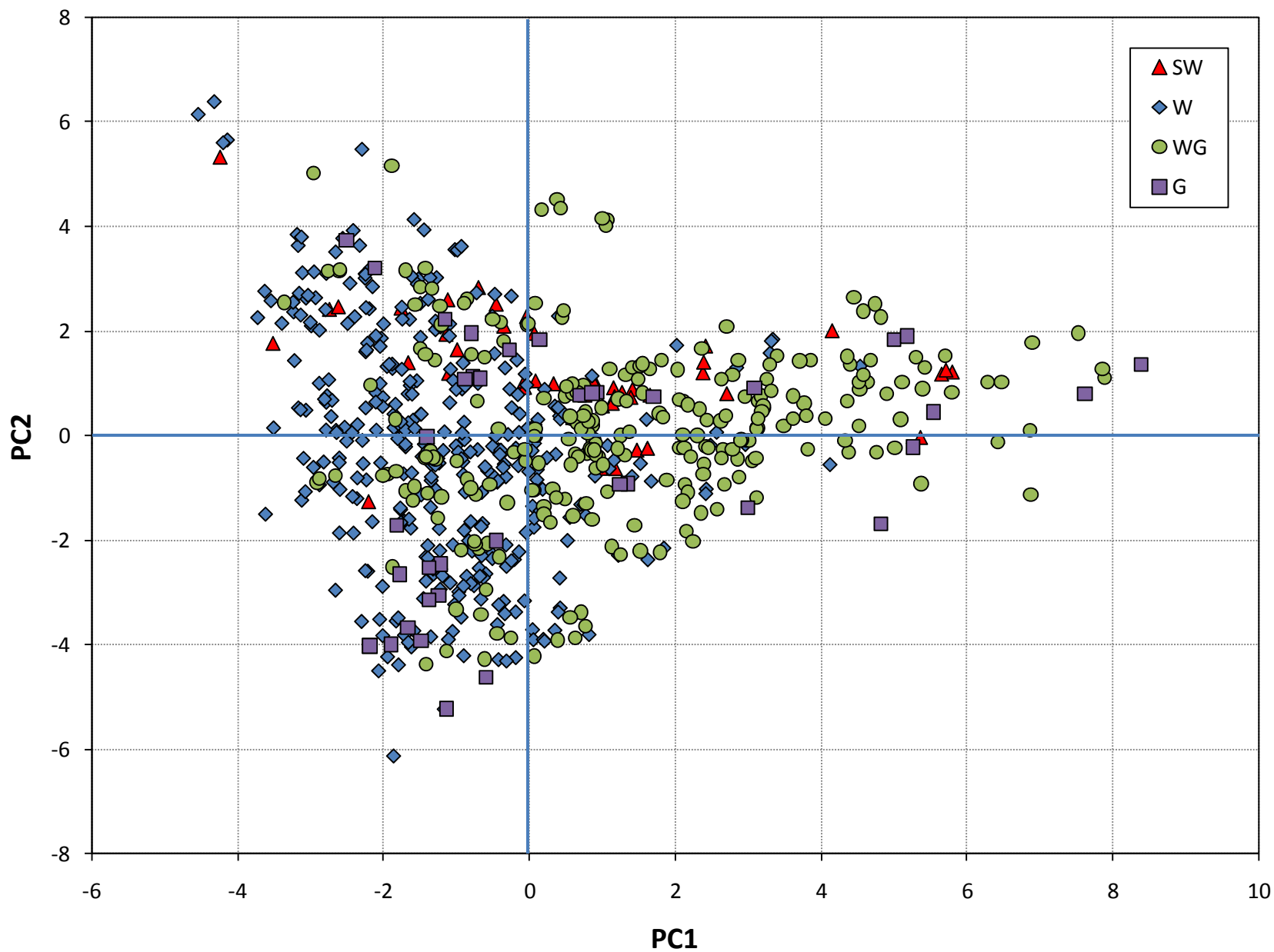
Figure 24. Biplot of PC1 against PC 2 with samples coded according to well geology. SW - wells producing from Saddle Mountains and Wanapum Basalts, W - wells producing from the Wanapum Basalt, WG - wells producing from the Wanapum and Grande Ronde Basalts, G - wells producing from the Grande Ronde Basalt.
