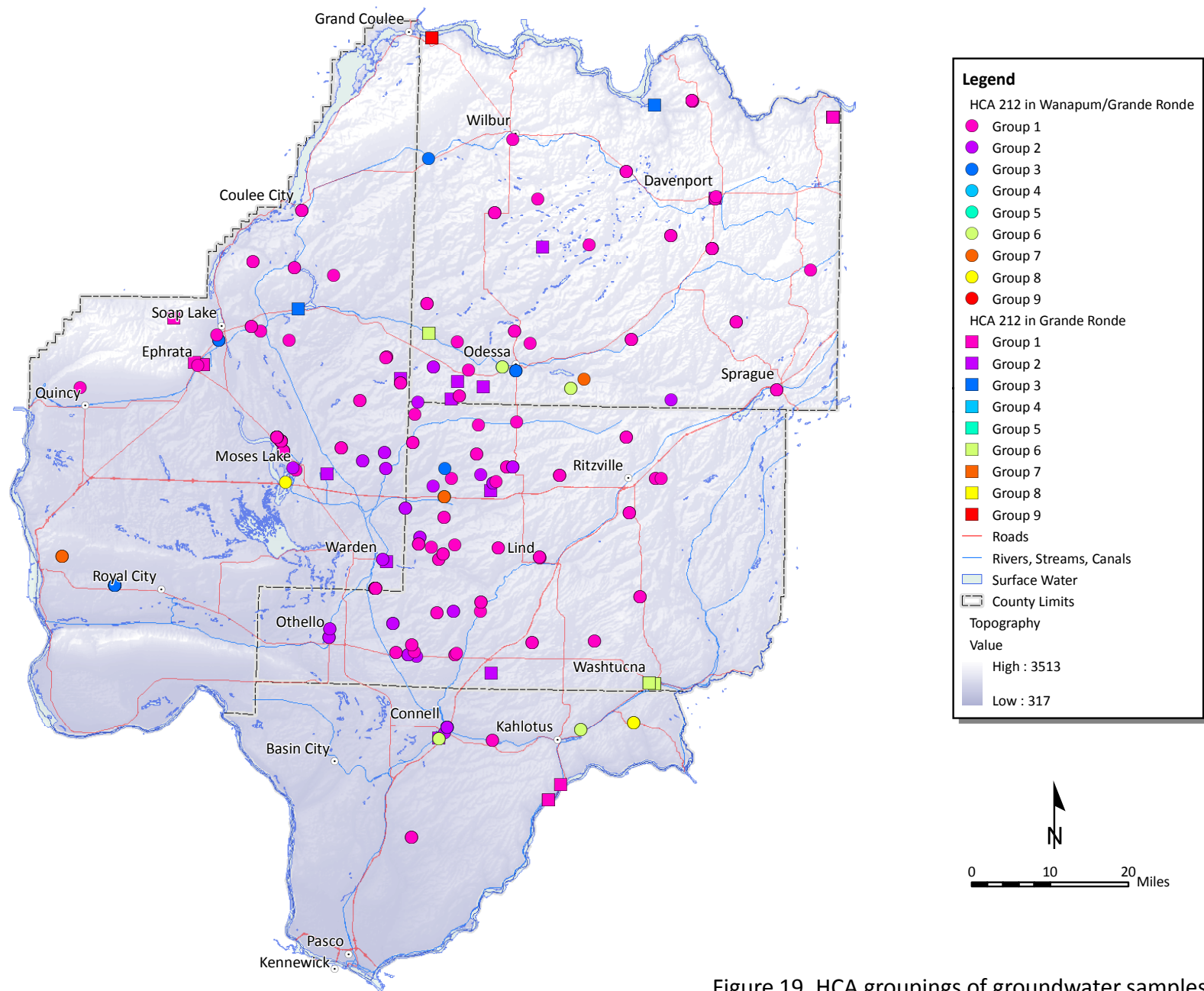
Figure 19. HCA groupings of groundwater samples from wells producing from the Grande Ronde Basalt.
