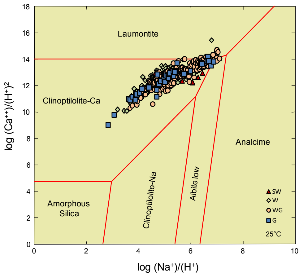
Figure 11. Activity diagrams depicting mineral stability fields relative to calculated ion activity ratios in groundwater. SW - wells producing from Saddle Mountains and Wanapum Basalts, W - wells producing from the Wanapum Basalt, WG - wells producing from the Wanapum and Grande Ronde Basalts, G - wells producing from the Grande Ronde Basalt.
