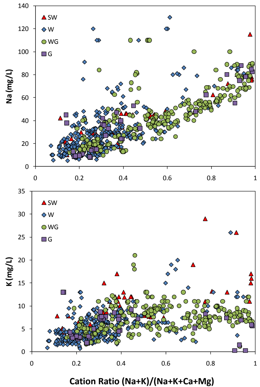
Figure 7. Variation of major cation concentrations in CRBG groundwater with cation ratio (Na+K)/(Na+K+Ca+Mg) . SW - wells producing from the Saddle Mountains and Wanapum Basalts, W - wells producing from the Wanapum Basalt, WG - wells producing from the Wanapum and Grande Ronde Basalts, G - wells producing from the Grande Ronde Basalt.
