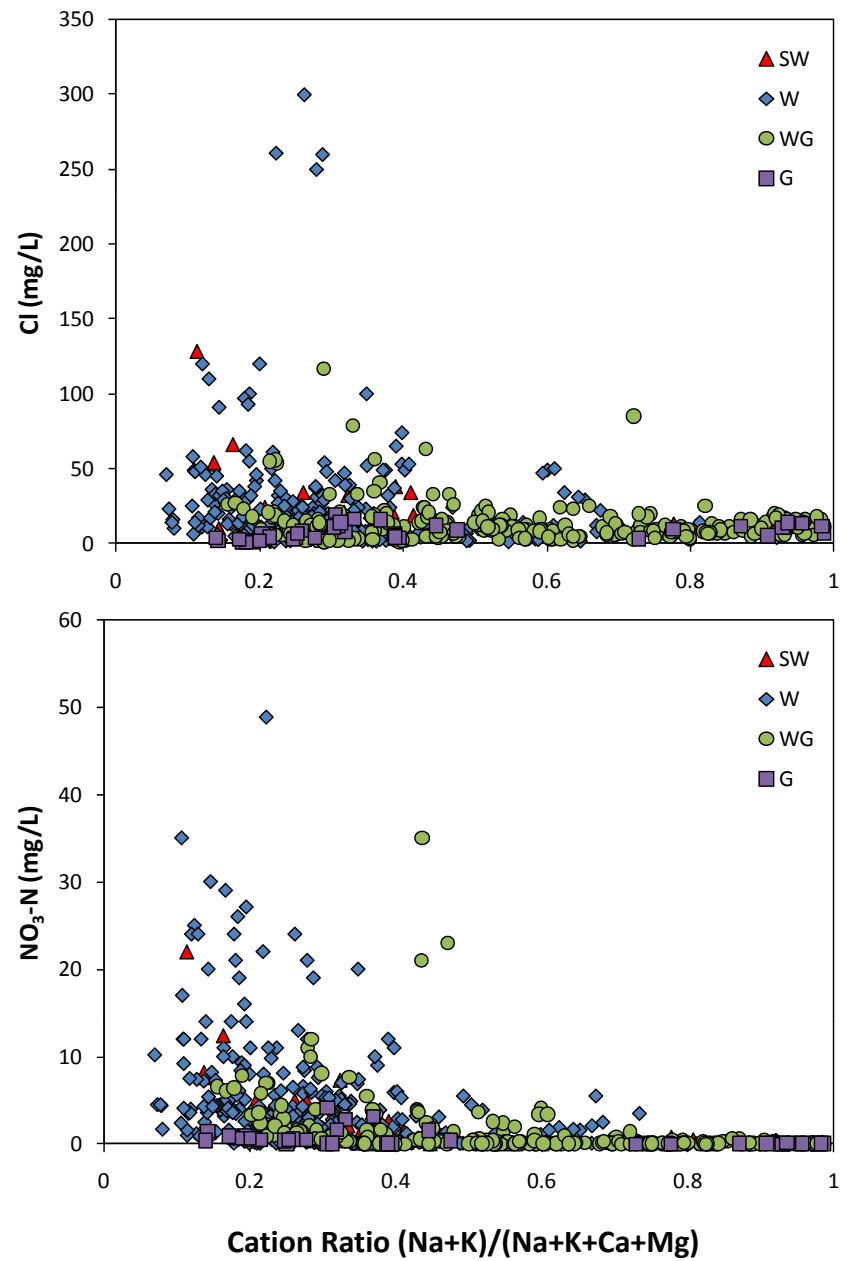
Figure 8. Variation of major anion concentrations in CRBG groundwater with cation ratio (\text{Na}+\text{K})/(\text{Na}+\text{K}+\text{Ca}+\text{Mg}) . SW - wells producing from Saddle Mountains and Wanapum Basalts, W - wells producing from the Wanapum Basalt, WG - wells producing from the Wanapum and Grande Ronde Basalts, G - wells producing from the Grande Ronde Basalt.
