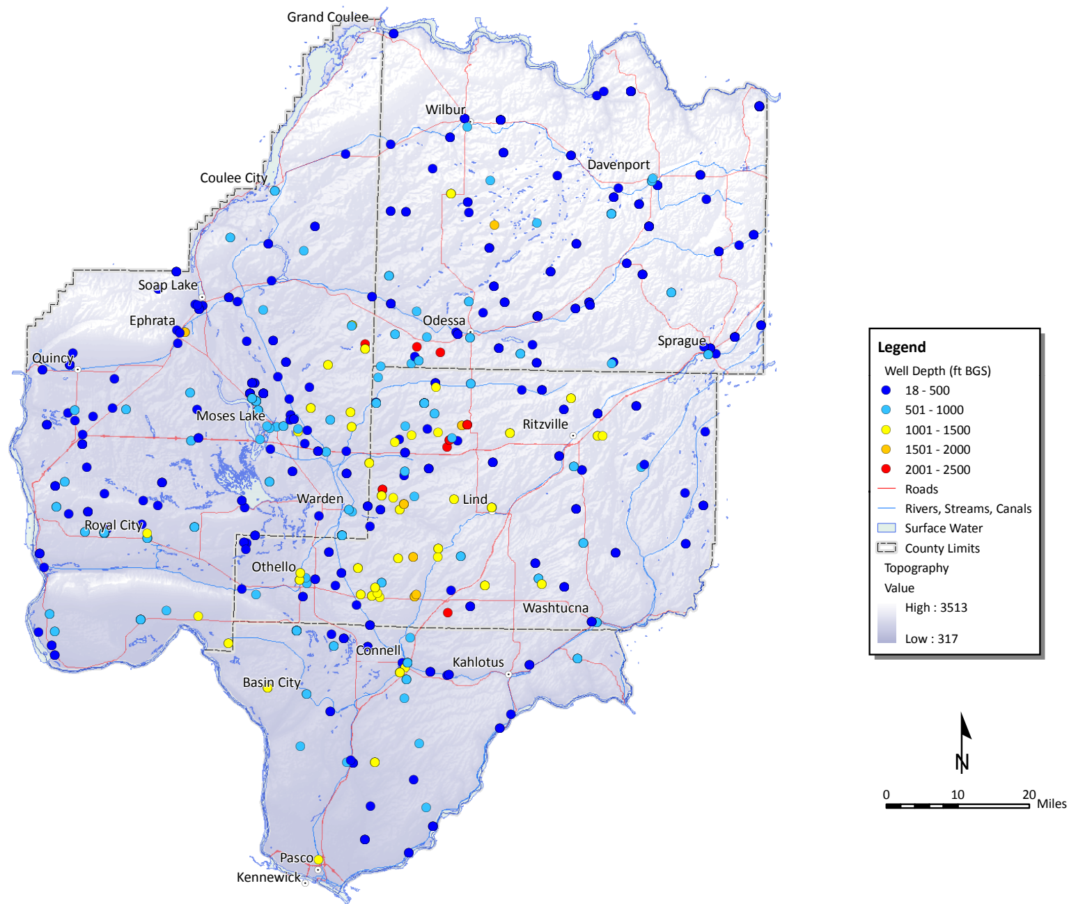
Figure 3. Well locations and total depth
