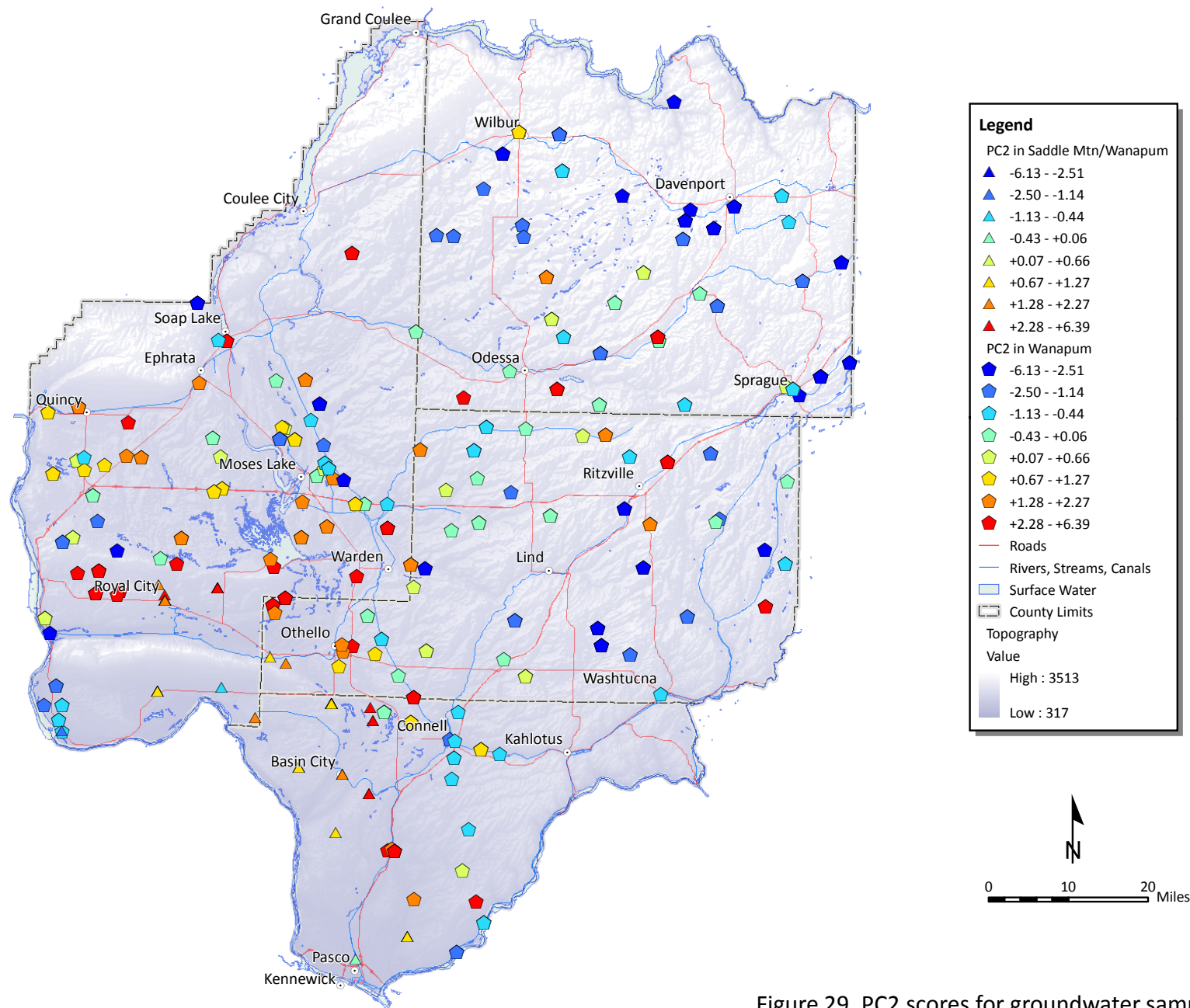
Figure 29. PC2 scores for groundwater samples from wells producing from the Wanapum Basalt.
