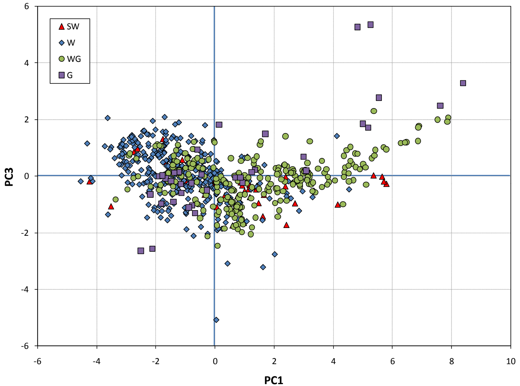
Figure 26. Biplot of PC1 against PC3 with samples coded according to well geology. SW - wells producing from Saddle Mountains and Wanapum Basalts, W - wells producing from the Wanapum Basalt, WG - wells producing from the Wanapum and Grande Ronde Basalts, G - wells producing from the Grande Ronde Basalt.
