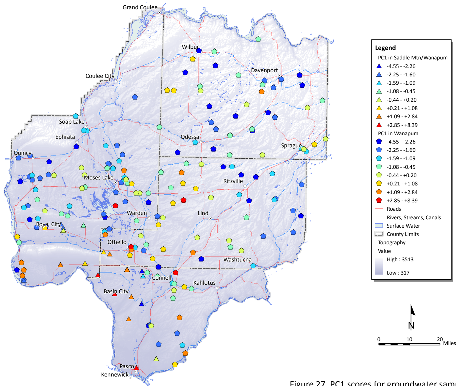
Figure 27. PC1 scores for groundwater samples from wells producing from the Wanapum Basalt.
