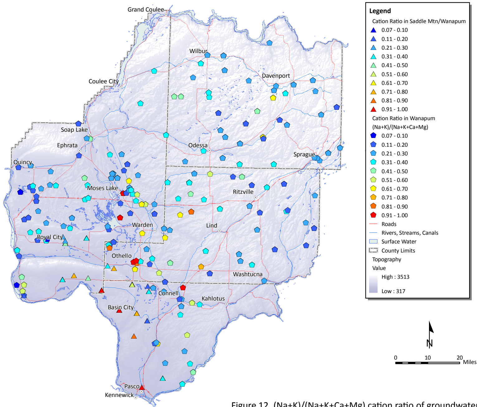
Figure 12. (\text{Na}+\text{K})/(\text{Na}+\text{K}+\text{Ca}+\text{Mg}) cation ratio of groundwater samples from wells producing from the Wanapum Basalt.
