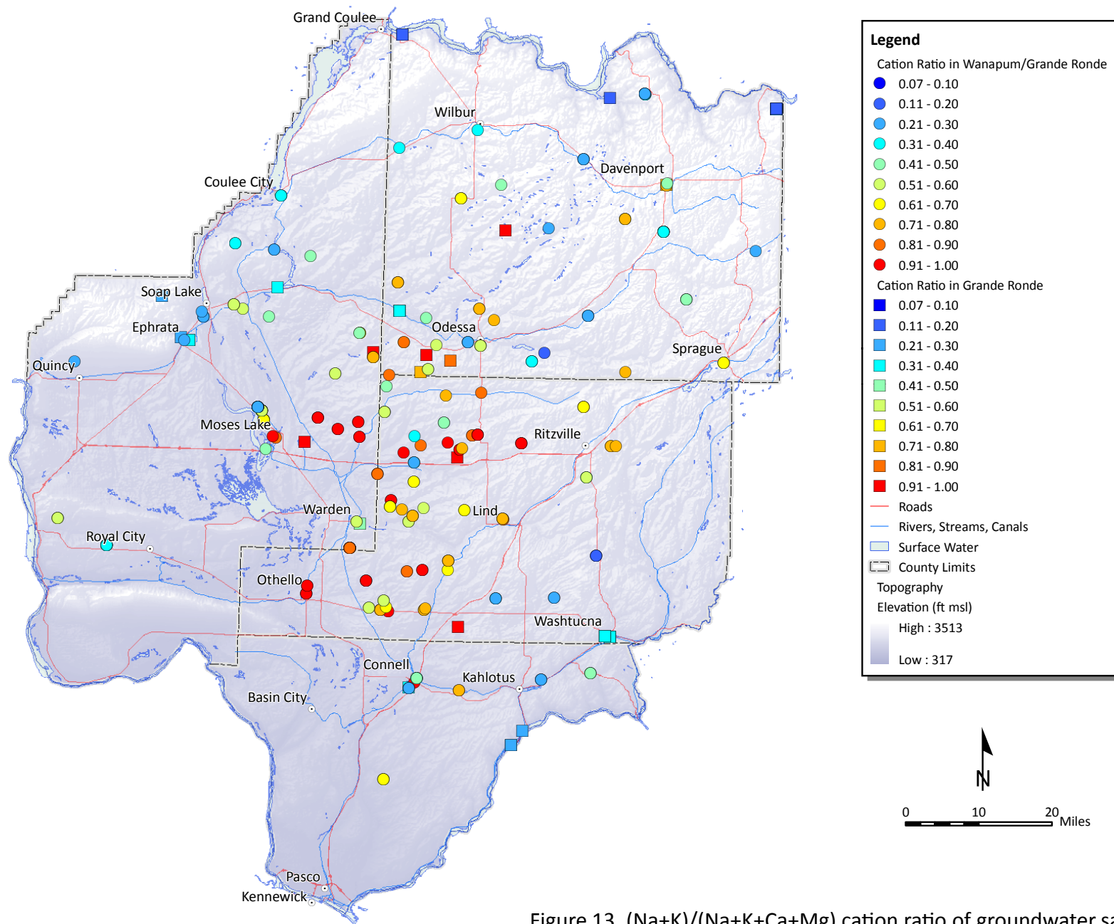
Figure 13. (\text{Na}+\text{K})/(\text{Na}+\text{K}+\text{Ca}+\text{Mg}) cation ratio of groundwater samples from wells producing from the Grande Ronde Basalt.
