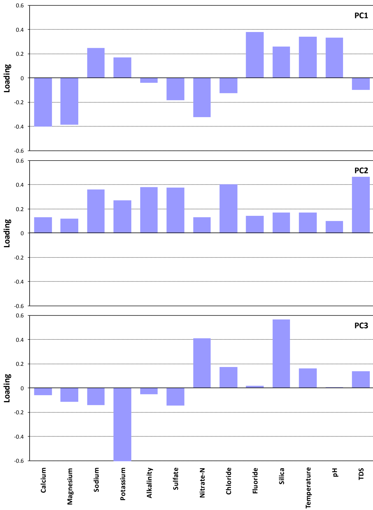
Figure 21. Variable loadings on the first three principal components.
