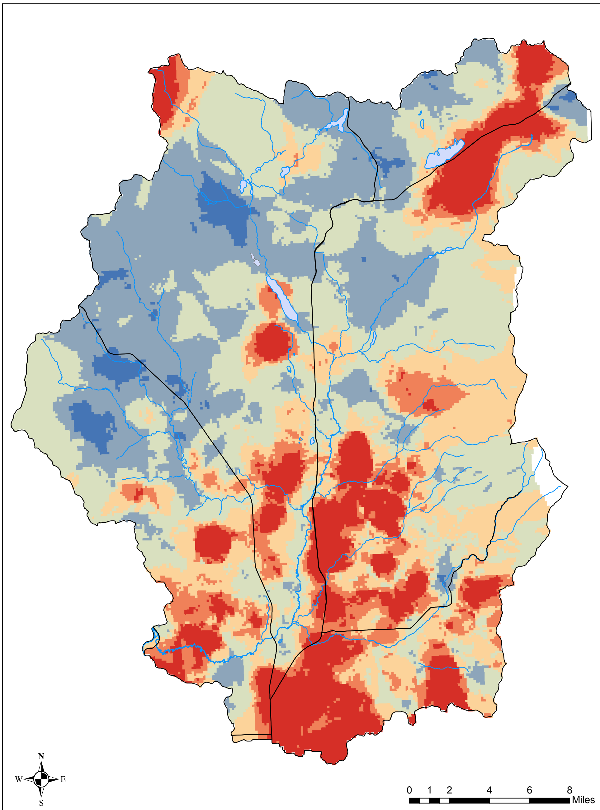
Figure 2-5 WRIA 55 Water Well Static Water Level Spatial Variation
