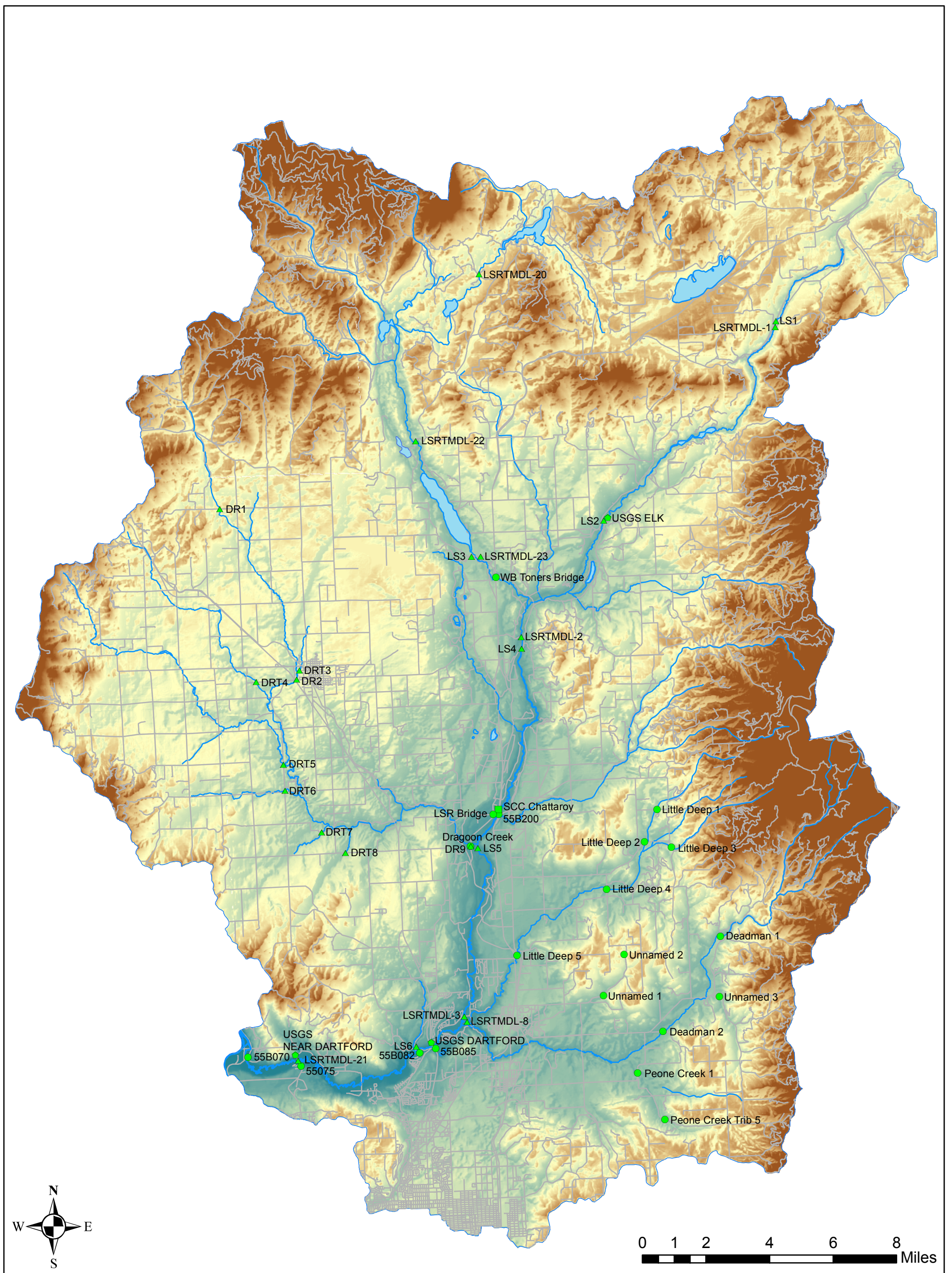
Figure 5-1 WRIA 55 Stream Flow Measurement Locations
