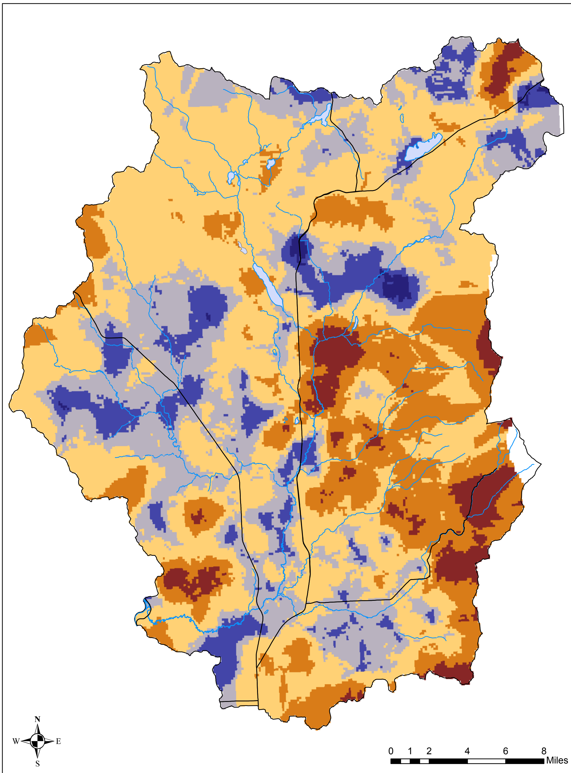
Figure 2-4 WRIA 55 Water Well Total Depth Spatial Variation
