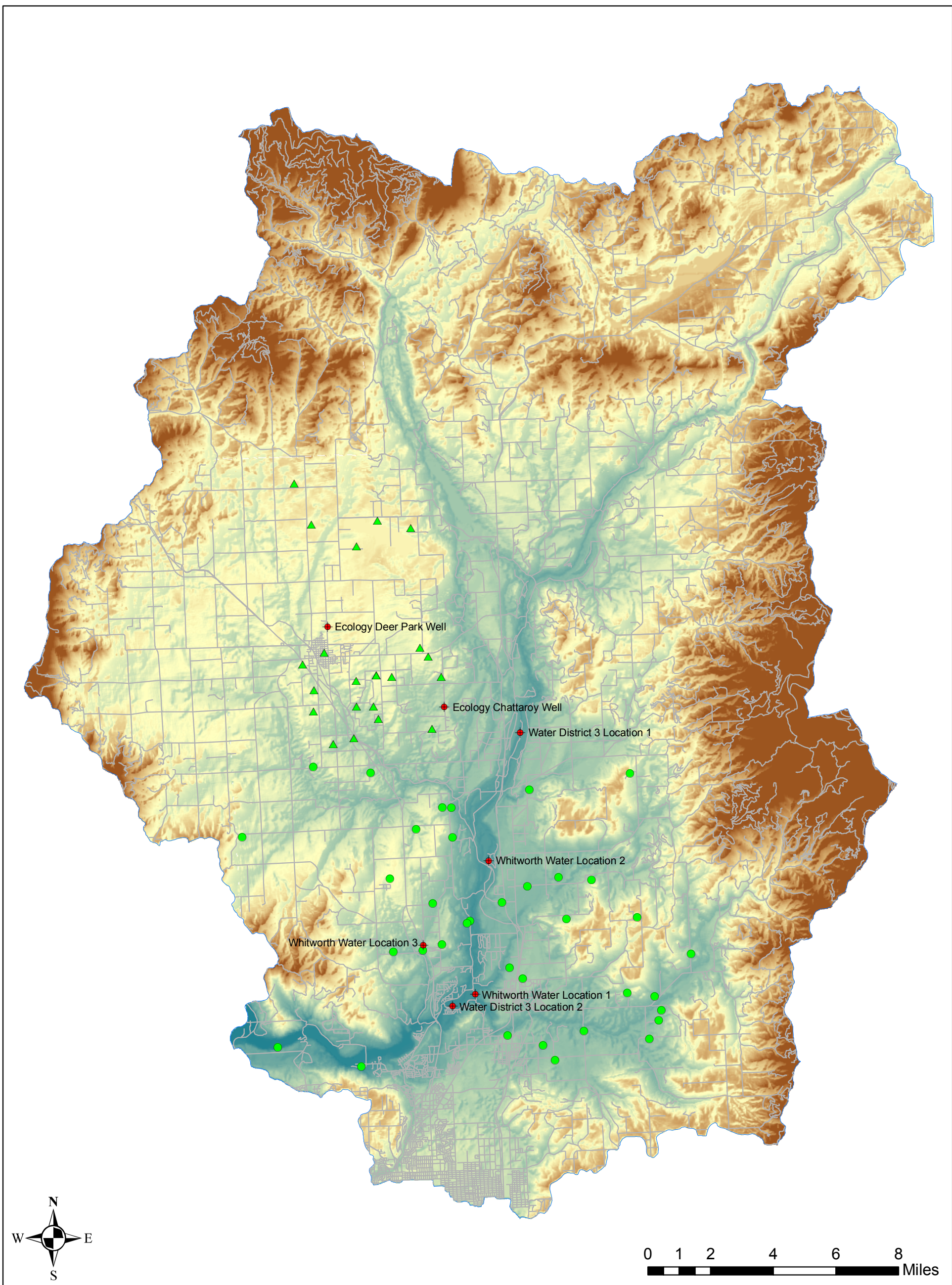
Figure 6-1 WRIA 55 Groundwater Elevation Monitoring Opportunities
