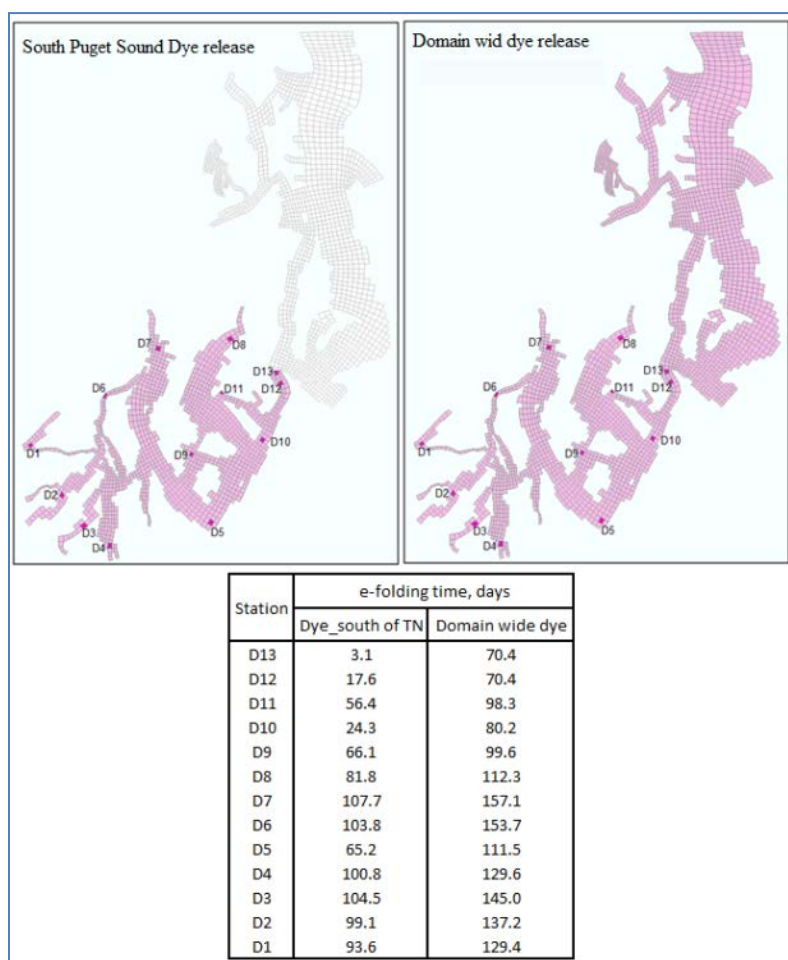
Figure 56. Flushing times at stations following South Puget Sound and domain wide initial dye release.
