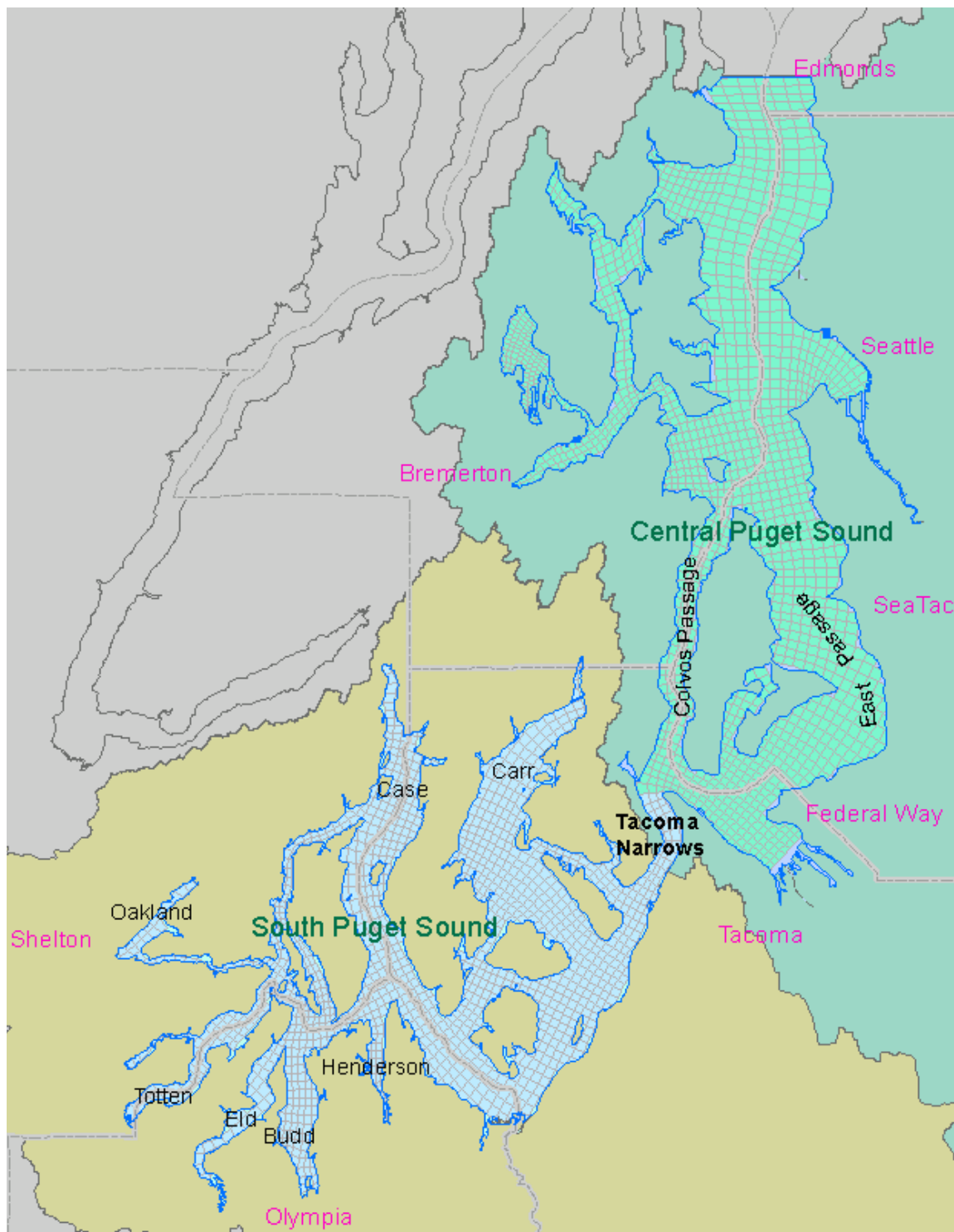
Figure 1. South Puget Sound Dissolved Oxygen Study waterbodies and place names.
