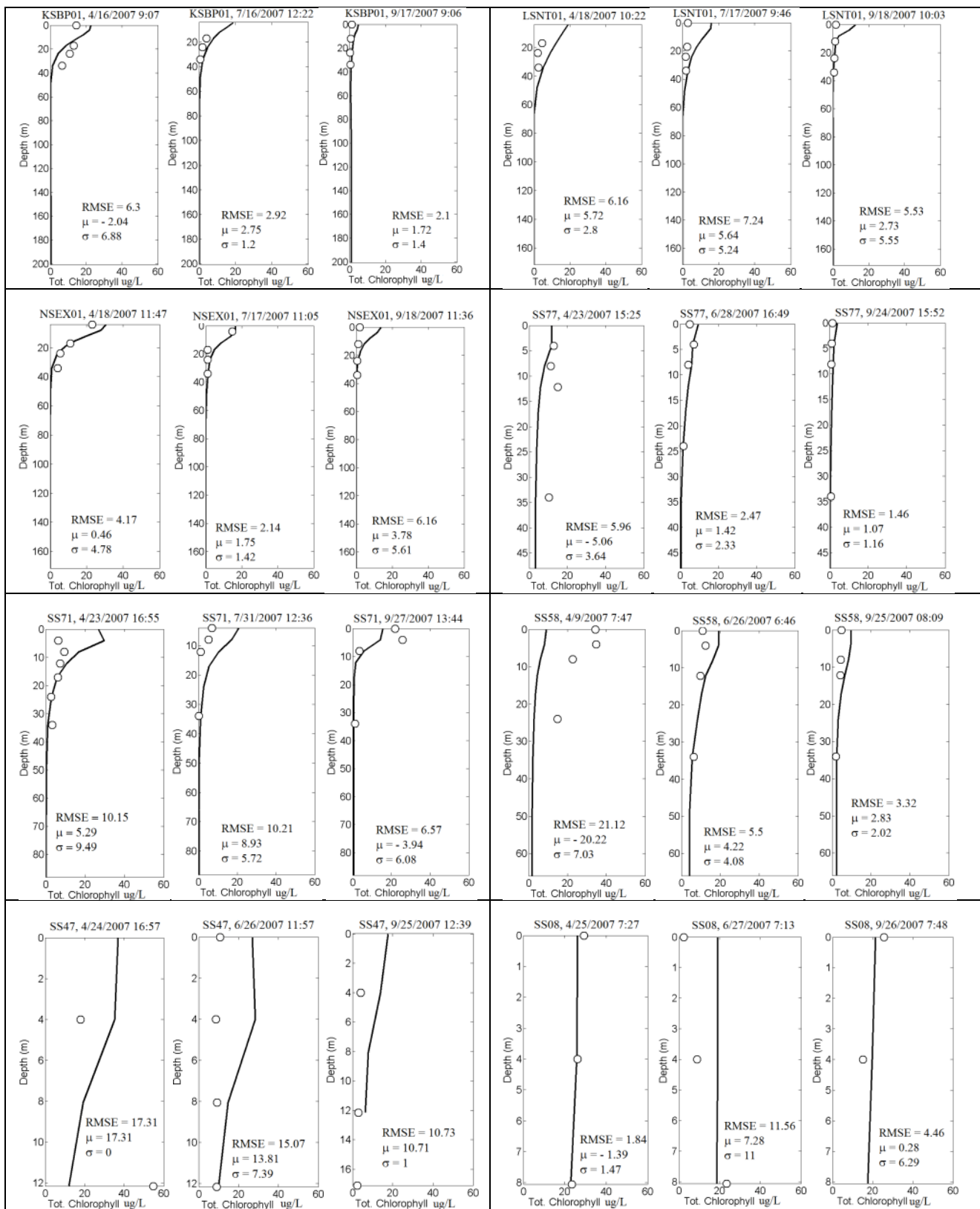
Figure 33. Chlorophyll profiles at selected stations in South and Central Puget Sound for spring, summer, and fall.
