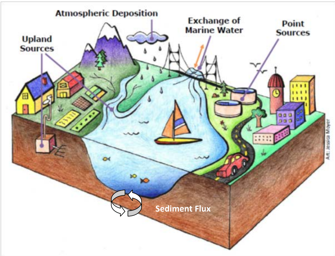
Figure 2. Sources of nitrogen in South and Central Puget Sound.
