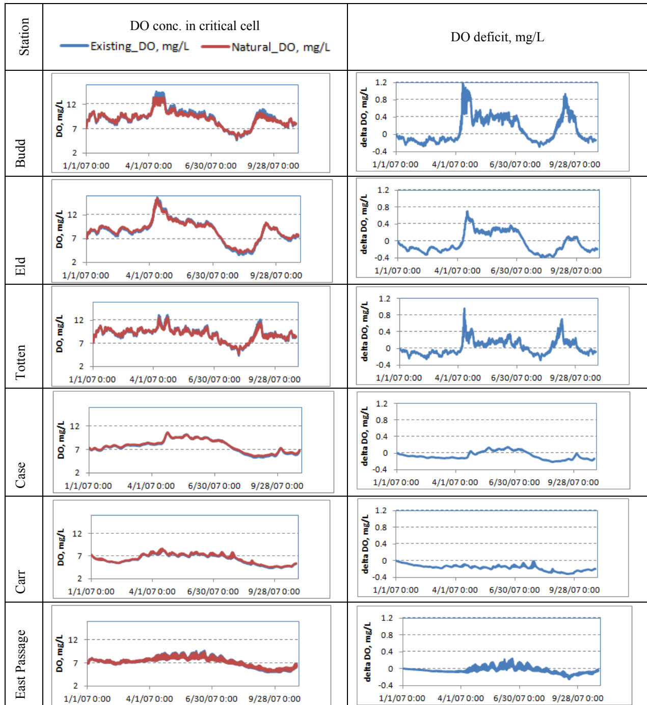
Figure 48. Existing and predicted natural DO concentration and deficit (delta DO) time series at critical cell (lowest DO concentration and maximum deficit) within each inlet and in East Passage
