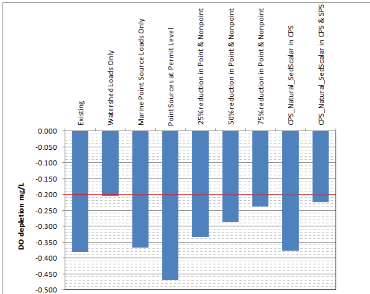
Figure 75. DO depletion in excess of 0.2 mg/L in the critical Eld Inlet cell.
