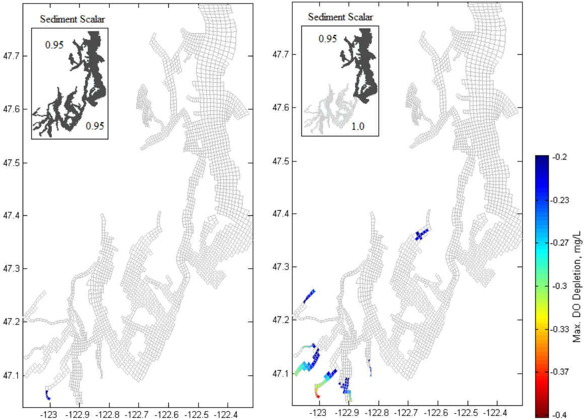
Figure 54. Regions of DO violations due to South Puget Sound sources only with Central Puget Sound at natural condition for sediment scalars adjusted in (a) both South and Central Puget Sound and (b) Central Puget Sound only.
