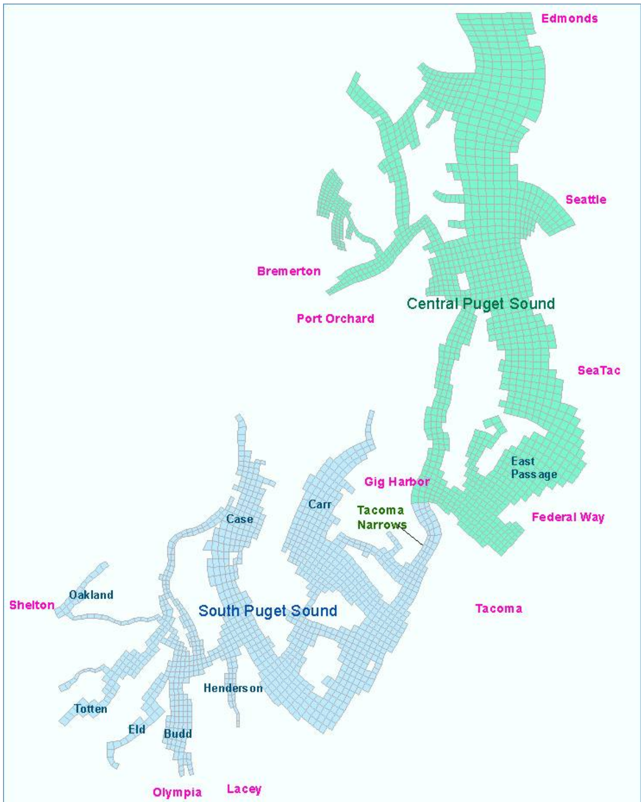
Figure 10. GEMSS model grid for South and Central Puget Sound showing major cities and inlet names.
