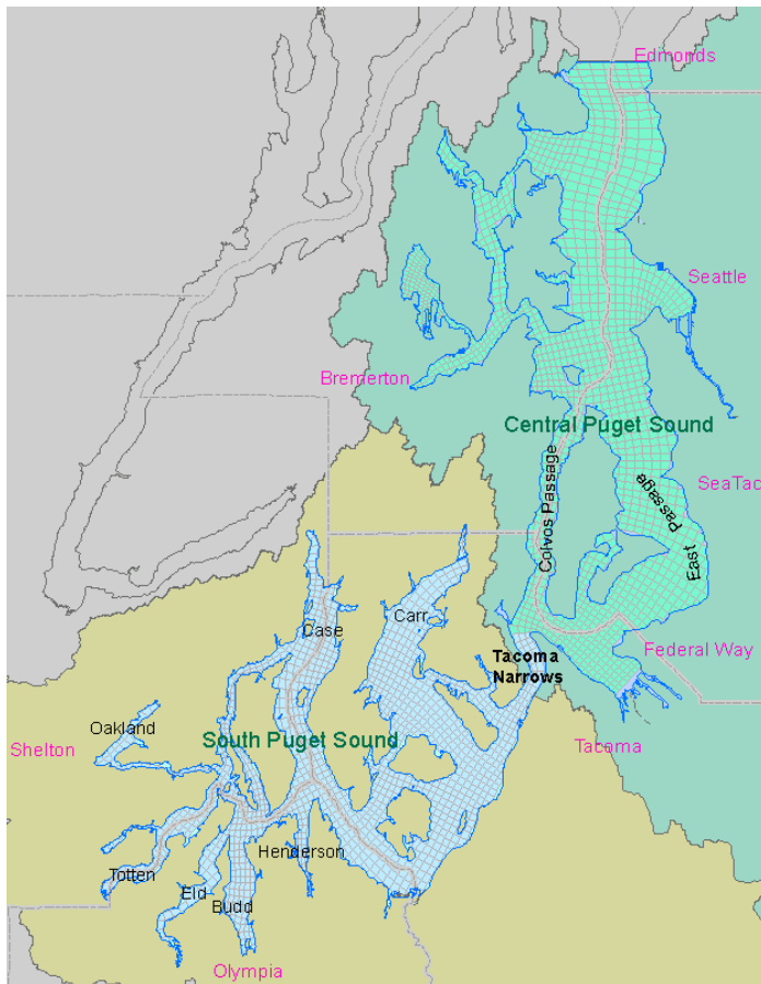
Figure ES-2. South and Central Puget Sound study area.
