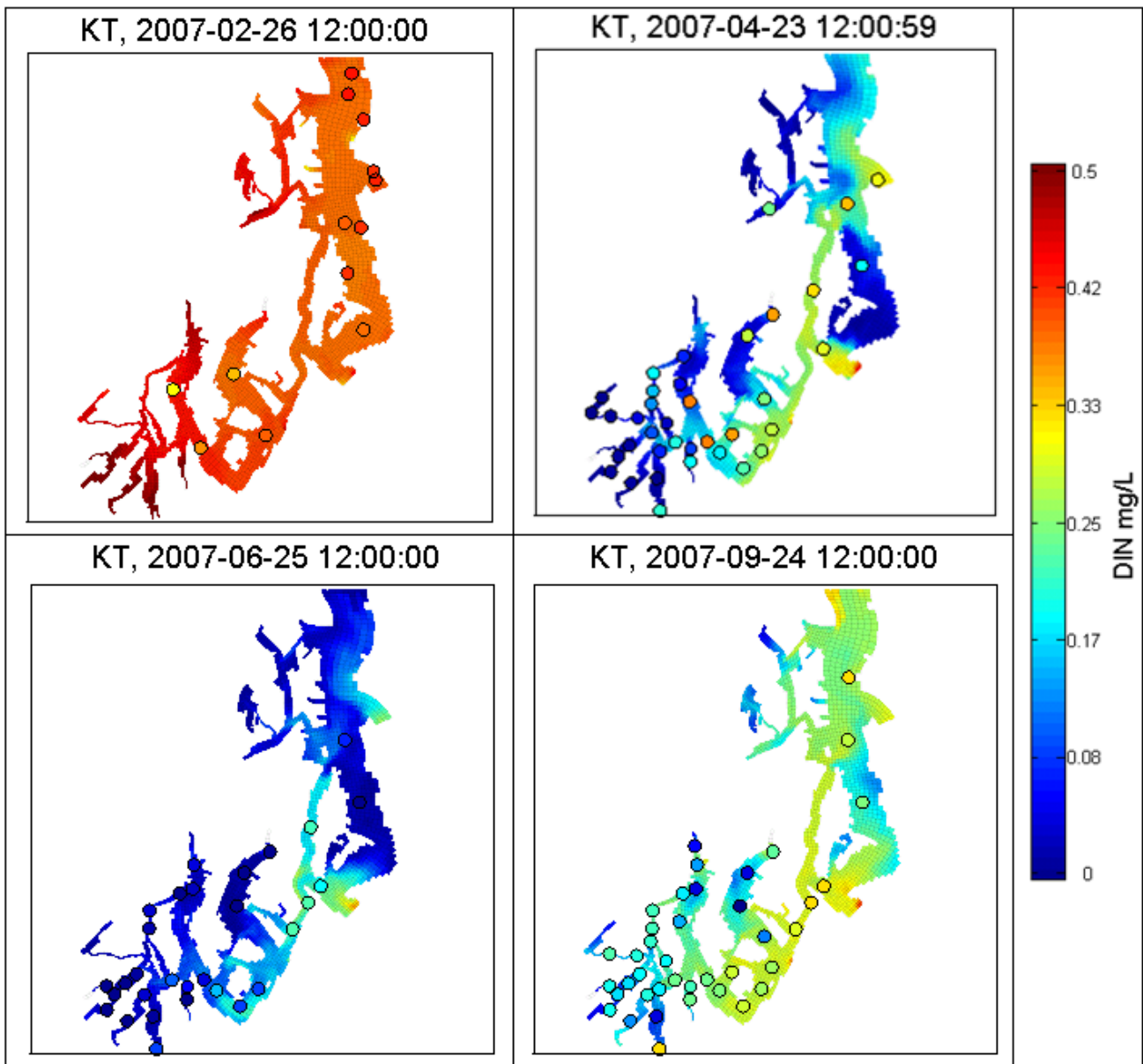
Figure 38. Spatial patterns for DIN in the surface (KT) layer during different times of the year (2007).
