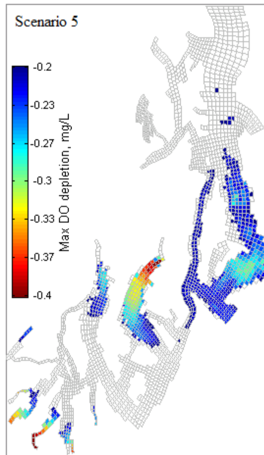
Figure 52. Regions of DO violations due to marine point sources at maximum permit values.
