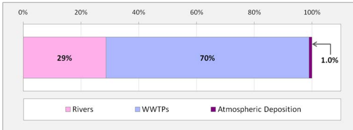
Figure 5. Annual dissolved inorganic nitrogen (DIN) loads from rivers, WWTPs, and atmospheric deposition to the surface of South and Central Puget Sound from 2006 to 2007.
