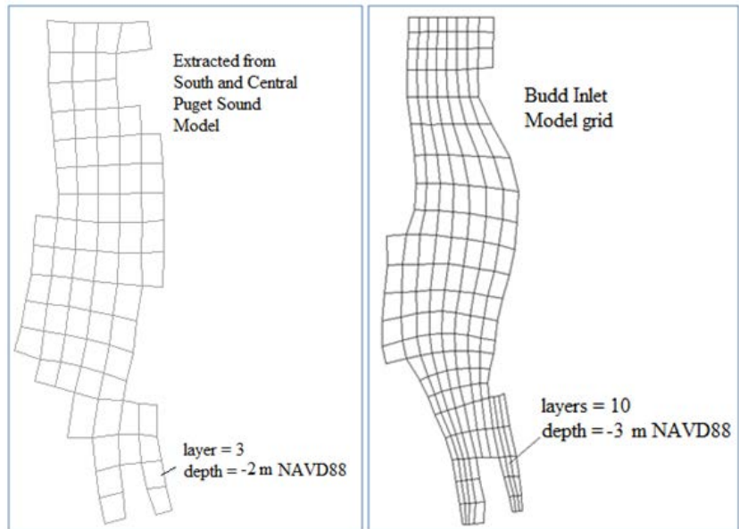
Figure 60. Budd Inlet grid distribution in South and Central Puget Sound Model (left) and Budd Inlet Model (right).
