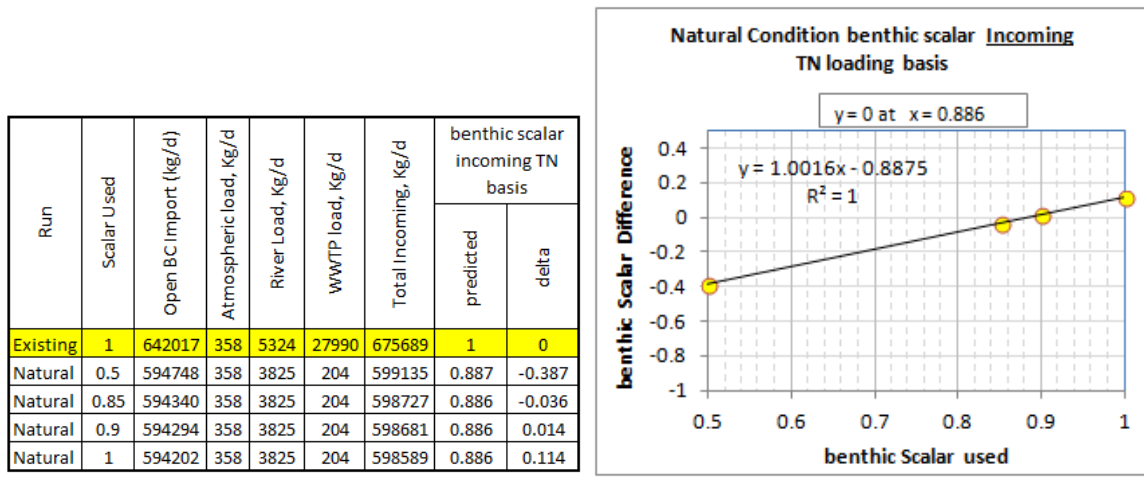
Figure F-2. Sediment scalar under natural conditions based on incoming total nitrogen load.
