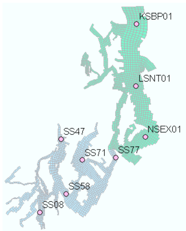
Figure 30. South Puget Sound and Central Puget Sound stations where water quality profiles were evaluated.
