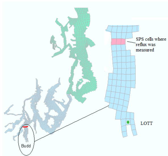
Figure 46. Northern boundary of Budd Inlet where reflux was measured when LOTT was turned off.
