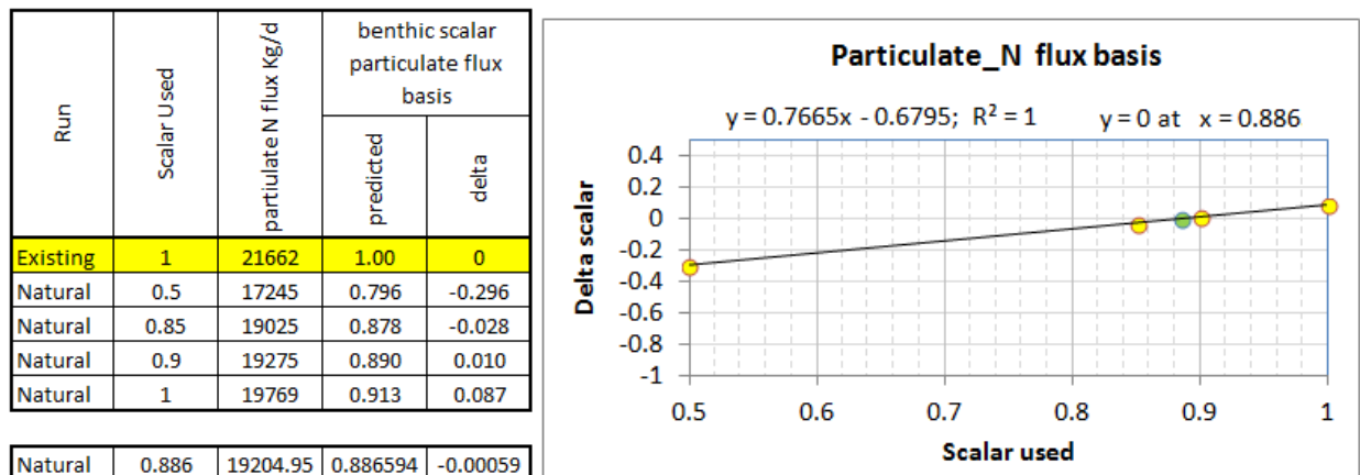
Figure F-1. Sediment scalar under natural conditions based on particulate nitrogen flux
