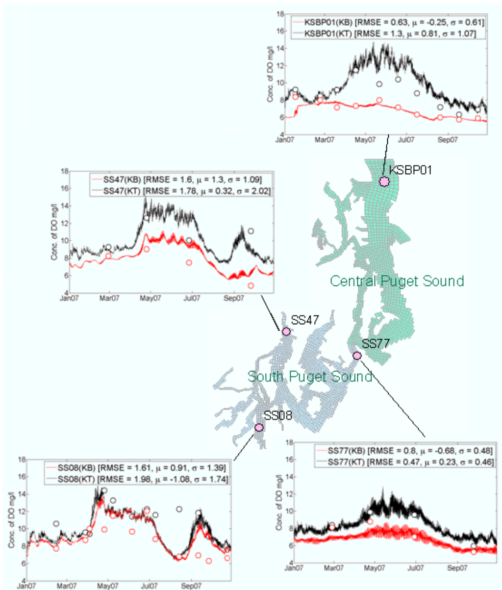
Figure 65. Measured and predicted DO concentrations in the surface (KT) and bottom layer (KB).
