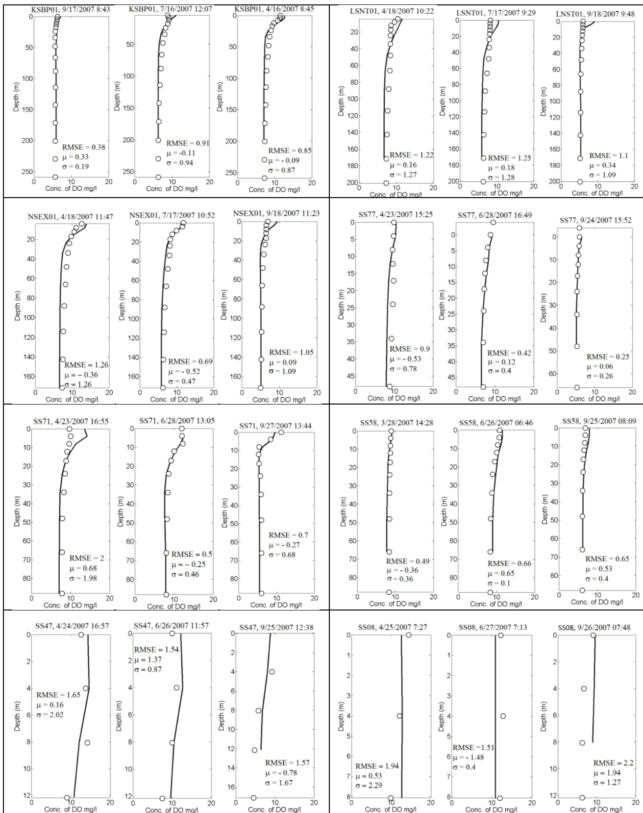
Figure 31. DO profiles at selected stations in South and Central Puget Sound for spring, summer, and fall.
