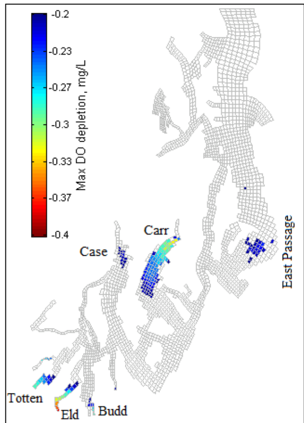
Figure ABS-1. Predicted dissolved oxygen standard violations under current conditions.
