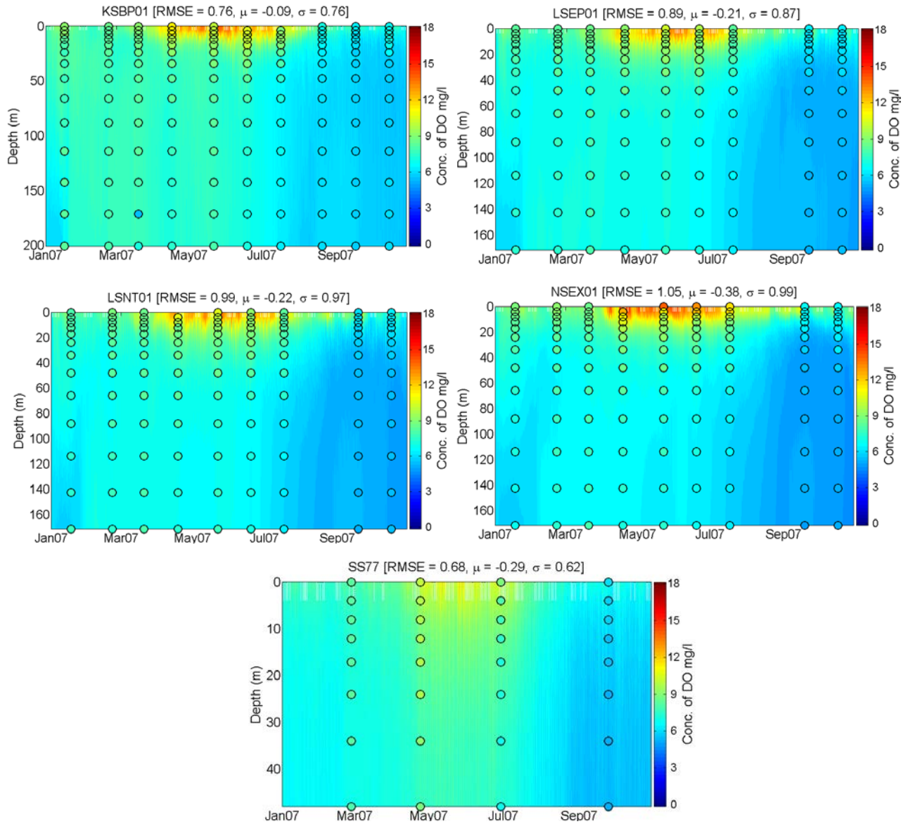
Figure 21. Time-depth contour plots of predicted and observed DO at Central Puget Sound calibration stations.
