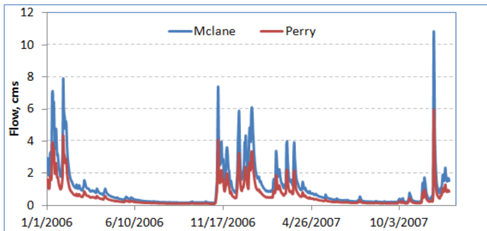
Figure 58. Flows in McLane and Perry Creeks.
