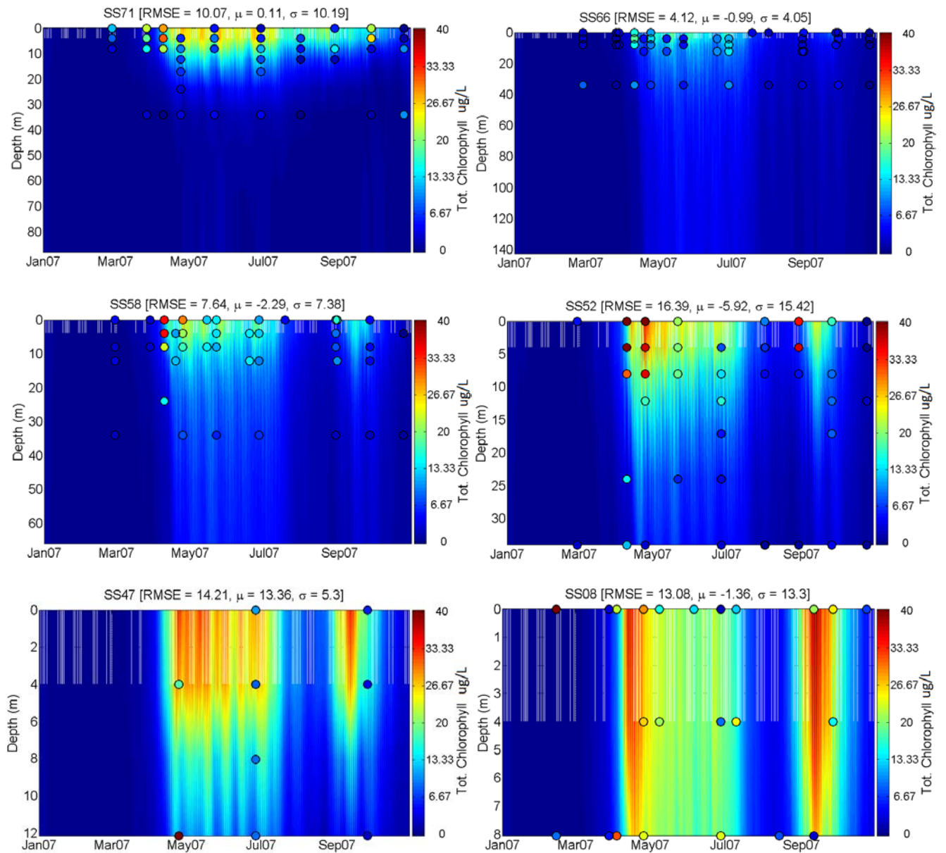
Figure 26. Time-depth contour plots of predicted and observed chlorophyll at South Puget Sound calibration stations.
