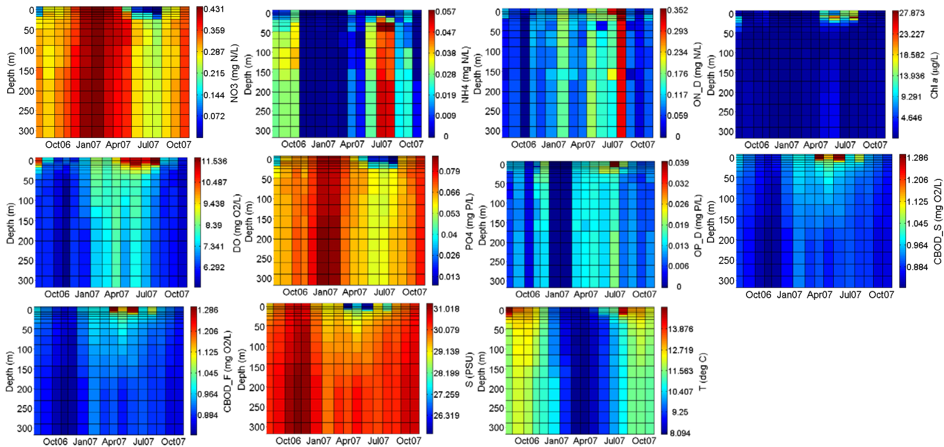
Figure 17. Water Quality characteristics at open boundary station EdmW based on monthly profiles.
