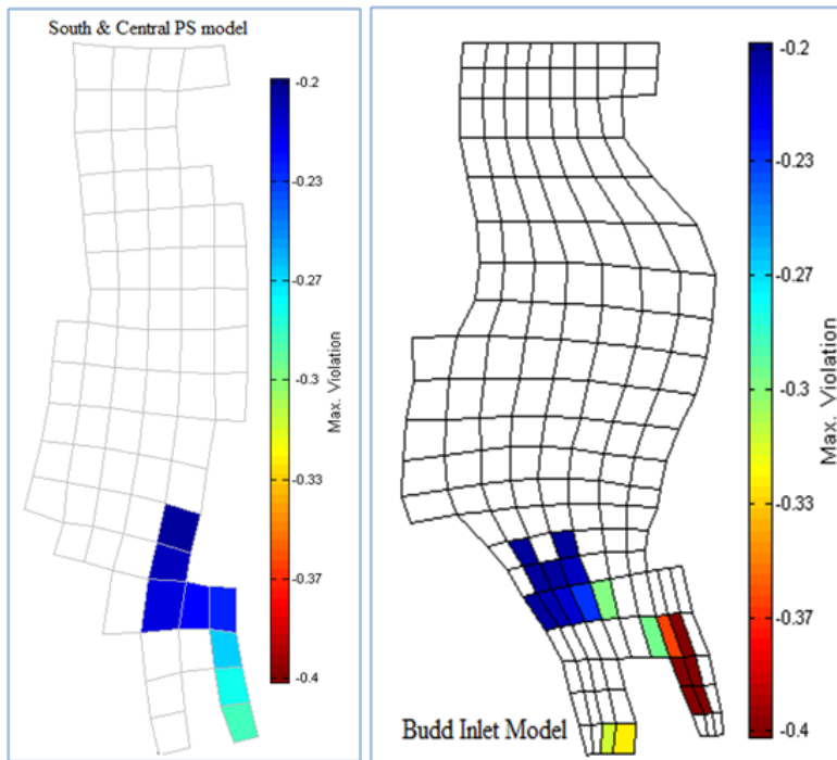
Figure 61. DO violations in Budd Inlet in South and Central Puget Sound model (with Capitol Lake) and Budd Inlet Model (without Capitol Lake) (Roberts et al., 2012).
