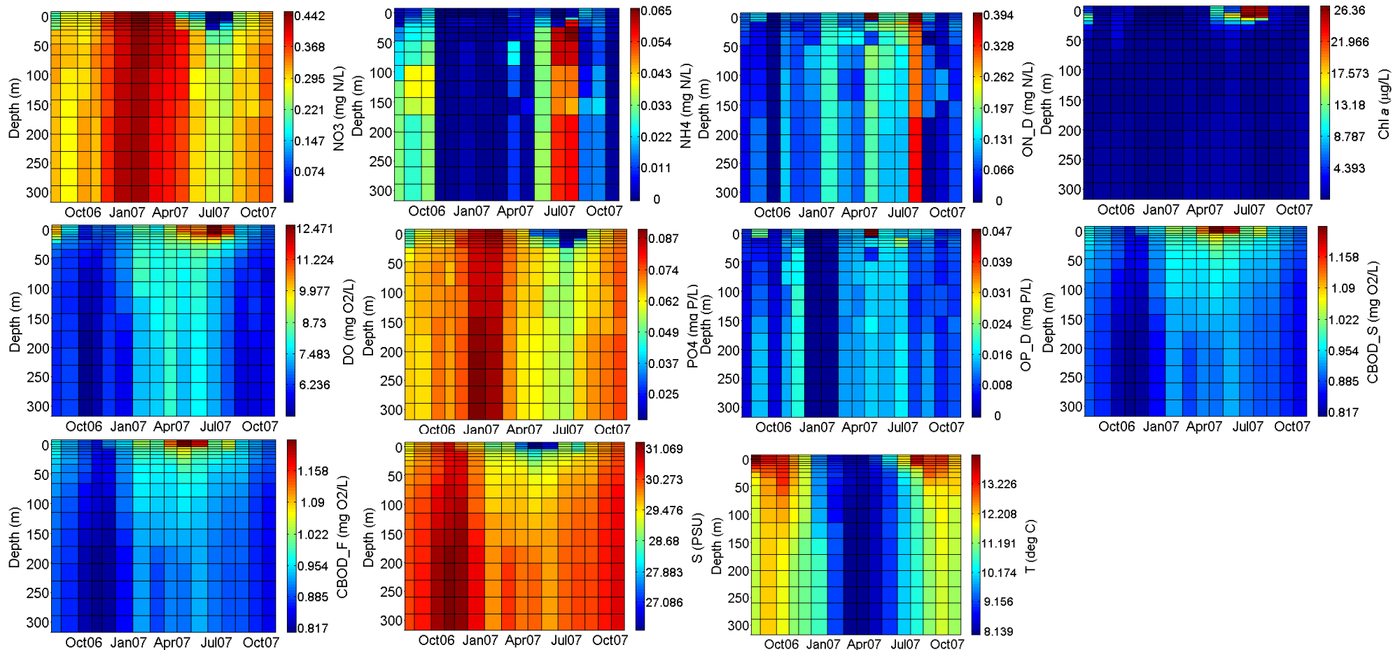
Figure 16. Water quality characteristics of open boundary station EdmE based on monthly profiles.
