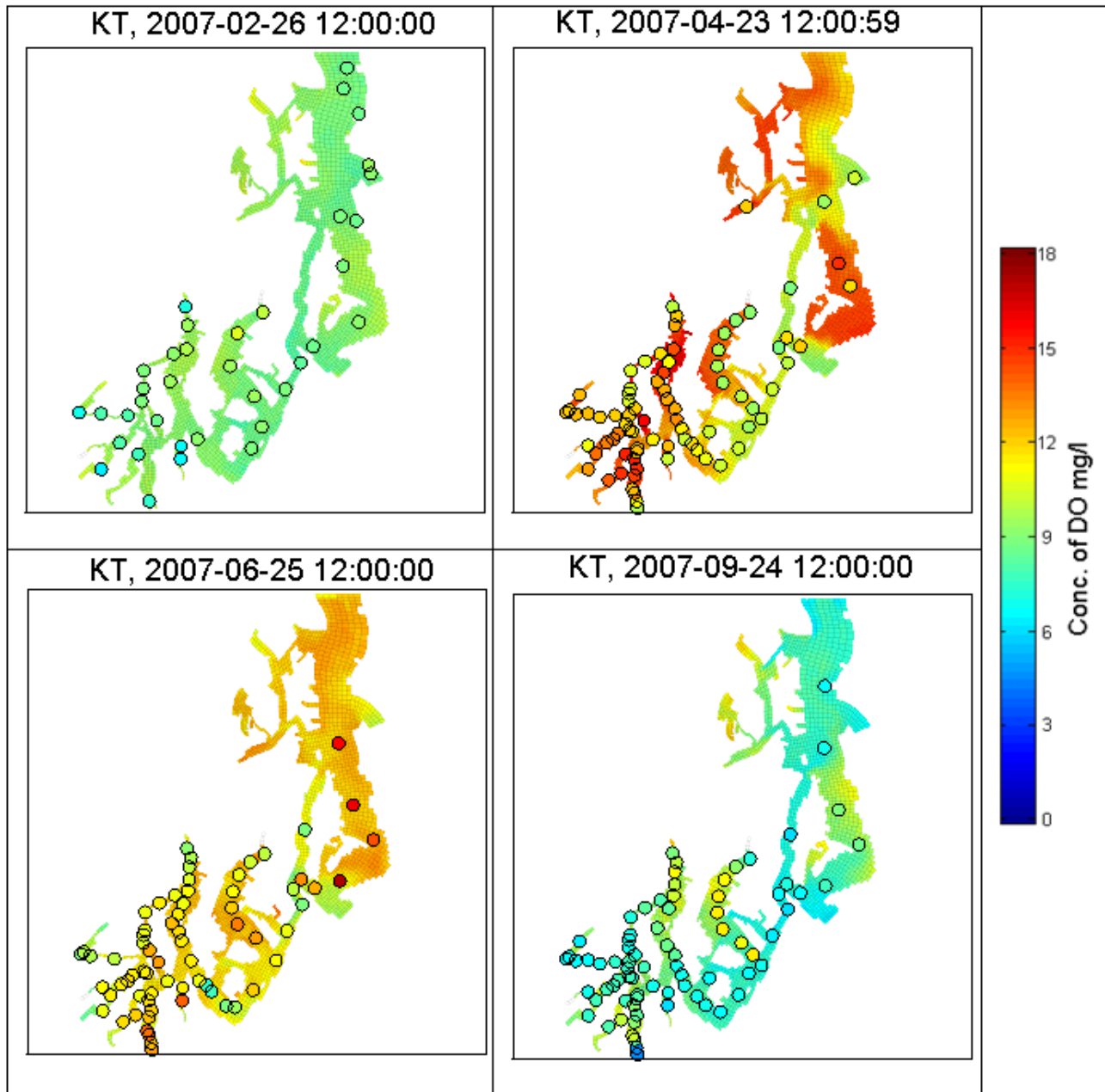
Figure 36. Spatial patterns for DO in the surface (KT) layer during different times of the year (2007).
