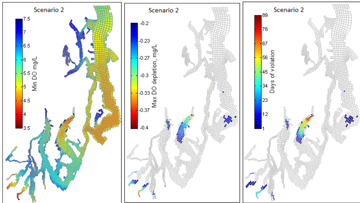
Figure 47. Minimum DO and DO standard violations (magnitudes and duration) due to current anthropogenic loads (2007 conditions).
