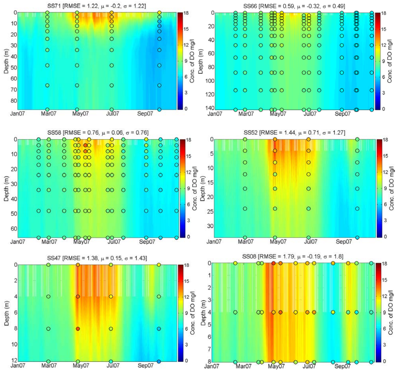
Figure 22. Time-depth contour plots of predicted and observed DO at South Puget Sound calibration stations.
