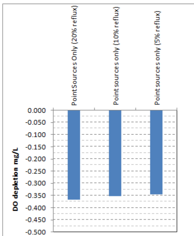
Figure 62. Sensitivity analysis for different percent reflux on DO depletion at the critical Eld Inlet cell.
