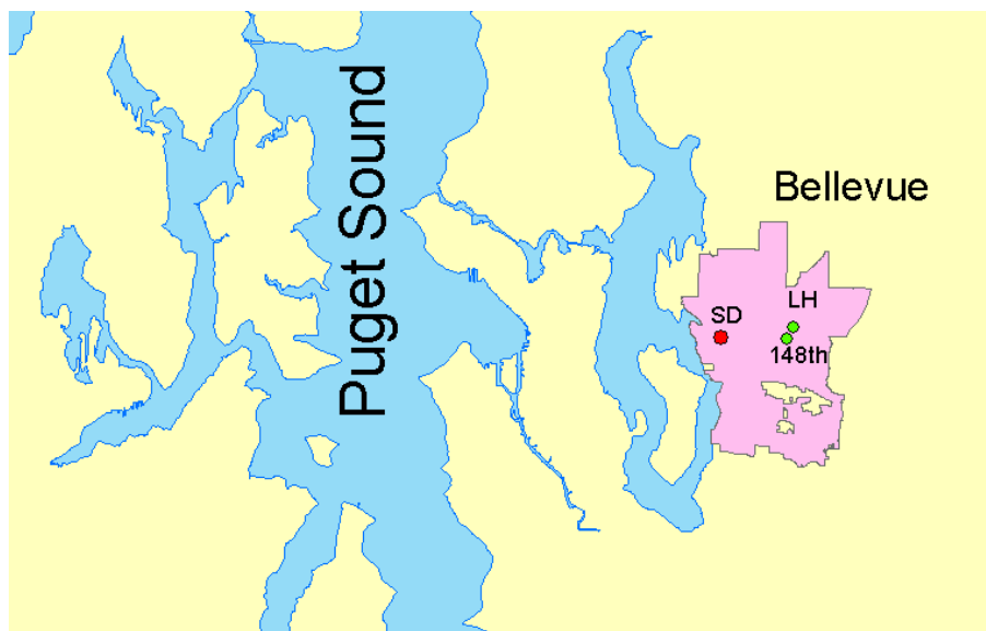
Figure 14. Locations of stations in the city of Bellevue, WA where atmospheric deposition rates were measured by Ebbert et al. (1985).
