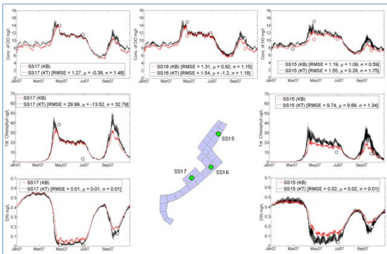
Figure 59. Time series plots for DO, chlorophyll, and dissolved inorganic nitrogen (DIN) in Eld Inlet stations.
