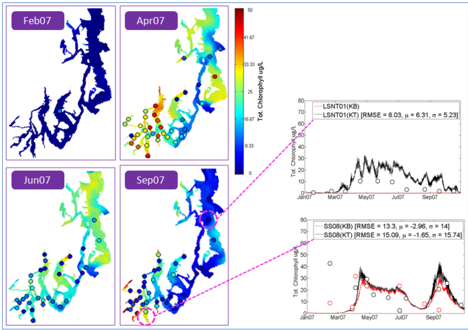
Figure 68. Hourly predictions of surface layer chlorophyll a concentrations (ug/L) for (a) February 2007, (b) April 2007, (c) June 2007, and (d) September 2007 with data collected within 5 days of the simulated date and time in circles.
