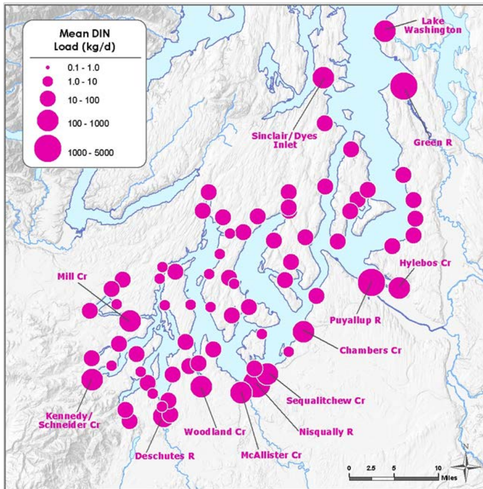
Figure 12. Mean annual dissolved inorganic nitrogen (DIN) loads from watersheds into South and Central Puget Sound (2006-07). Source: Mohamedali et al. (2011).
