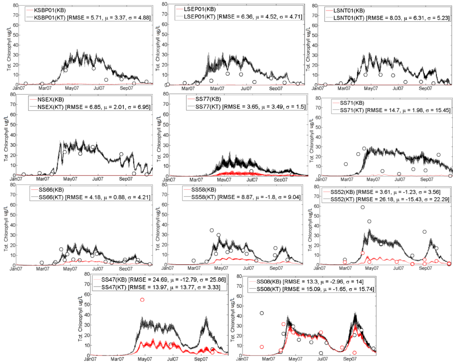
Figure 29. Time series plot of chlorophyll at surface (KT) and bottom (KB) layers (see Figure 20 for station locations).
