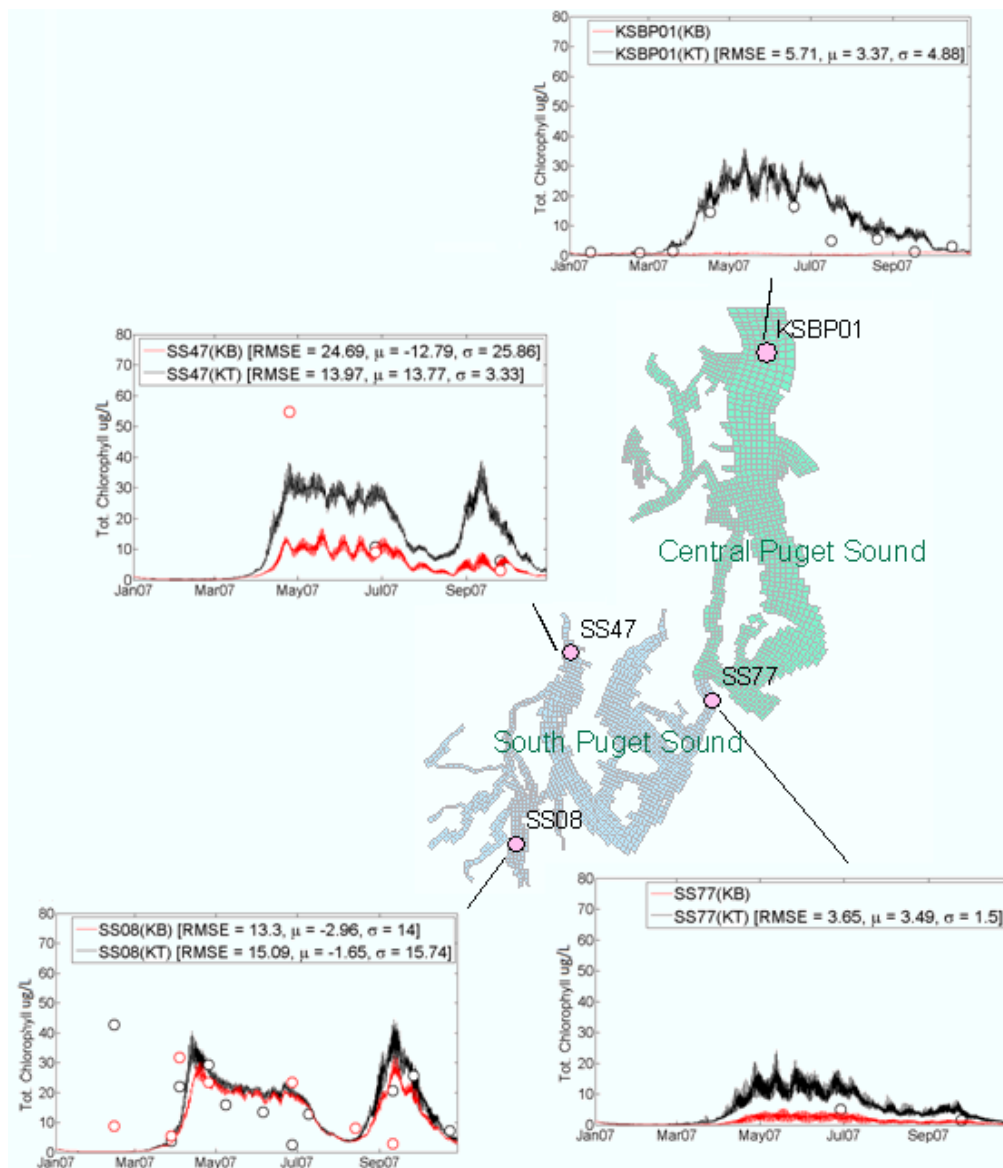
Figure 67. Measured and predicted chlorophyll concentrations in the surface (KT) and bottom layer (KB).
