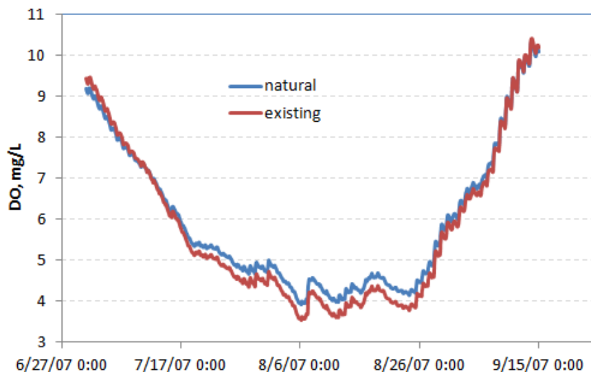
Figure 74. DO concentrations at critical cell in Eld Inlet under current and natural conditions
