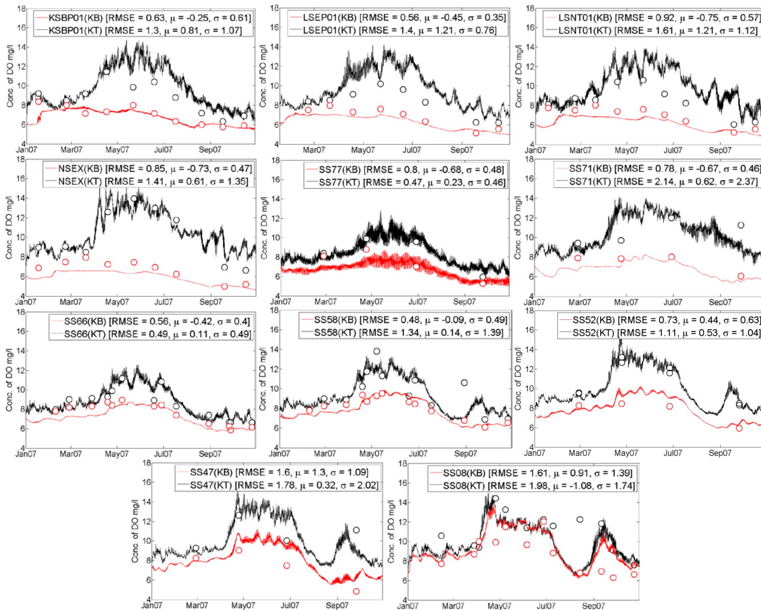
Figure 27. Time-series plot of DO at surface (KT) and bottom (KB) layers (see Figure 20 for station locations).
