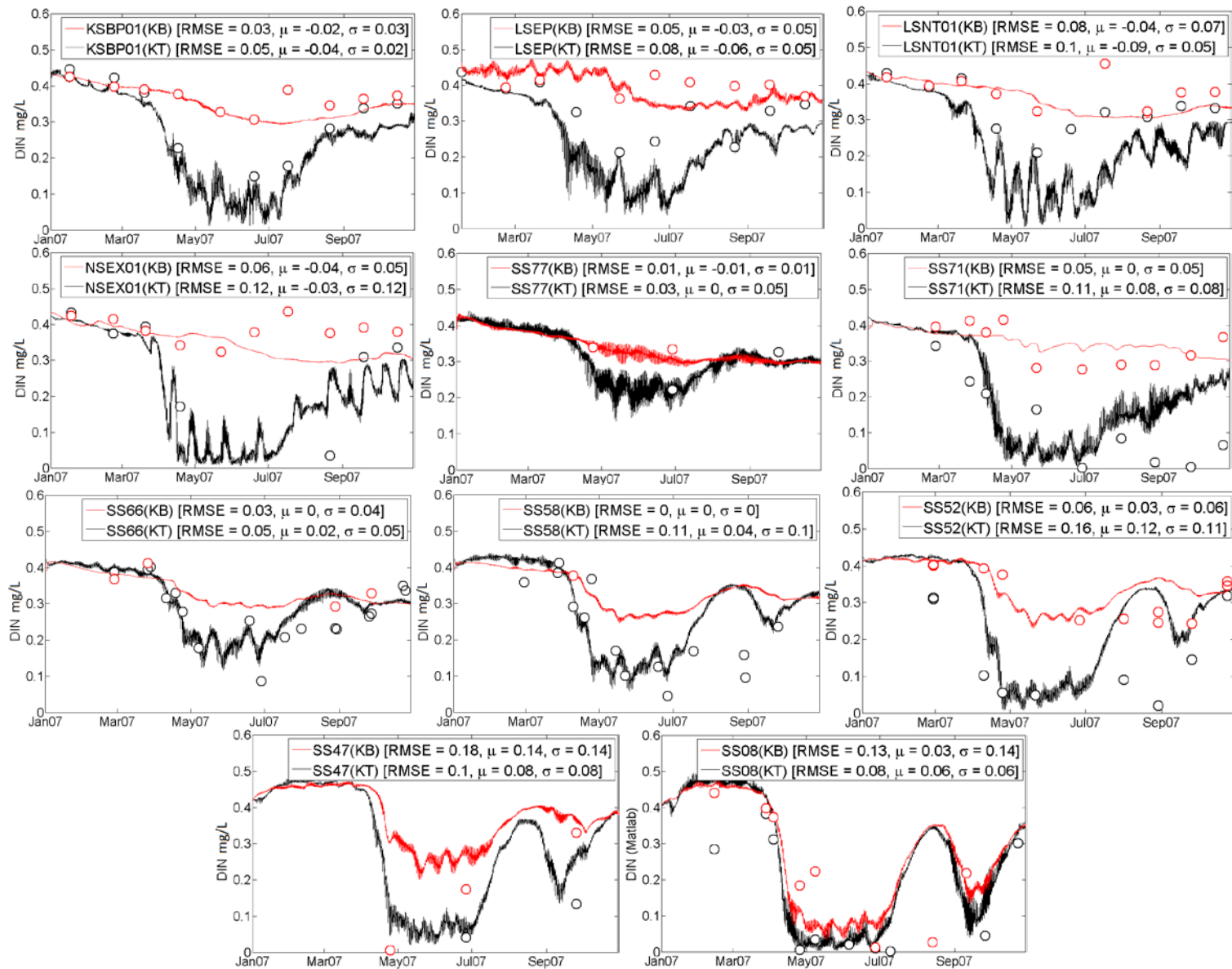
Figure 28. Time-series plot of DIN at surface (KT) and bottom (KB) layers (see Figure 20 for station locations).
