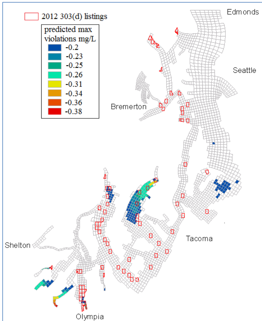
Figure 73. Predicted violations of water quality standards for DO (based on limiting numeric criteria and/or natural conditions) and 303(d) listings (based on numeric standards)
