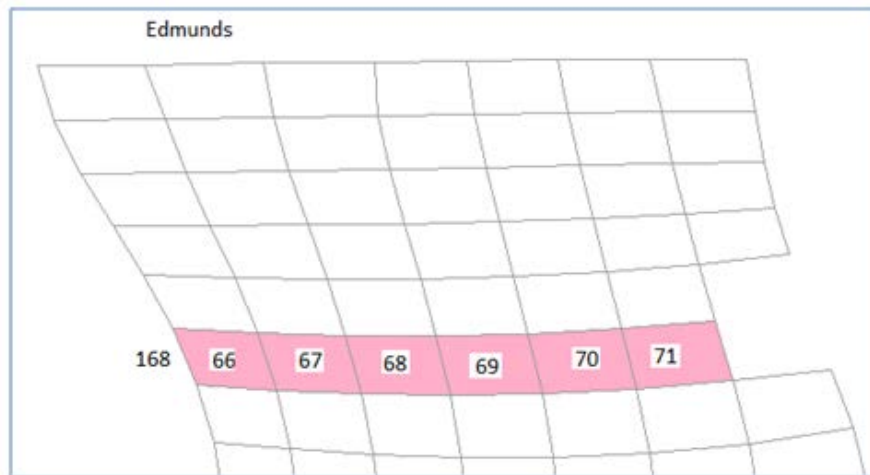
Figure F-3. Grid cells south of Edmonds where incoming total nitrogen load was estimated.
