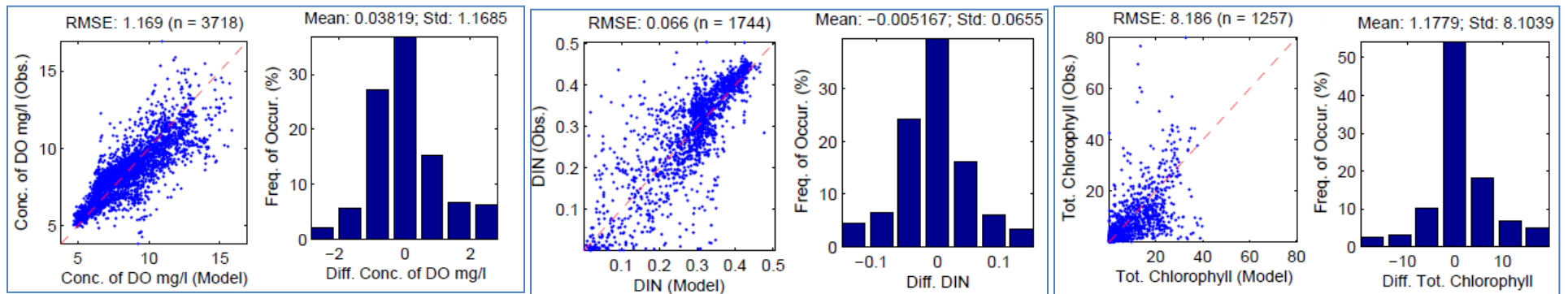
Figure 35. Goodness of fit for DO, DIN, and total chlorophyll predictions for 2007 across all stations used in the calibration.
