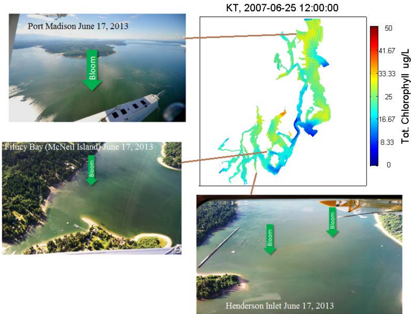
Figure 43. Comparing surface photos (June 17, 2013) from Eyes Over Puget Sound (EOPS) to model predictions (June 25, 2007).
