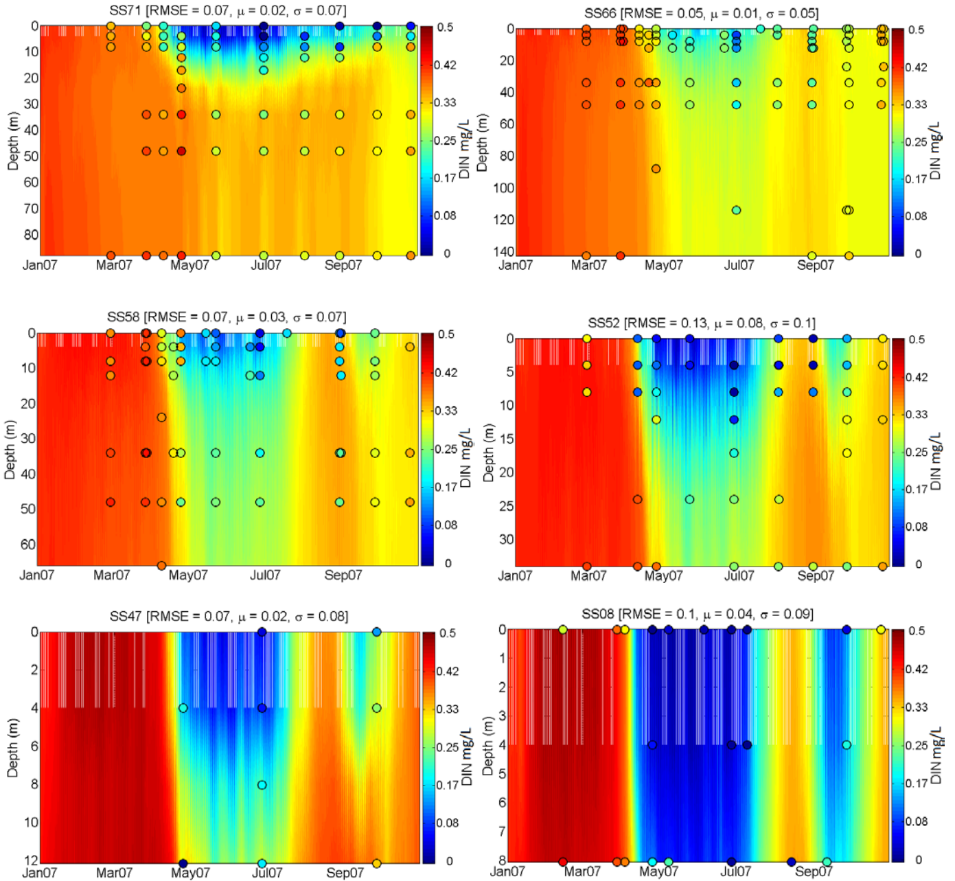
Figure 24. Time-depth contour plots of predicted and observed DIN at South Puget calibration stations. See Figure 20 for station locations.
