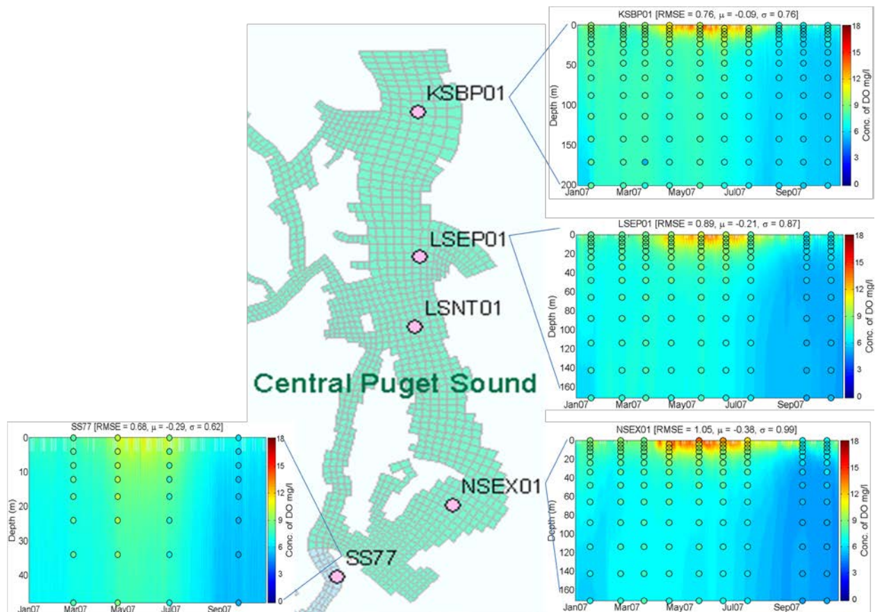
Figure 63. Predicted DO depth-time plots for key stations in Central Puget Sound.
