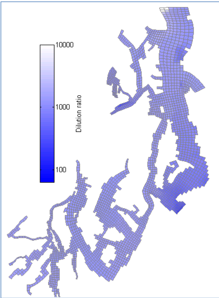
Figure 55. Dilution factors calculated from maximum water-column dye concentrations for Central Puget Sound wastewater discharge tracer simulations (September 2007).
