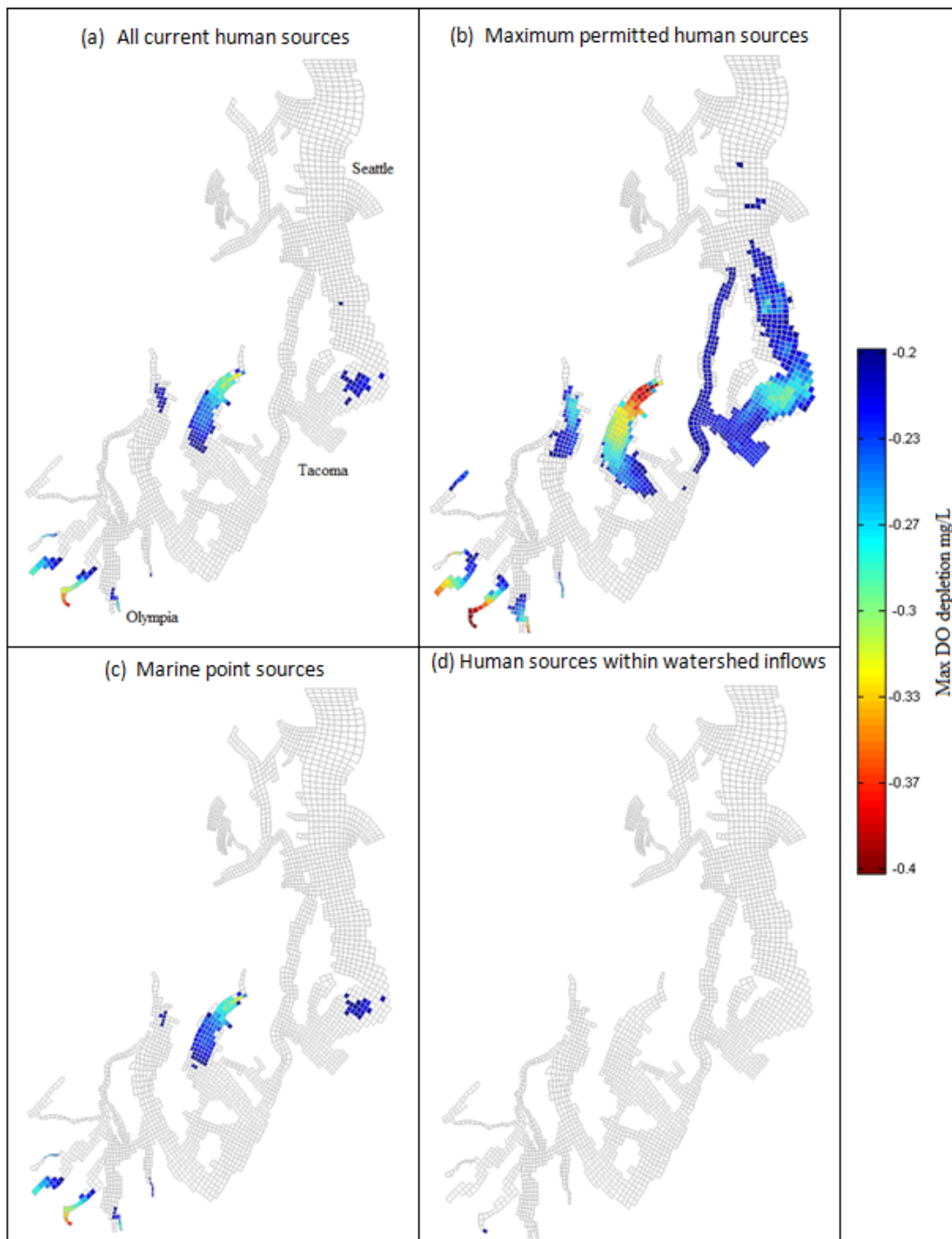
Figures ES-3. Regions where current nutrient loads cause > 0.2 mg/L DO depletion for 2007 conditions.
