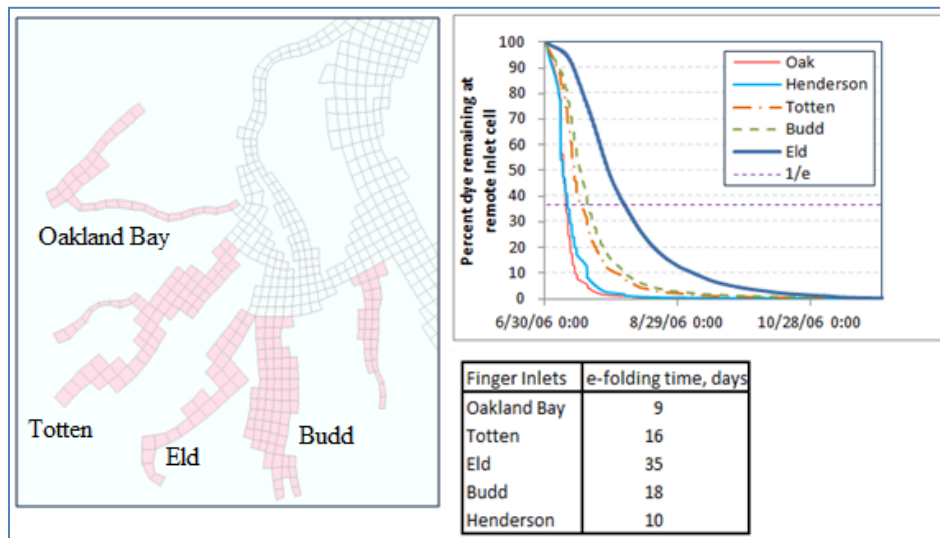
Figure 57. E-folding time for remote cell in each inlet. Time to dilute to 1/e level, i.e., 37% of original concentration.
