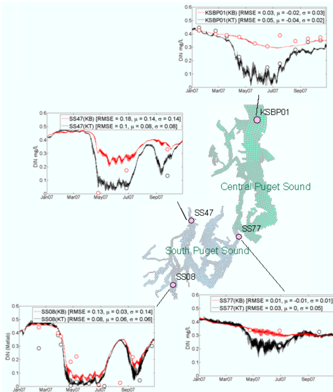
Figure 66. Measured and predicted dissolved inorganic nitrogen (DIN) concentrations in the surface (KT) and bottom layer (KB).
