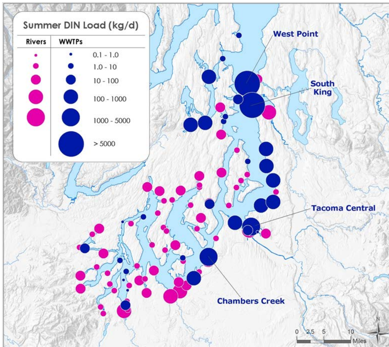
Figure 4. Mean summer dissolved inorganic nitrogen (DIN) loads from rivers and WWTPs into South and Central Puget Sound from 2006 to 2007.
