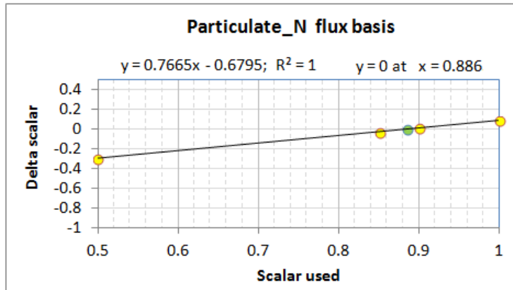
Figure 44. Plot of difference between used and predicted sediment scalars versus scalar used. The yellow dots represent the different trials on which the regression equation is based. The green dot signifies the final scalar for which the difference between used and predicted scalar is zero.
