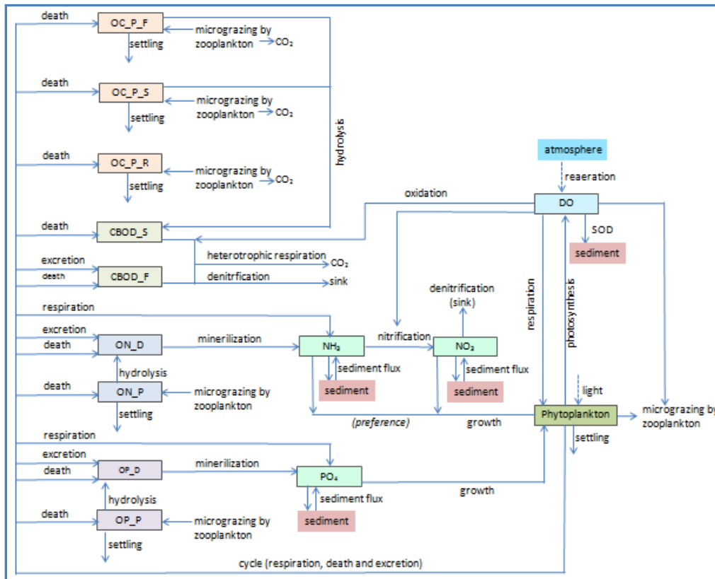
Figure 9. Flowchart of GEMSS-WQCBM model.
