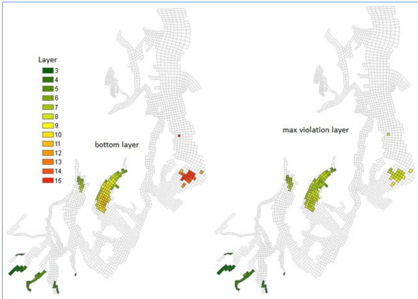
Figure 49. Number of layers in the water column (left) and the layer with DO standard violation (right) in cells where DO standard violations were predicted.
