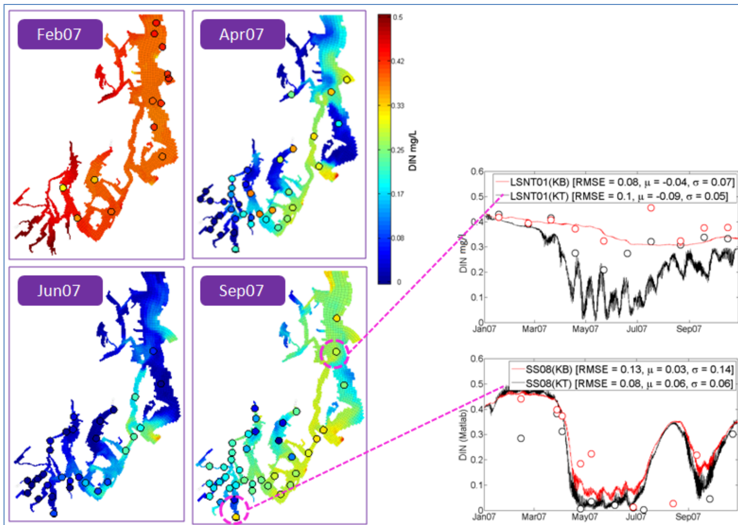
Figure 70. Hourly predictions of surface layer dissolved inorganic nitrogen (DIN) concentrations (mg/L) for (a) February 2007, (b) April 2007, (c) June 2007, and (d) September 2007 with data collected within 5 days of the simulated date and time in circles.
