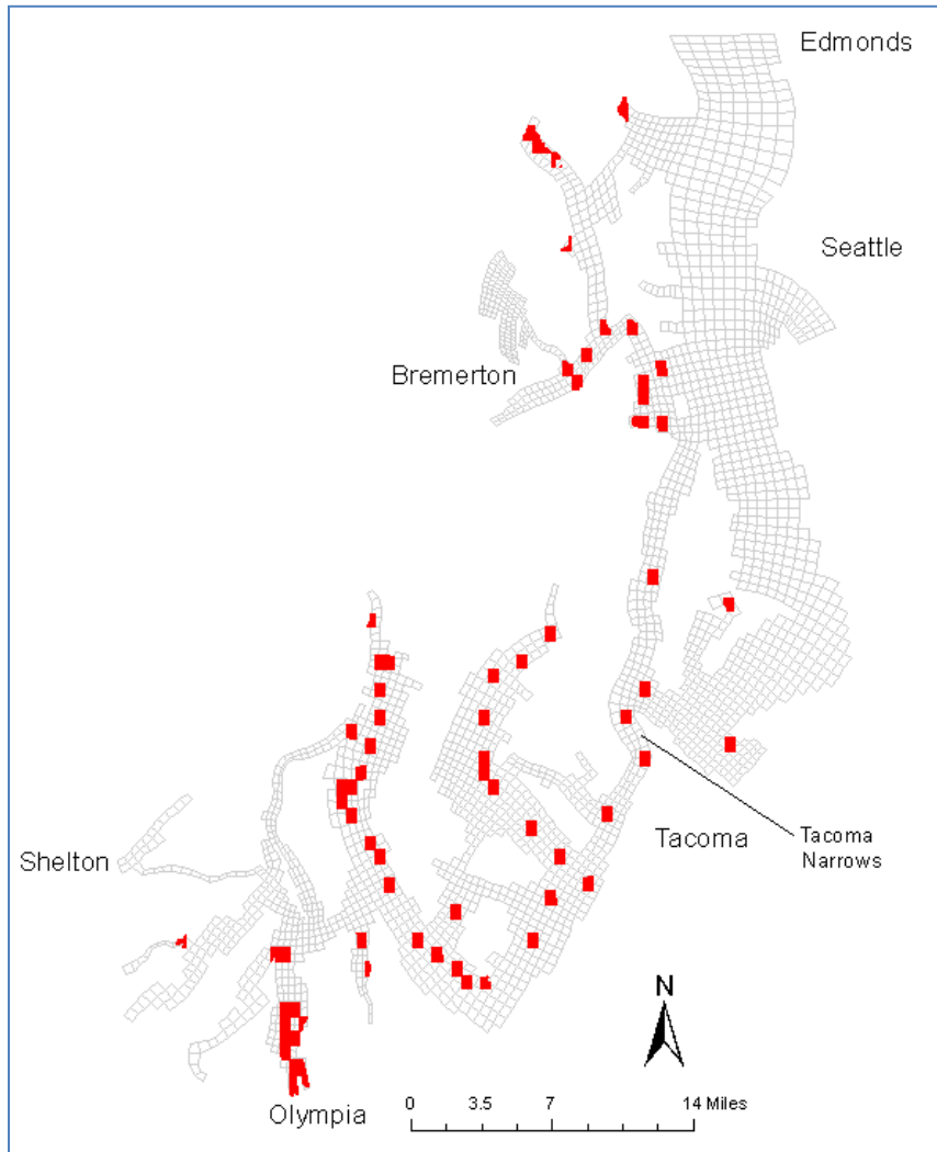
Figure 8. 2012 Category 5 (impaired waters) listings of marine DO in South and Central Puget Sound.
