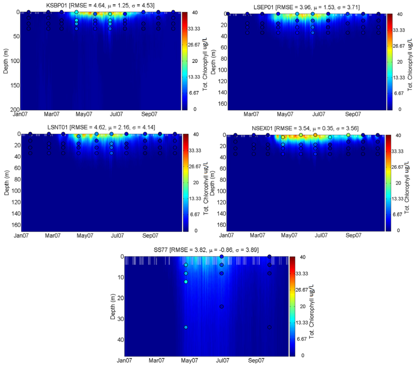
Figure 25. Time-depth contour plots of predicted and observed chlorophyll at Central Puget Sound calibration stations.
