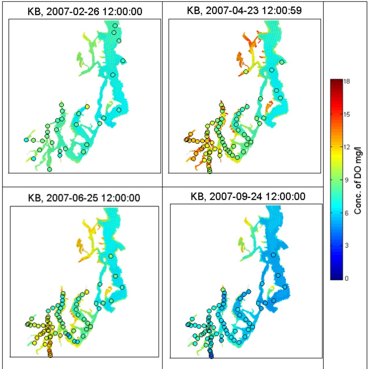
Figure 37. Spatial patterns for DO in the bottom (KB) layer during different times of the year (2007).
