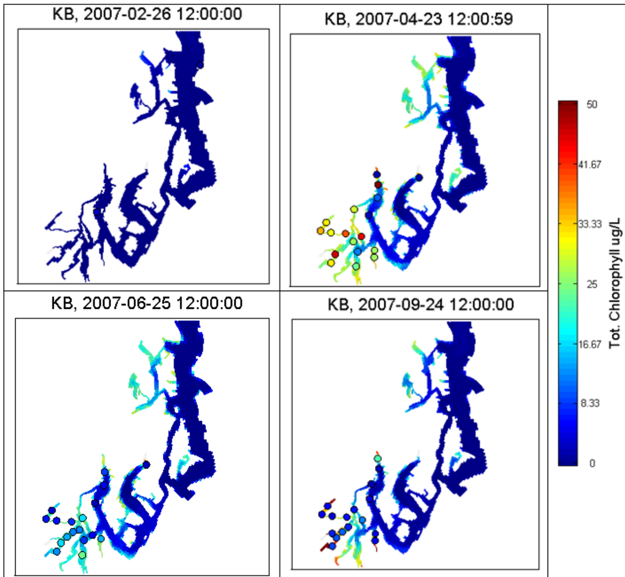
Figure 41. Spatial patterns for total chlorophyll in the bottom (KB) layer during different times of the year (2007).
