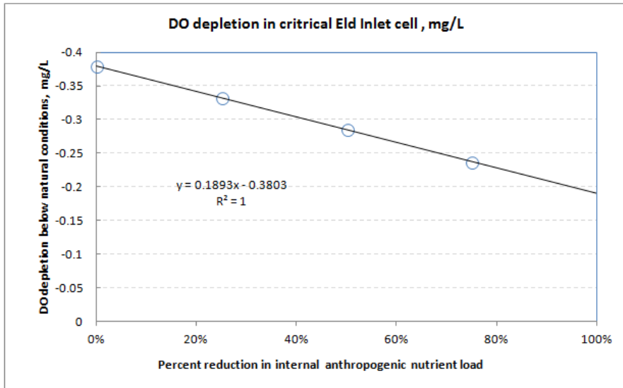
Figure 76. DO depletion in critical Eld Inlet cell in response to percent reductions in internal anthropogenic nutrient load.
