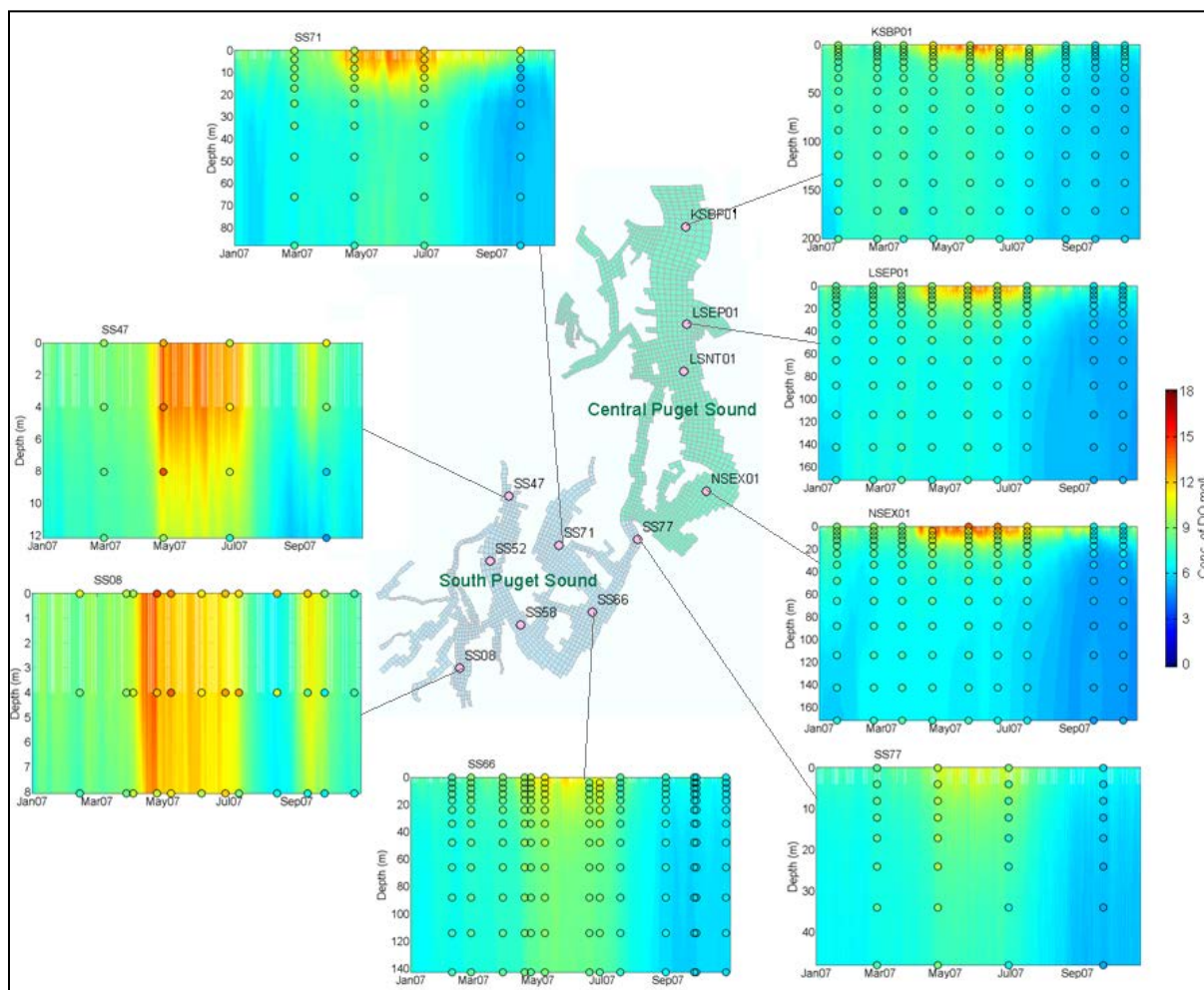
Figure ES-5. Predicted and observed DO at key locations in (a) Central and (b) South Puget Sound.
