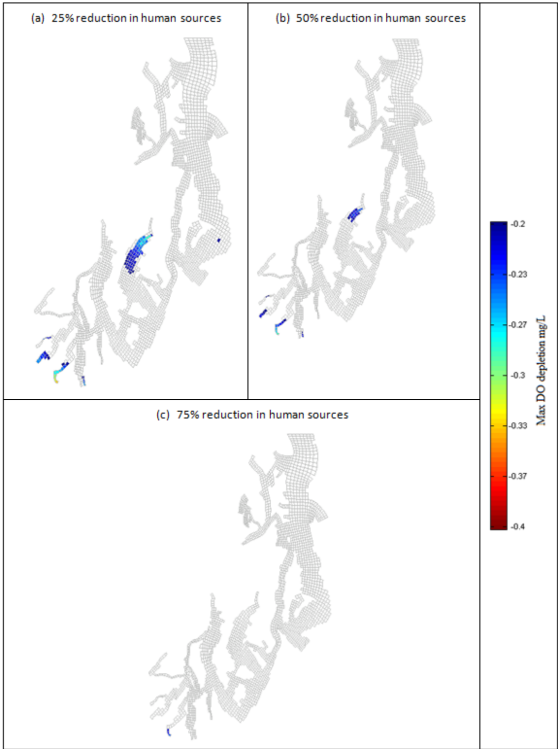
Figure ES-4. Regions where loads reduced by (a) 25%, (b) 50%, or (c) 75% would cause >0.2 mg/L DO depletion for 2007 conditions.
