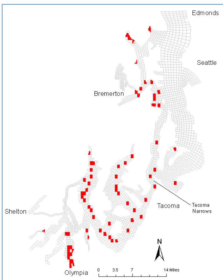
Figure ES-1. 2012 Clean Water Act Section 303(d) Category 5 (impaired waters) listings for marine DO in South and Central Puget Sound with the model grid.
