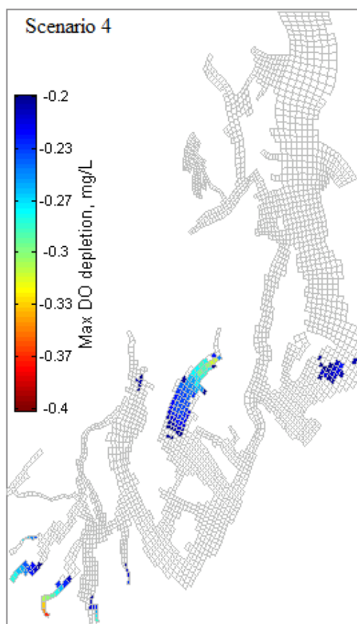
Figure 51. Regions of DO violations due to marine point sources only.
