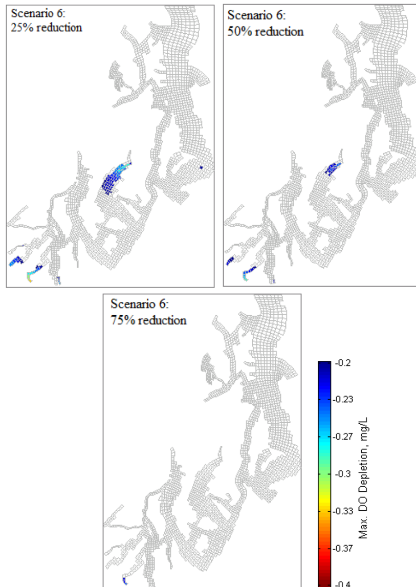
Figure 53. Regions of DO violations with 25, 50 and 75 percent reductions of both human watershed loads and marine point sources loads.
