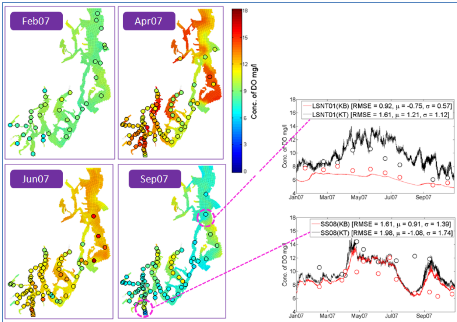
Figure 69. Hourly predictions of surface layer DO concentrations (mg/L) for (a) February 2007, (b) April 2007, (c) June 2007, and (d) September 2007 with data collected within 5 days of the simulated date and time in circles.
