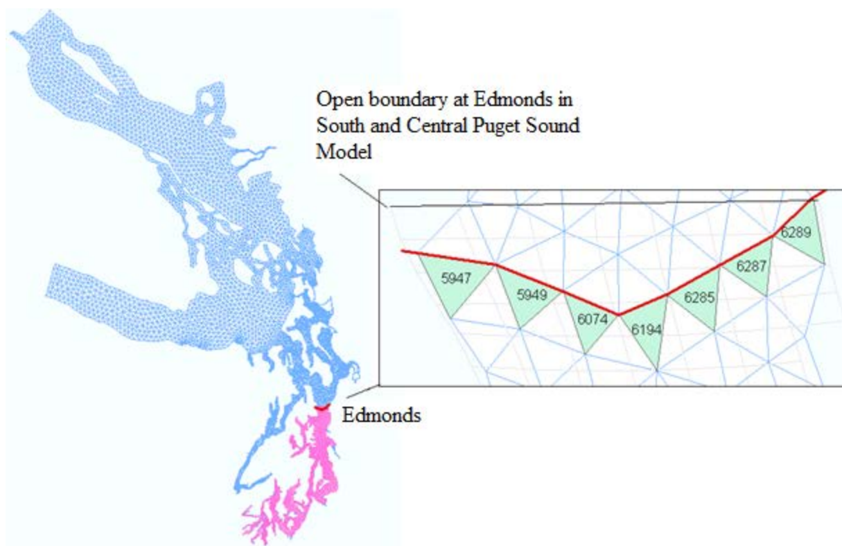
Figure E-1. Salish Sea model grid domain showing location of Edmonds open boundary for the South and Central Puget Sound model.
