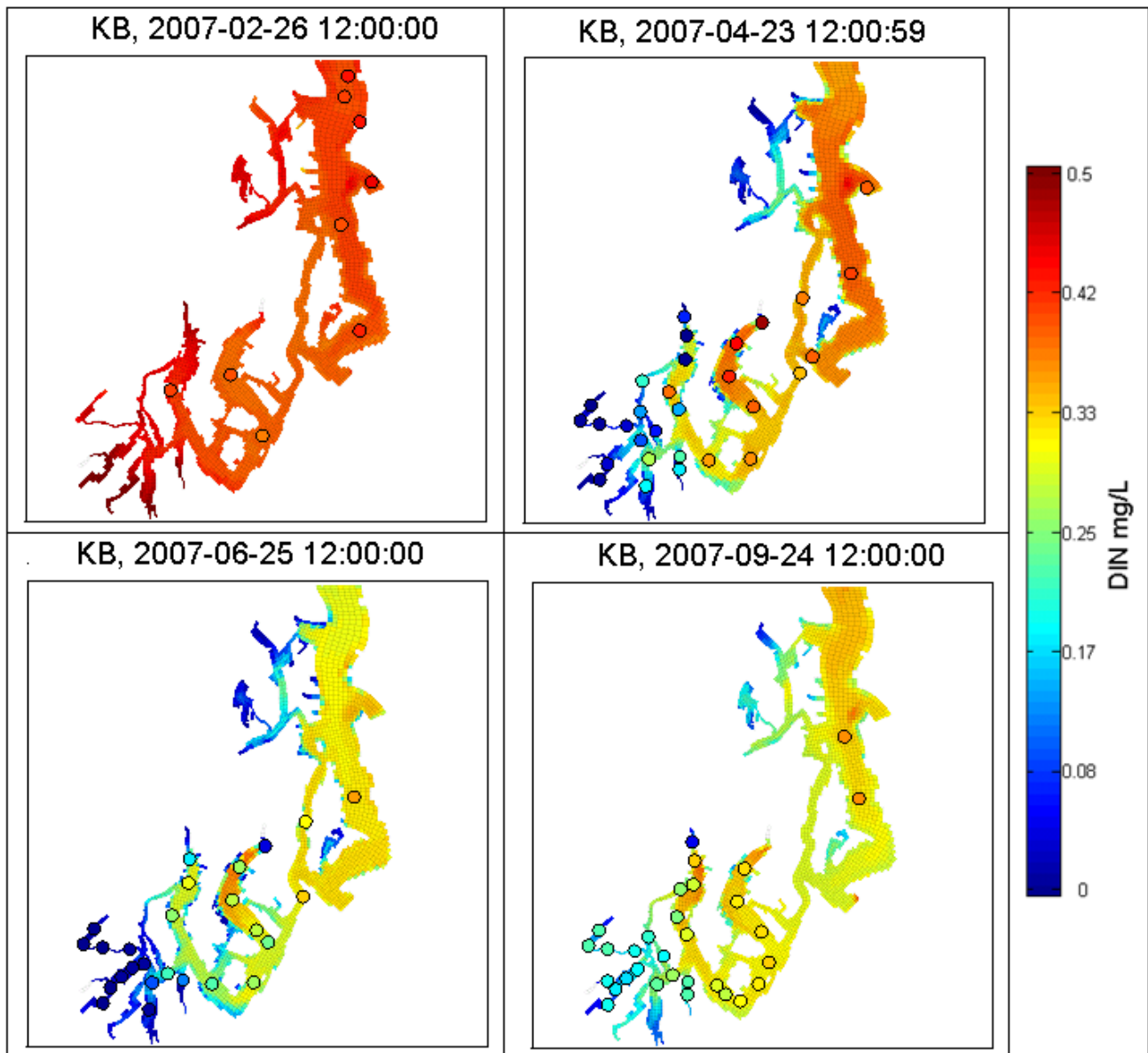
Figure 39. Spatial patterns for DIN in the bottom (KB) layer during different times of the year (2007).
