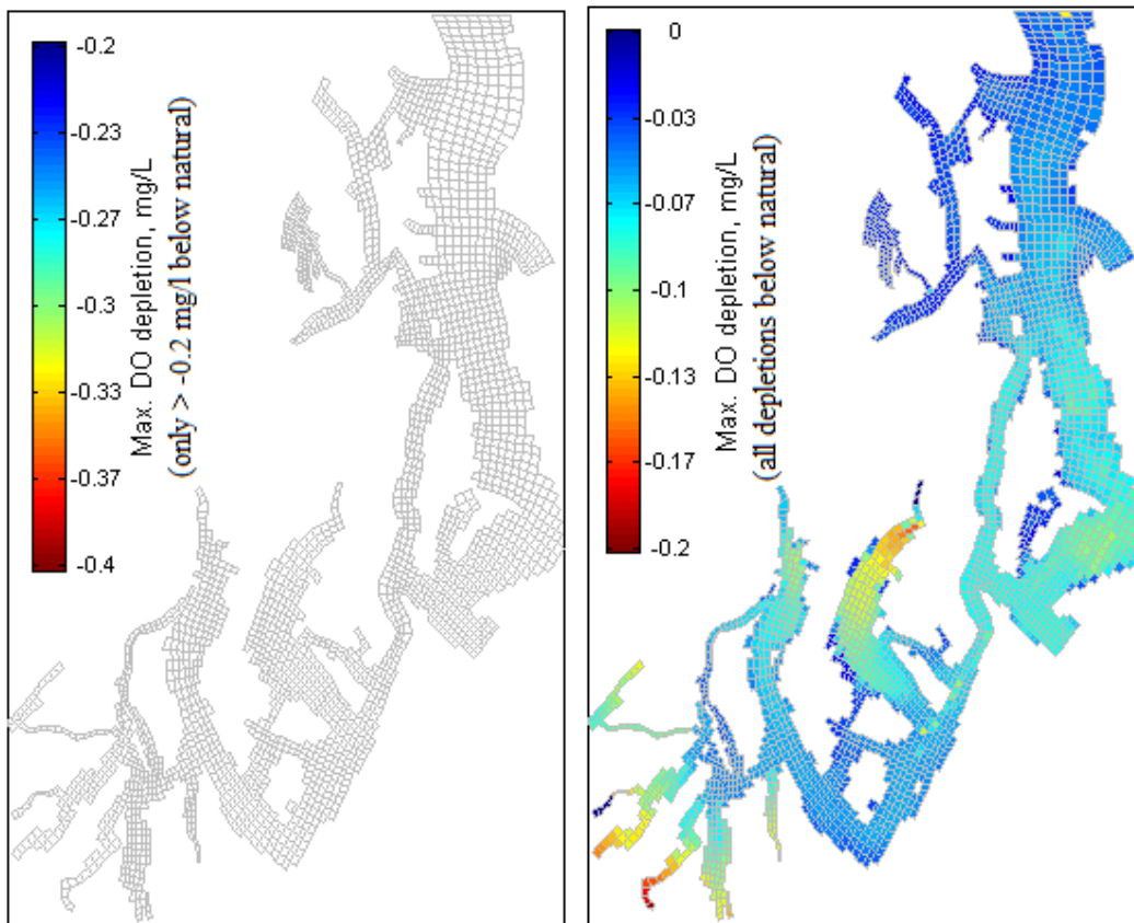
Figure 77. Regions of DO violations with external anthropogenic sources present at the Edmonds open boundary under natural conditions.
