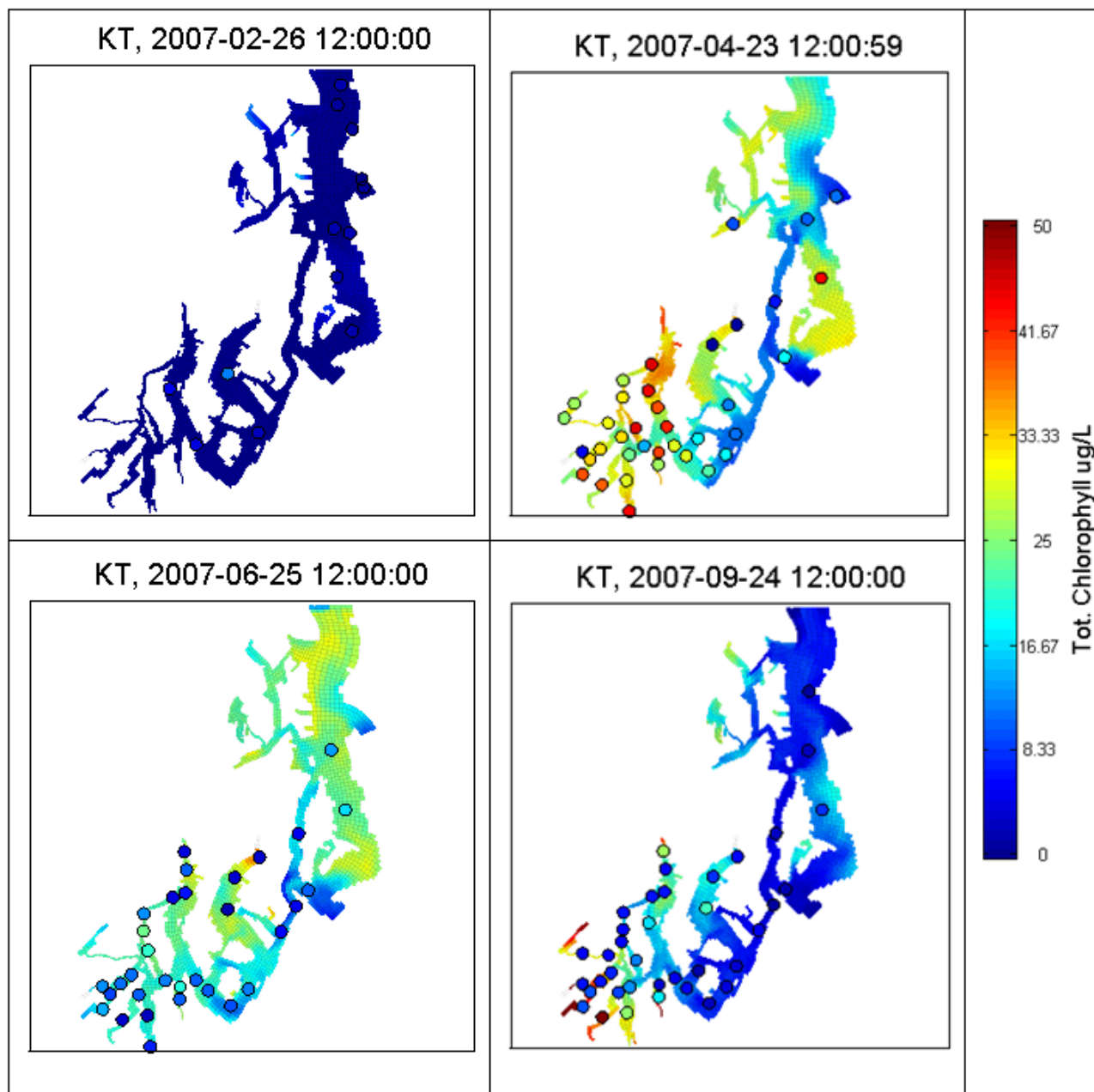
Figure 40. Spatial patterns for total chlorophyll in the surface (KT) layer during different times of the year (2007).
