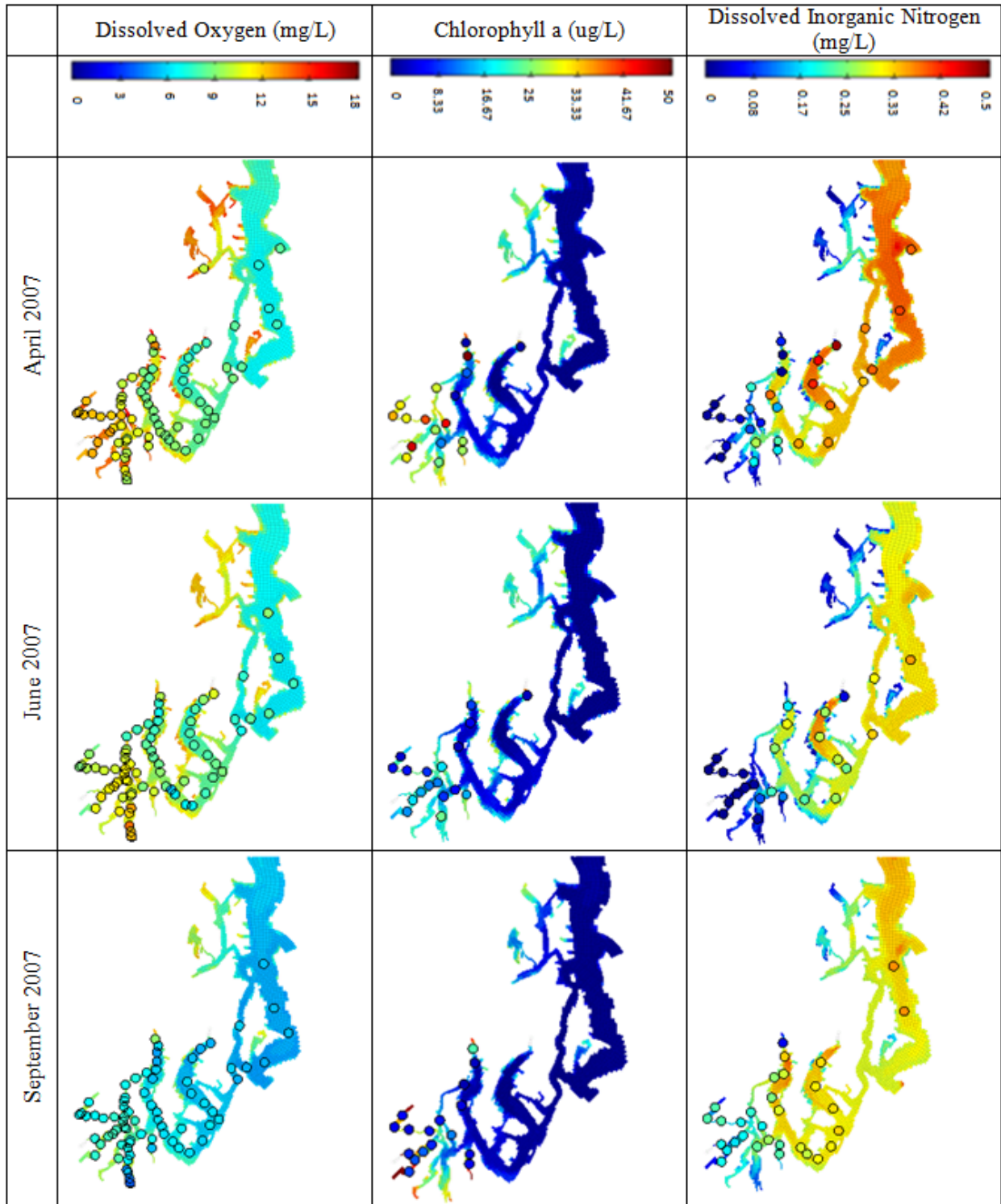
Figure 71. Predicted and observed bottom-layer DO, chlorophyll a, and DIN.
