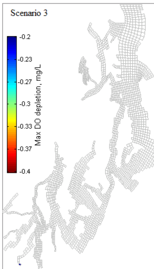
Figure 50. Regions of DO violations due to human sources within watersheds only. Point sources to marine waters have been turned off, external anthropogenic sources at Edmonds open boundary are still present.
