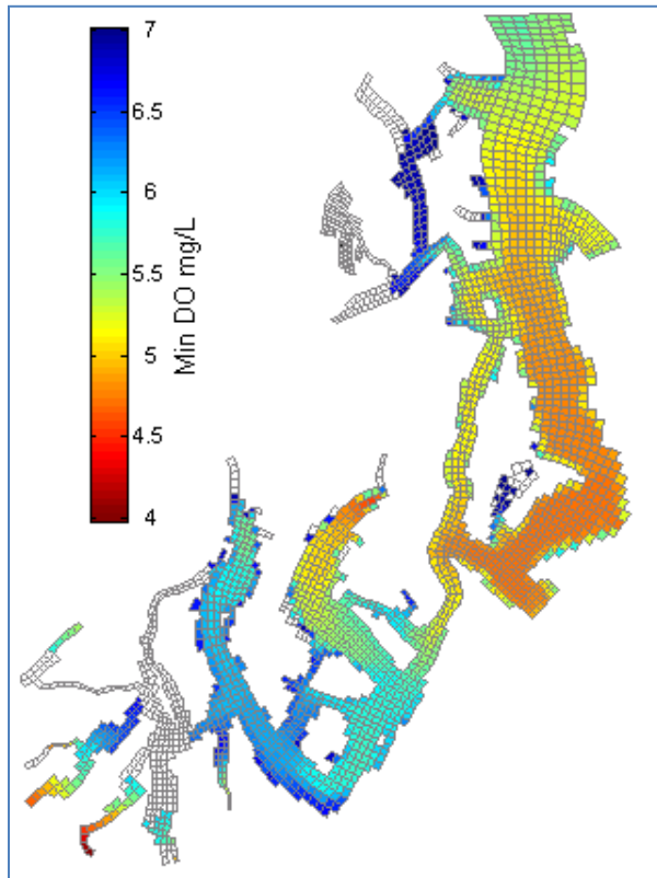
Figure 72. Annual minimum DO concentrations under natural conditions predicted by the model where they are lower than the numeric criteria in the water quality standards.
