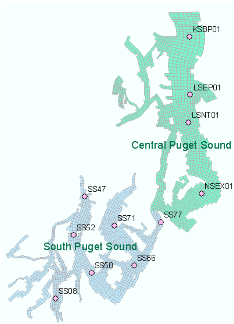
Figure 20. Selected stations in the model domain for time-series model output for water quality calibration.
