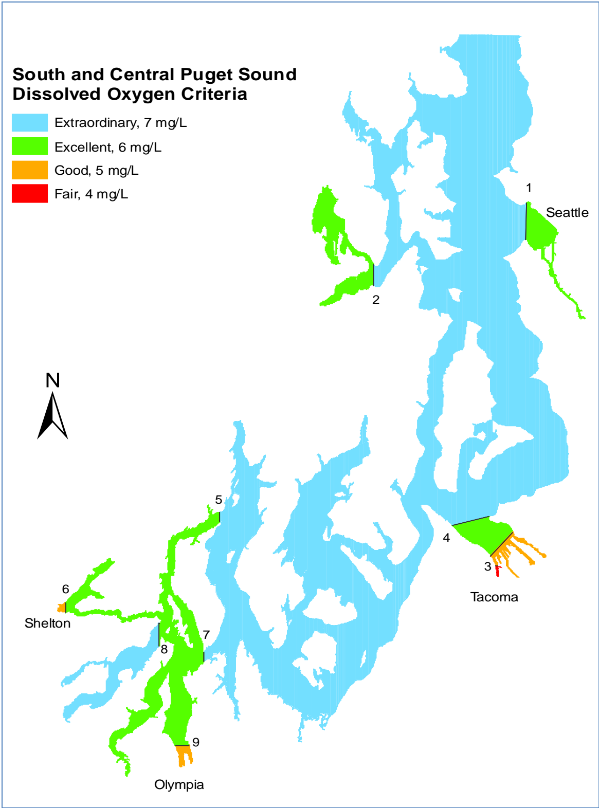
Figure 6. Marine DO standards in South and Central Puget Sound.
