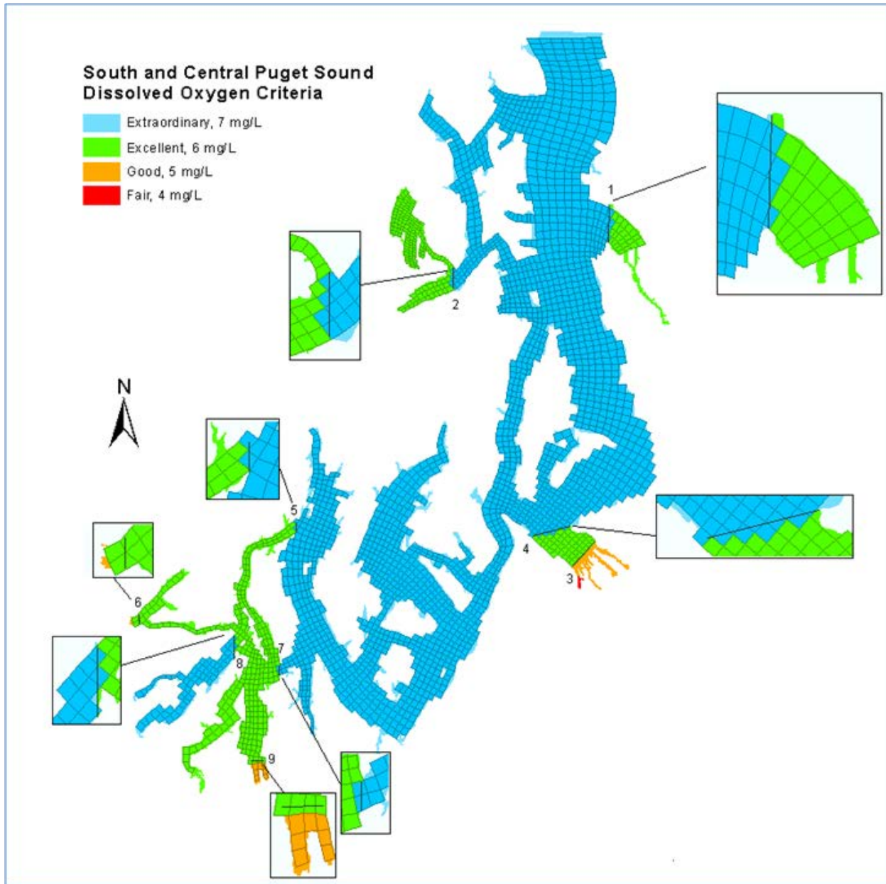
Figure 7. DO standards delineations applied to South and Central Puget Sound model grid.
