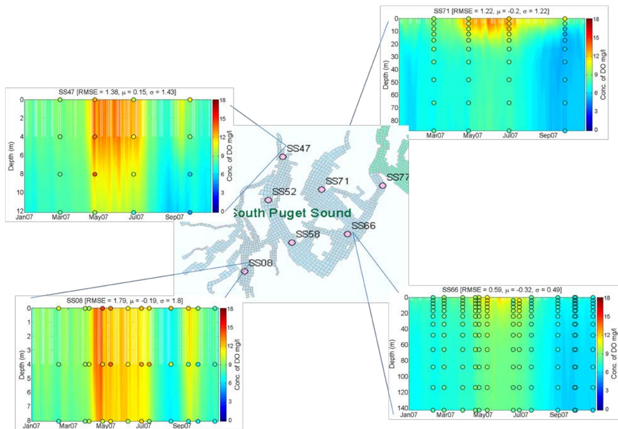
Figure 64. Predicted DO depth-time plots for key stations in South Puget Sound. Observation data are indicated with circles.
