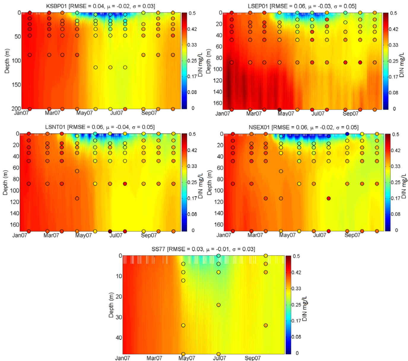
Figure 23. Time-depth contour plots of predicted and observed DIN at Central Puget Sound calibration stations.
