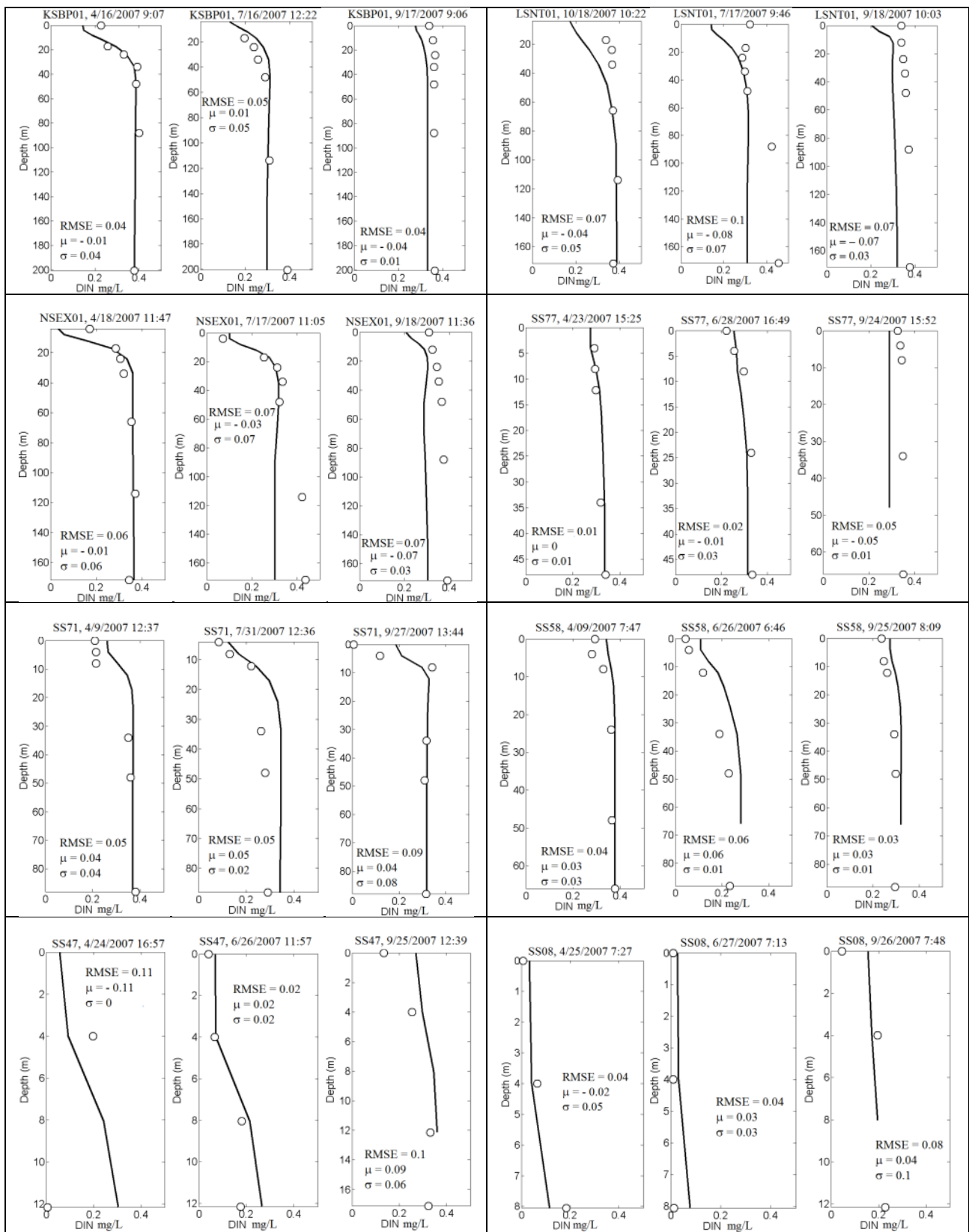
Figure 32. DIN profiles at selected stations in South and Central Puget Sound for spring, summer, and fall.
