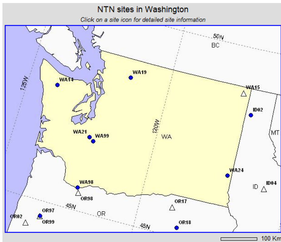
Figure 13. Location of NADP stations in Washington State used for atmospheric deposition load estimates.
