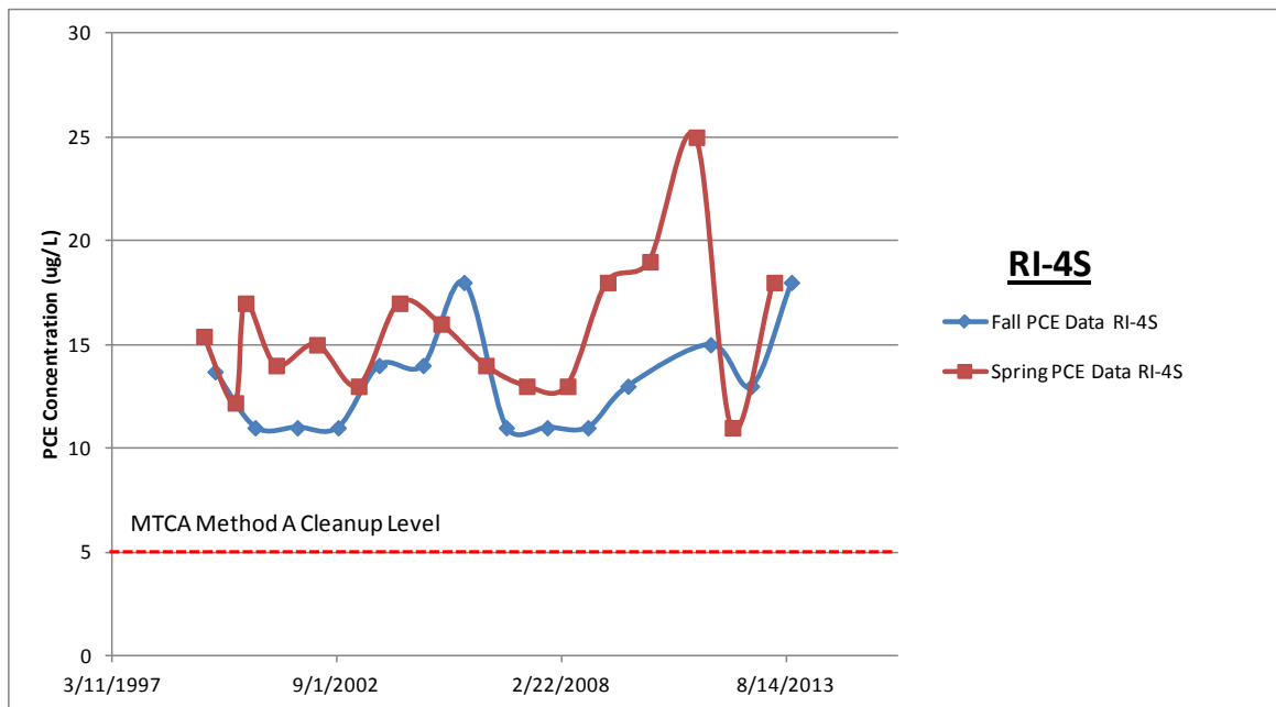
Figure 42. YRRA Remedial Investigation Well RI-4S PCE Results, June 1999 to October 2013.
