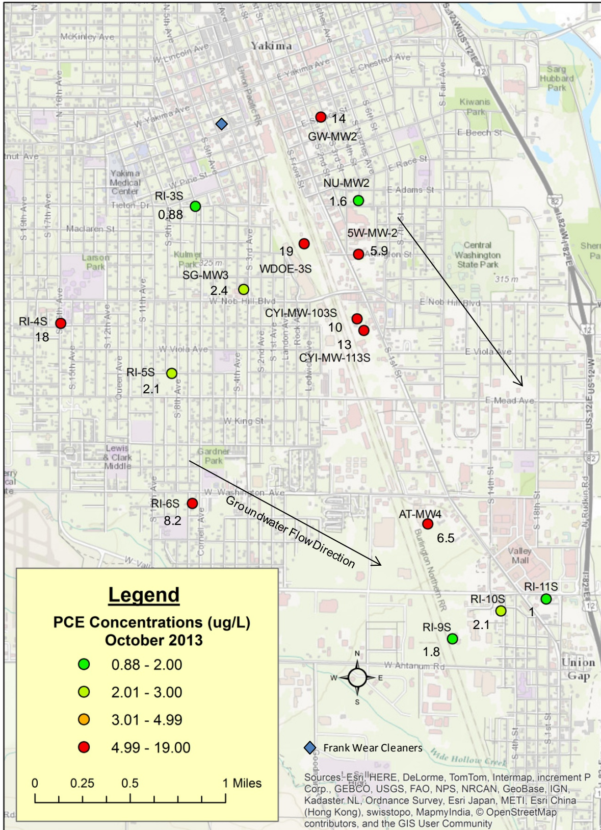
Figure 12. Shallow Zone PCE Concentrations (ug/L), October 2013.
