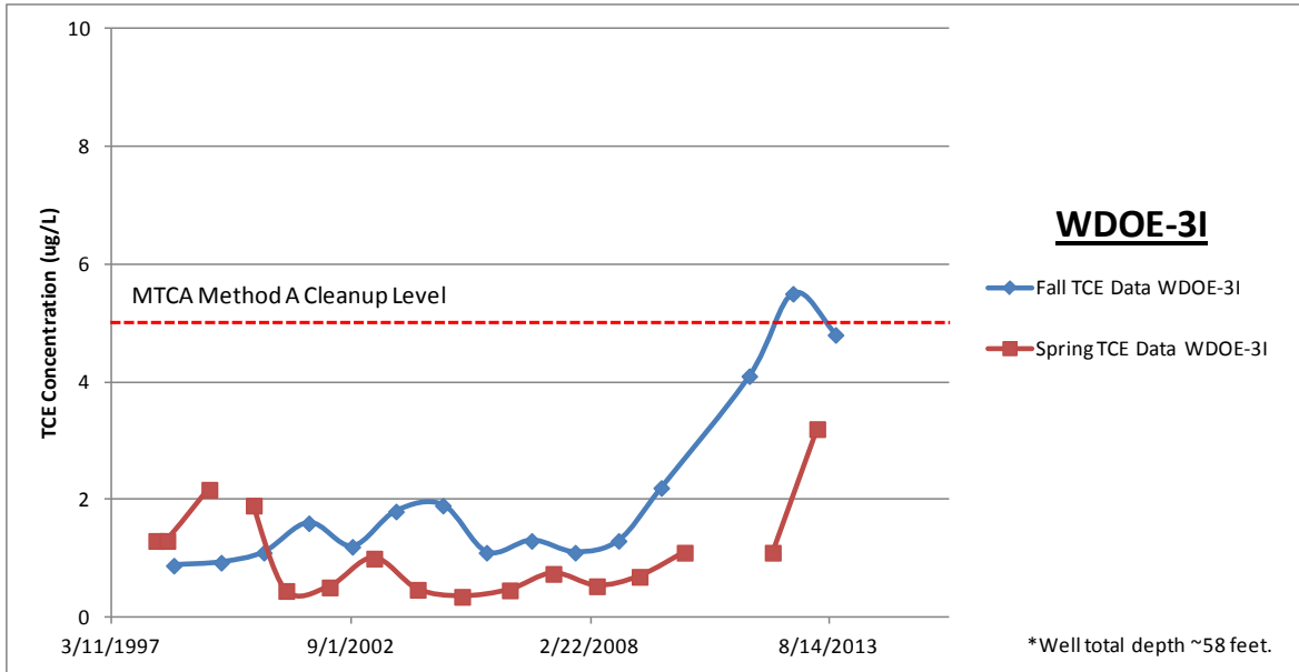
Figure 25. Washington Central Railroad Roundhouse, Well WDOE-3I TCE Results (ug/L), June 1999 to October 2013.
