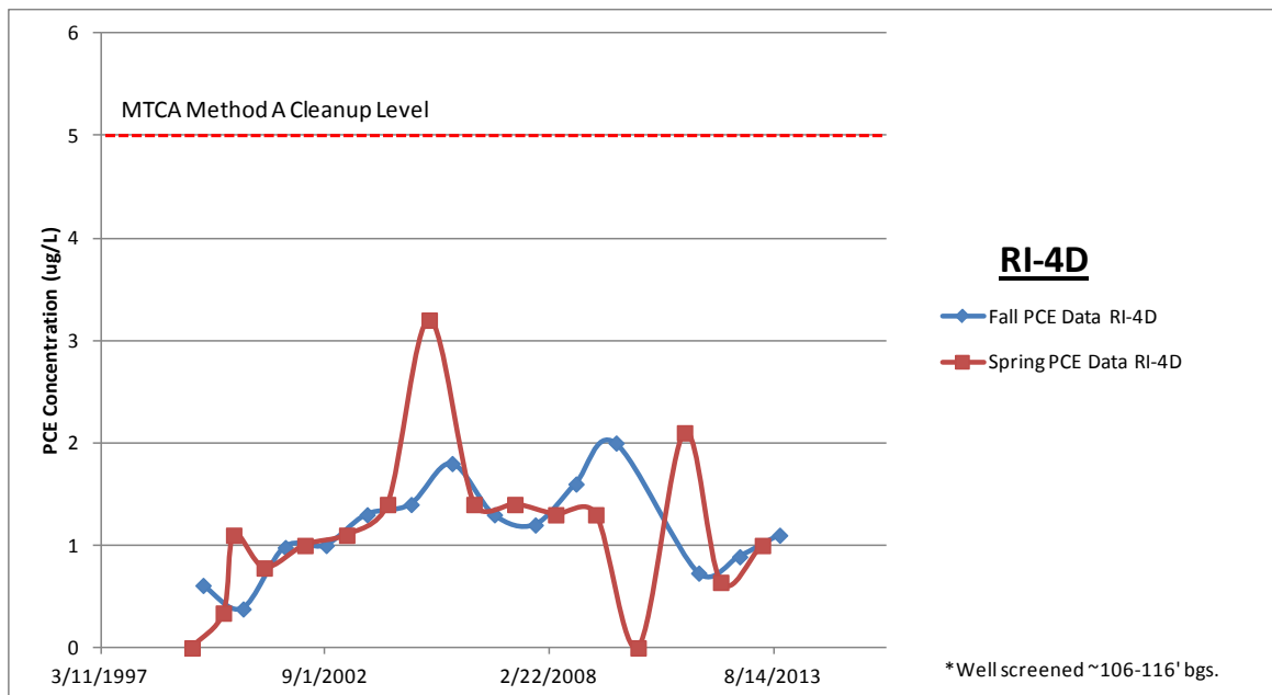
Figure 43. YRRA Remedial Investigation Well RI-4D PCE Results, June 1999 to October 2013.
