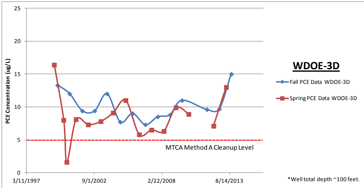
Figure 24. Washington Central Railroad Roundhouse, Well WDOE-3D PCE Results (ug/L), June 1999 to October 2013.
