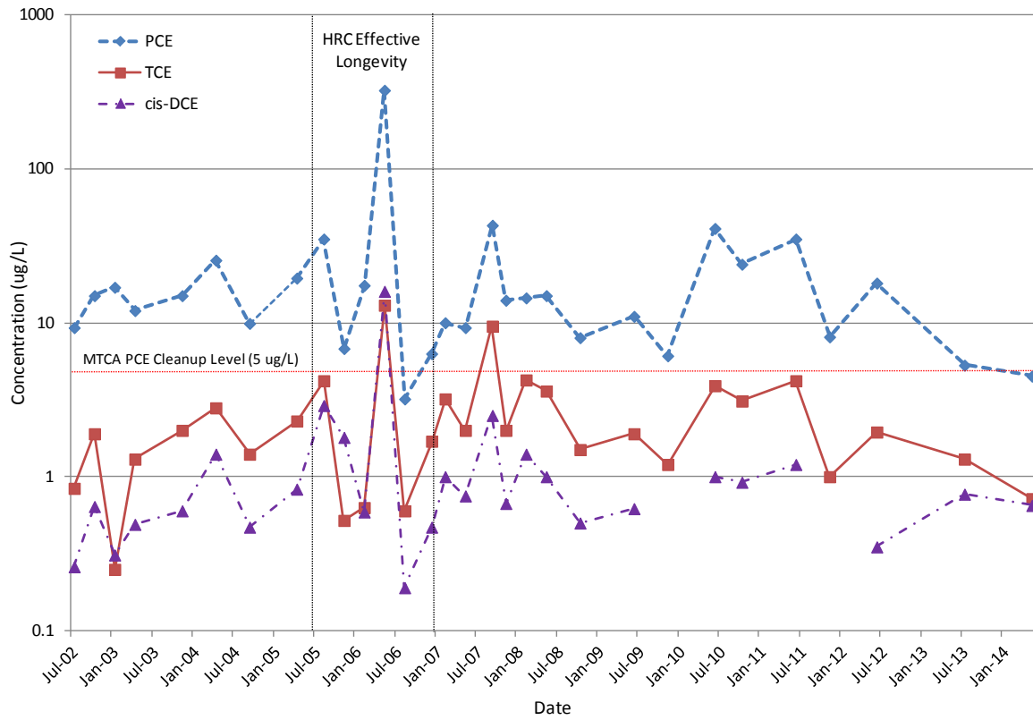
Figure 2. PCE, TCE, and cis-DCE Concentrations (ug/L – log scale) in Well 4W, July 2002 through May 2014.
