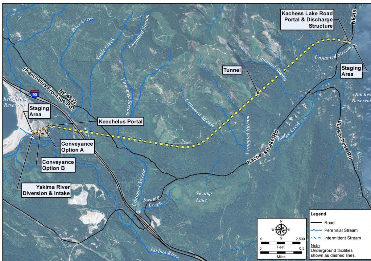
Figure 2-13. KKC North Tunnel Alignment Overview
