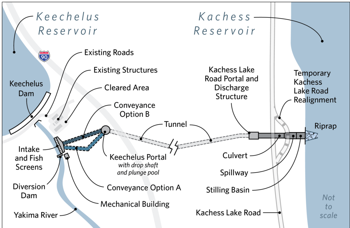
Figure 2-14. KKC North Tunnel Alignment Conceptual Site Plan
