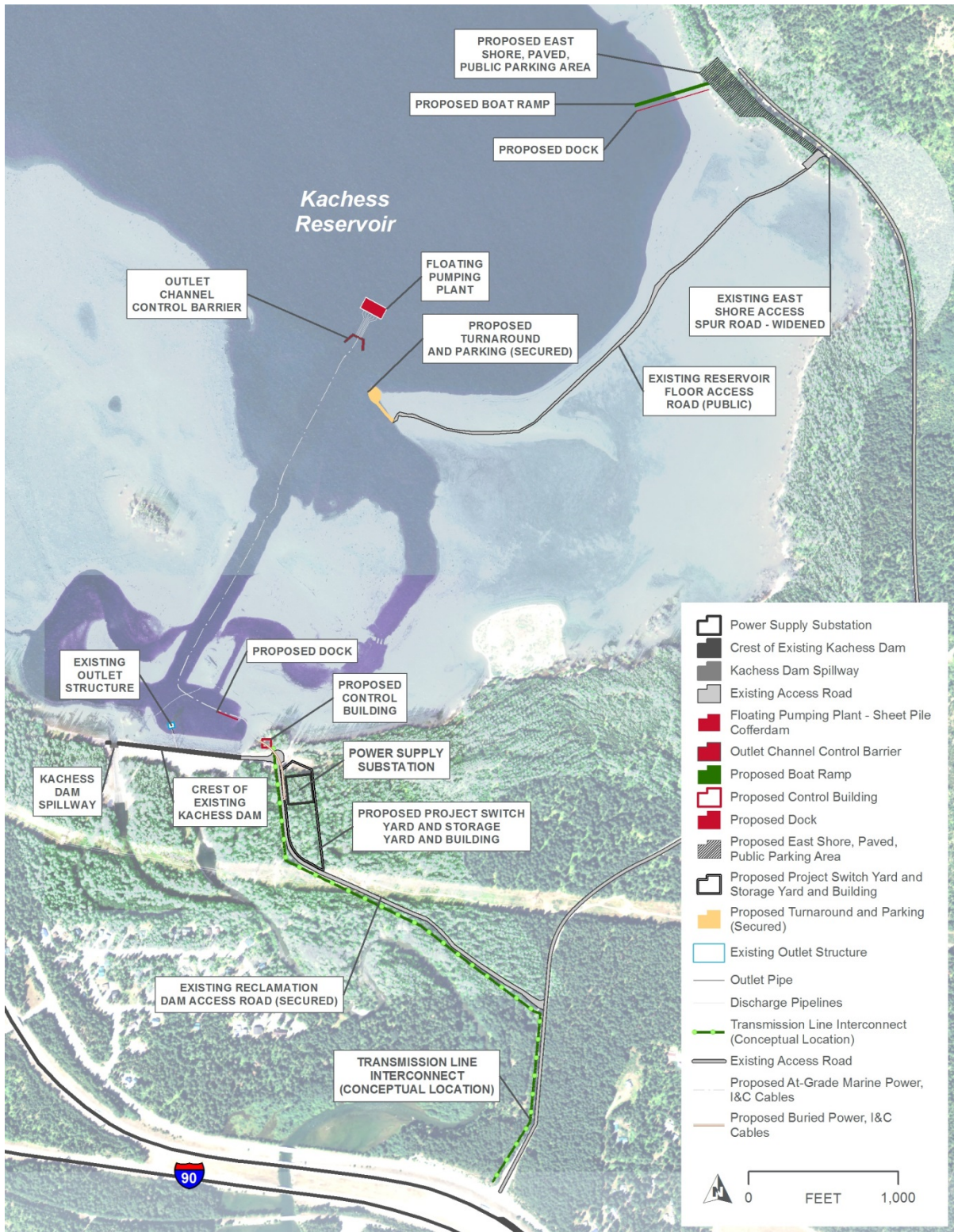
Figure 2-8. Alternative 4 – KDRPP Floating Pumping Plant Overview
