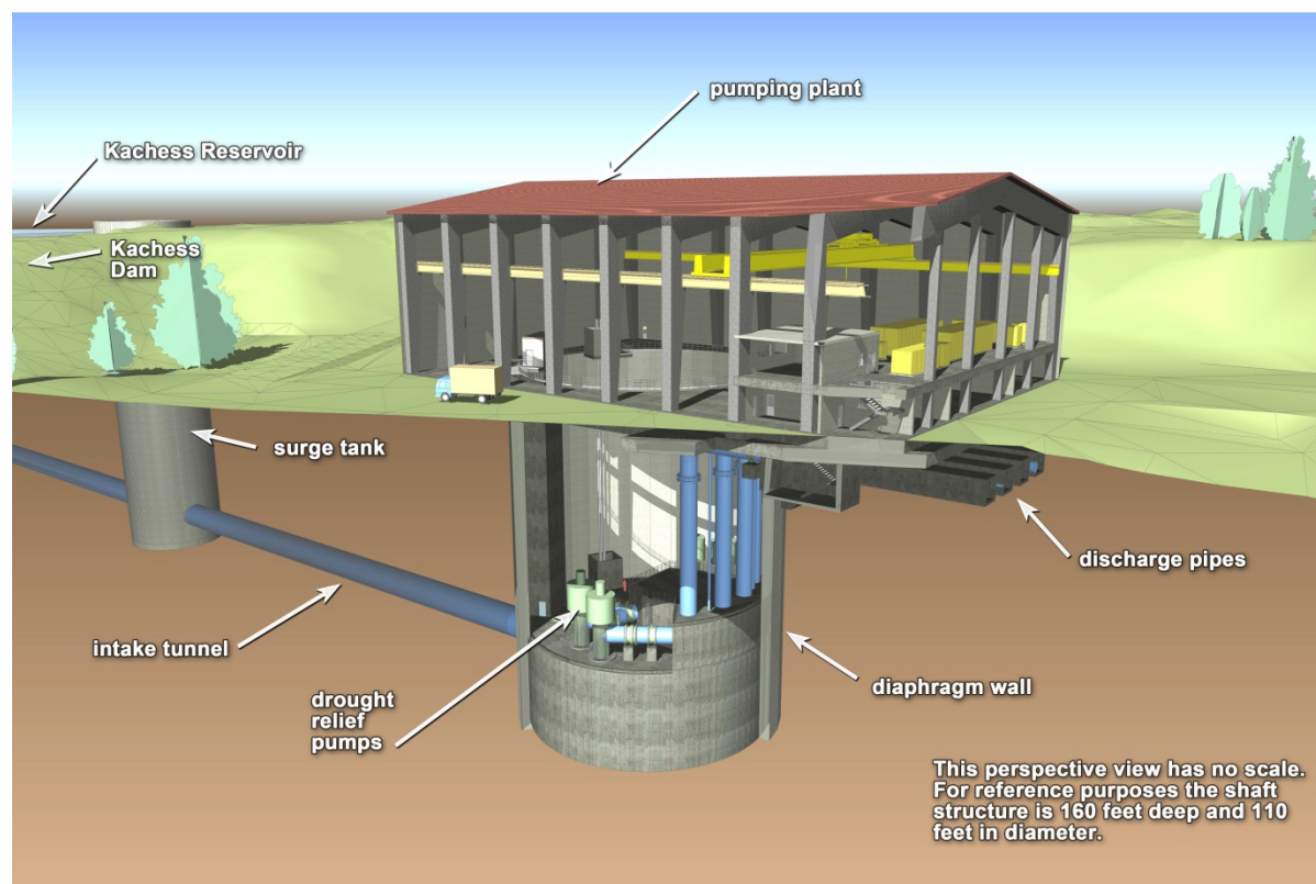
Figure 2-7. KDRPP South Pumping Plant Conceptual Rendering
