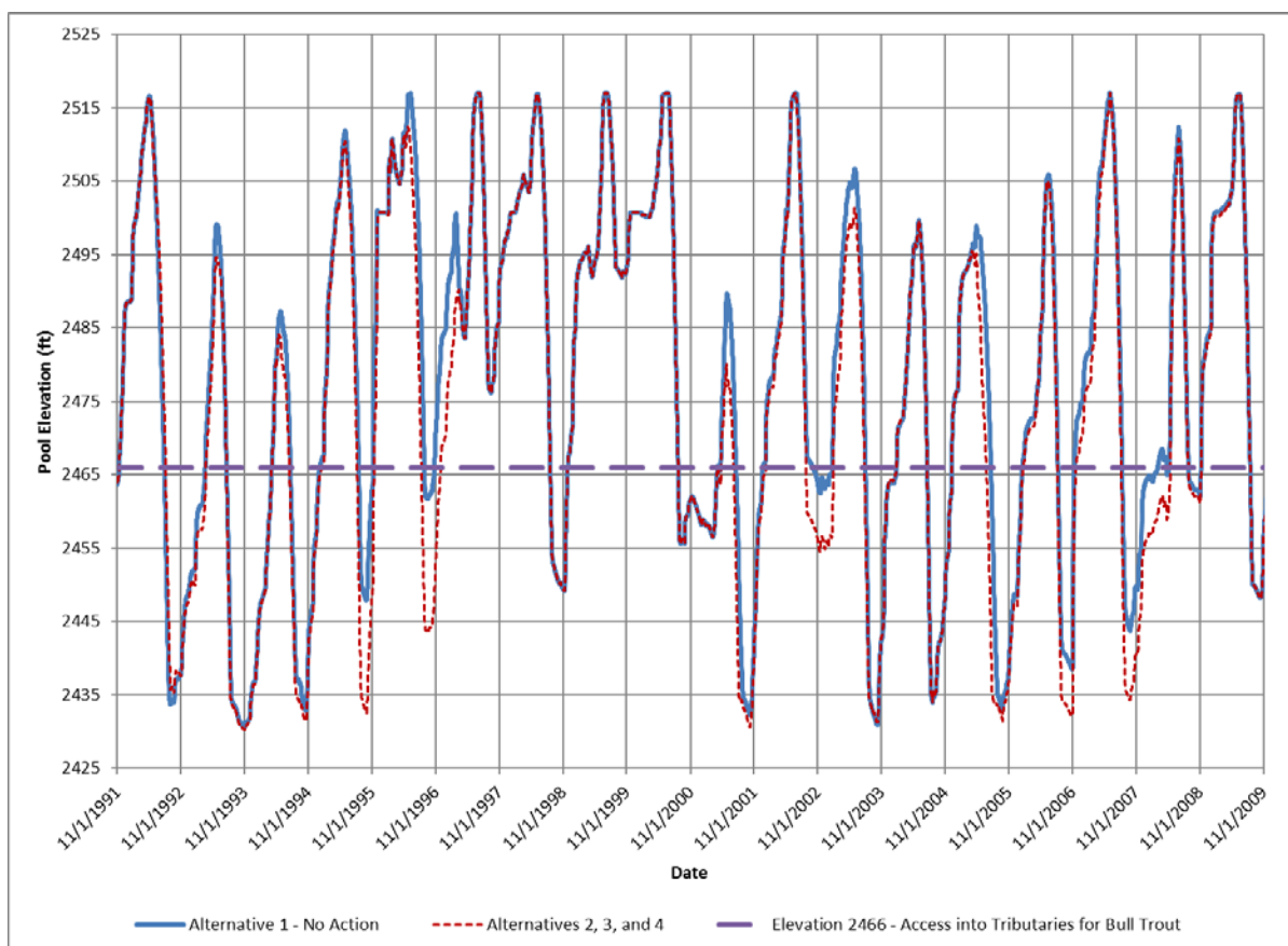
Figure 4-4. Change in Keechelus Reservoir Pool Elevation under Alternative 2 – KDRPP East Shore Pumping Plant
