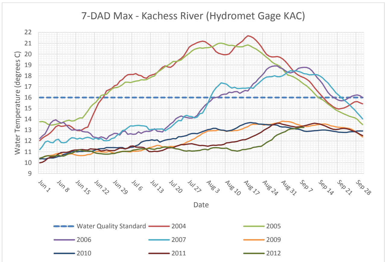
Figure 3-14. Kachess River 7-Day Average Daily Maximum Temperature
