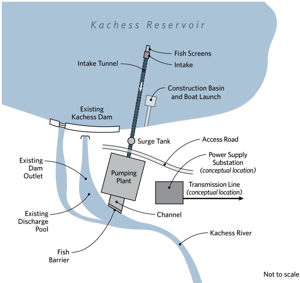
Figure 2-6. KDRPP South Pumping Plant Conceptual Site Plan
