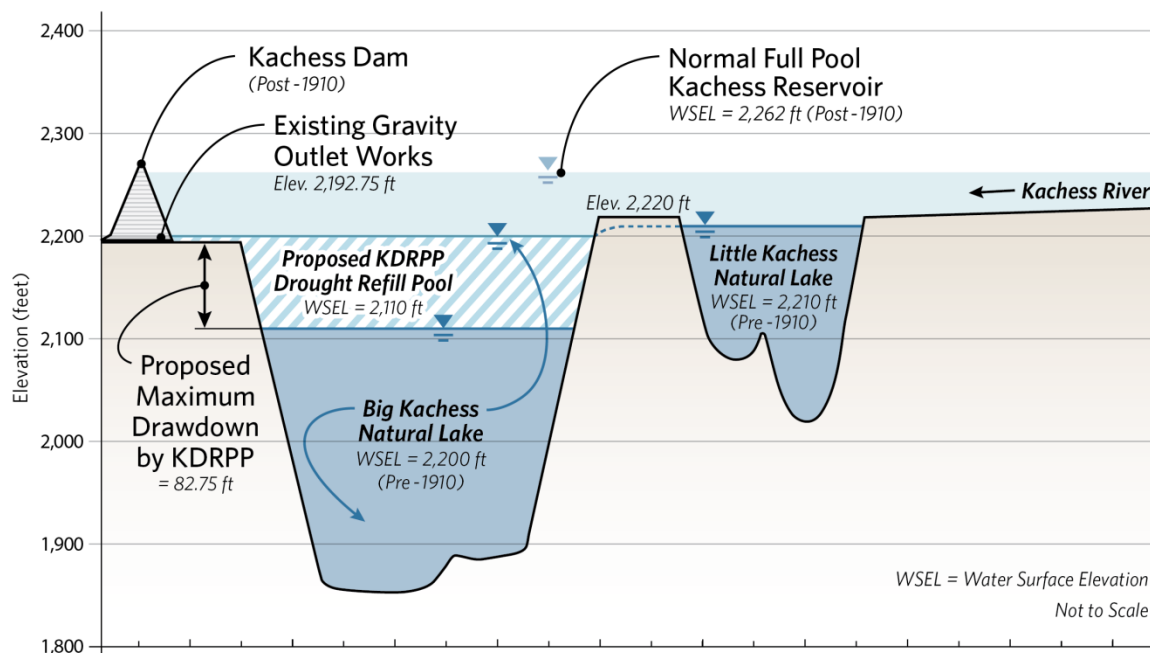
Figure 4-1. Kachess Hydraulic Profile
