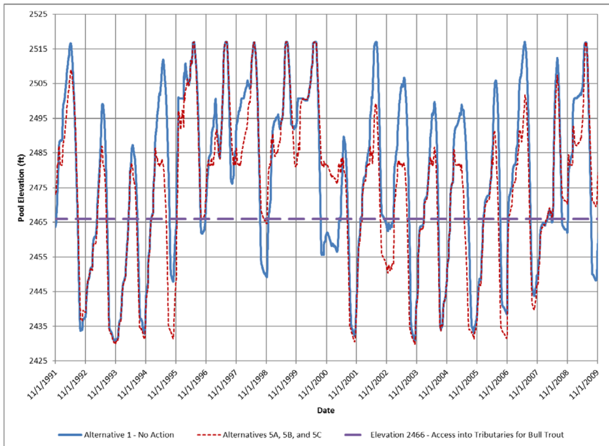
Figure 4-6. Keechelus Reservoir Pool Elevation under Alternative 5A – KDRPP East Shore Pumping Plant with KKC North Tunnel Alignment
