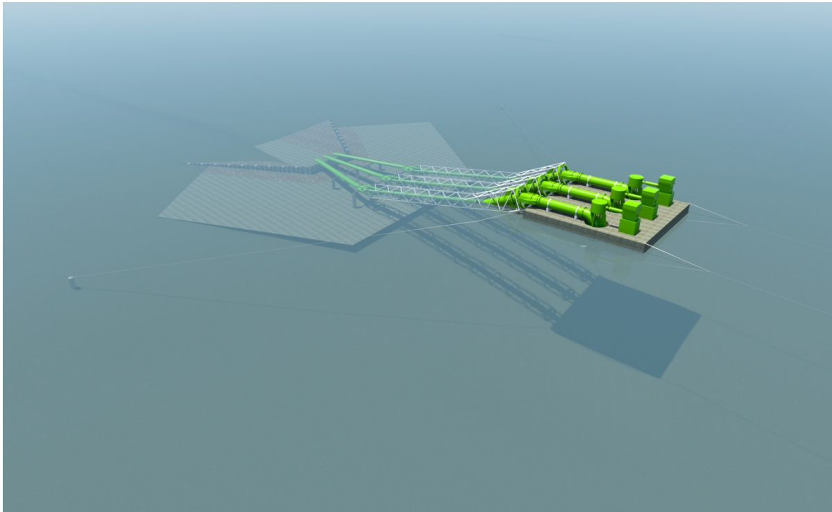
Figure 2-10. Alternative 4 – Floating Pumping Plant Conceptual Rendering – Maximum Pool
