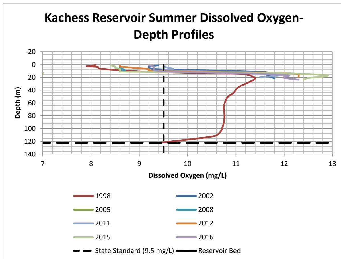
Figure 3-13. Kachess Reservoir Summer Dissolved Oxygen versus Depth Profile
