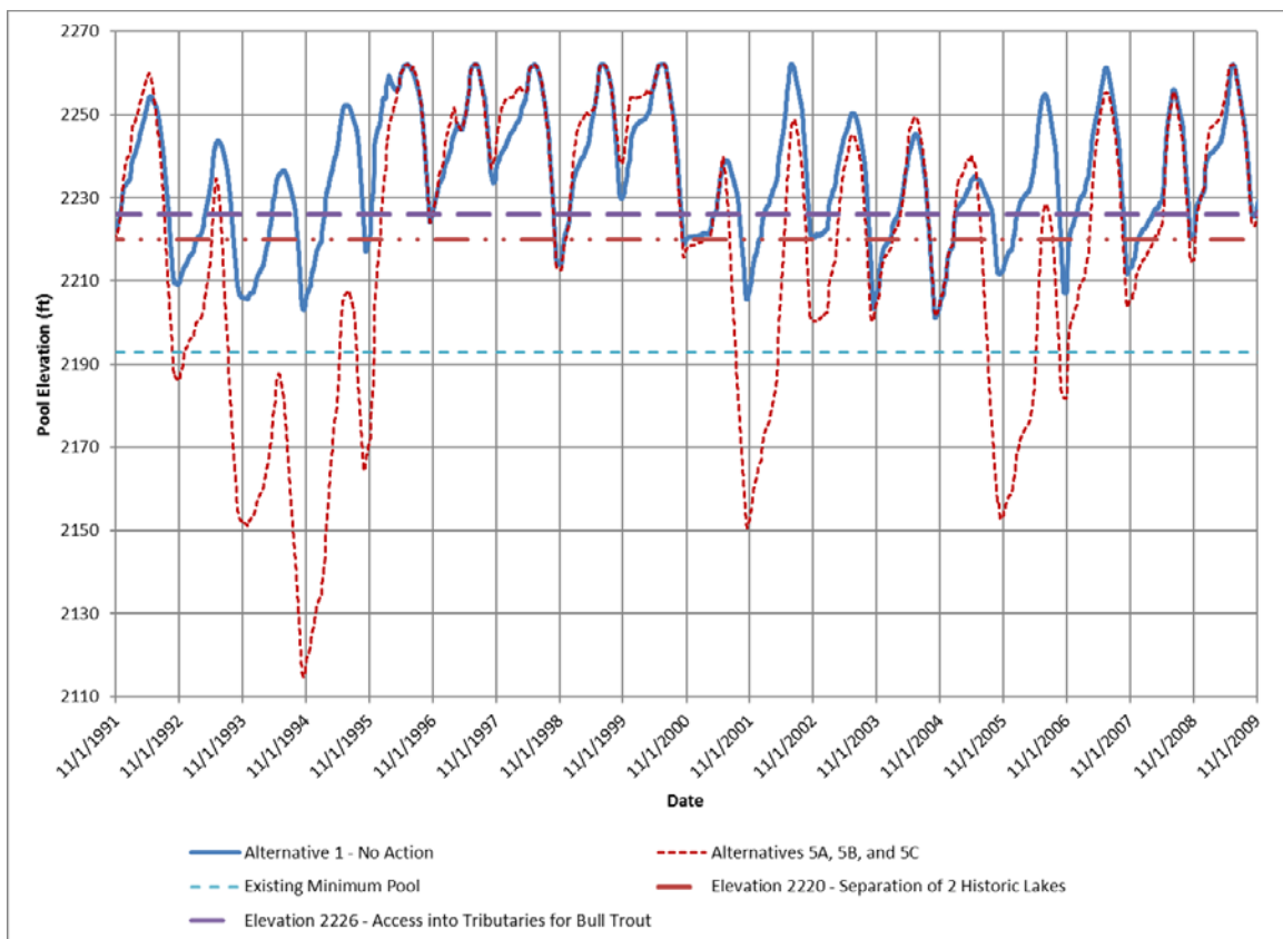
Figure 4-5. Kachess Reservoir Pool Elevation under Alternative 5A – KDRPP East Shore Pumping Plant with KKC North Tunnel Alignment
