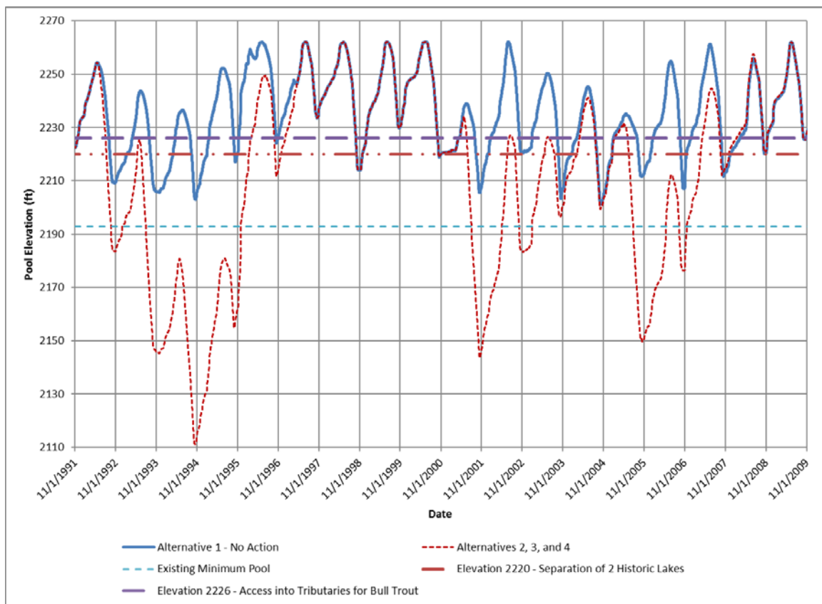
Figure 4-3. Kachess Reservoir Pool Elevations under Alternative 2 – KDRPP East Shore Pumping Plant
