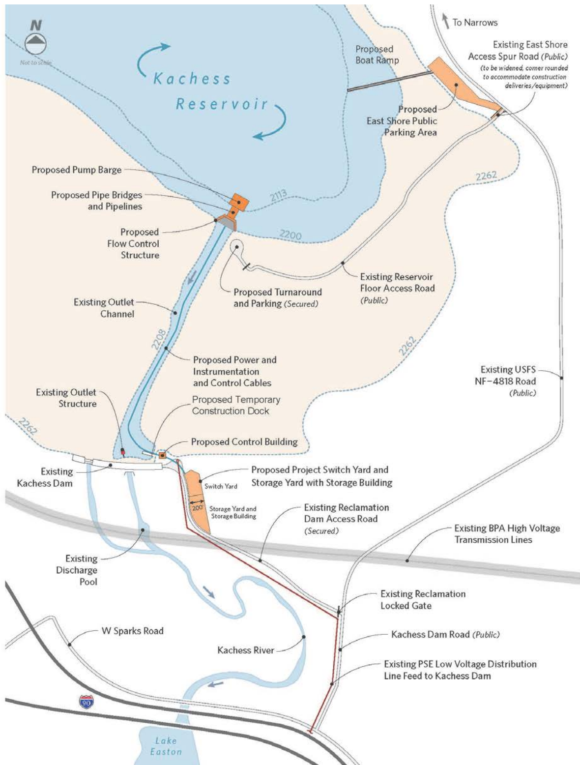
Figure 2-9. Conceptual Site Plan - Alternative 4 – KDRPP Floating Pumping Plant
