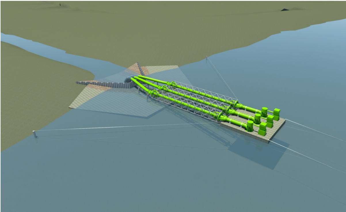
Figure 2-11. Alternative 4 – Floating Pumping Plant Conceptual Rendering – Start of Drought Relief Pumping
