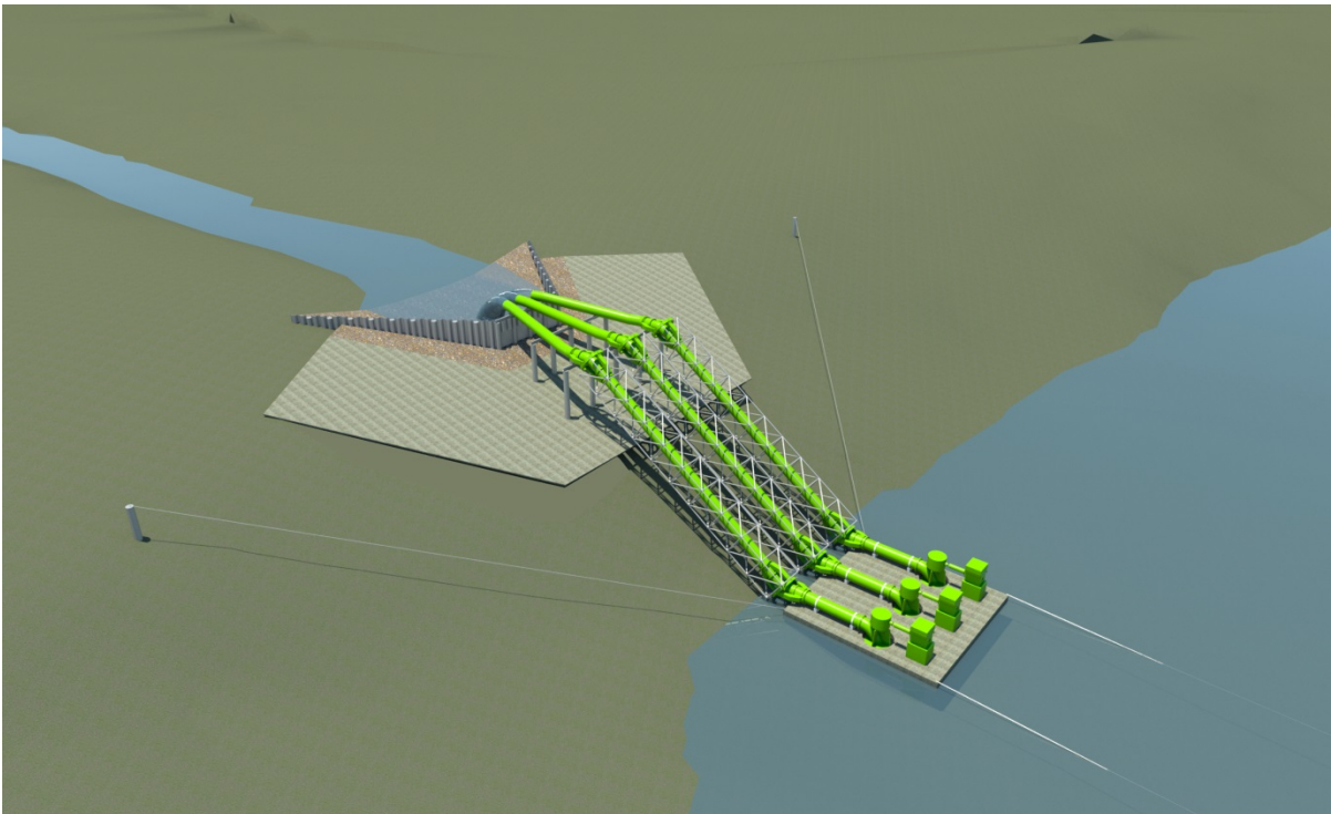
Figure 2-12. Alternative 4 – Floating Pumping Plant Conceptual Rendering – Minimum Drought Relief Pool
