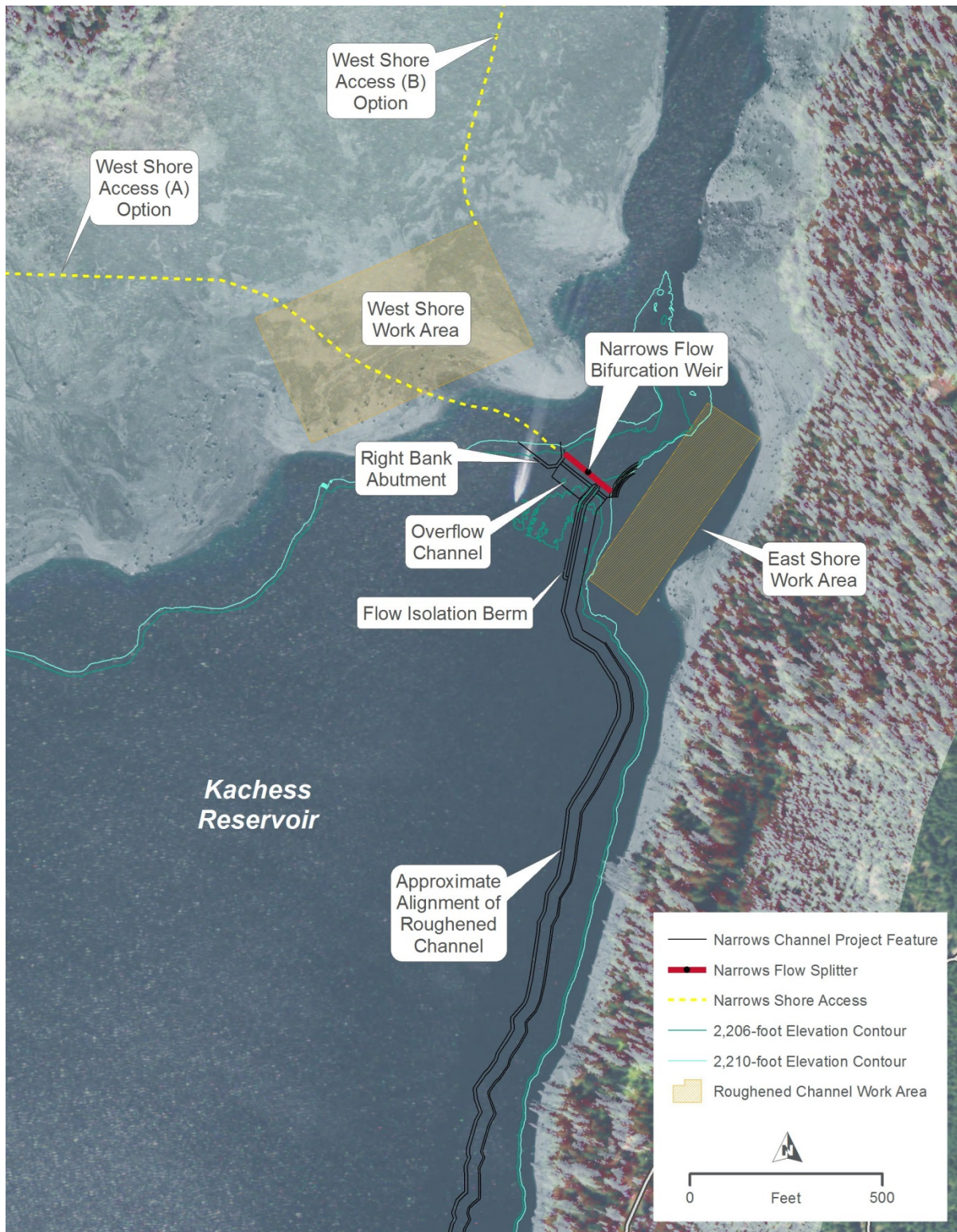
Figure 2-4. Proposed Volitional Bull Trout Passage Improvements at the Kachess Narrows
