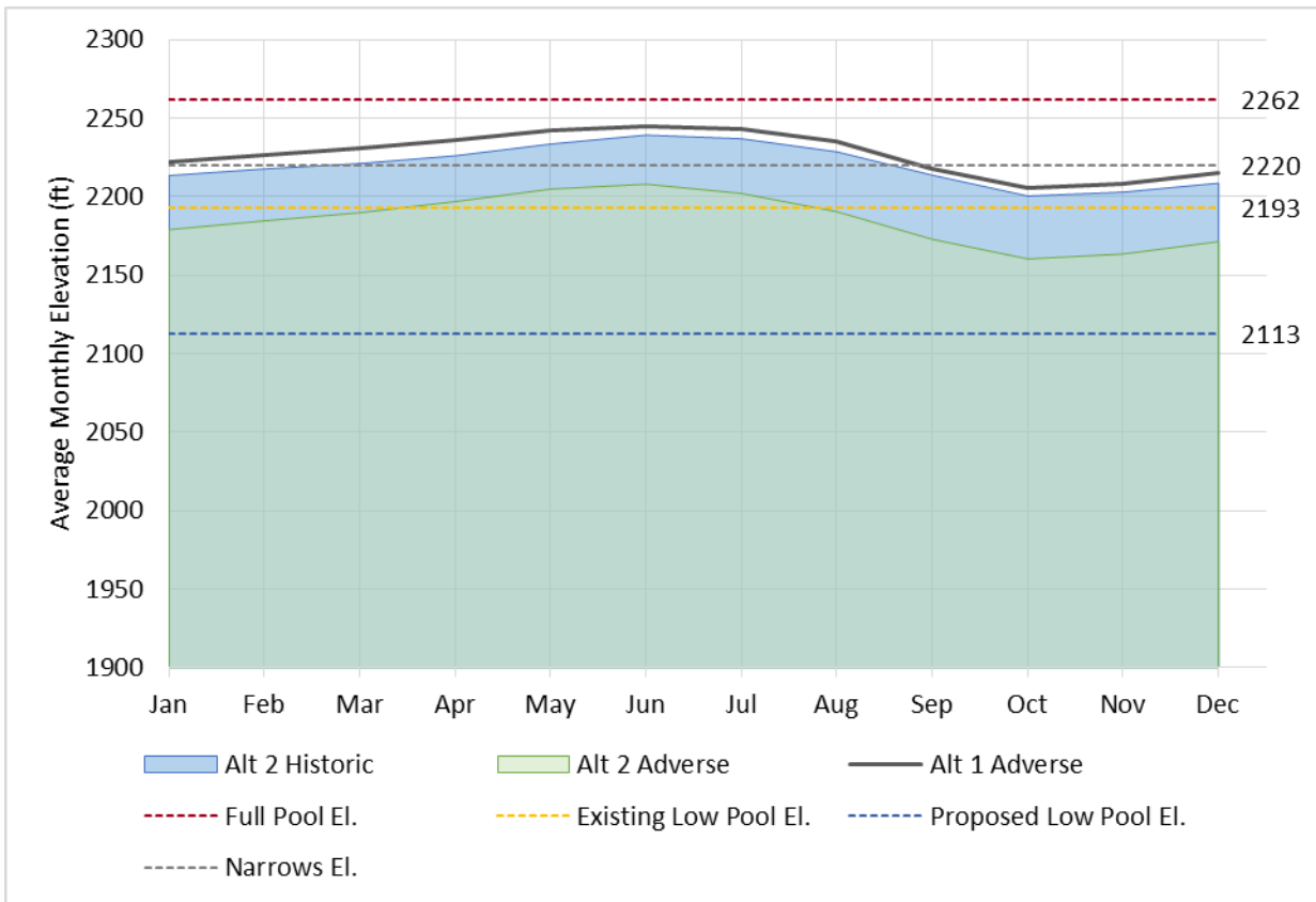
Figure 4-14. Effect of Climate Change on Average Kachess Reservoir Water Surface Elevation – Alternatives 2, 3, and 4
