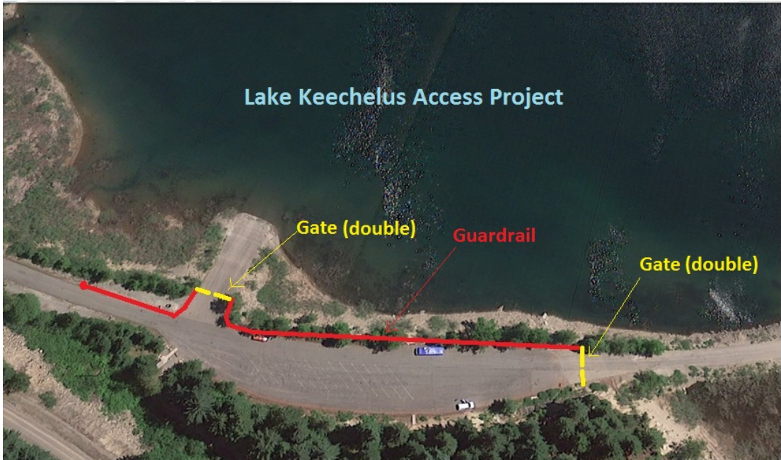
Figure 3-5. Concept design for the Keechelus Reservoir and Lower Gold Creek Access Management project. Two gates (yellow) and approximately 1,900 feet of guardrail (red) would be installed to control reservoir access during low pool conditions.
