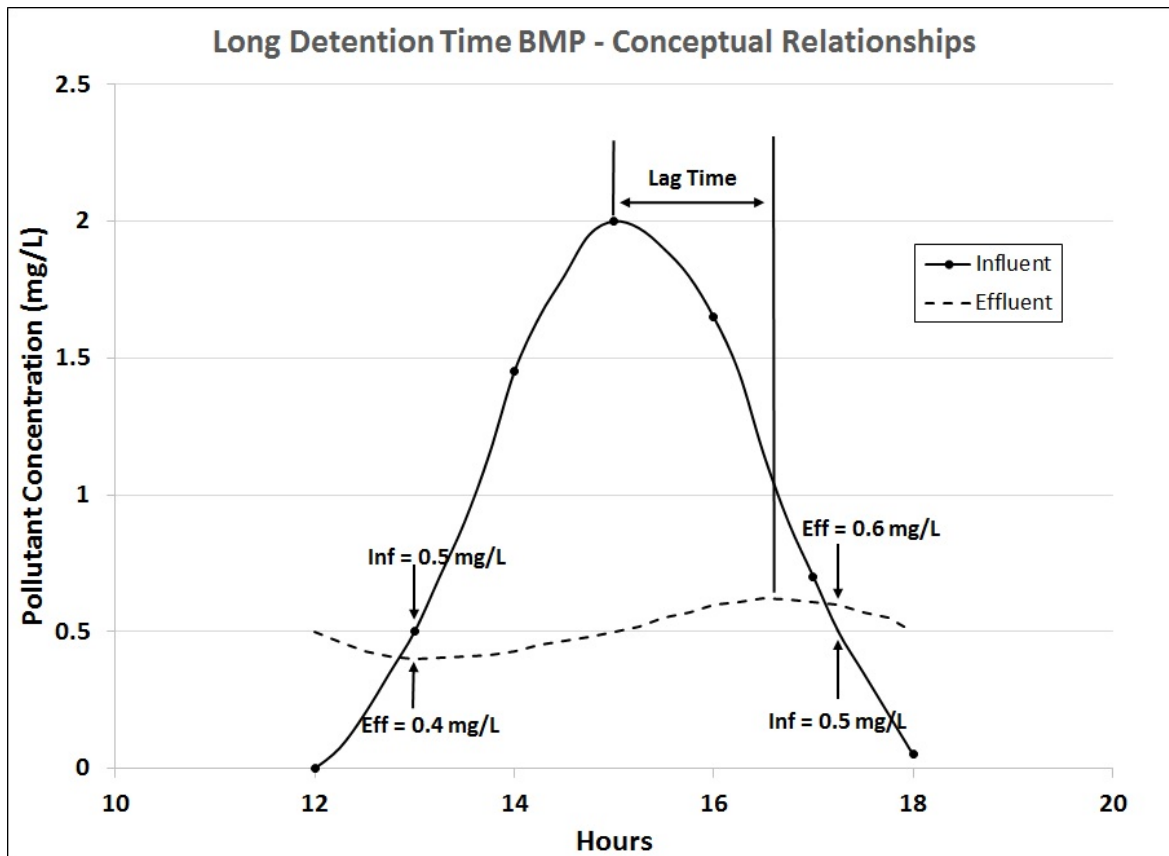
Figure 1 Conceptual Relationships of Influent and Effluent for BMPs with Long Detention Times
