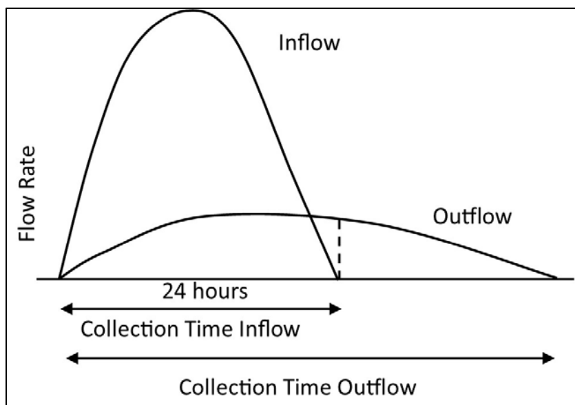
Figure 2. Depiction of Portions of Influent and Effluent Hydrographs for a BMP with a Long Detention Time
