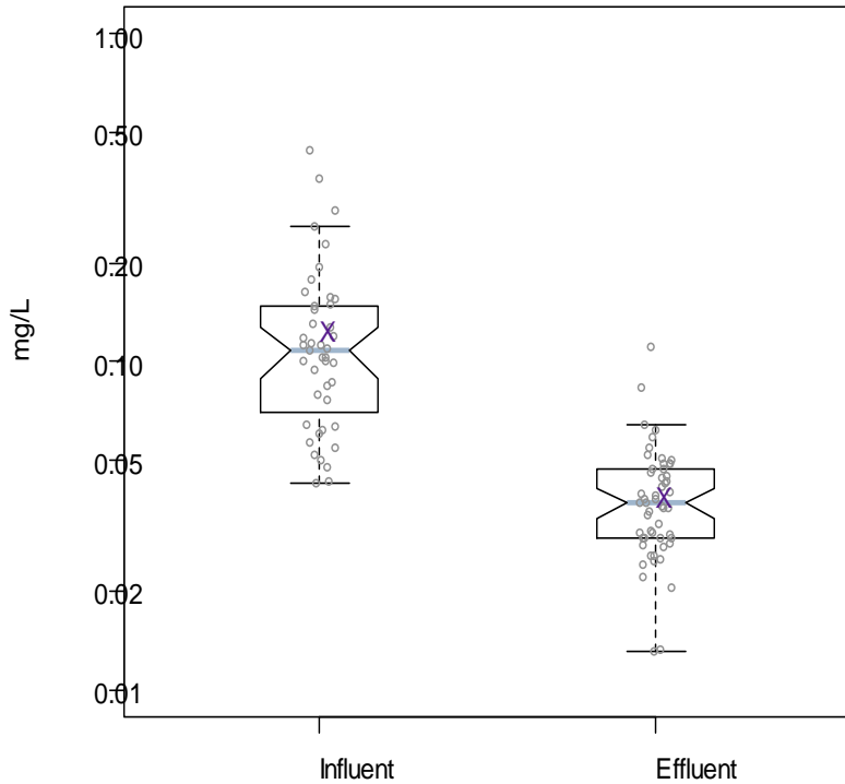
Figure 4. Example Tukey style box plot showing distribution of influent and effluent dissolved copper concentrations
