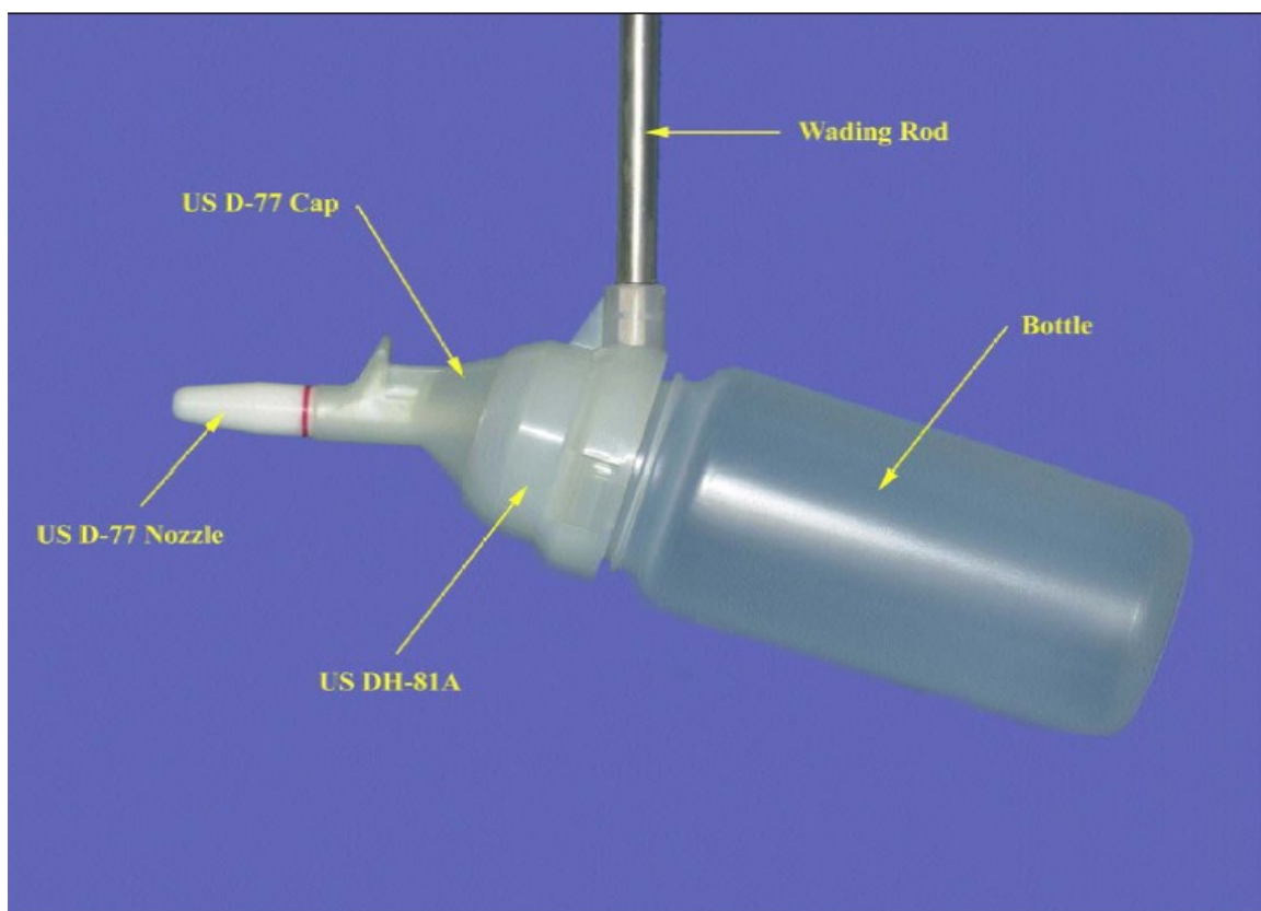
Figure 1. US DH-81 complete assembly.
