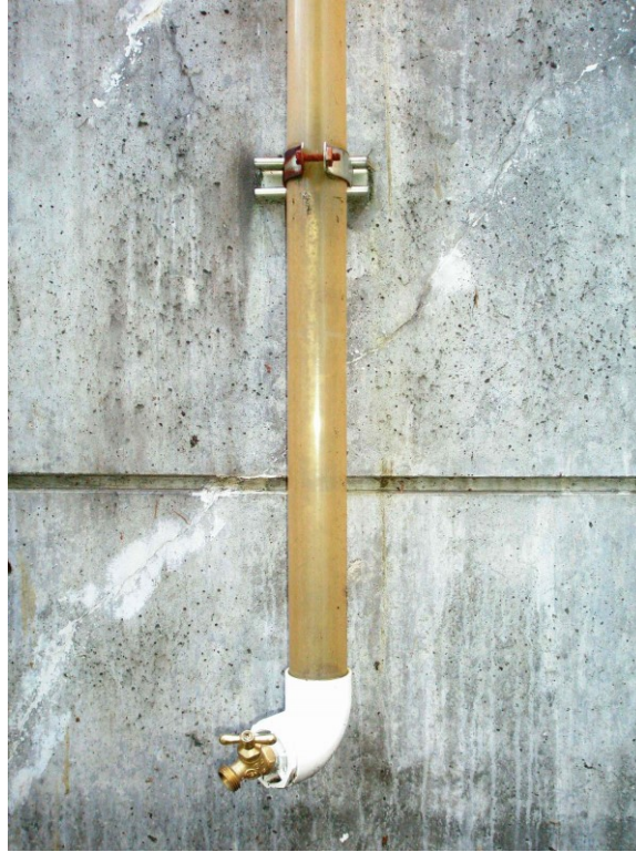
Figure B-1. Bottom portion of EAP’s transducer check stilling tube
