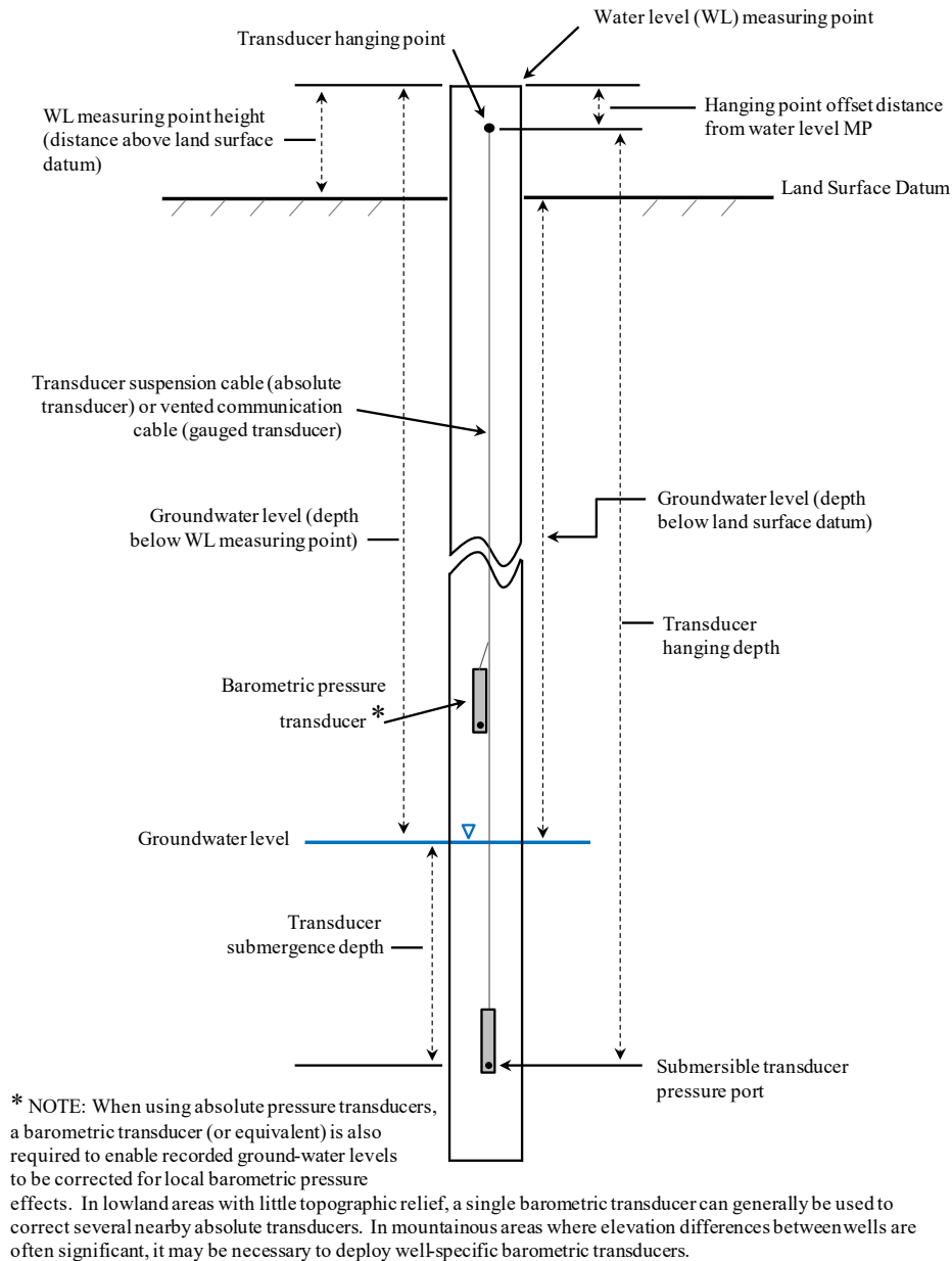
Figure 5 – Schematic of a typical transducer deployment and associated field measurements (Adapted from Freeman et al., 2004).
