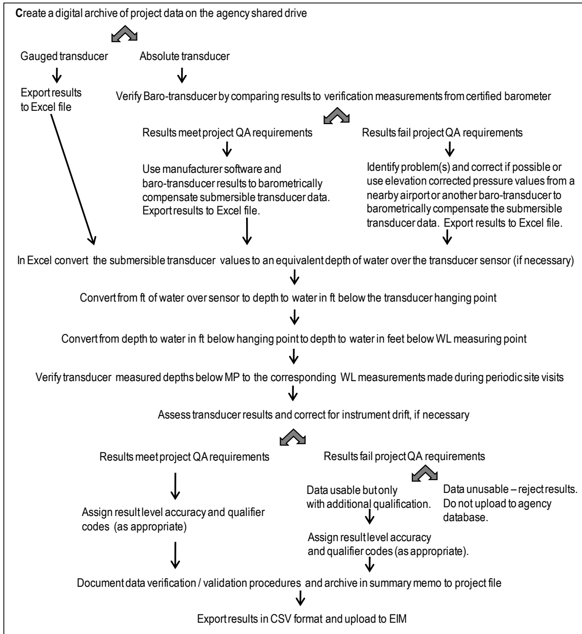
Figure 8 – General data processing steps for transducers
