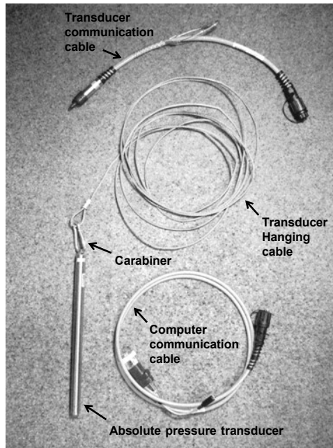
Figure 3 – Typical components for installing an absolute pressure transducer on a stainless steel hanging cable or equivalent.
