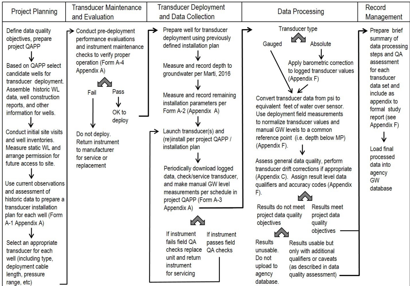
Figure 2 – Generalized workflow for deploying and assessing the results from submersible pressure transducers
