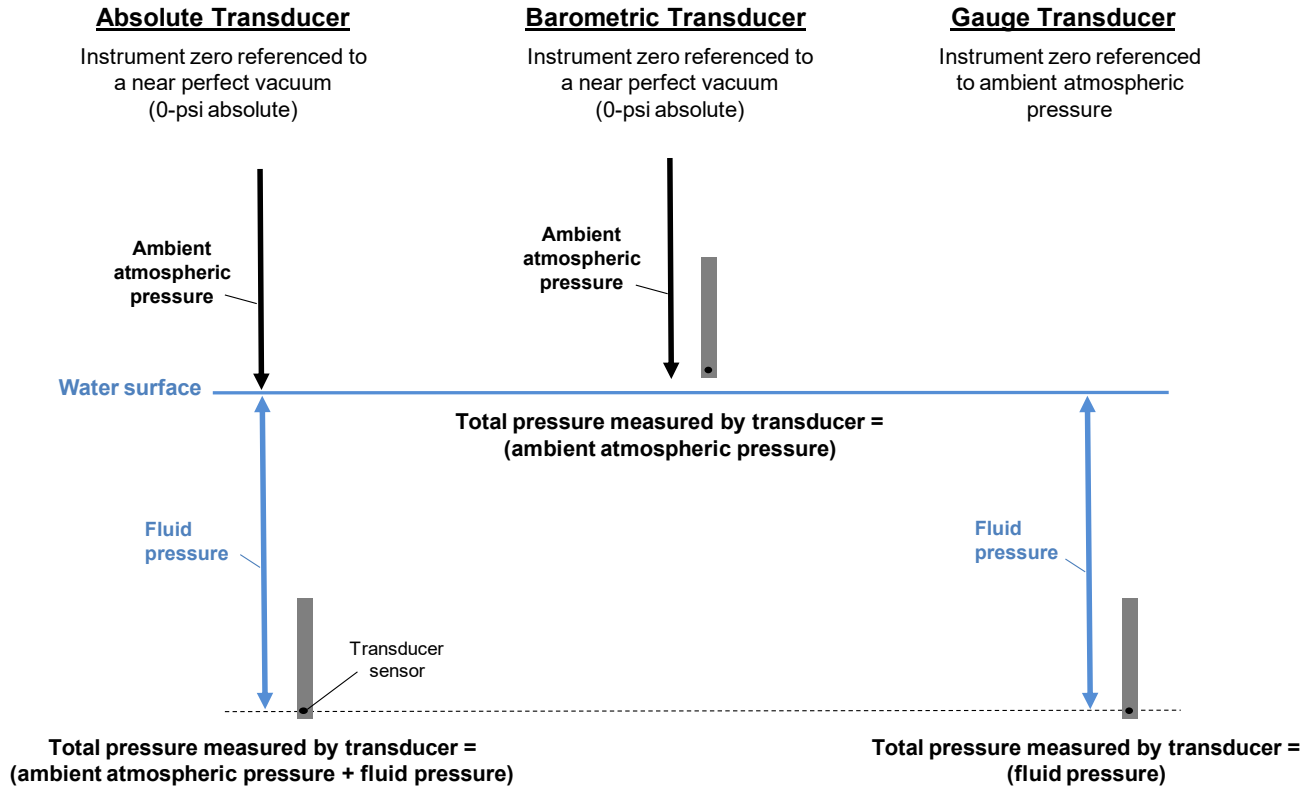
Figure 1 – Transducer Types and Associated Pressure Measurements
