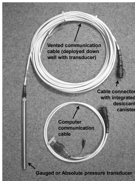
Figure 4 – Typical components for deploying a gauged/ absolute pressure transducer on a vented communication cable
