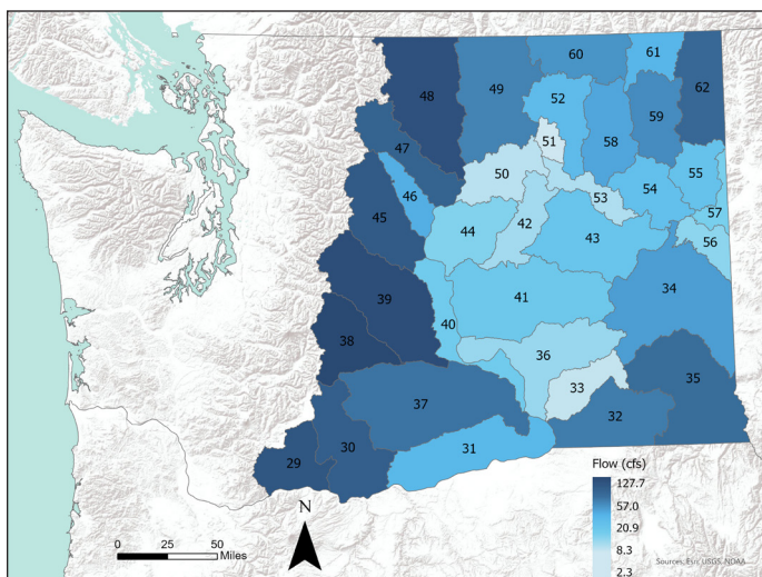
Figure 31. Historical (1982-2011) annual minimum 7-day average streamflow with a 2-year recurrence interval (7Q2) across Washington State's WRIs. Map produced for this 2021 Forecast using data obtained from Mauger et al. (2021).
