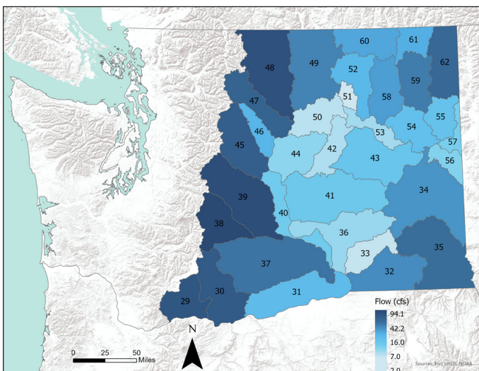
Figure 29. Historical (1982-2011) annual minimum 7-day average streamflow with a 10-year recurrence interval (7Q10) across Washington State's WRIsAs. Map produced for this 2021 Forecast using data obtained from Mauger et al. (2021).
