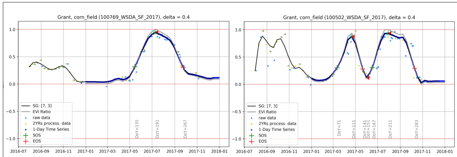
Figure 7. Schematic of greenness cycles for a single-cropping system (left) and for a double-cropped system (right). These curves were obtained from time series of Enhanced Vegetation Index (EVI) obtained from Sentinel-2 optical data.
