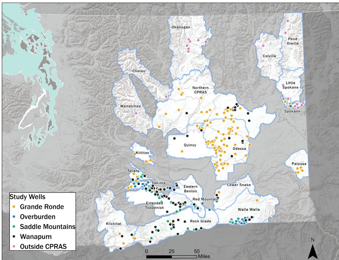
Figure 35. Washington's Aquifers geographic scope, showing the distribution of well locations (circles) used in the groundwater trends analysis. The colors of each well location show which aquifer layer the well accesses if within the Columbia Plateau Regional Aquifer System (CPRAS), or whether the well accesses a source of groundwater outside of the CPRAS.
