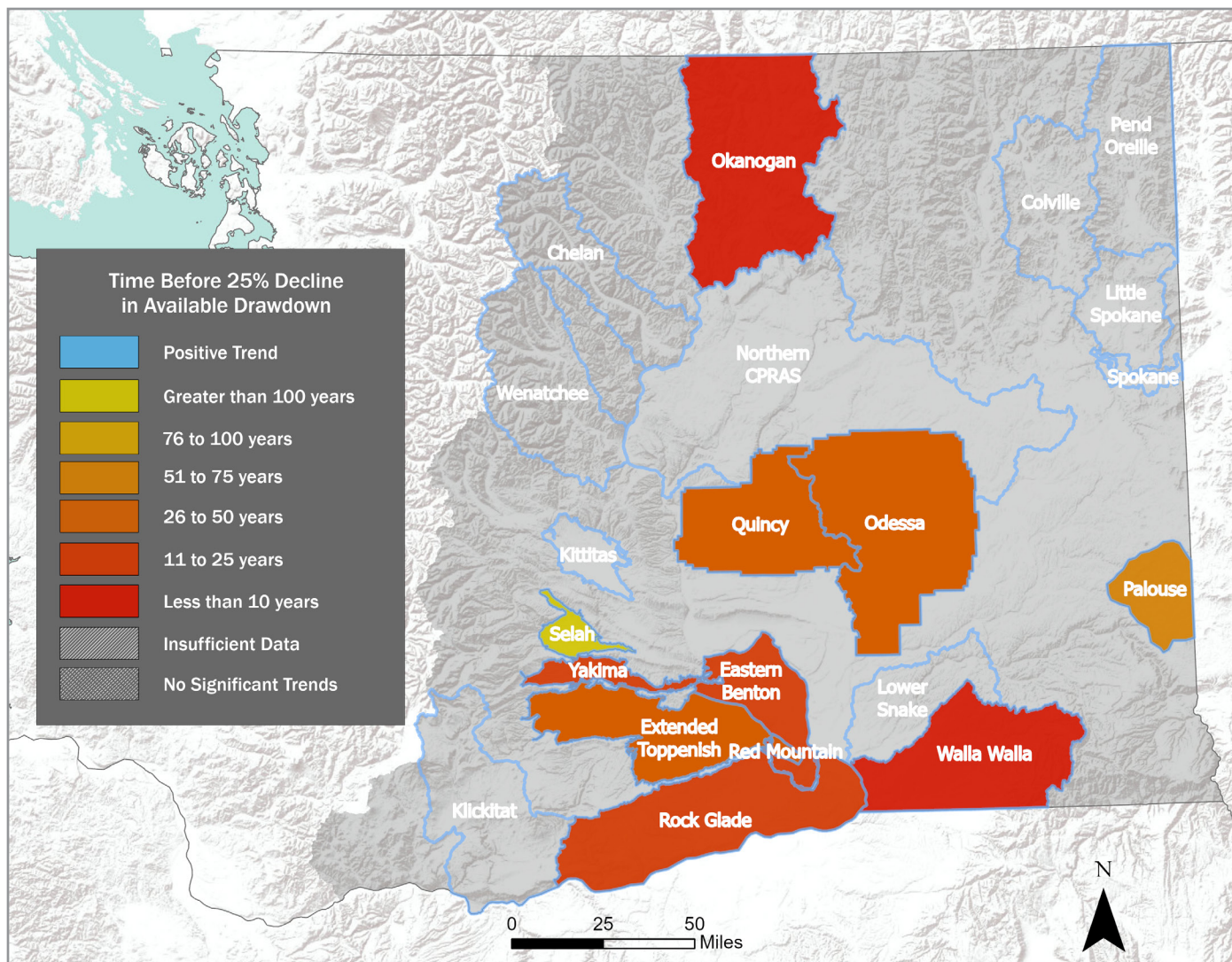
Figure ES-2. Time (in years) until the average available saturated thickness has declined by 25% in at least one aquifer layer in each groundwater subarea. These times are based on declines in available saturated thickness in different aquifer layers, as we show the most vulnerable aquifer layer for each subarea; that is, the time until 25% decline in available saturated thickness may reflect the vulnerability related to declines in the Grande Ronde layer for some subareas, for the Wanapum layer for other subareas, and the Overburden layer for other subareas (for more details see the Forecast Results for Aquifer Layers section).
