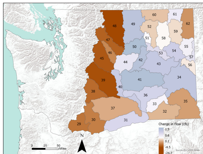
Figure 32. Expected changes in annual minimum 7-day average streamflow with a 2-year recurrence interval (7Q2) across Washington State's WRIs, between the historical (1982-2011) and the projected future (2030-2059) time periods. Future projections summarize results from 12 climate change scenarios, developed using dynamic downscaling, under greenhouse gas emissions scenario RCP 8.5. Map produced for this 2021 Forecast using data obtained from Mauger et al. (2021).
