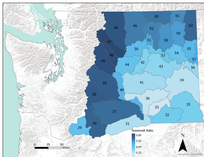
Figure 19. Historical (1976-2005) snowmelt ratio, obtained from an independent dataset. The snowmelt ratio reflects the relative contributions of snowmelt and rainfall to streamflow. The higher the ratio, the greater the contribution from snowmelt.
