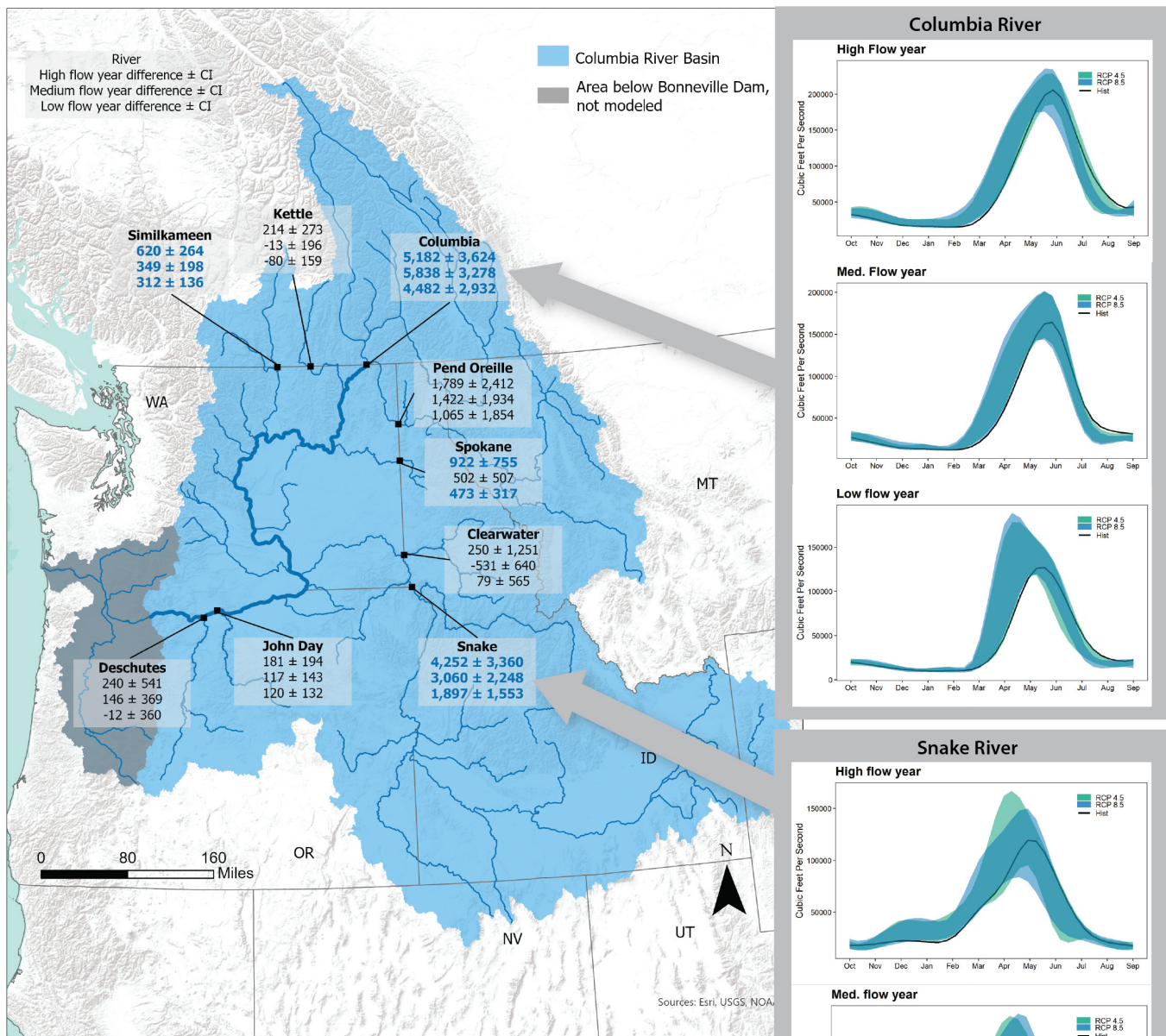
Figure 12. Expected change by 2040 in surface water supplies for major Columbia River tributaries entering Washington State (values measured just upstream of the point where the rivers enter Washington). The top number for each tributary refers to change expected by 2040 during high (80th percentile) supply years; the middle number refers to change expected by 2040 during median (50th percentile) supply years. The bottom number refers to change expected by 2040 during low (20th percentile) supply years. The confidence interval around the average change quantifies the uncertainty in possible future change, determined by the 34 climate change scenarios considered. All values are in cubic feet per second. Changes highlighted in orange and blue are decreases and increases in supply (expected to be associated with decreasing and increasing water availability), respectively, that are statistically different to zero. Values in black show metrics that are expected to remain mostly stable into the future. Inset panels show the historical (1986-2015) and forecast (2040) regulated surface water supplies (in thousands of acre-feet per month) on the Snake and Columbia Rivers upstream of the point where they enter Washington State for low (20th percentile; bottom graph in each inset panel), median (50th percentile; middle graph in each inset panel), and high (80th percentile; top graph in each inset panel) supply years. The spread of forecast (2040) supply is due to the range of climate change scenarios considered.
