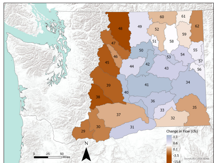
Figure 30. Expected changes in annual minimum 7-day average streamflow with a 10-year recurrence interval (7Q10) across Washington State's WRIsAs, between the historical (1982-2011) and the projected future (2030-2059) time periods. Future projections summarize results from 12 climate change scenarios, developed using dynamic downscaling, under greenhouse gas emissions scenario RCP 8.5. Map produced for this 2021 Forecast using data obtained from Mauger et al. (2021).
