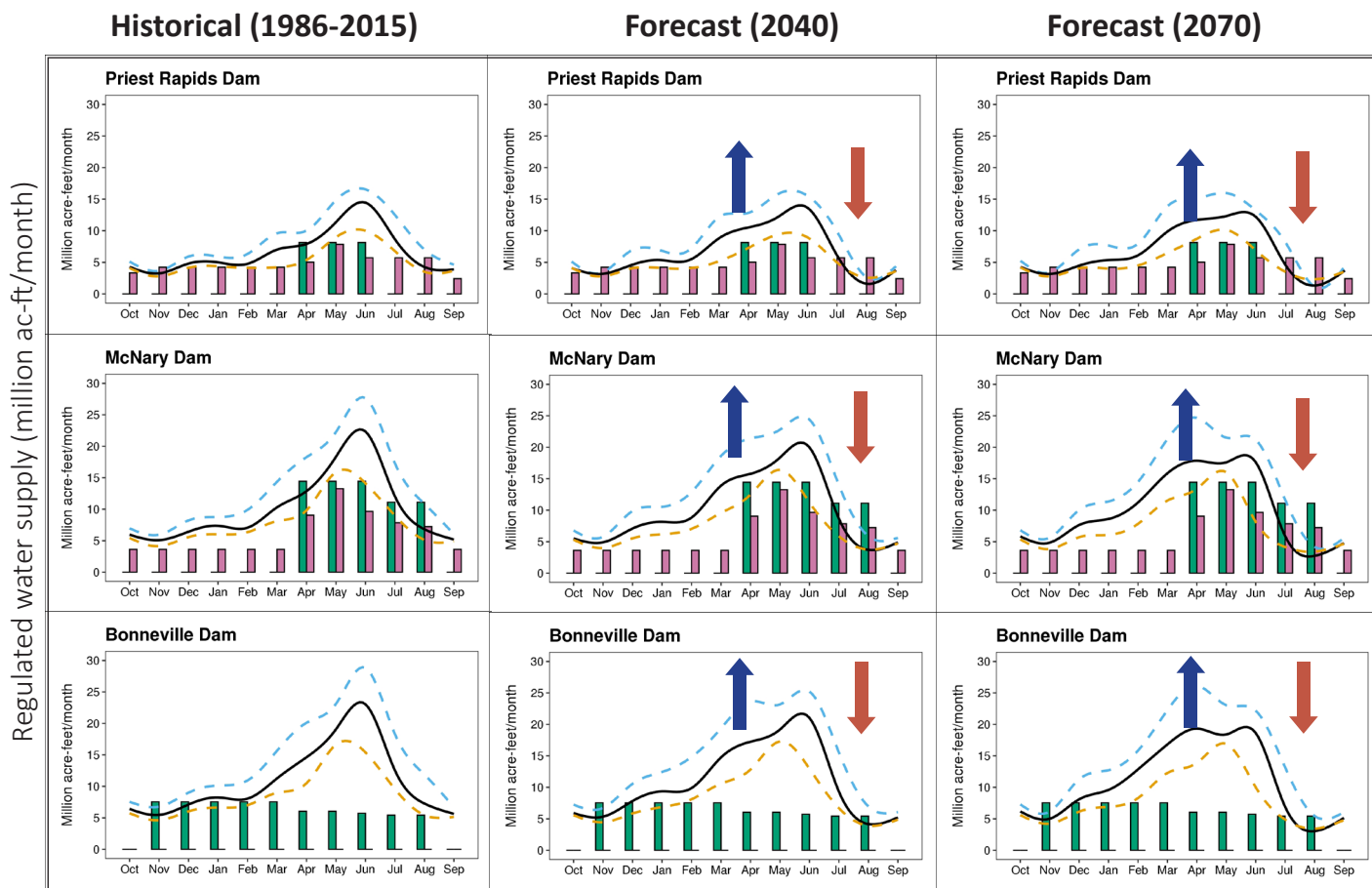
Figure 40. Historical (1986-2015: left column) and forecast (2040: center column; and 2070: right column) regulated surface water supply at Priest Rapids (top row), McNary (center row) and Bonneville (bottom row) Dams for low (20th percentile), median (50th percentile), and high (80th percentile) supply years, averaged across 34 climate change scenarios. Supplies presented are prior to accounting for out-of-stream demands. Also shown are the Washington State instream flow (WA ISF) and federal Biological Opinion (BiOp) flow targets (bars). The brown arrows show where future changes are worsening the Mainstem's ability to meet flow targets, while the blue arrows show where future changes are improving conditions.
