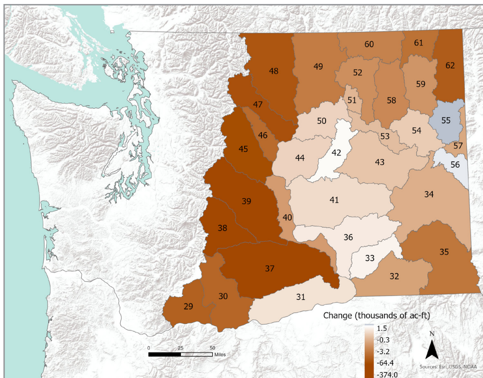
Figure ES-6. Change in surface water supply during summer months (June, July and August) from historical (1986-2015) to forecast (2040) periods, by WRIA. Changes in demand are expressed in thousands of acre-feet per year. One value is given for WRIs 37, 38, and 39, reflecting the sum of changes in those WRIs. Likewise, one value is given for WRIs 44 and 50, reflecting the sum of changes in those WRIs.
