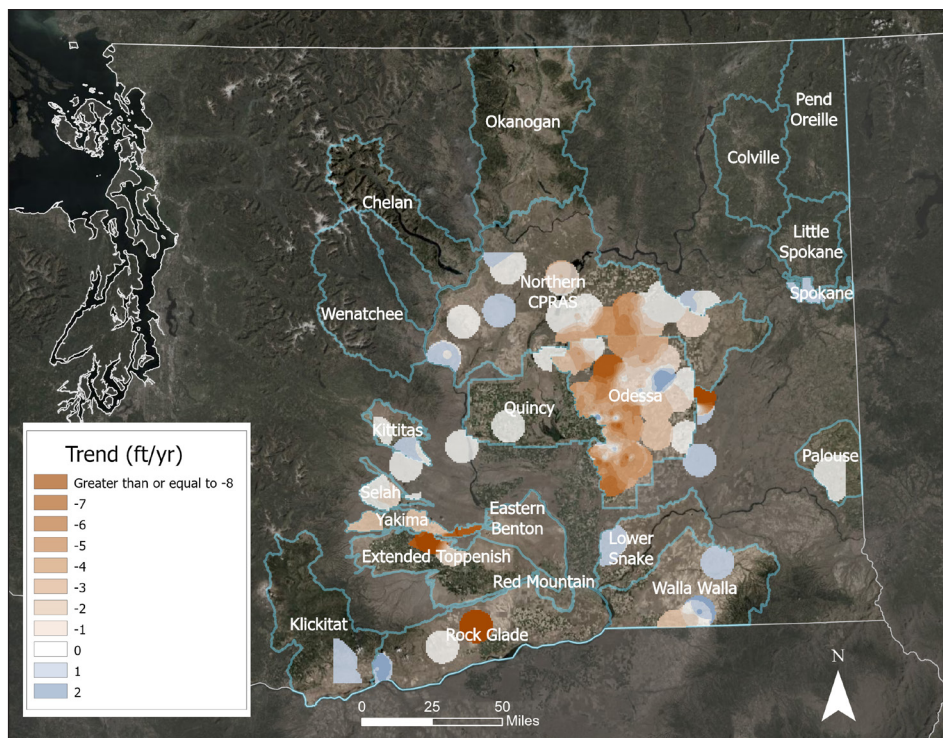
Figure 36. Interpolated trends in groundwater levels in the Grande Ronde Aquifer Layer. Interpolations were completed within each individual subarea based on a minimum of three wells (for further details see the Grande Ronde pages in the Forecast Results for Aquifer Layers section). Areas that do not have interpolated shading lacked adequate data to complete the analysis. The trends are overlaid on a satellite map where cultivated land area is visible in darker green for the central and southern subareas.
