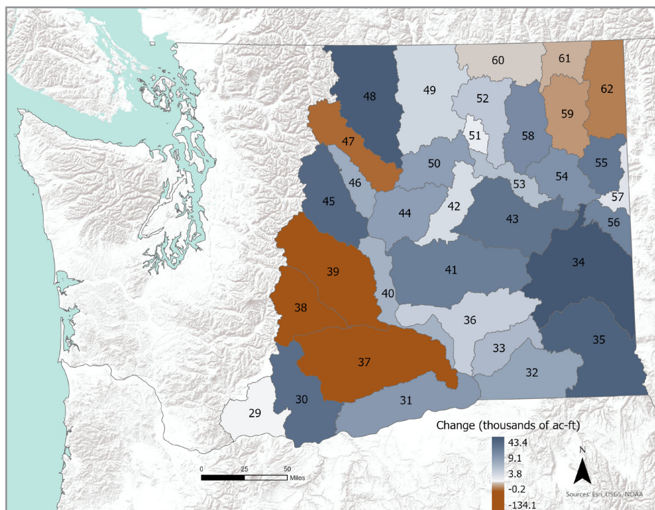
Figure ES-4. Changes in annual water supply expected during low flow years (20th percentile) by 2040, in thousands of acre-feet. WRIAs are colored based on the magnitude of change in annual water supply between historical (1986-2015) and forecast (2026-2055) time periods. Future supplies were represented by the median of 34 climate change scenarios. Note that one value is given for WRIAs 37, 38 and 39, and one value is given for WRIAs 44 and 50, reflecting the sum of changes in those groups of WRIAs.
