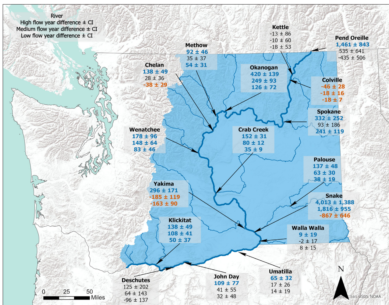
Figure 17. Expected change by 2040 in surface water flows (prior to accounting for demands) where tributaries join Washington's Columbia River Mainstem (above Bonneville Dam). The three numbers for each river refer to forecast (2040) surface water supply for a high (80th percentile; top), median (50th percentile; middle) and low supply year (20th percentile; bottom), averaged across 34 climate change scenarios (confidence interval around that average in parentheses). Changes highlighted in orange and blue are decreases and increases in supply (expected to be associated with decreasing and increasing water availability), respectively, that are statistically different to zero. All values are in cubic feet per second.
