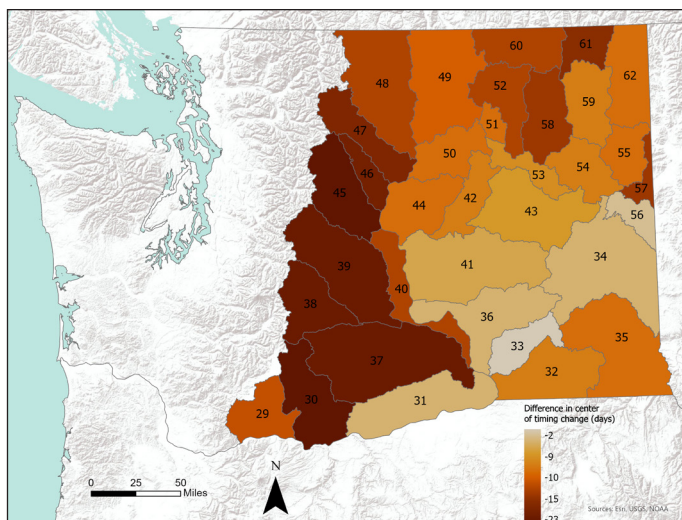
Figure 18. Changes in the timing of water supply expected during high flow years (80th percentile) by 2040. We quantified the shift based on the change, in number of days, of the center of timing of supply from the historical (1986-2015) to the forecast (2040) period (using the median of 34 climate change scenarios). Note that one value is given for WRIAs 37, 38 and 39, and one value is given for WRIAs 44 and 50, reflecting the sum of changes in those groups of WRIAs.
