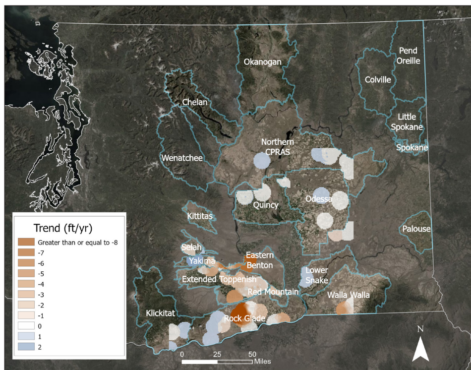
Figure 37. Interpolated trends in groundwater levels in the Wanapum Aquifer Layer. Interpolations were completed within each individual subarea based on a minimum of three wells (for further details see the Wanapum pages in the Forecast Results for Aquifer Layers section). Areas that do not have interpolated shading lacked adequate data to complete the analysis. The trends are overlaid on a satellite map where cultivated land area is visible in darker green for the central and southern subareas.
