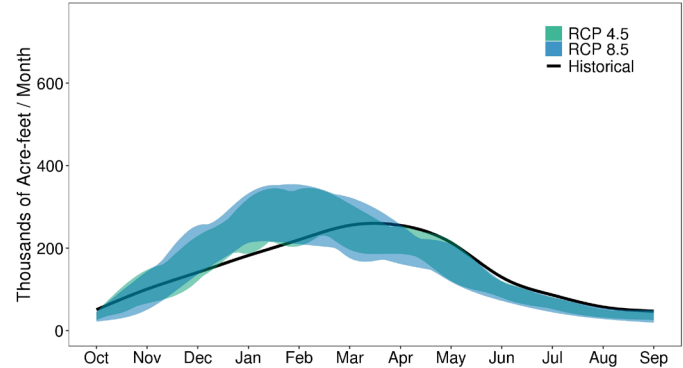
Low Flow Year - Future GCMs (2070)
