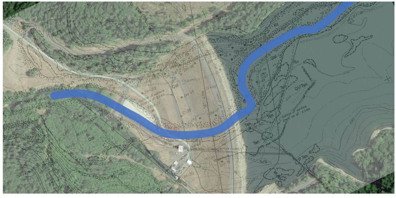
Figure 11 Historical Alignment of Skookumchuck River in Relationship to Current Dam Configuration (View shows Google Earth aerial image overlain with geologic map (drawing C-5110) from original dam construction.)
