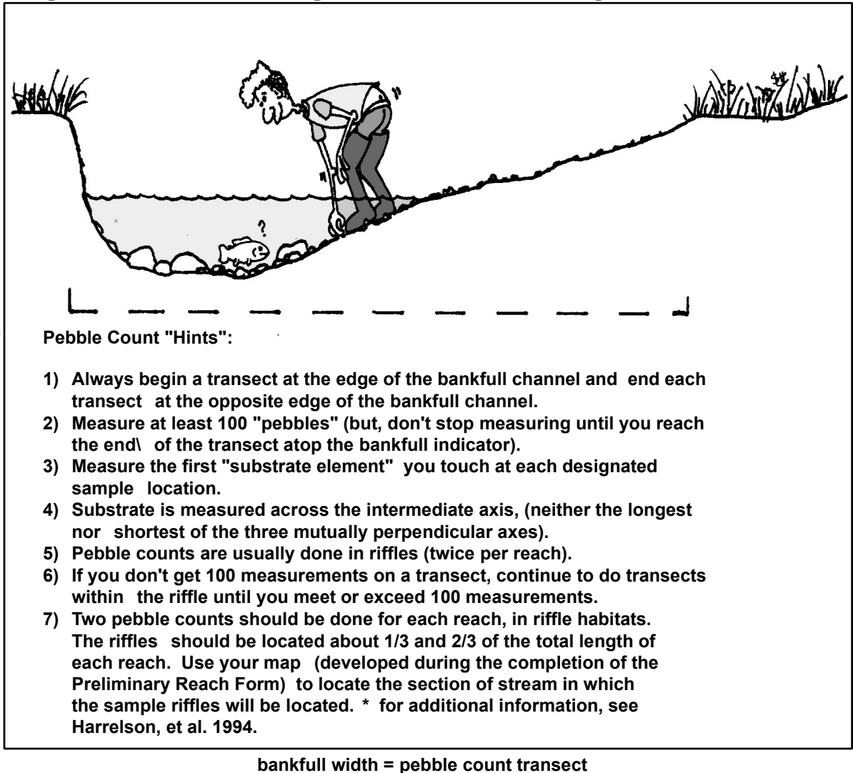
Figure 19: General guidelines for doing pebble counts
