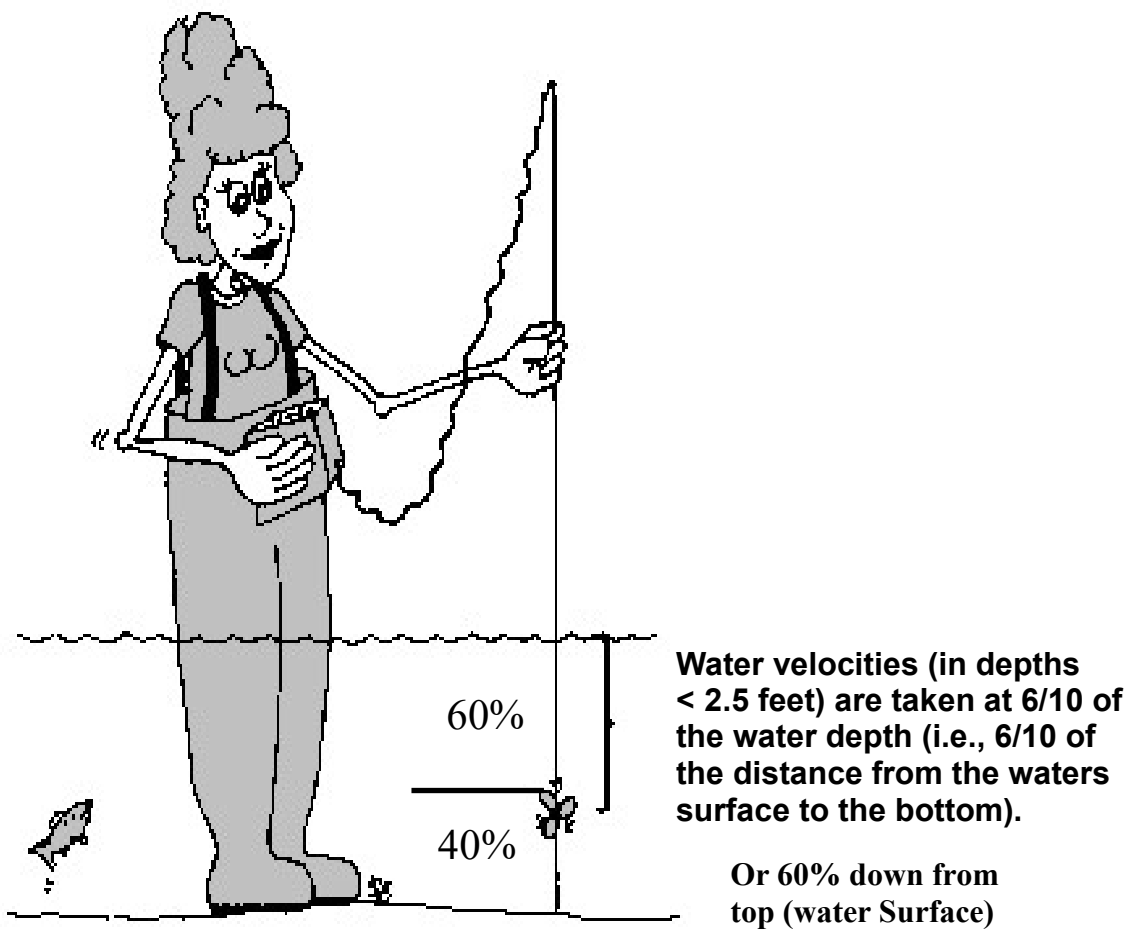
Figure 17: Water velocities are measured at 6/10 of the water column depth
