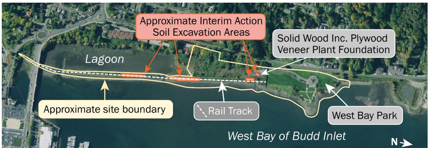
Figure 3. A diagram showing the proposed interim action work.
