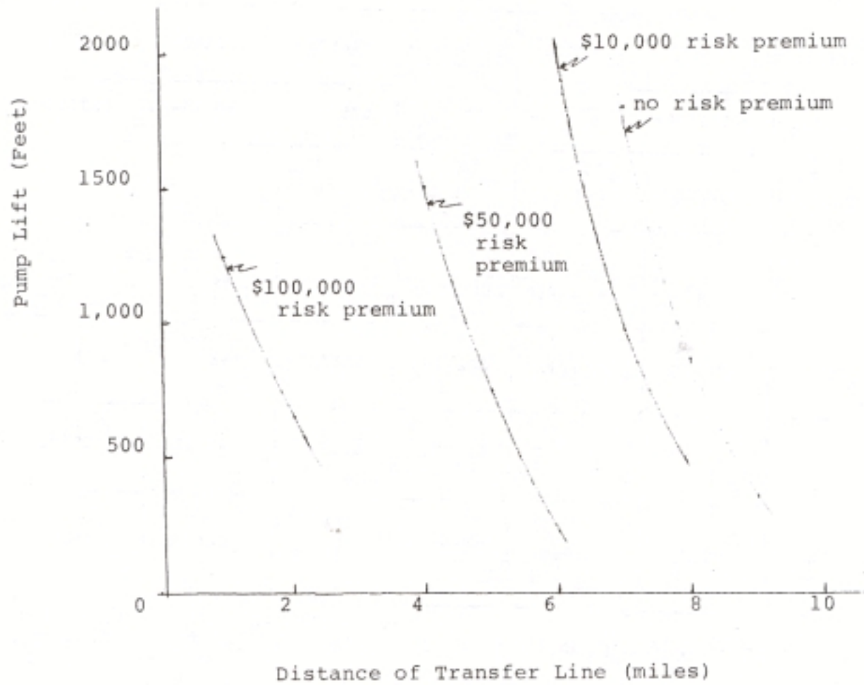
Figure 3. "Break-even" Curves for Various Risk Premiums; Soil Class A
