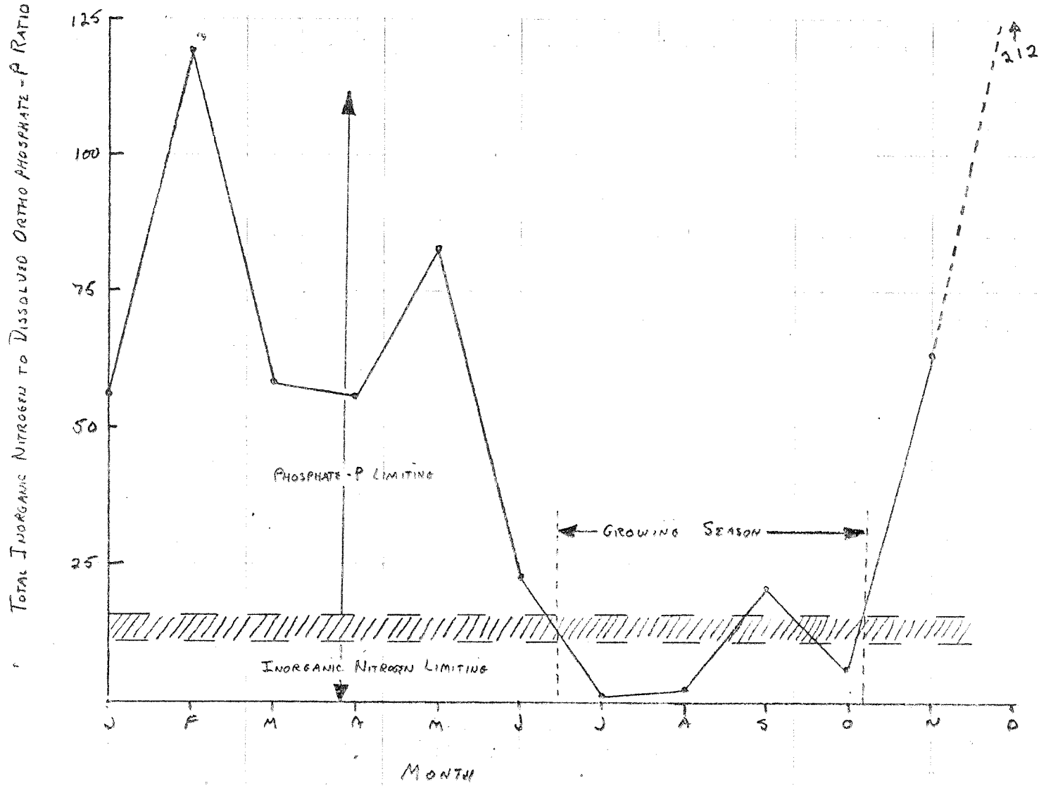
FIGURE 3. AVAILABLE NITROGEN:PHOSPHORUS RATIO / CHEHALIS RIVER MELLEN ST. BRIDGE (AVERAGE VALUES 10/77 to 6/80)
