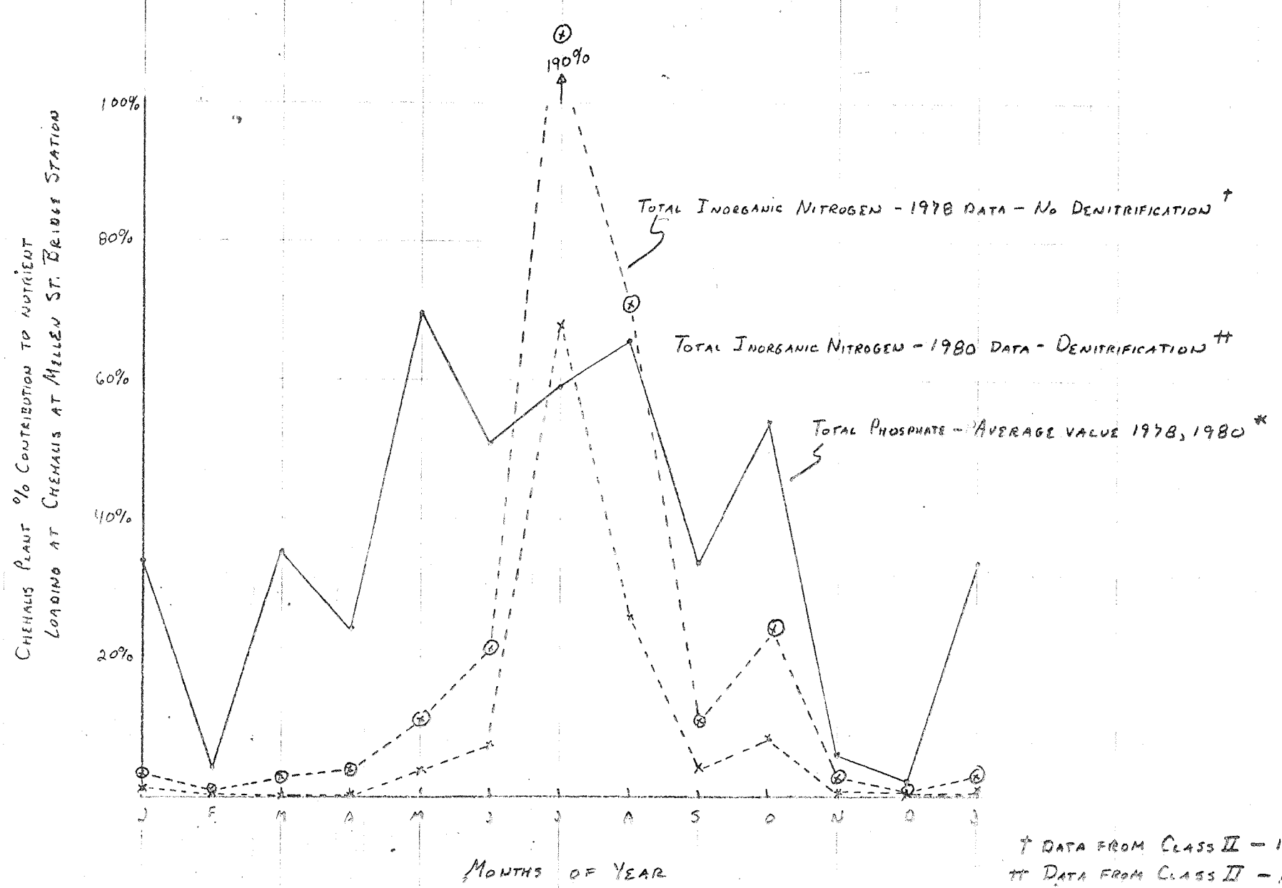
FIGURE 4. CONTRIBUTION OF CHEHALIS PLANT EFFLUENT TO NUTRIENTS IN CHEHALIS RIVER AT MILLEN ST. BRIDGE STATION
