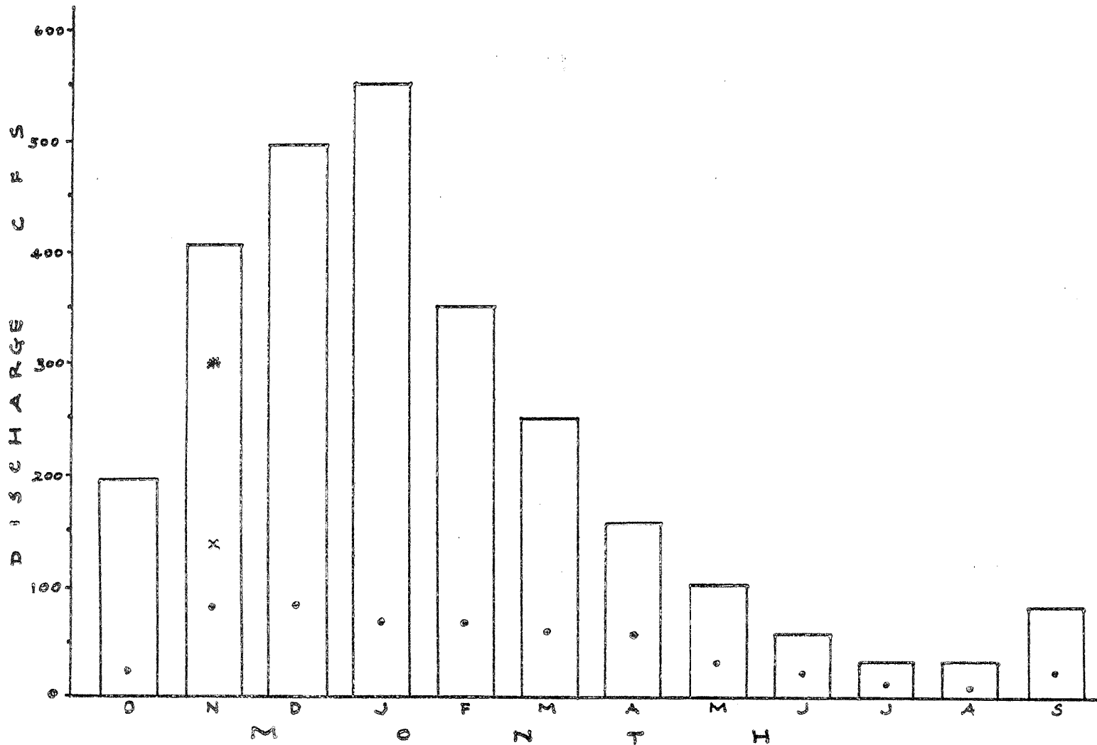
Figure 3. Monthly mean and mean minimum discharge (●) for the Moclips River at Moclips, Station 12039220 (USGS 1975 - 1981), compared to November 7, 1984, discharges taken on Joe Creek below Stream #0744 (x) and on the Moclips River (*).
