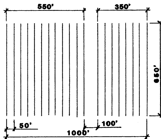
Facility Configuration
