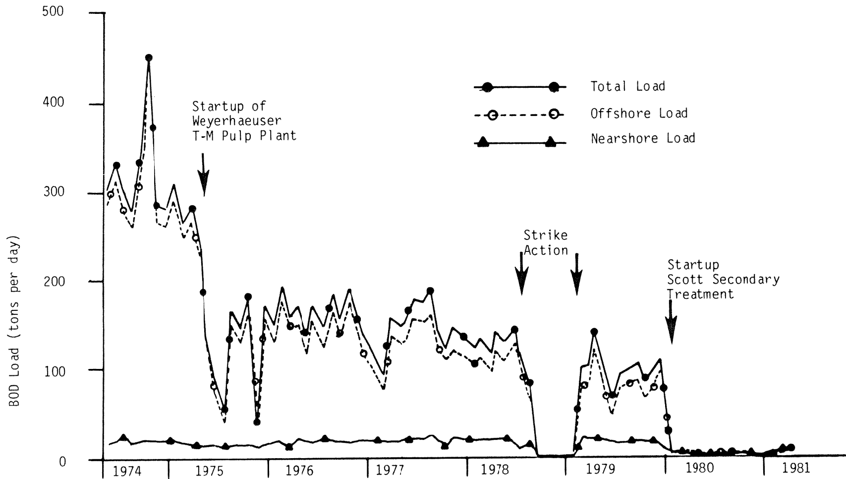
Figure 3. Waste loads vs. time from pulp mills into Port Gardner during ECOBAM 1974 - 1981.
