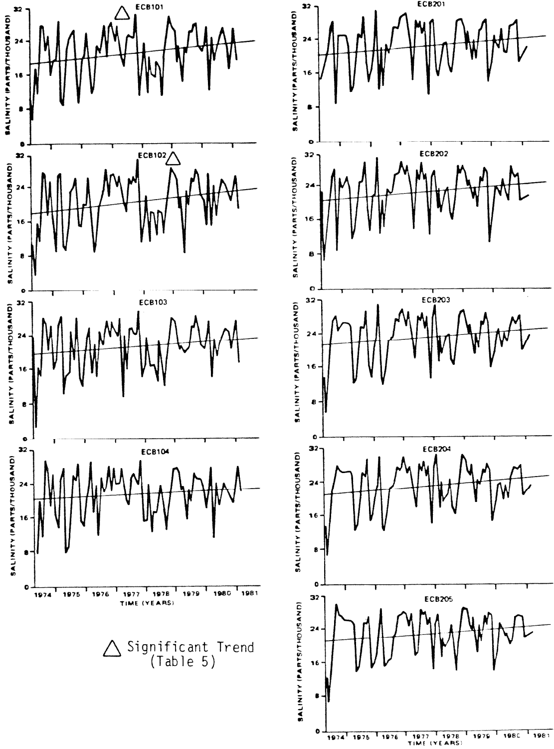
Figure 8. Salinity versus time from ECOBAM beach and deep seine stations (trend analysis was not done).
