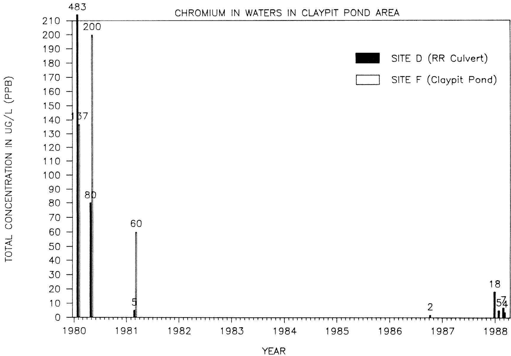
Figure 2. Historical trend in chromium levels in Claypit Pond vicinity. Site letters refer to Figure 1 and Table 1.
