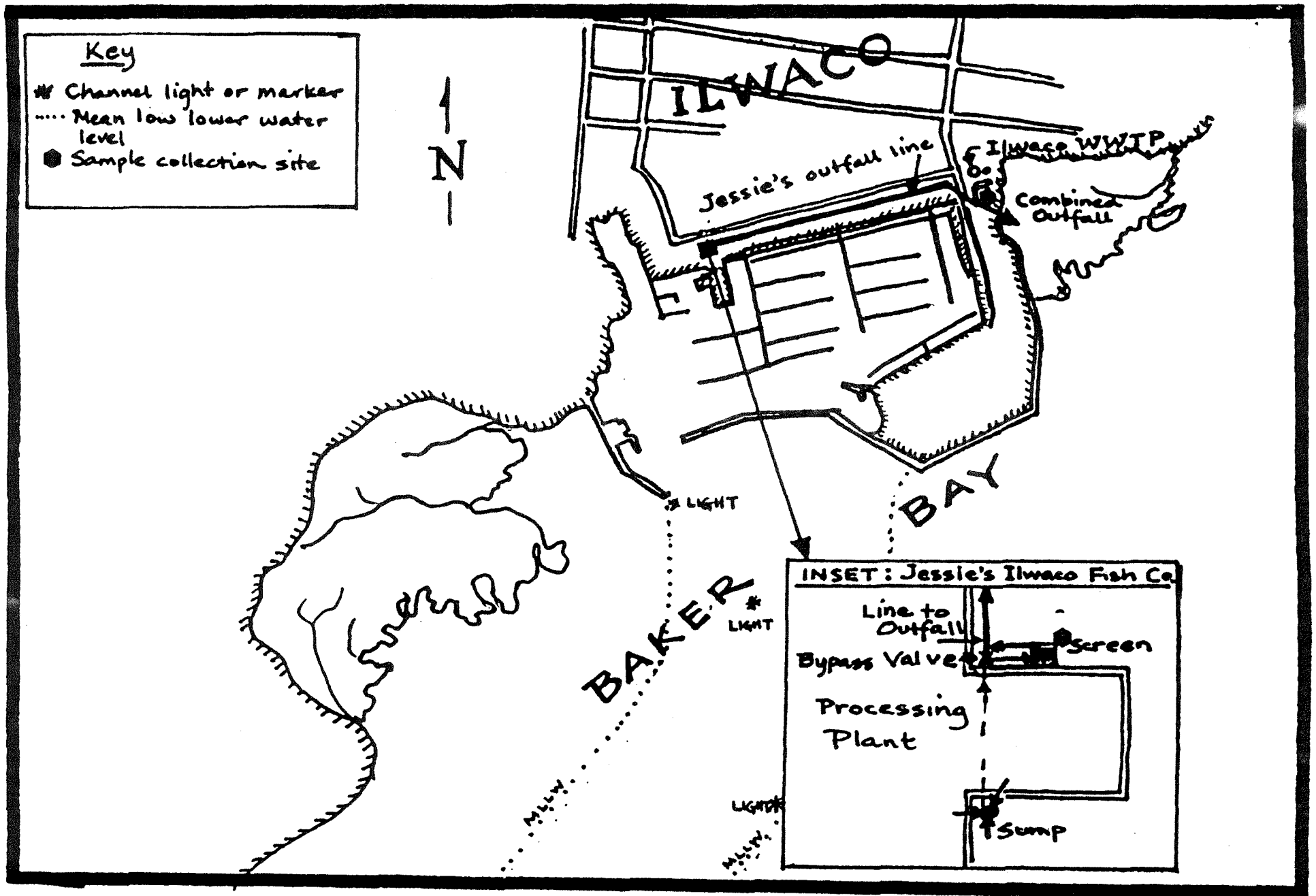
Figure 2. Jessie's Ilwaco Fish Company site and sampling locations used during the September 1988 survey.
