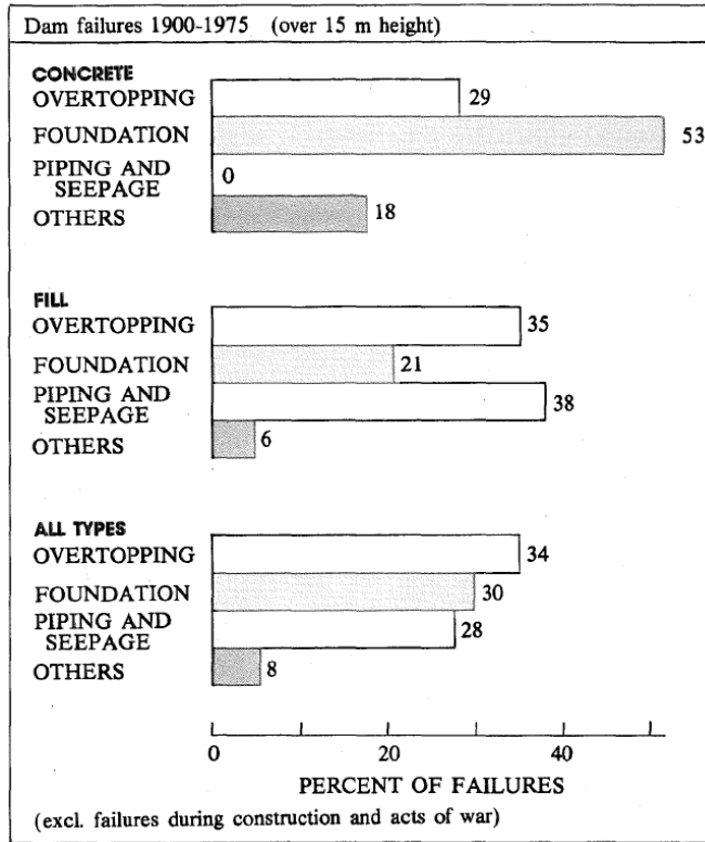
Figure 3.3 Cause of Failure. – Source: ICOLD (1973)
