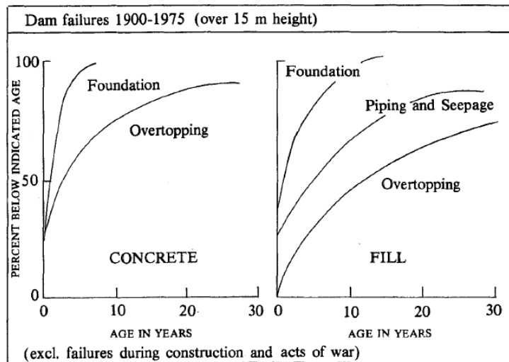
Figure 3.4 Age at Failure. – Source: ICOLD (1973)
