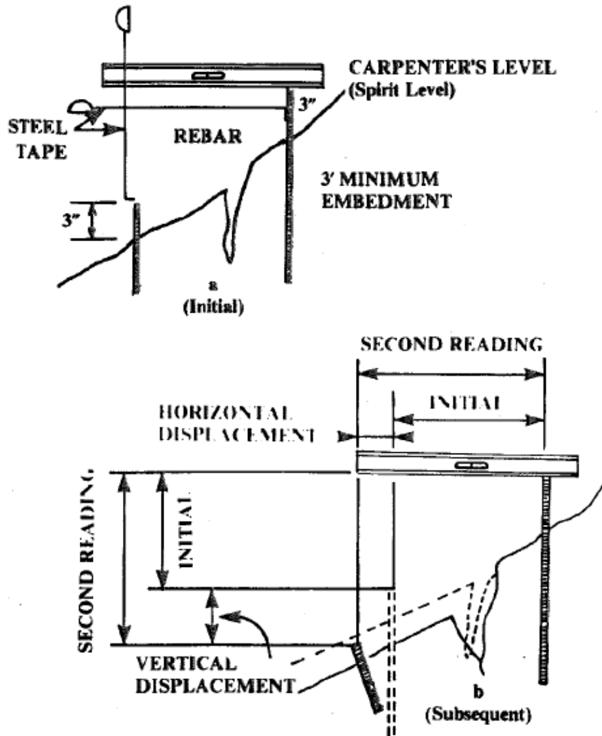
Figure 6.2 Monitoring Cracks on Embankment
