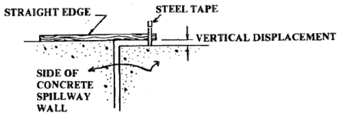
b. Straight edge and tape plus reference points
