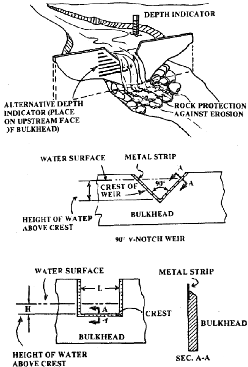
Figure 6.7 Standard Weirs
