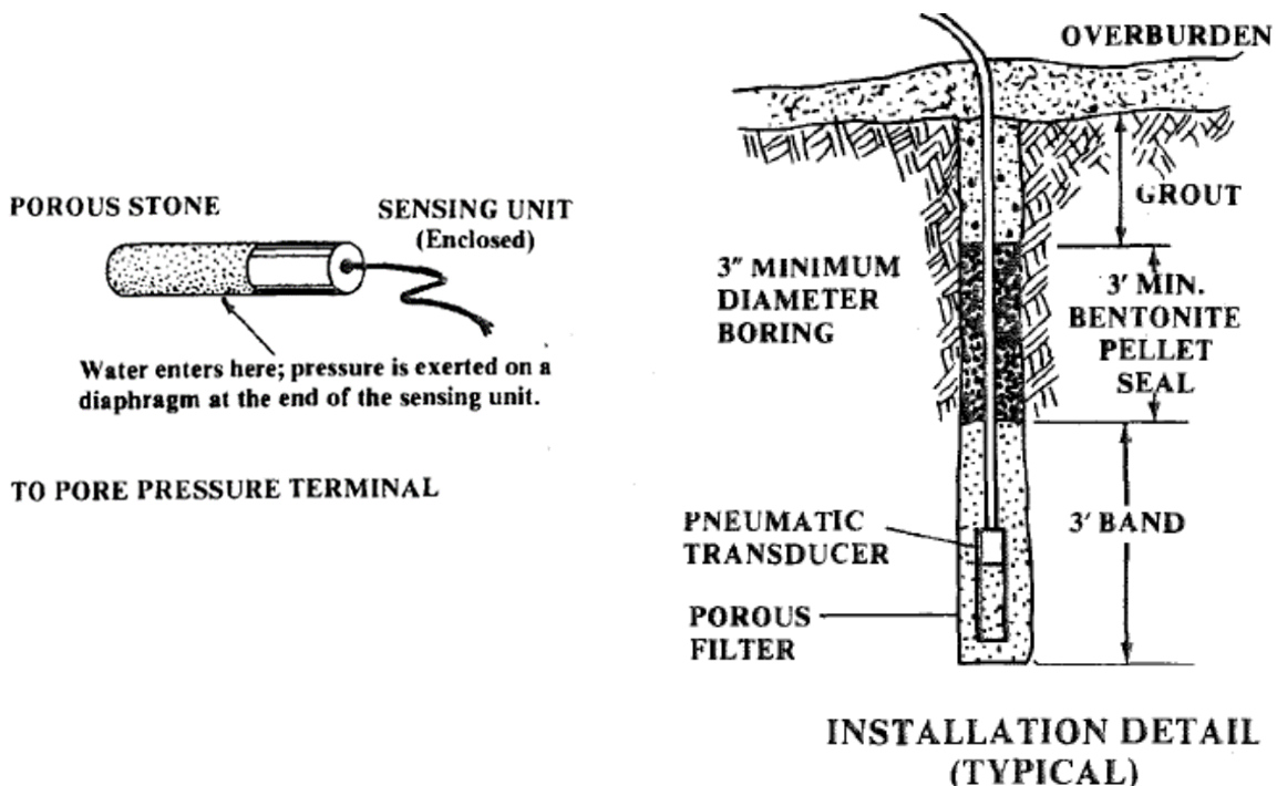
Figure 6.5 Porous Stone Piezometer
