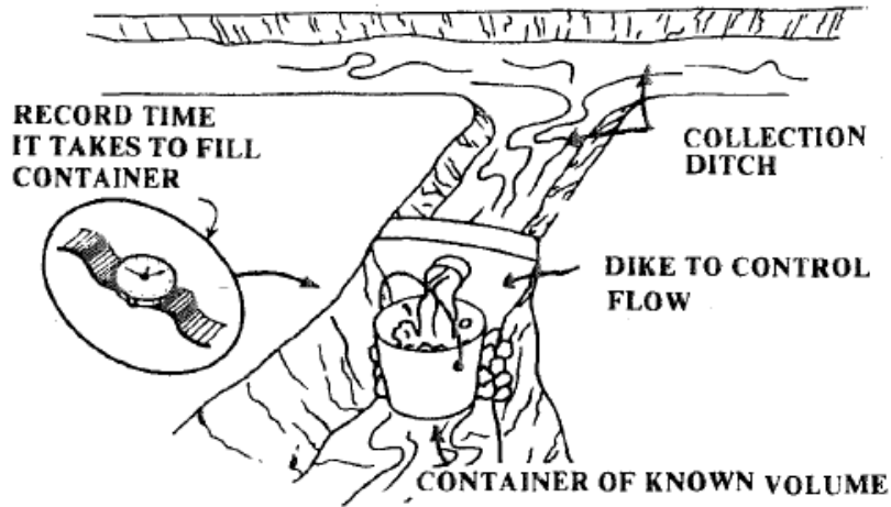
Figure 6.9 Bucket and Stopwatch Method
