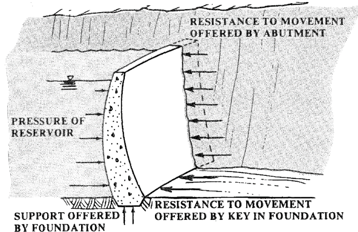
Figure 2.4 Concrete Arch Dam
