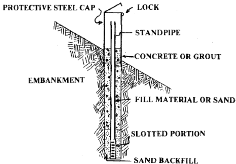
Figure 6.6 Typical Observation Well Installation
