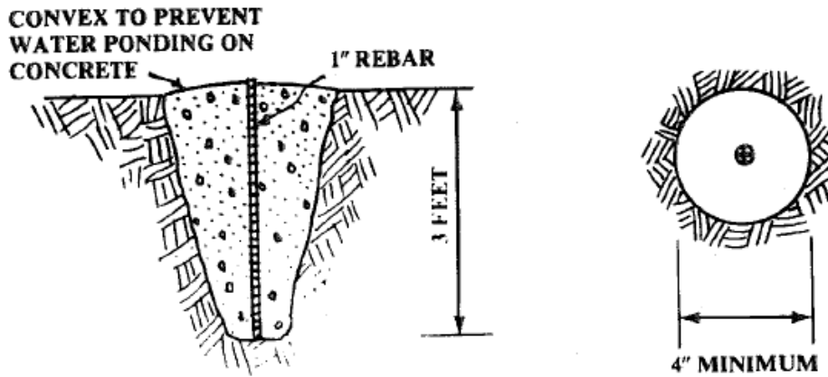
Figure 6.1a Installation of Permanent Points
