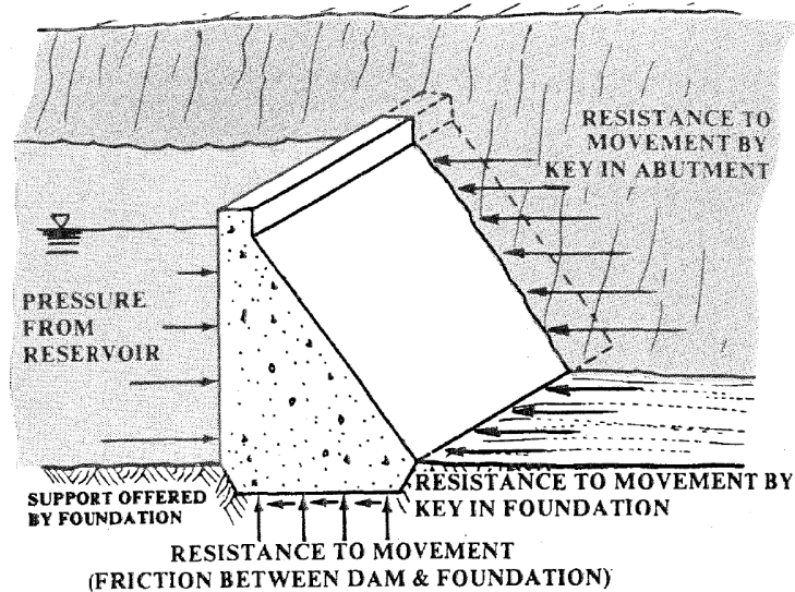
Figure 2.3 Concrete Gravity Dam
