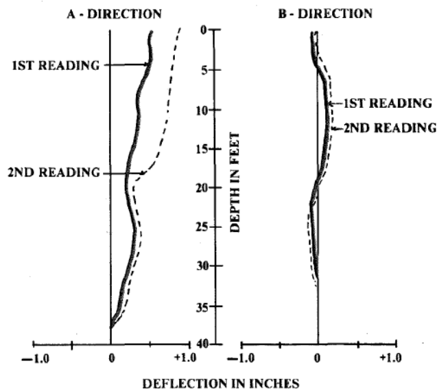
Figure 6.3b Plot of Inclinometer Readings
