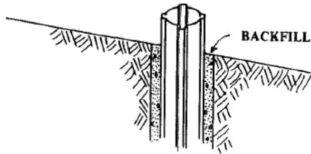
Figure 6.3a Inclinometer – Detail at Surface
