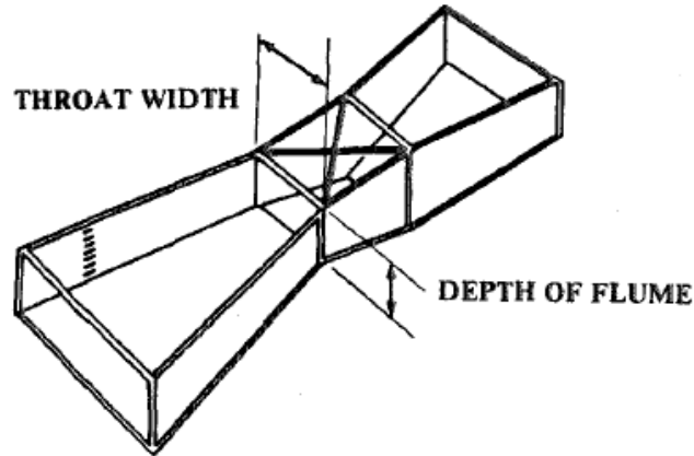
Figure 6.8 Parshall Flume
