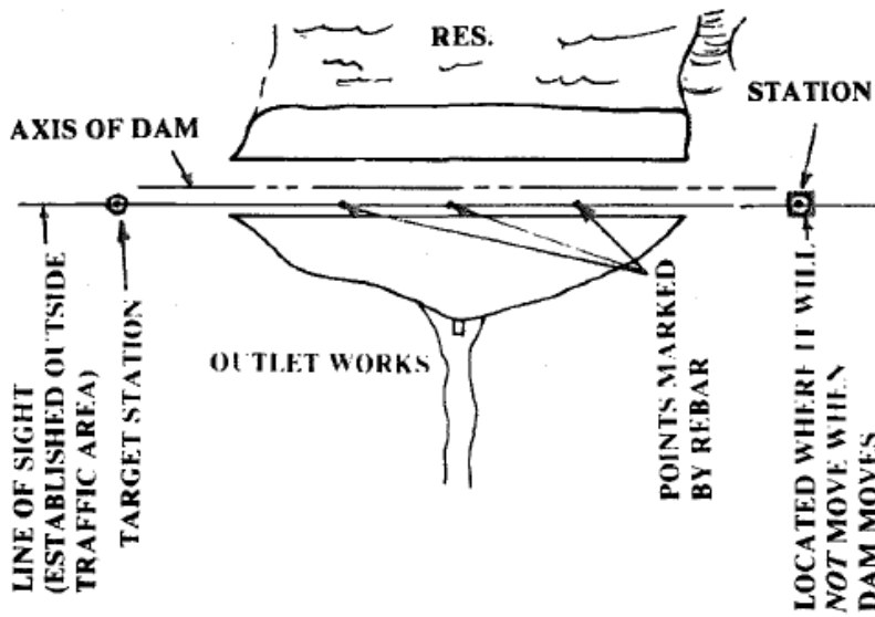
Figure 6.1b Plan of Alignment System
