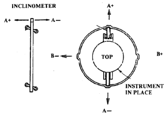
Figure 6.3c Inclinometer and Casing
