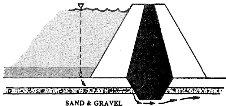
Figure 2.5 Cutoff Trench and Upstream Blanket
