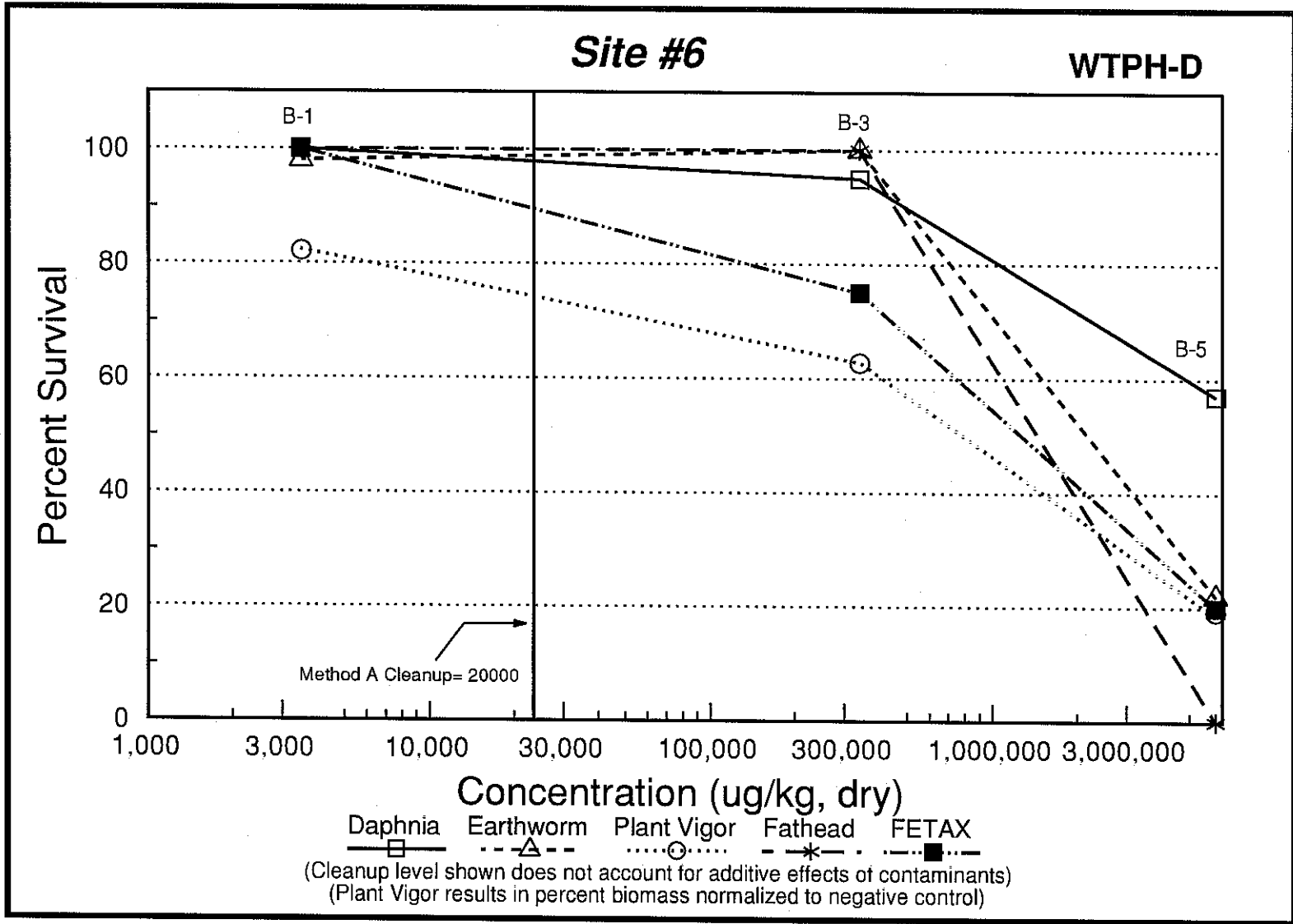
Figure 8: Response of bioassay suite to primary contaminants in soils at Site #6.
