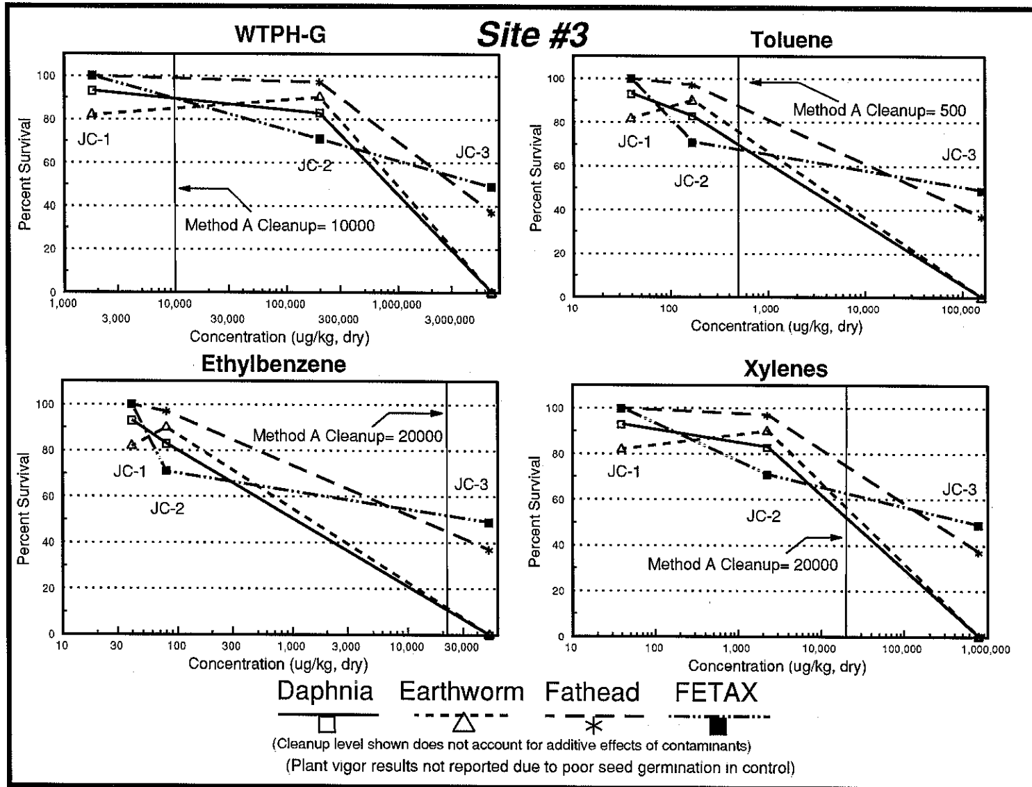
Figure 5: Response of bioassay suite to primary contaminants in soils at Site #3.
