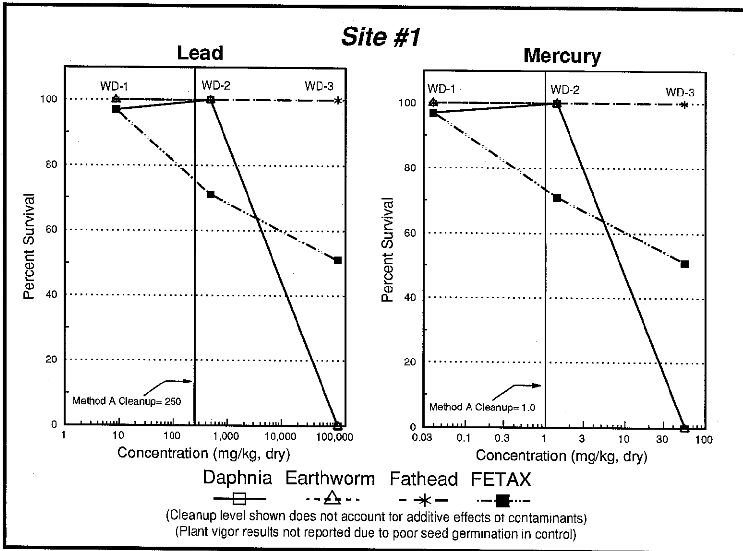
Figure 3: Response of bioassay suite to primary contaminants in soils at Site #1.
