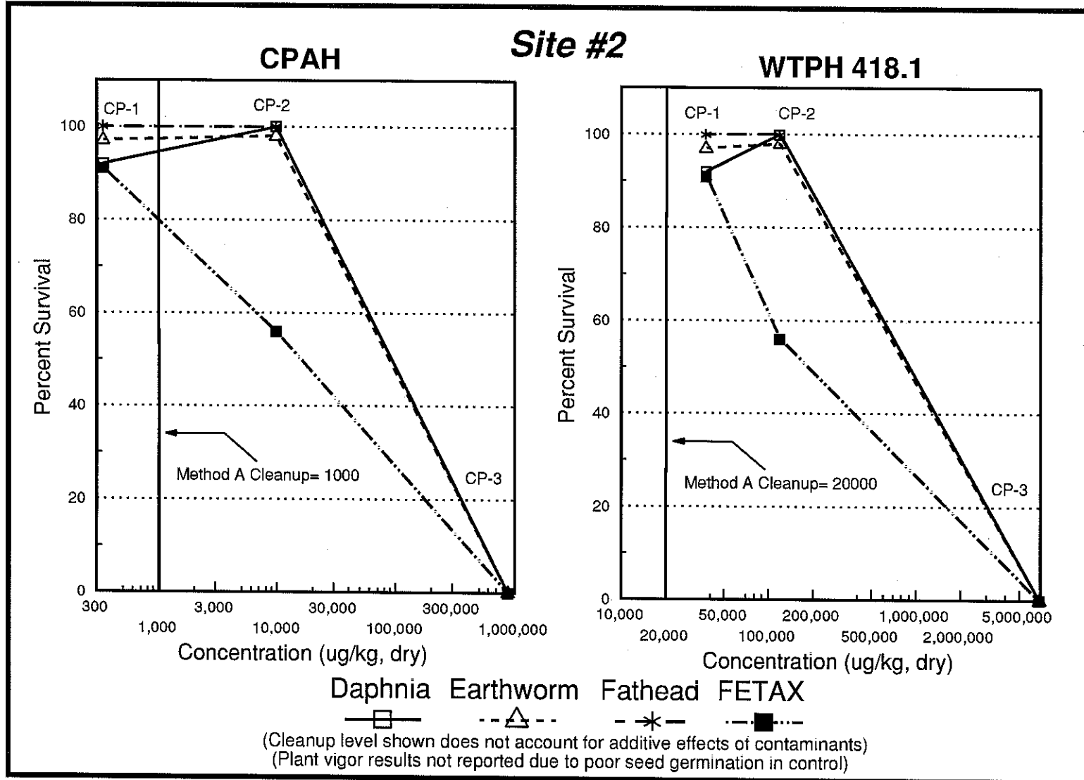
Figure 4: Response of bioassay suite to primary contaminants in soils at Site #2.
