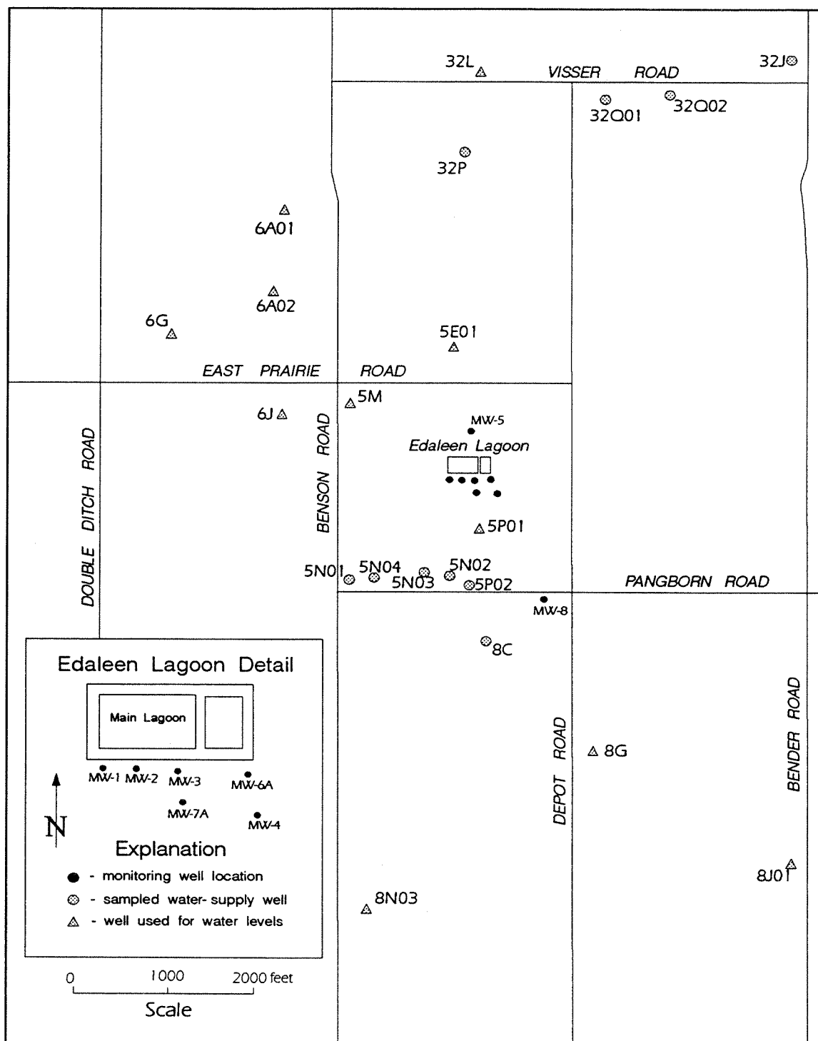
Figure 3. Well locations in the Edaleen study area
