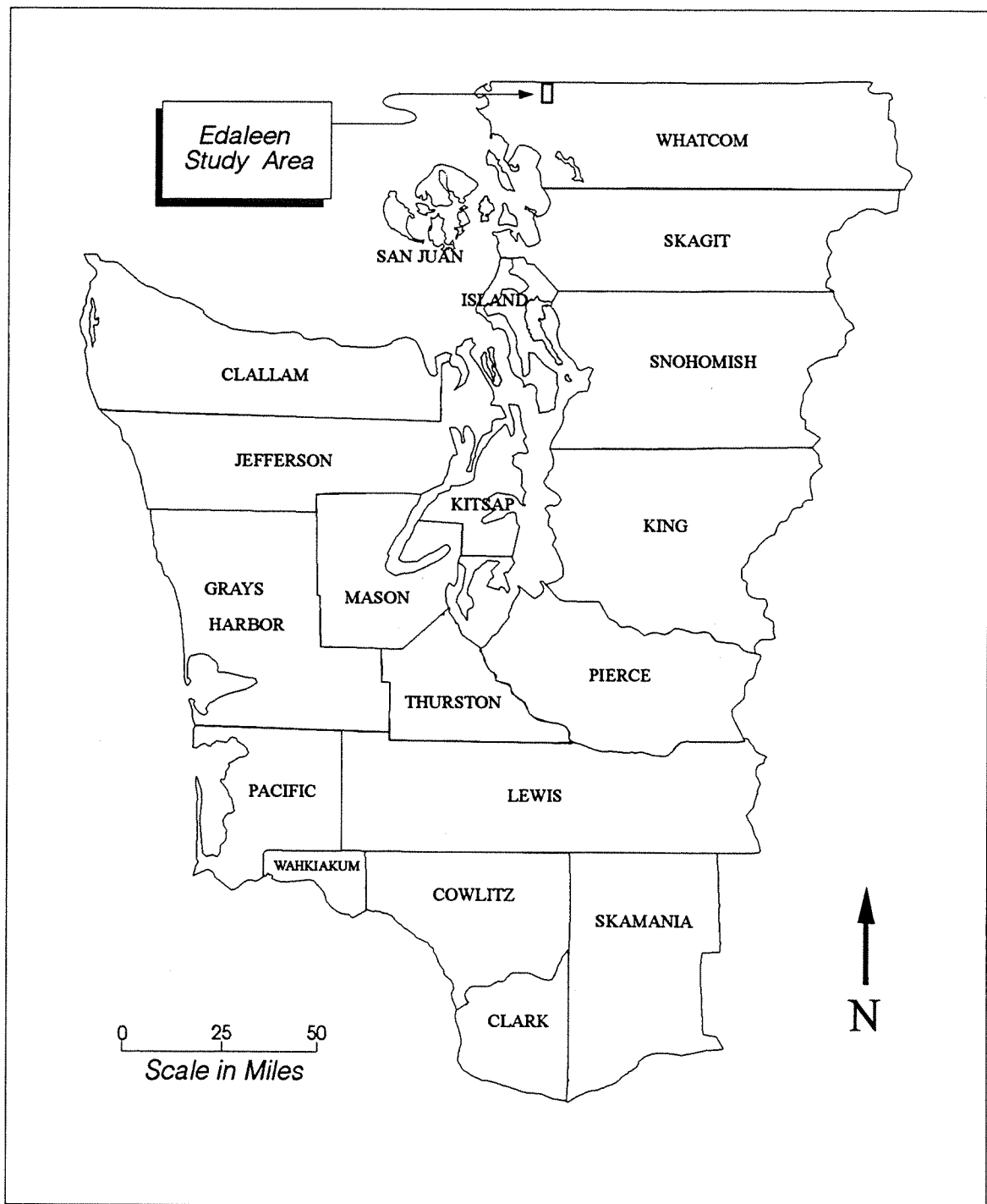
Figure 1. Edaleen study area location
