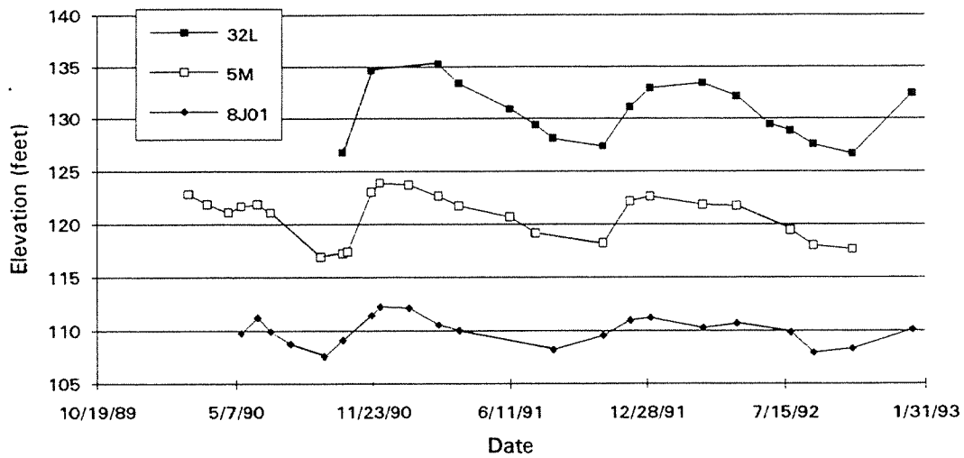
Figure 4. Hydrographs for irrigation wells near Edaleen Dairy.
