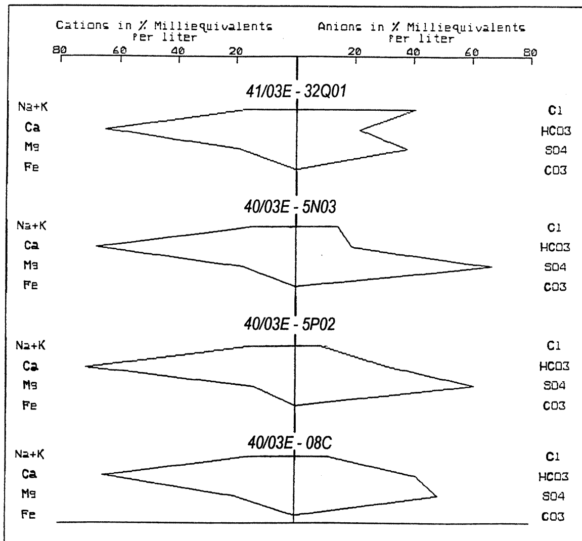
Figure 9. Comparison of water quality in four domestic wells.
