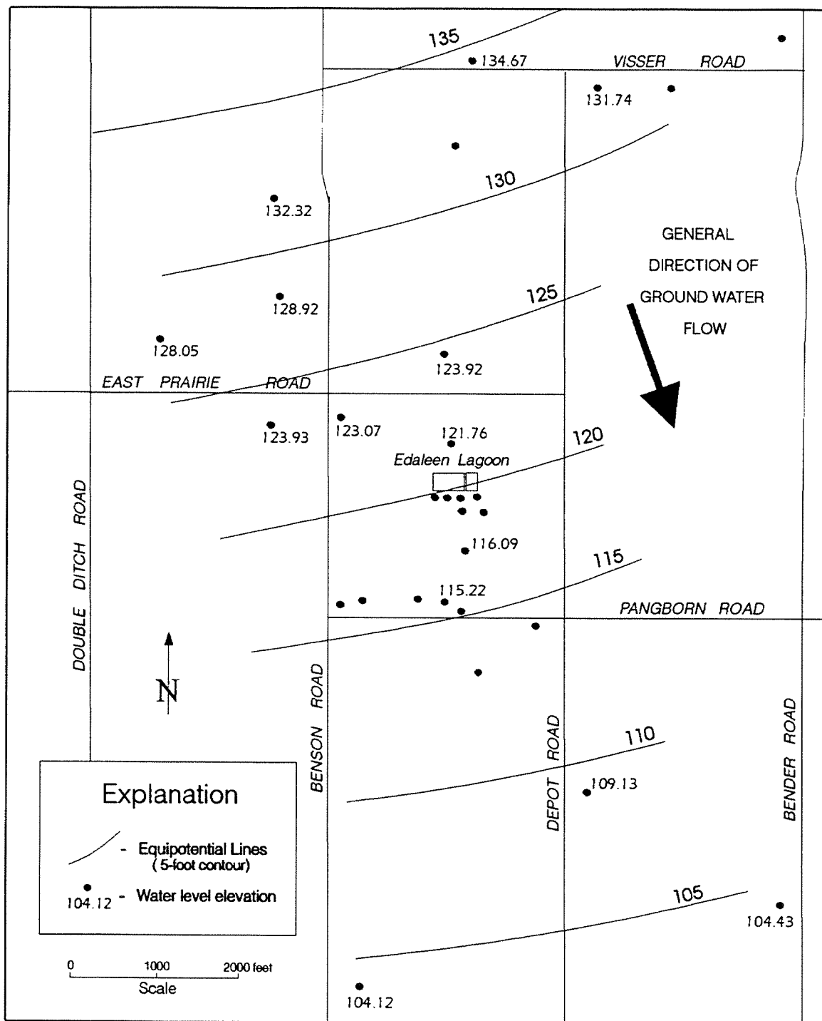
Figure 6. Water-table contours in the Edaleen study area based on well measurements taken Nov. 21, 1990.
