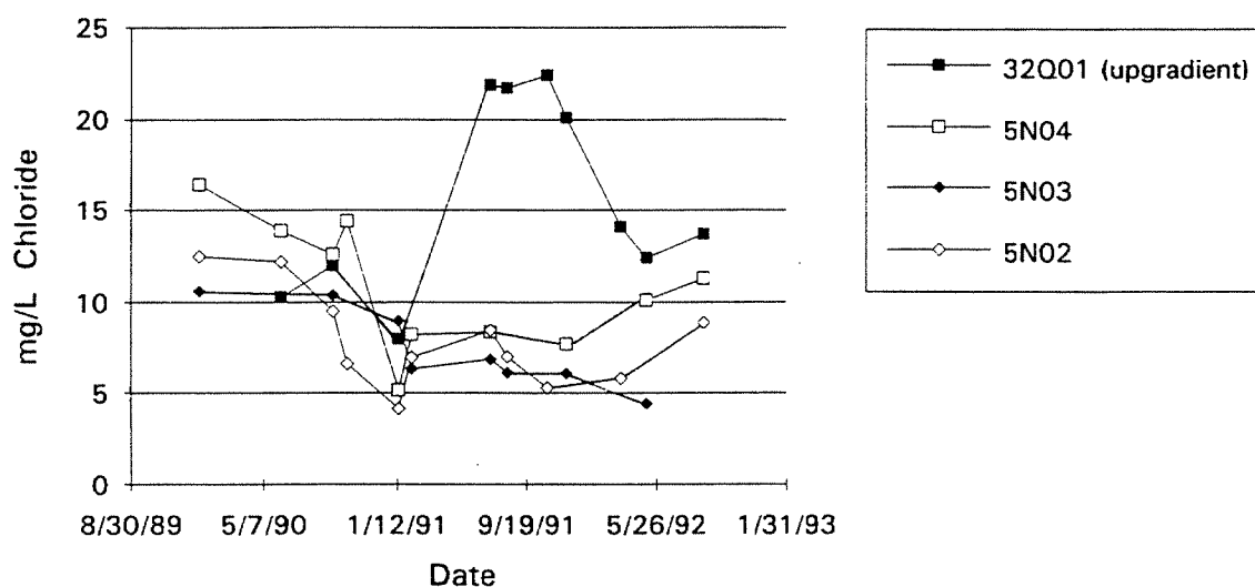
Figure 7. Chloride in domestic wells near Edaleen Dairy.
