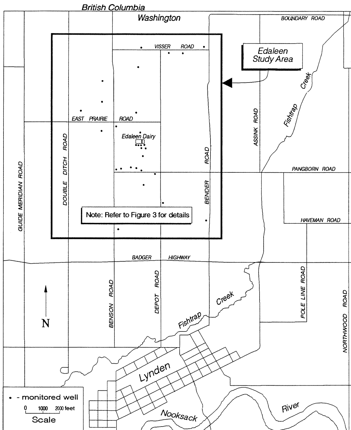
Figure 2. Edaleen study area.
