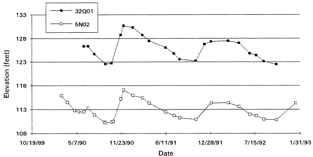
Figure 5. Hydrographs for domestic wells near Edaleen Dairy.
