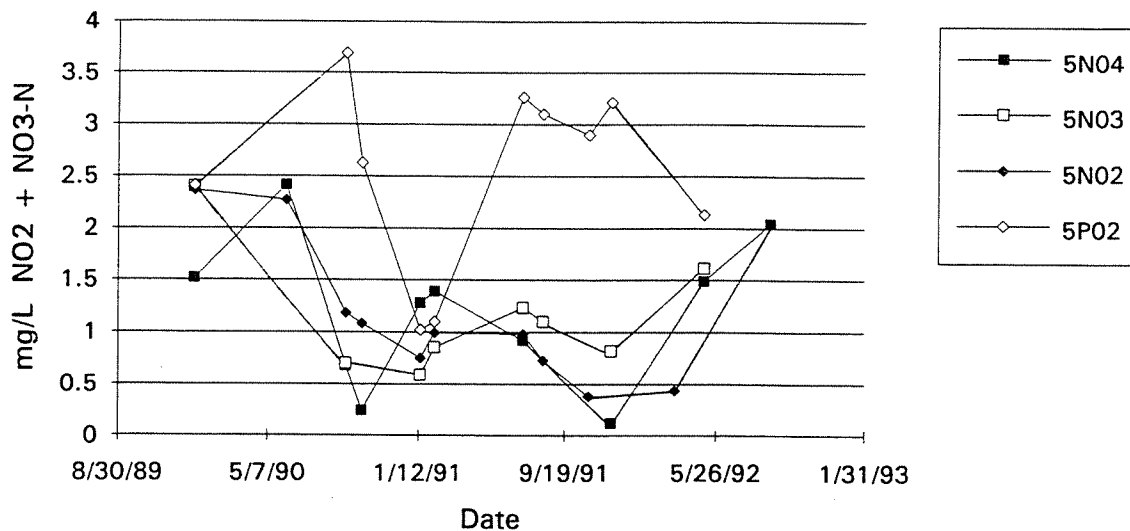
Figure 8. Nitrate in domestic wells near Edaleen Dairy.
