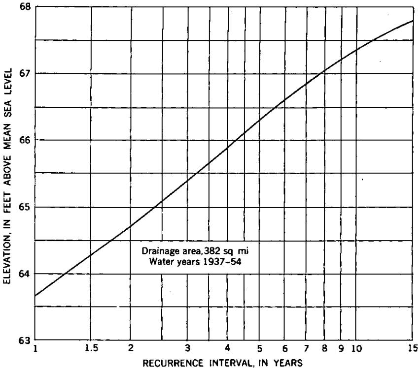
FIGURE 26.—Flood-stage frequency curve, Green River near Auburn.
