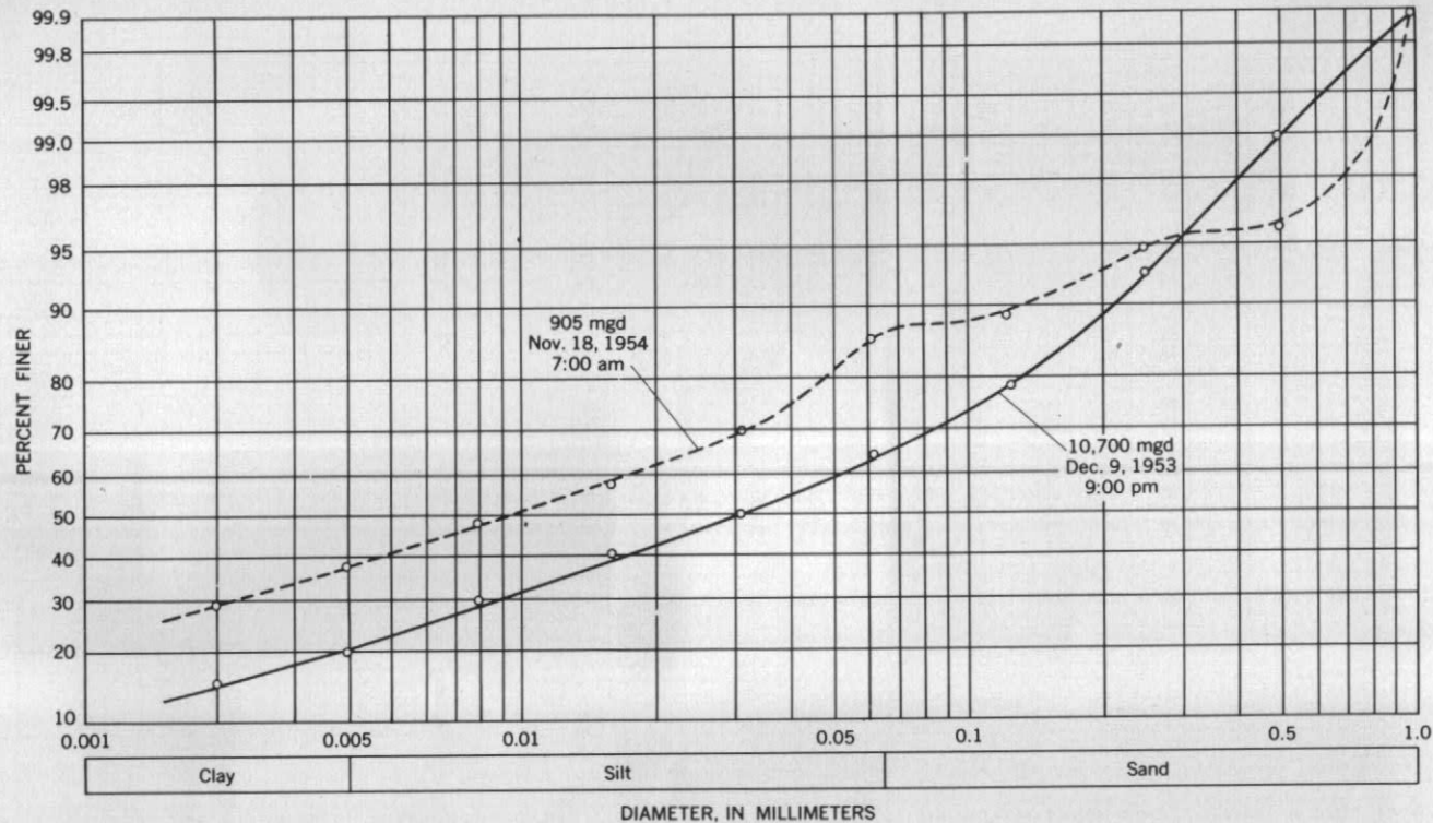
FIGURE 28.—Particle-size distribution of suspended-sediment samples analyzed in dispersion medium, Green River near Palmer.
