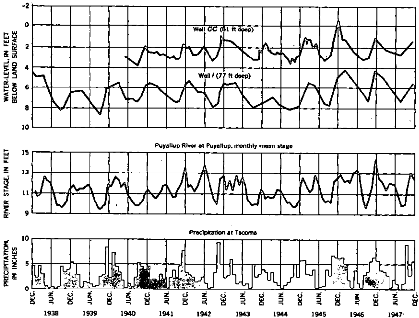
FIGURE 24.—Hydrographs of water levels in two shallow wells in the Puyallup River Valley, monthly mean stage of the Puyallup River at Puyallup, and precipitation at Tacoma.
