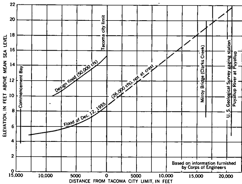
FIGURE 23.—Flood profiles on the Puyallup River from Commencement Bay to the gaging station at Puyallup.
