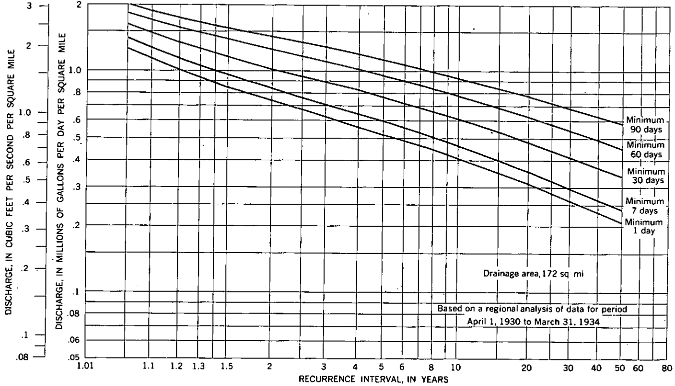
FIGURE 19.—Low-flow frequency curves, Puyallup River near Orting.
