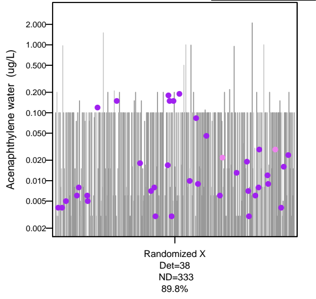
Jitter Plot
