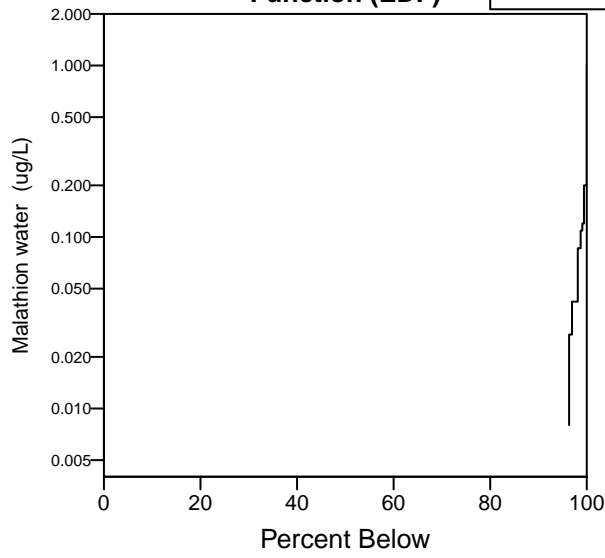
Empirical Distribution Function (EDF)
