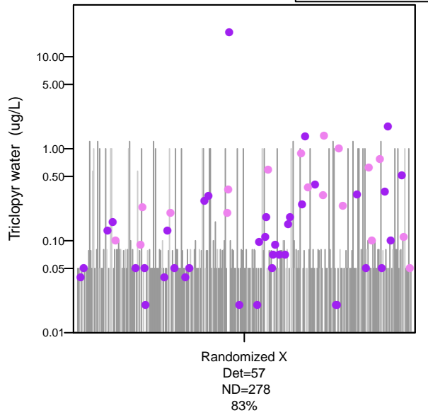
Jitter Plot
