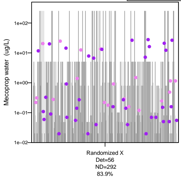
Jitter Plot
