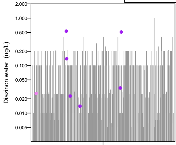
Jitter Plot
