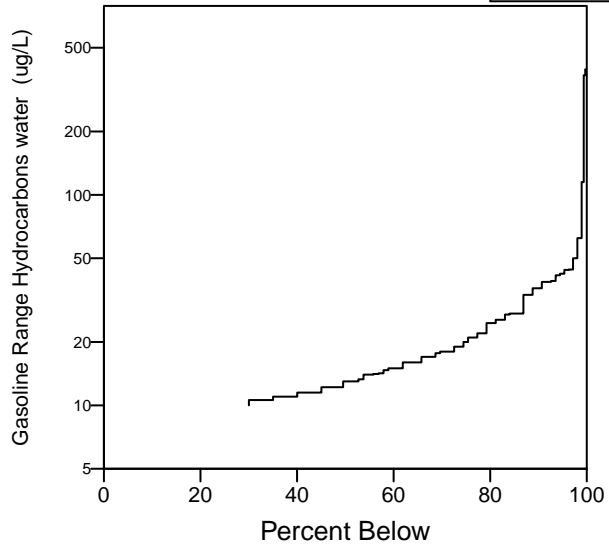
Empirical Distribution Function (EDF)
