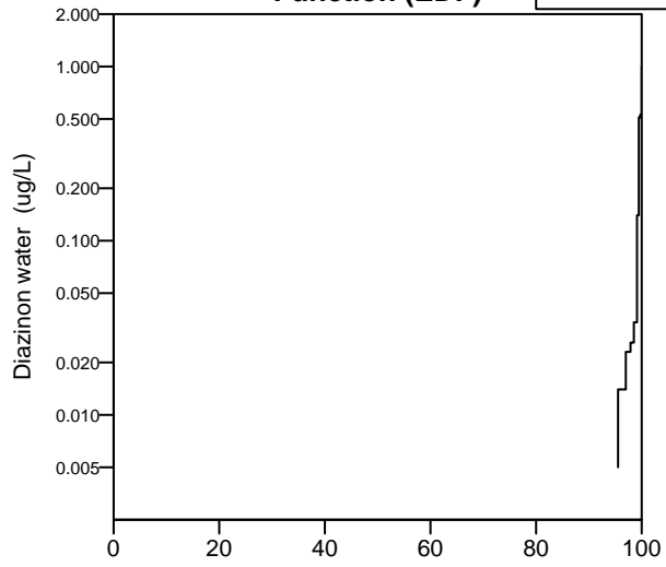
Empirical Distribution Function (EDF)
