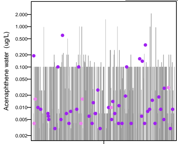
Jitter Plot
