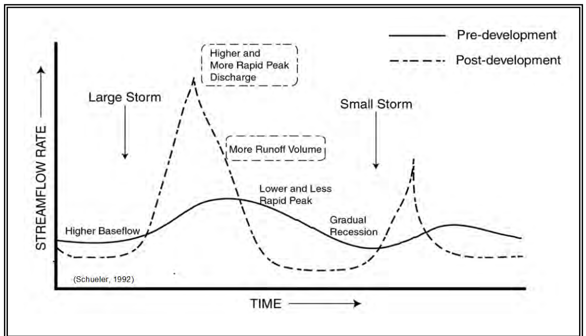
Figure 1.7.1 – Changes in Hydrology after Development
