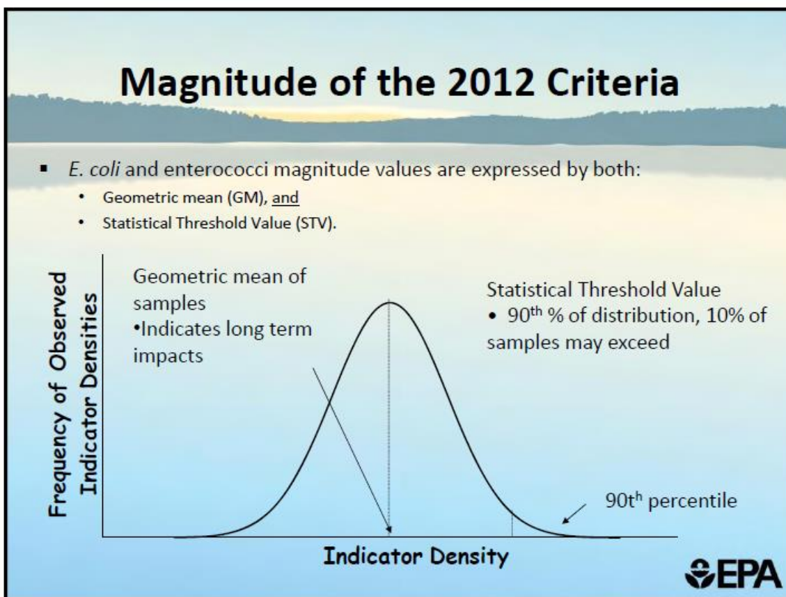
Figure 39: Comparison of geometric mean and statistical threshold values.
