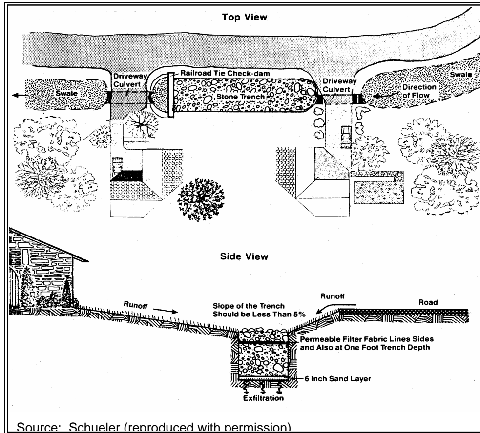
Figure 3.34 – Swale/Trench Design
