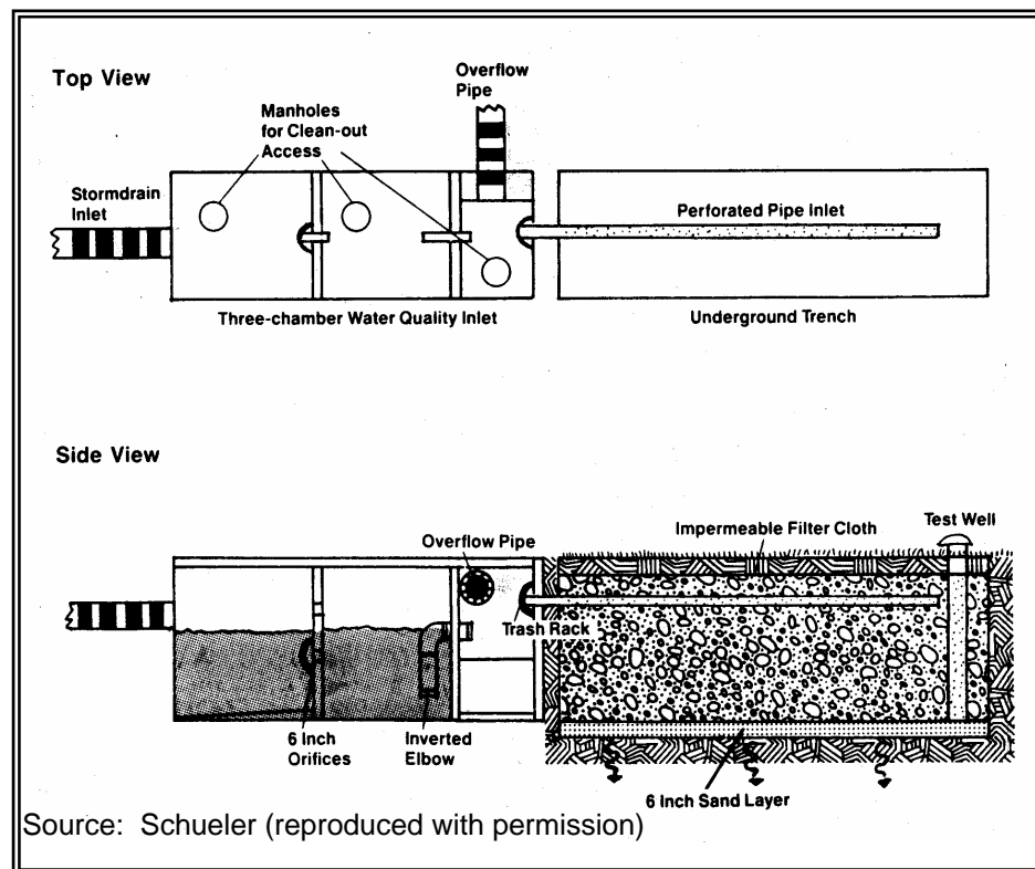
Figure 3.35 Underground Trench with Oil/Grit Chamber
