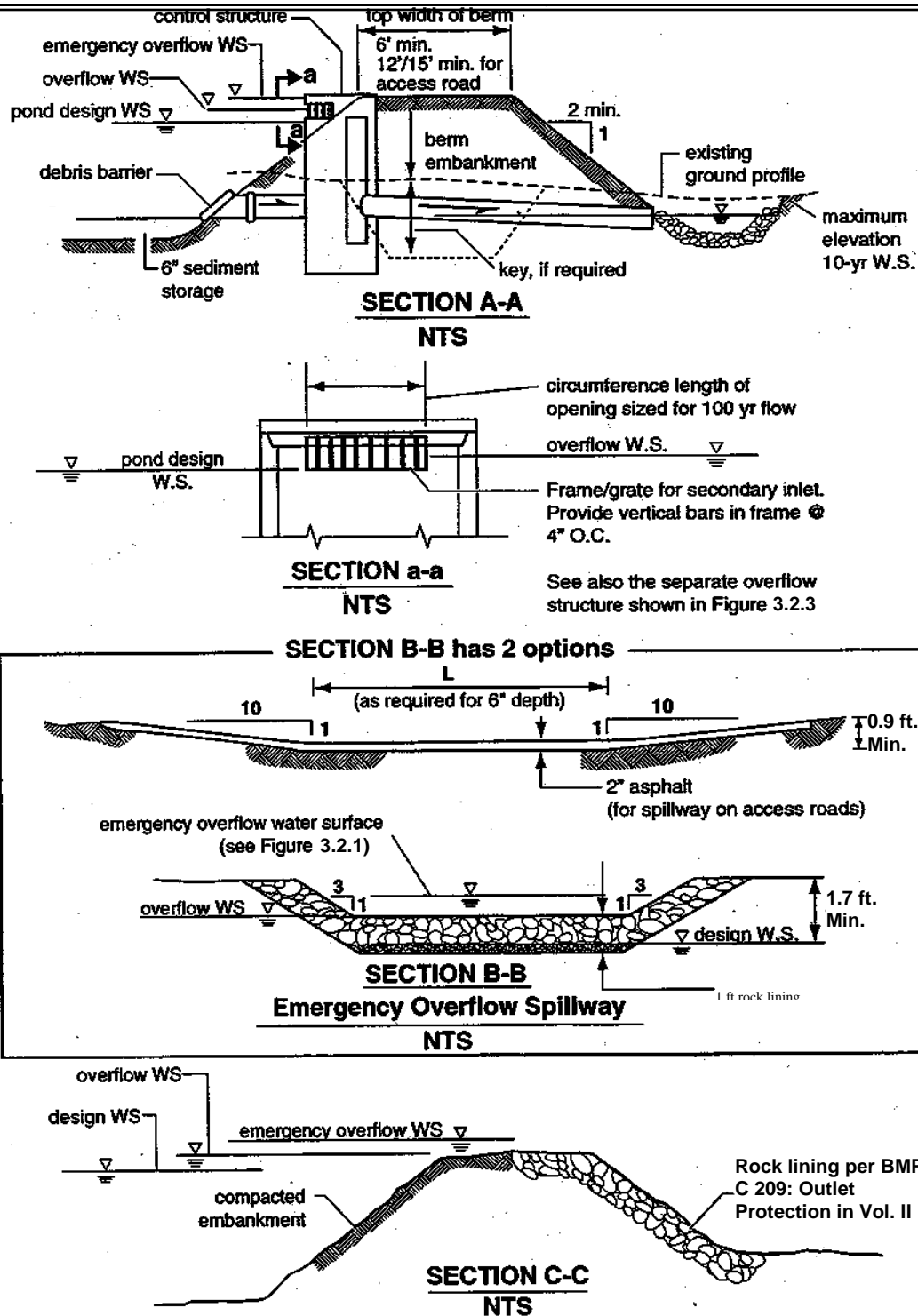
Figure 3.2.2 - Typical Detention Pond Sections
