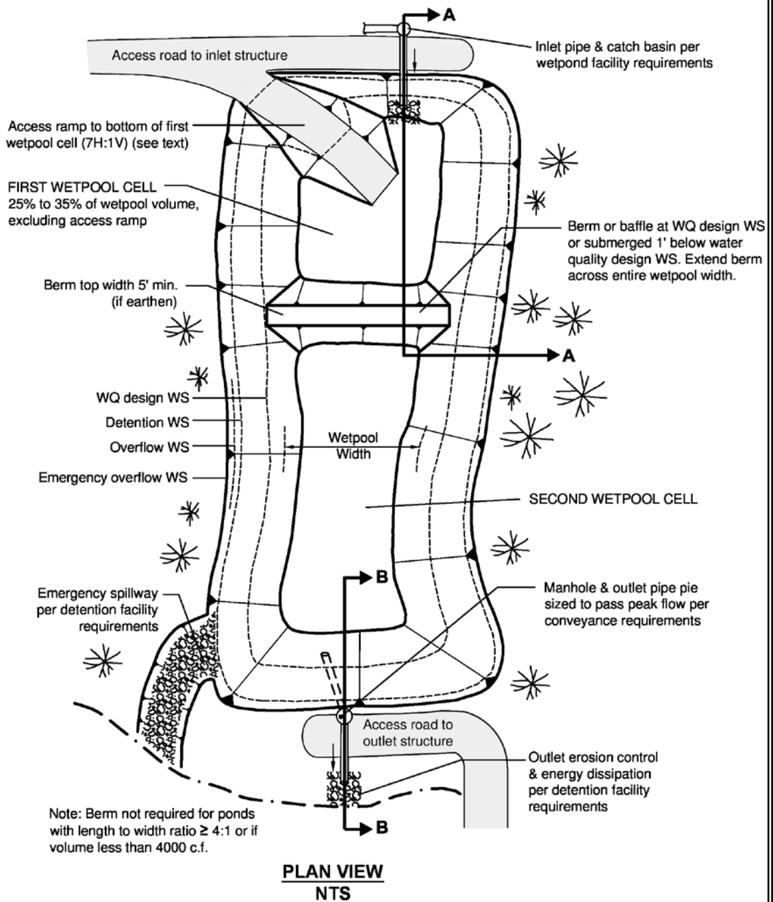
Figure 10.3.1a – Wetpond
